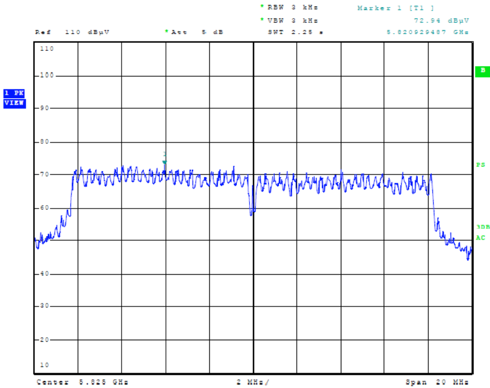
Figure Forty Plot of Power Spectral Density (n Mode, 5825 MHz)
