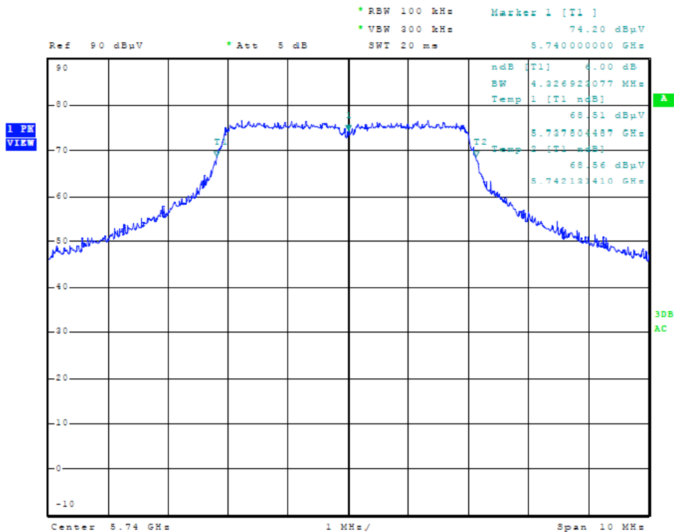
Figure Twenty-six Plot of 6dB Band width (5 MHz Mode, 5740 MHz)
