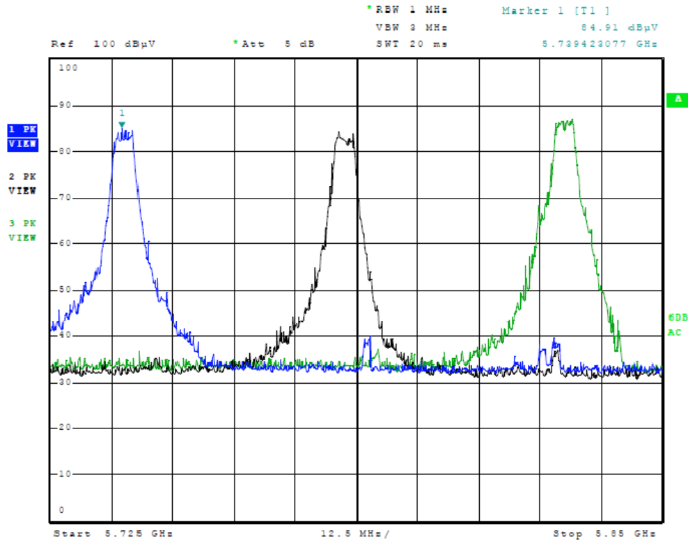
Figure Fifteen Plot of Radiated Emissions (Transmitter Operation in band, 5-MHz Mode)
