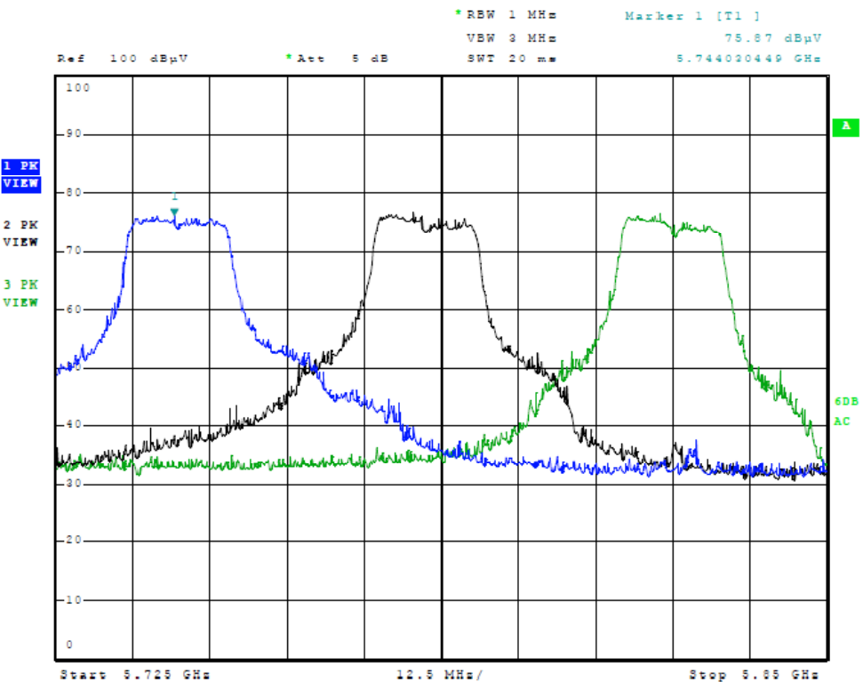
Figure Fourteen Plot of Radiated Emissions (Transmitter Operation in band, N Mode)
