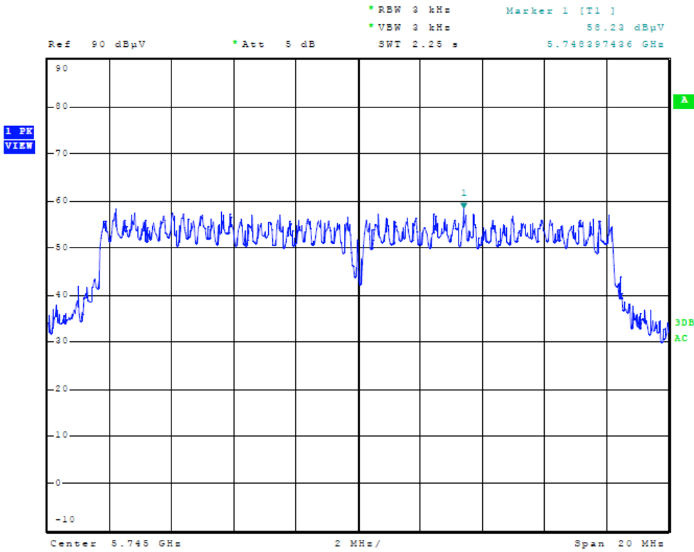
Figure Thirty-five Plot of Power Spectral Density (a/n Mode, 5745 MHz)
