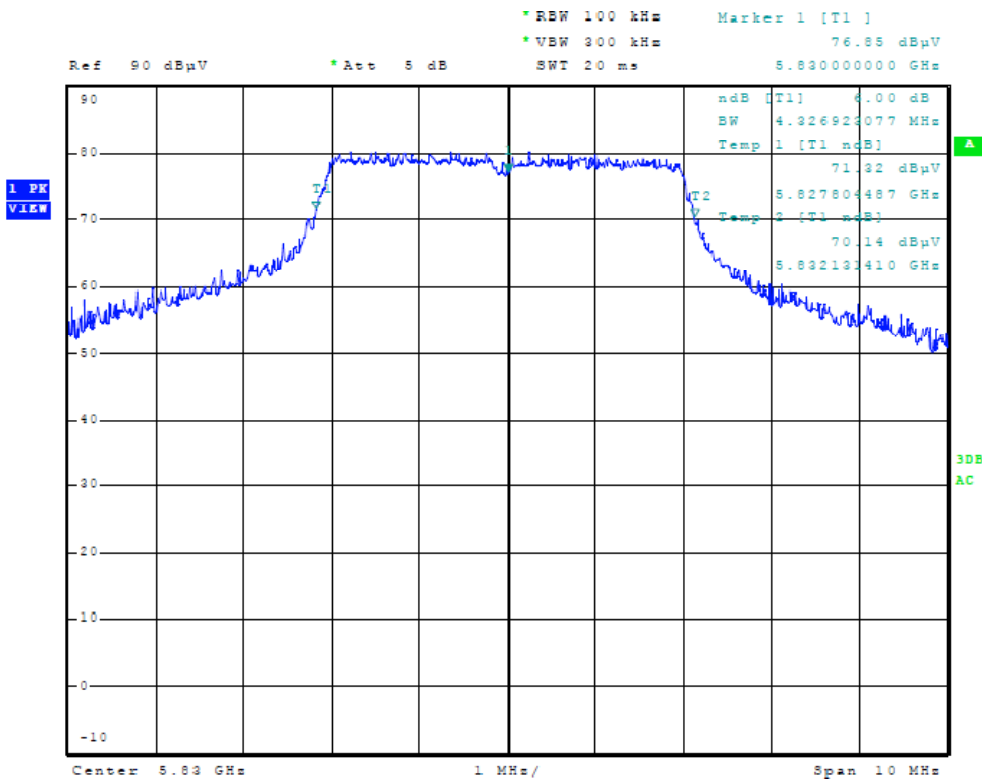
Figure Twenty-eight Plot of 6dB Band width (5 MHz Mode, 5830 MHz)
