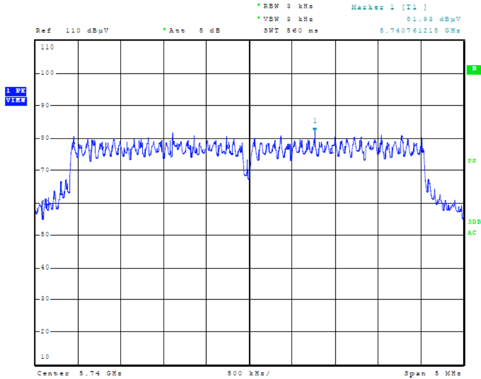
Figure Forty-one Plot of Power Spectral Density (5 MHz Mode, 5740 MHz)
