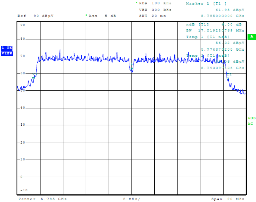
Figure Twenty-one Plot of 6dB Band width (a/n Mode, 5785 MHz)
