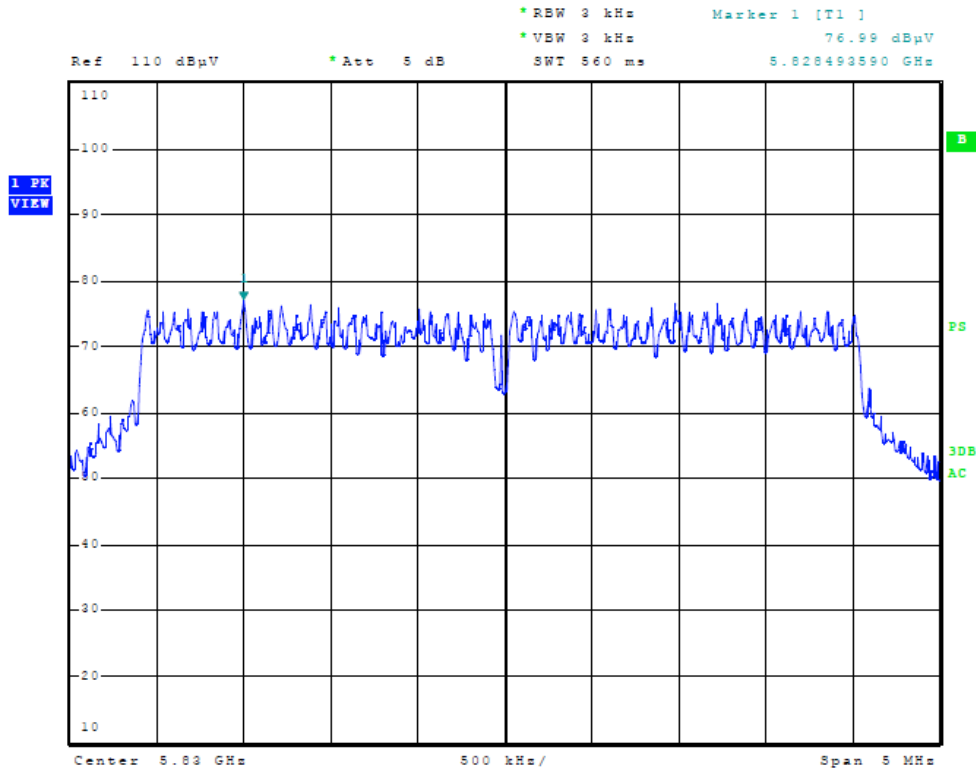
Figure Forty-three Plot of Power Spectral Density (5 MHz Mode, 5830 MHz)
