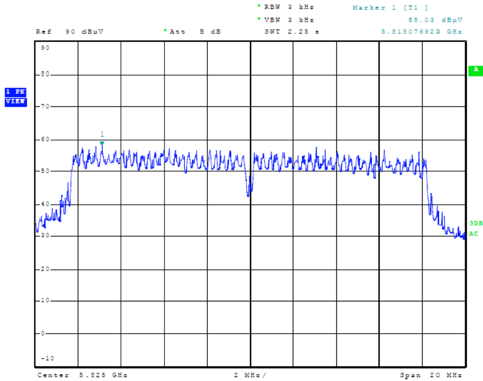
Figure Thirty-seven Plot of Power Spectral Density (a/n Mode, 5825 MHz)
