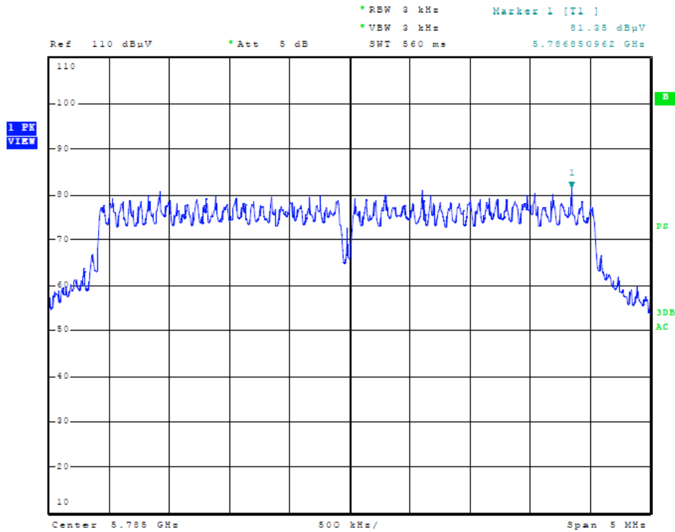
Figure Forty-two Plot of Power Spectral Density (5 MHz Mode, 5785 MHz)
