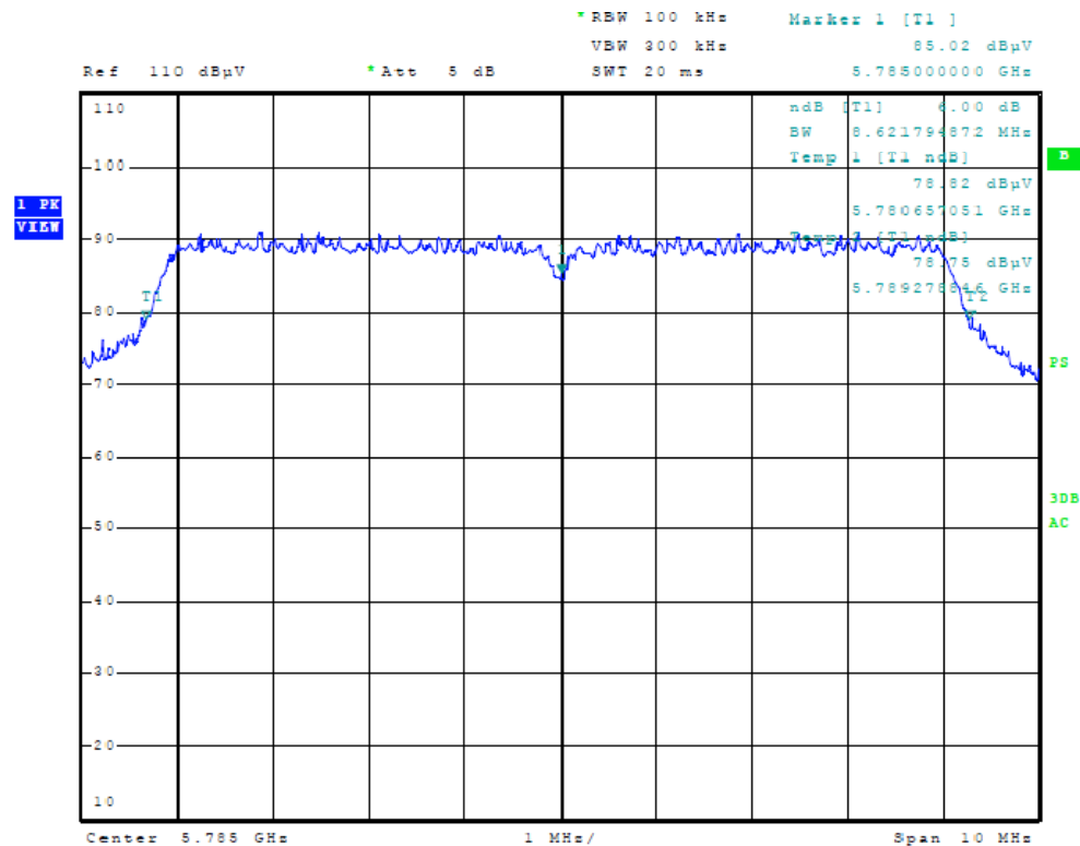
Figure Thirty Plot of 6dB Band width (10 MHz Mode, 5785 MHz)
