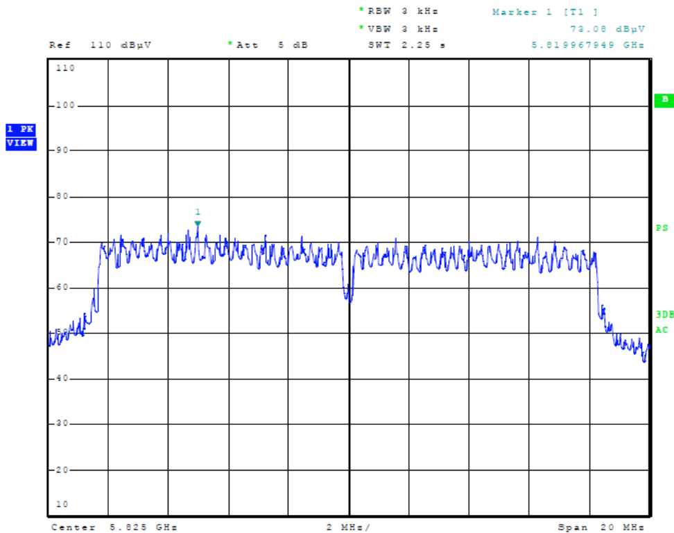
Figure Thirty-four Plot of Power Spectral Density (5GHz Mode, 5825 MHz)
