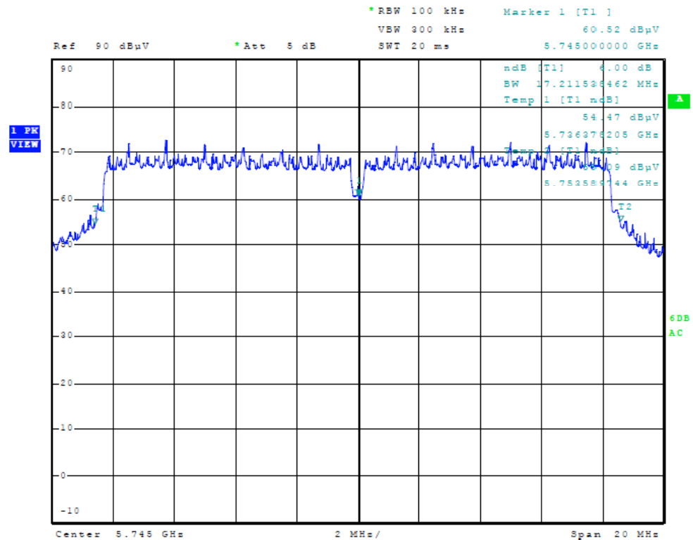
Figure Twenty Plot of 6dB Band width (a/n Mode, 5745 MHz)
