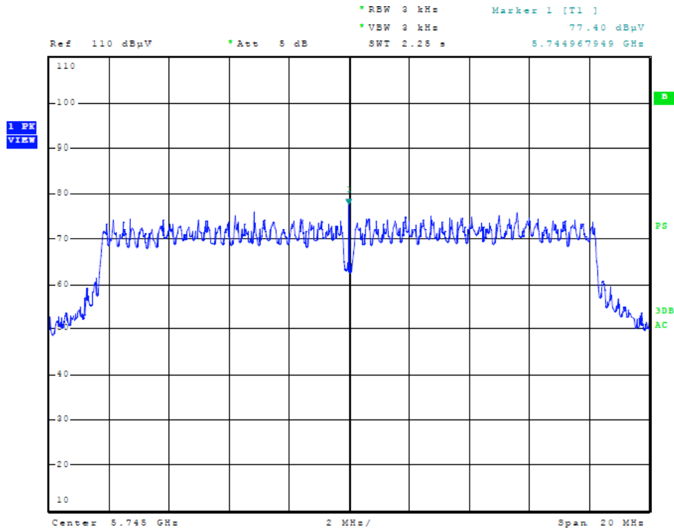
Figure Thirty-eight Plot of Power Spectral Density (n Mode, 5745 MHz)
