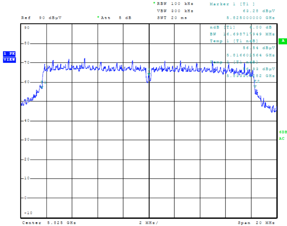
Figure Twenty-five Plot of 6dB Band width (n Mode, 5825 MHz)
