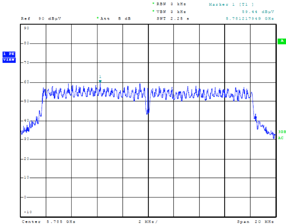
Figure Thirty-six Plot of Power Spectral Density (a/n Mode, 5785 MHz)
