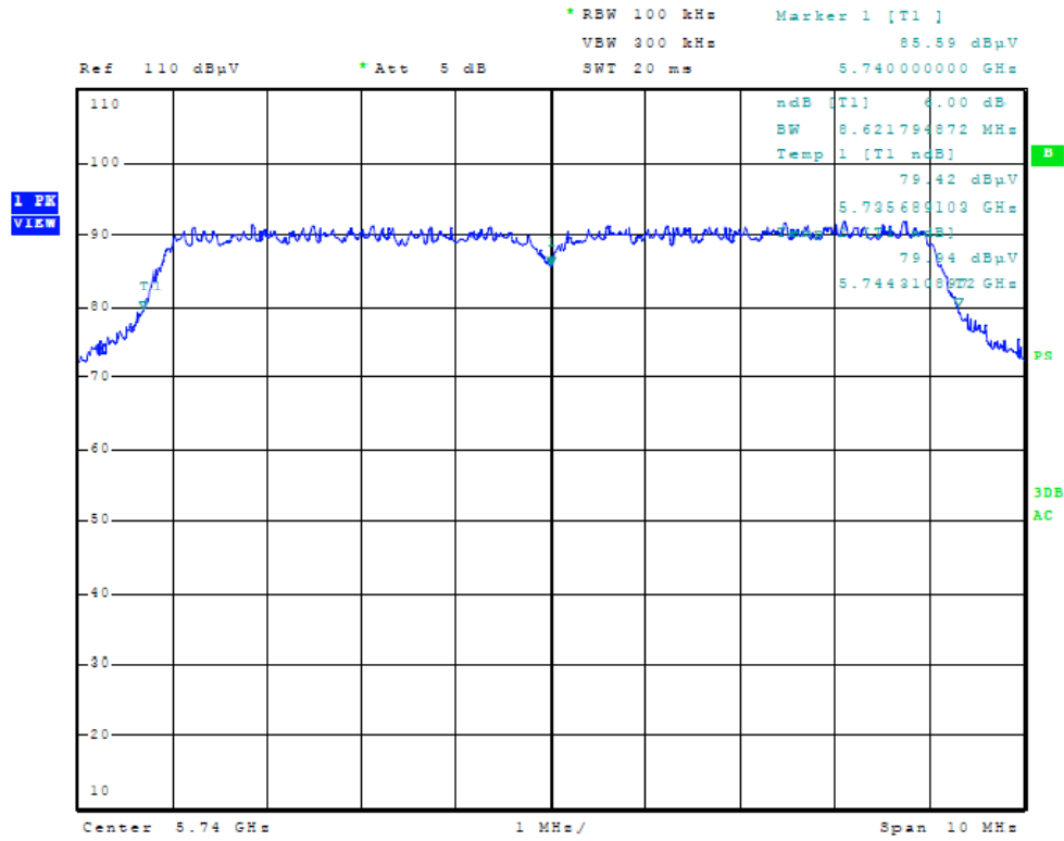
Figure Twenty-nine Plot of 6dB Band width (10 MHz Mode, 5740 MHz)
