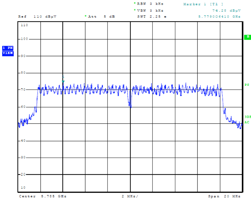
Figure Thirty-three Plot of Power Spectral Density (5GHz Mode, 5785 MHz)
