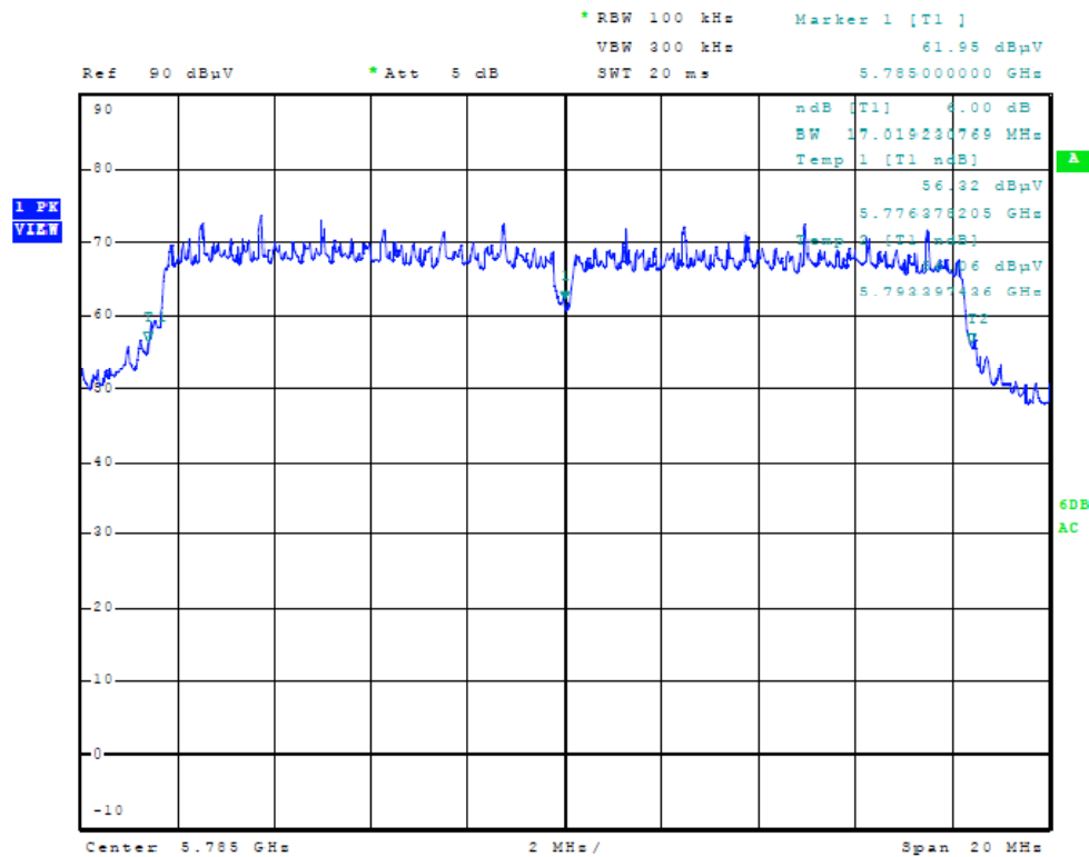
Figure Twenty-four Plot of 6dB Band width (n Mode, 5785 MHz)
