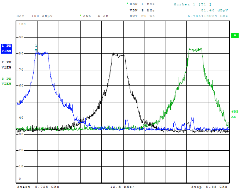
Figure Sixteen Plot of Radiated Emissions (Transmitter Operation in band, 10-MHz Mode)
