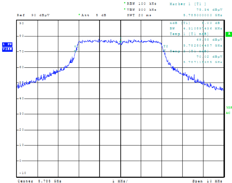
Figure Twenty-seven Plot of 6dB Band width (5 MHz Mode, 5785 MHz)
