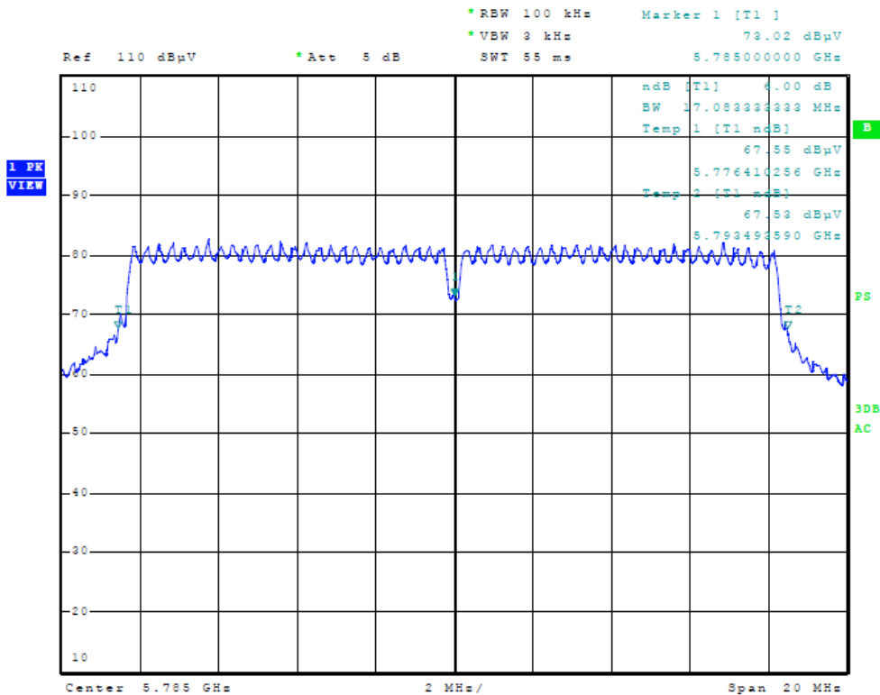
Figure Eighteen Plot of 6dB Band width (5GHz Mode, 5785 MHz)
