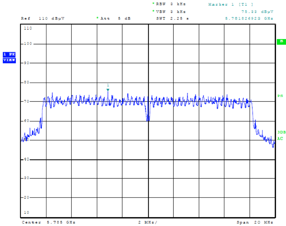
Figure Thirty-nine Plot of Power Spectral Density (n Mode, 5785 MHz)
