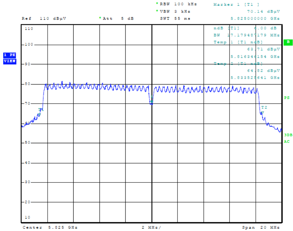
Figure Nineteen Plot of 6dB Band width (5GHz Mode, 5825 MHz)
