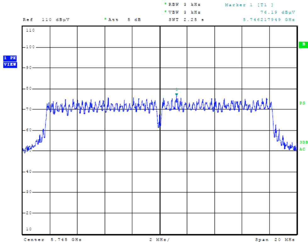
Figure Thirty-two Plot of Power Spectral Density (5GHz Mode, 5745 MHz)
