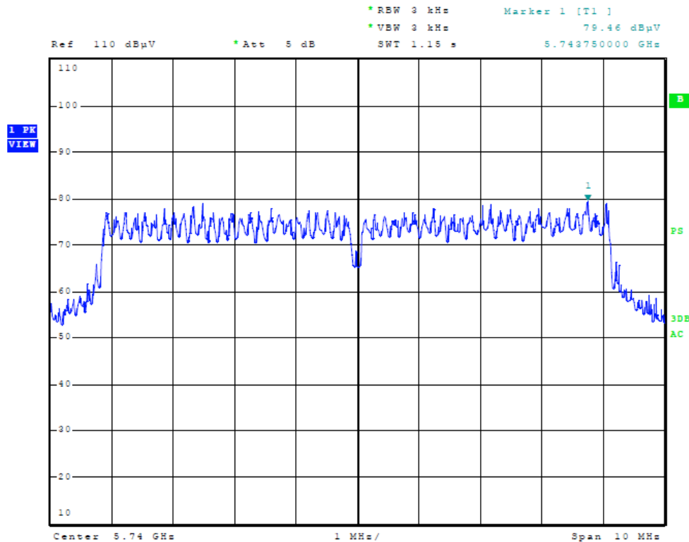
Figure Forty-four Plot of Power Spectral Density (10 MHz Mode, 5740 MHz)
