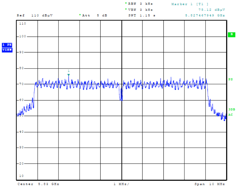
Figure Forty-six Plot of Power Spectral Density (10 MHz Mode, 5830 MHz)
