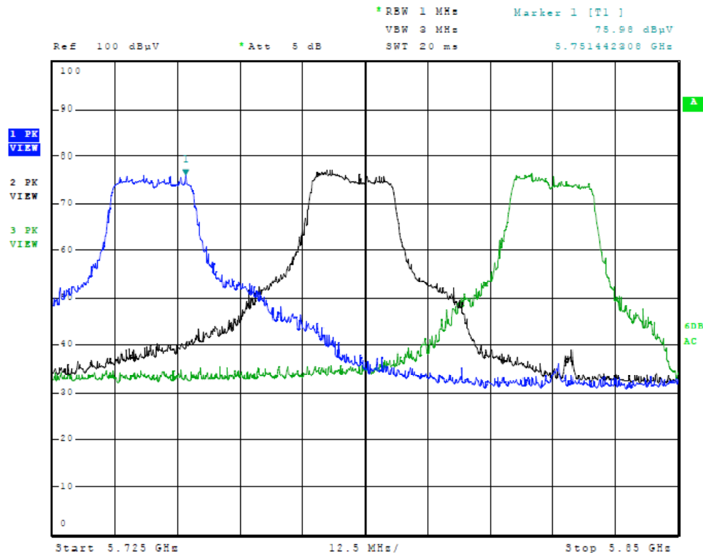
Figure Twelve Plot of Radiated Emissions (Transmitter Operation in band, 5GHz Mode)
