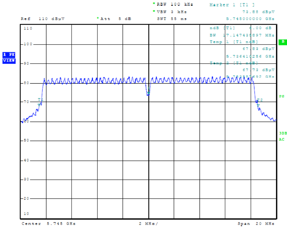
Figure Seventeen Plot of 6dB Band width (5GHz Mode, 5745 MHz)
