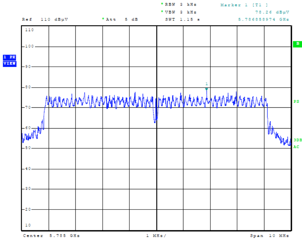
Figure Forty-five Plot of Power Spectral Density (10 MHz Mode, 5785 MHz)
