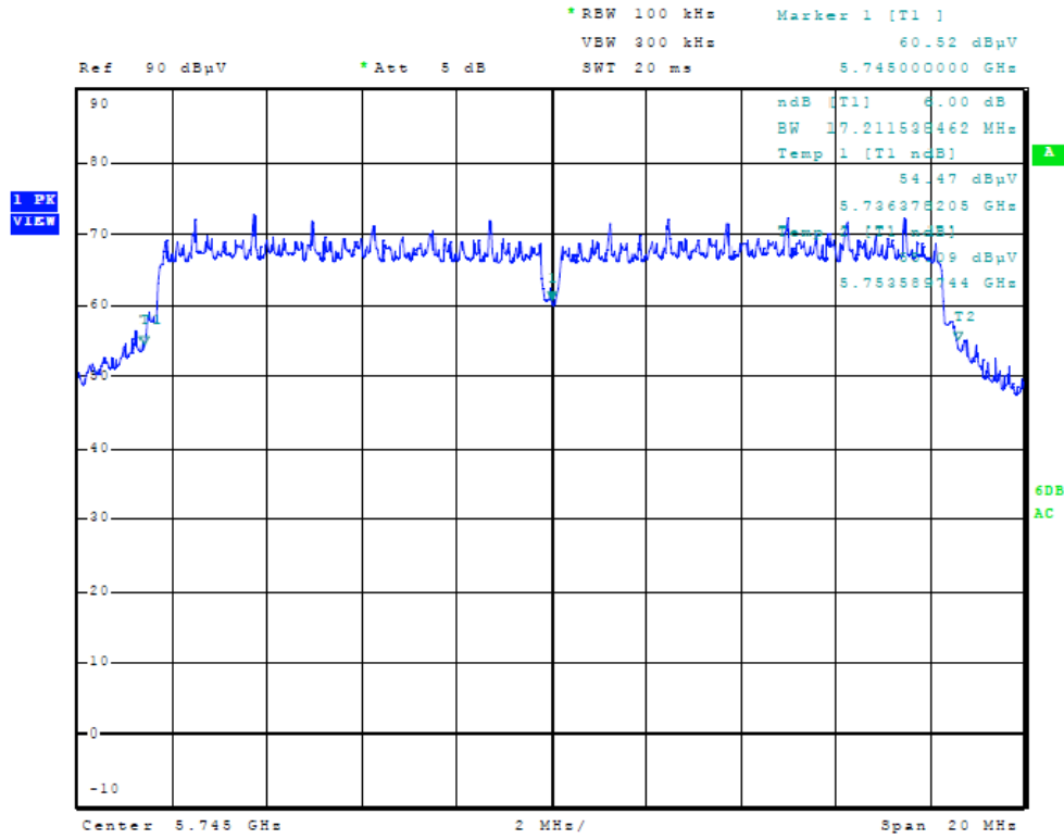
Figure Twenty-three Plot of 6dB Band width (n Mode, 5745 MHz)
