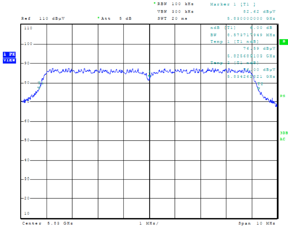
Figure Thirty-one Plot of 6dB Band width (10 MHz Mode, 5830 MHz)
