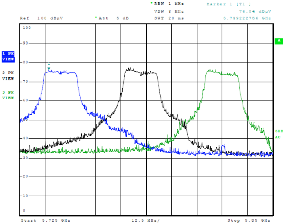
Figure Thirteen Plot of Radiated Emissions (Transmitter Operation in band, a/n Mode)
