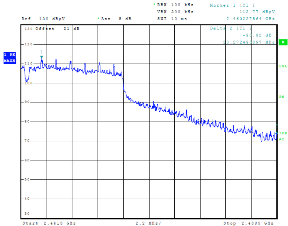
Figure 6 Plot of High Band Edge
