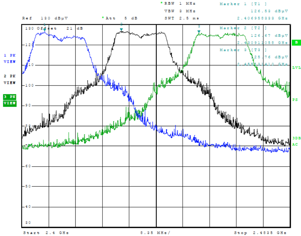
Figure 3 Plot of Transmitter Emissions (Across Operational Band, 20MHz Mode)
