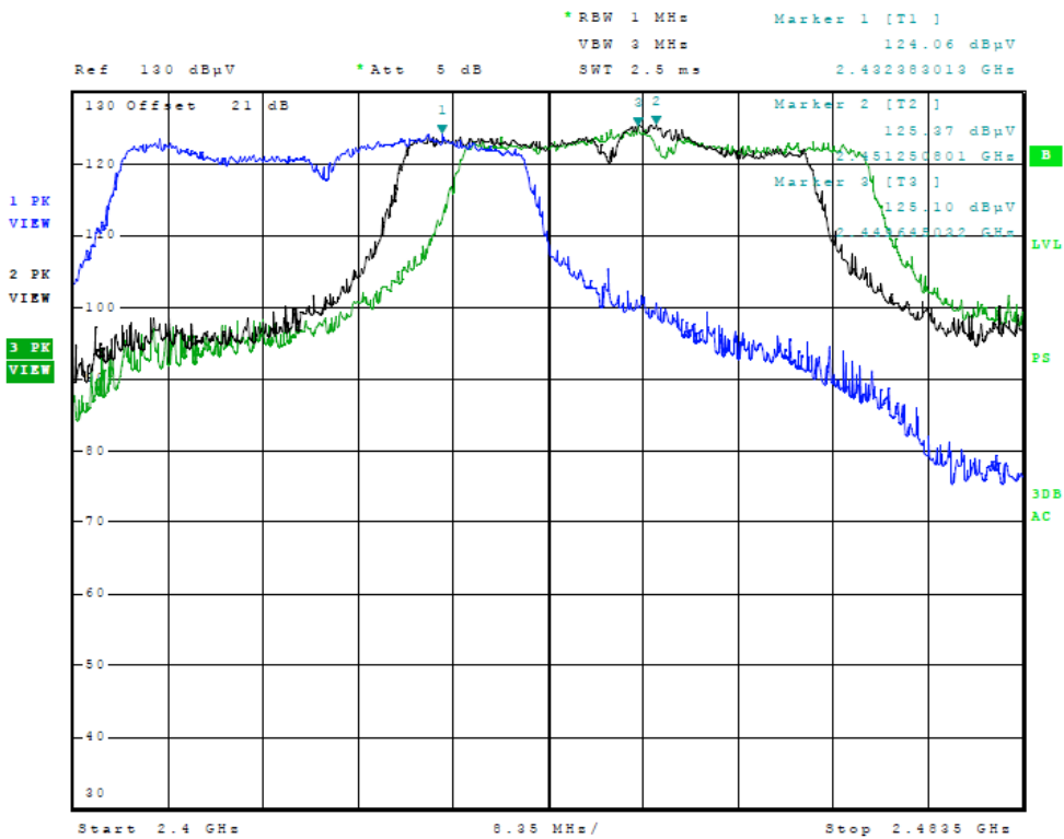
Figure 4 Plot of Transmitter Emissions (Across Operational Band, 40 MHz Mode)
