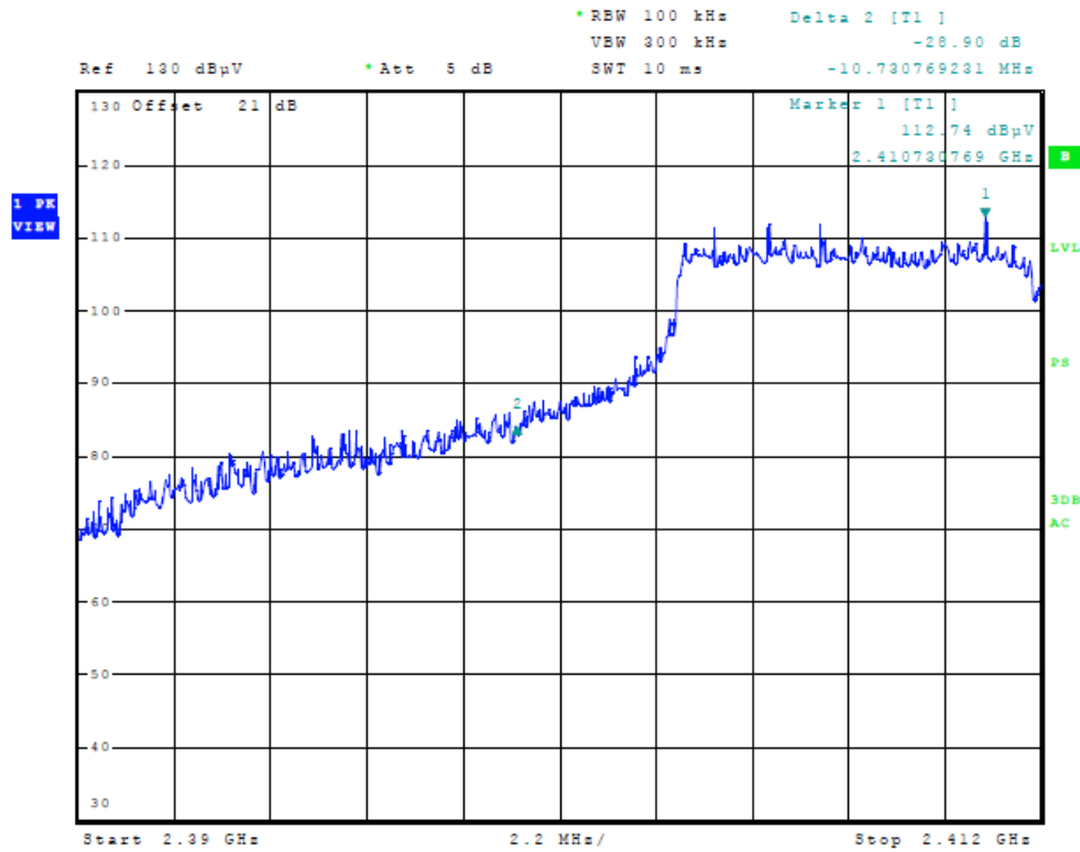
Figure 5 Plot of Low Band Edge
