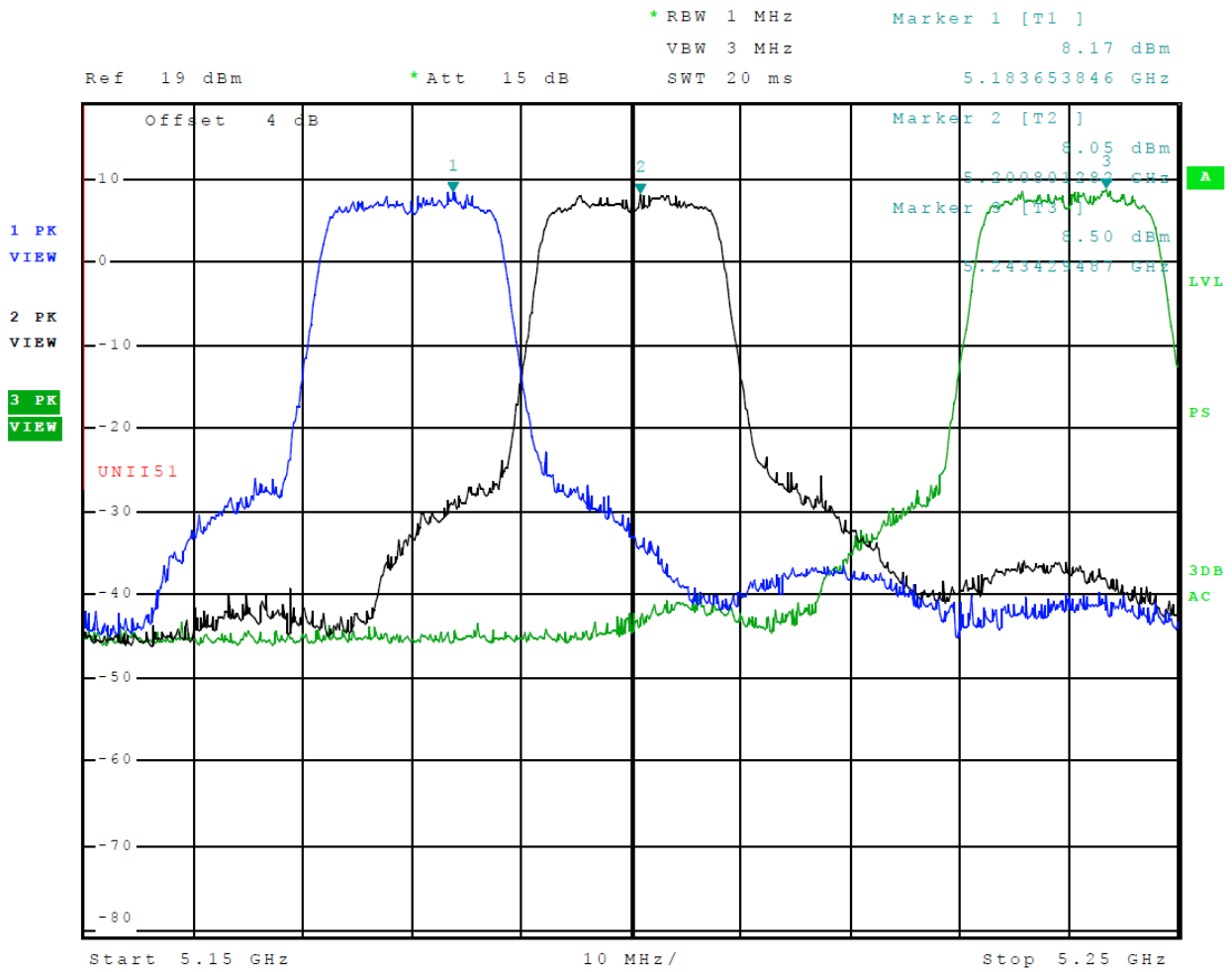
Figure 5 Plot of Transmitter Emissions (Across 5150-5250 MHz Band, Chain 0, 802.11n)
