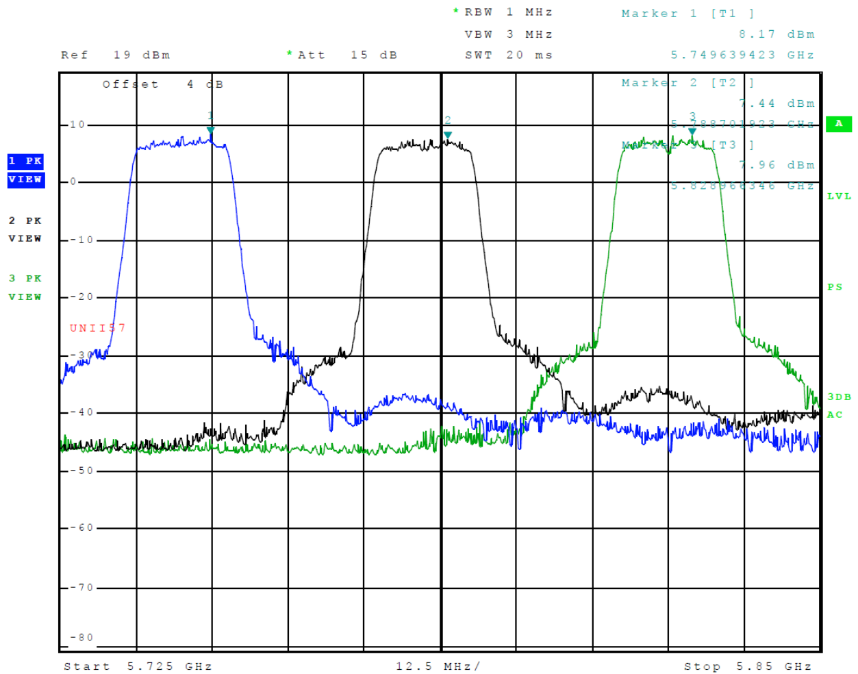
Figure 43 Plot of Transmitter Emissions (Across 5725-5850 MHz Band, Chain 0, 802.11a)
