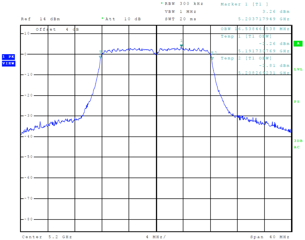
Figure 31 Plot of Transmitter Emissions (5150-5250 MHz Band, 802.11n, Chain 0, 99% OBW)
