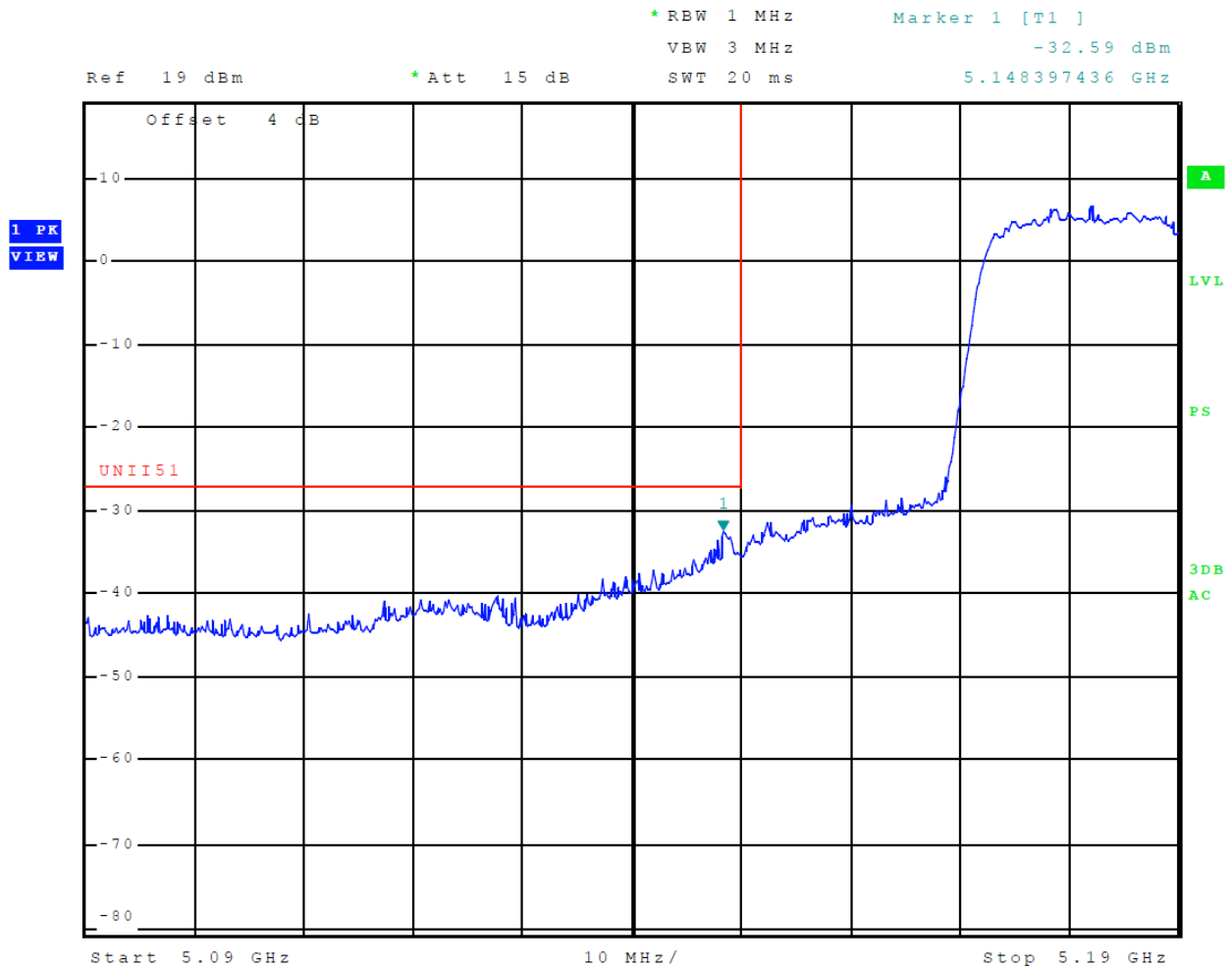
Figure 16 Plot of Transmitter Low Band Edge (5150-5250 MHz Band, Chain 1, 802.11n40)
