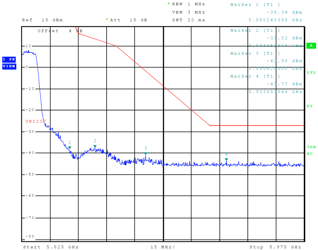
Figure 60 Plot of Transmitter High Band Edge (5725-5850 MHz Band, Chain 1, 802.11a)
