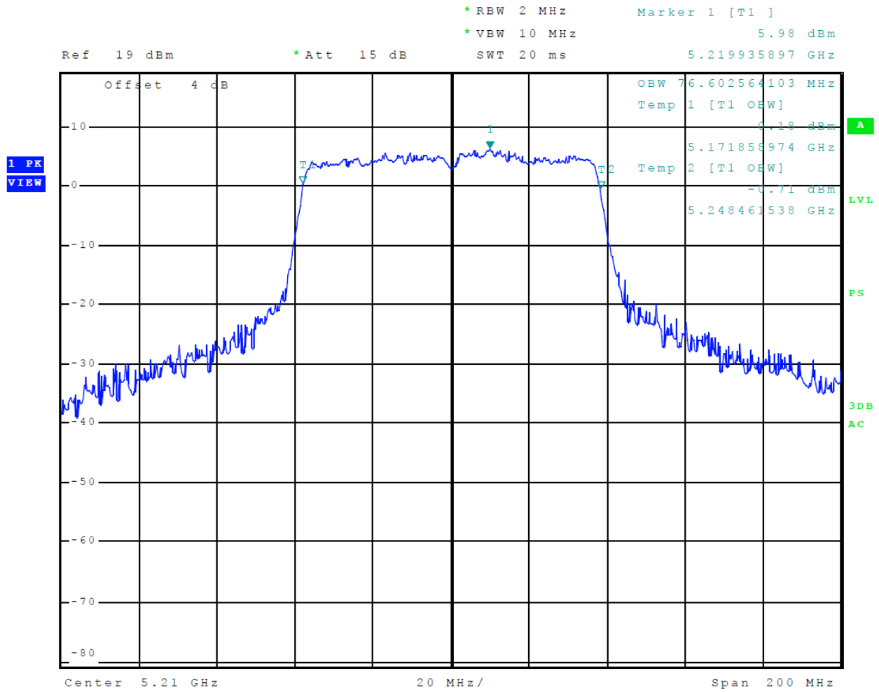
Figure 39 Plot of Transmitter Emissions (5150-5250 MHz Band, 802.11ac, Chain 0, 99% OBW)
