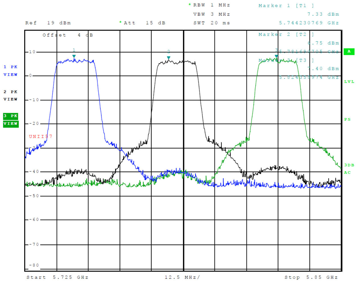
Figure 46 Plot of Transmitter Emissions (Across 5725-5850 MHz Band, Chain 1, 802.11n)
