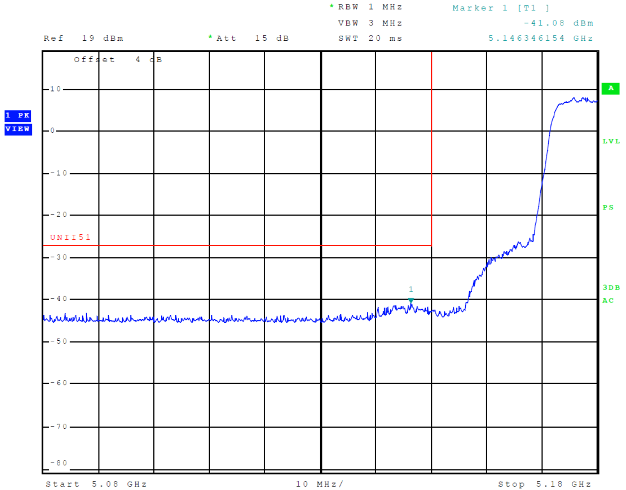
Figure 11 Plot of Transmitter Low Band Edge (5150-5250 MHz Band, Chain 0, 802.11a)
