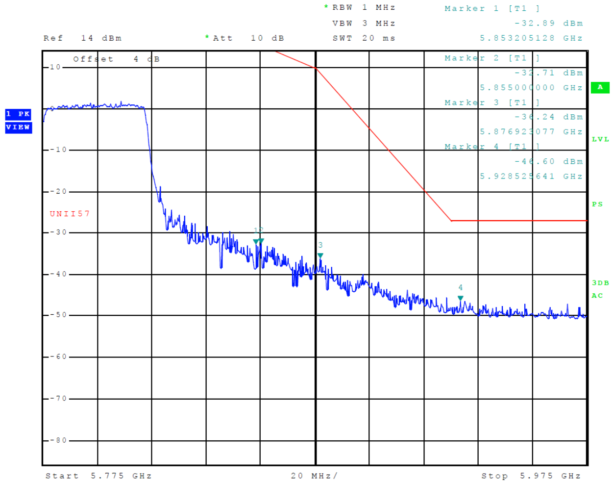
Figure 65 Plot of Transmitter High Band Edge (5725-5850 MHz Band, Chain 0, 802.11ac)
