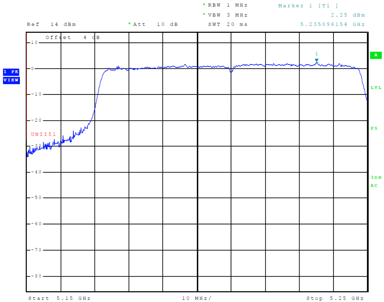
Figure 9 Plot of Transmitter Emissions (Across 5150-5250 MHz Band, Chain 0, 802.11ac)
