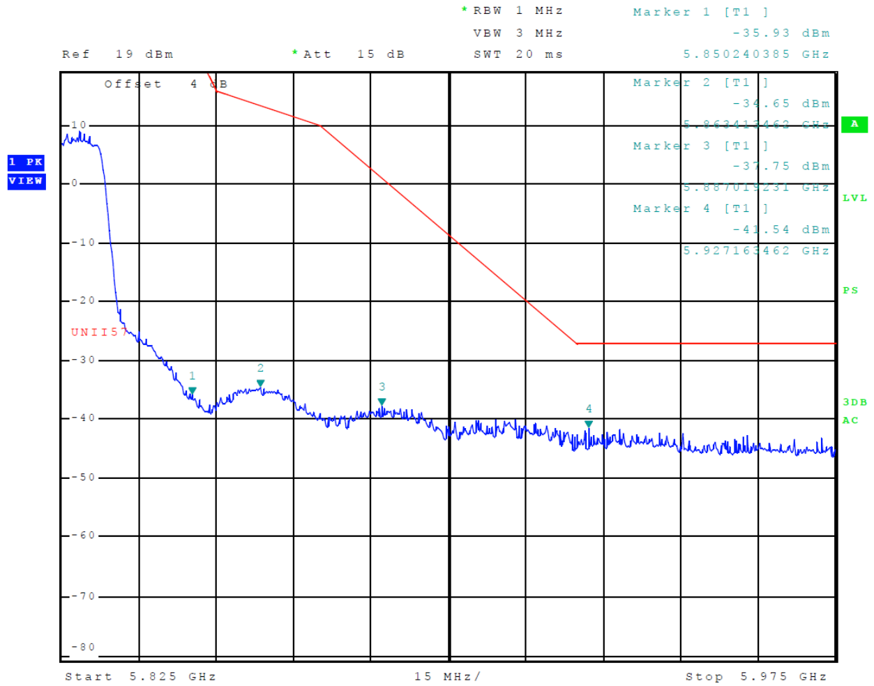
Figure 61 Plot of Transmitter High Band Edge (5725-5850 MHz Band, Chain 0, 802.11n)
