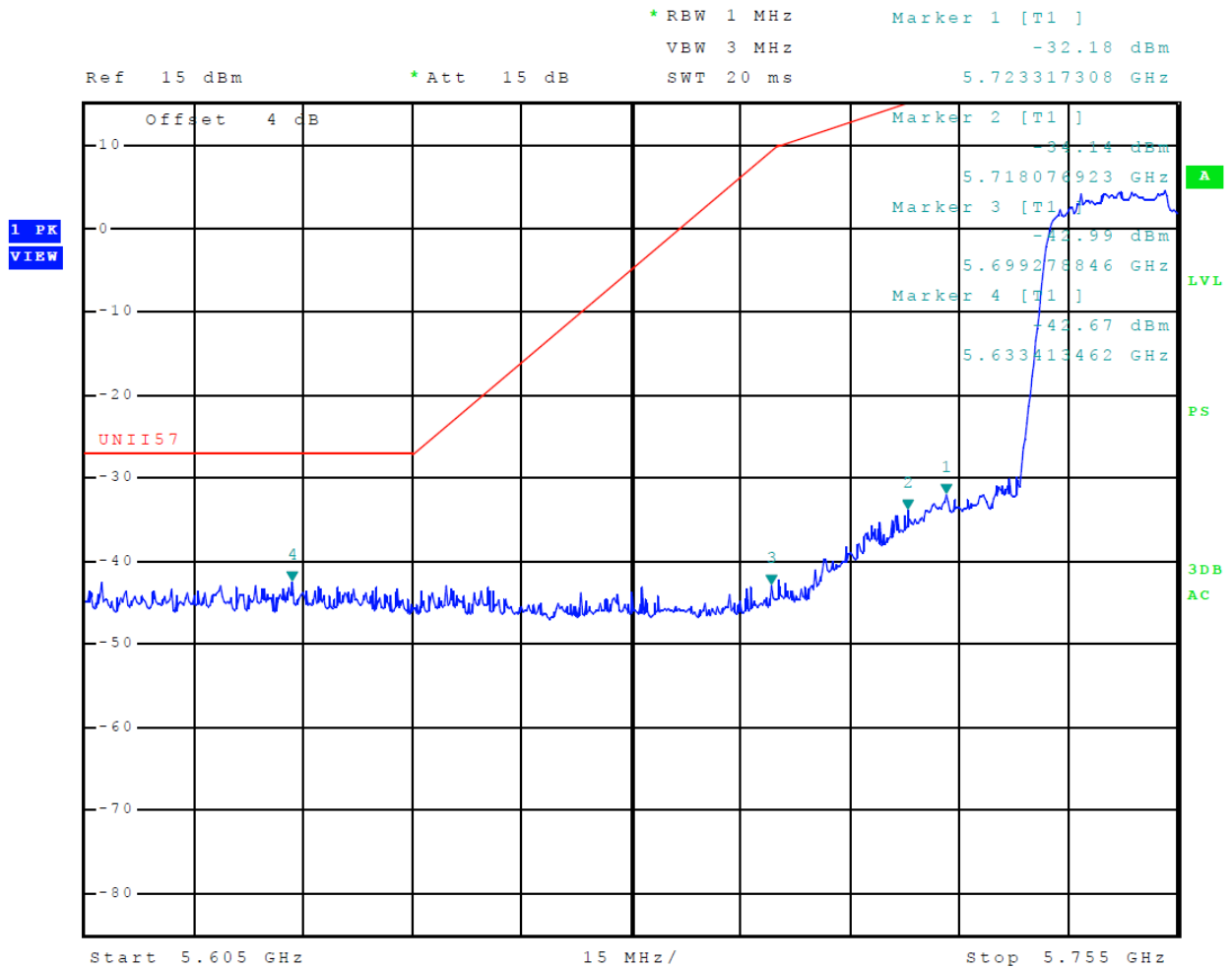
Figure 55 Plot of Transmitter Low Band Edge (5725-5850 MHz Band, Chain 0, 802.11n40)
