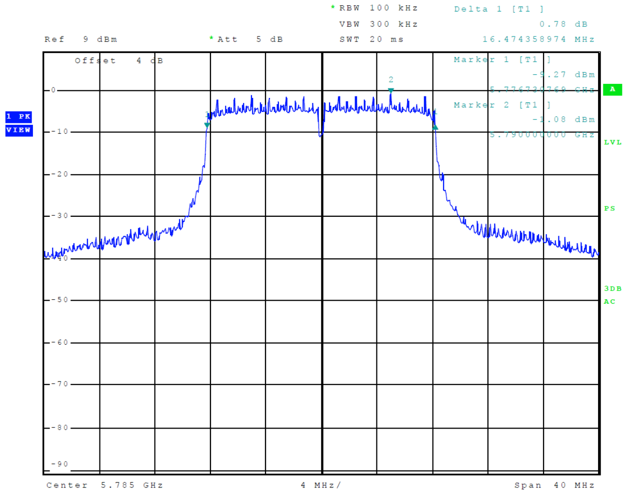
Figure 74 Plot of Transmitter Emissions (5725-5850 MHz Band, 802.11n, Chain 1, 6-dB OBW)
