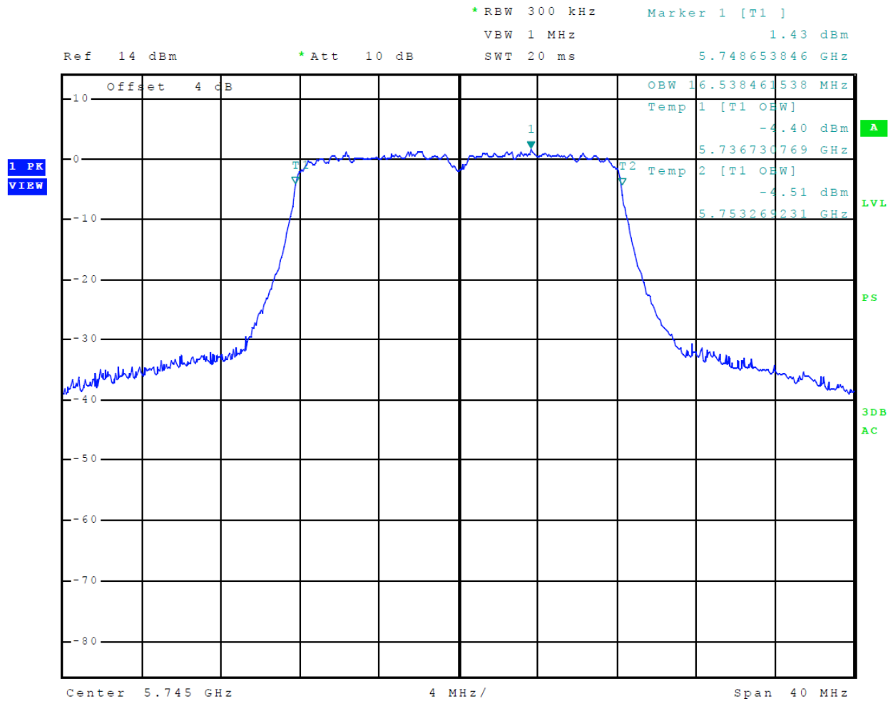
Figure 67 Plot of Transmitter Emissions (5725-5850 MHz Band, 802.11a, Chain 0, 99% OBW)
