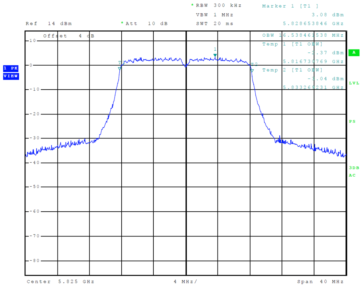
Figure 71 Plot of Transmitter Emissions (5725-5850 MHz Band, 802.11n, Chain 0, 99% OBW)
