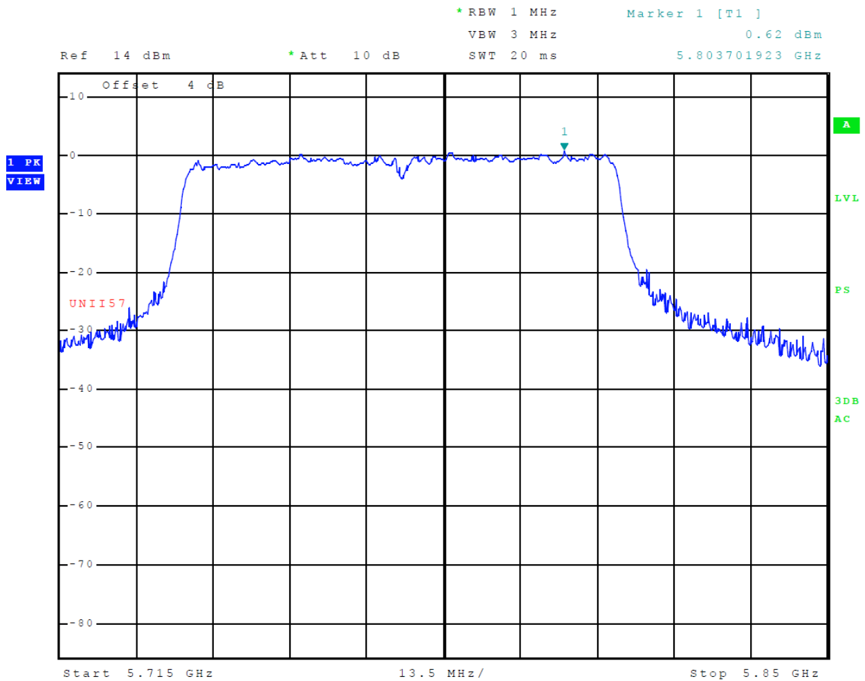
Figure 50 Plot of Transmitter Emissions (Across 5725-5850 MHz Band, Chain 1, 802.11ac)
