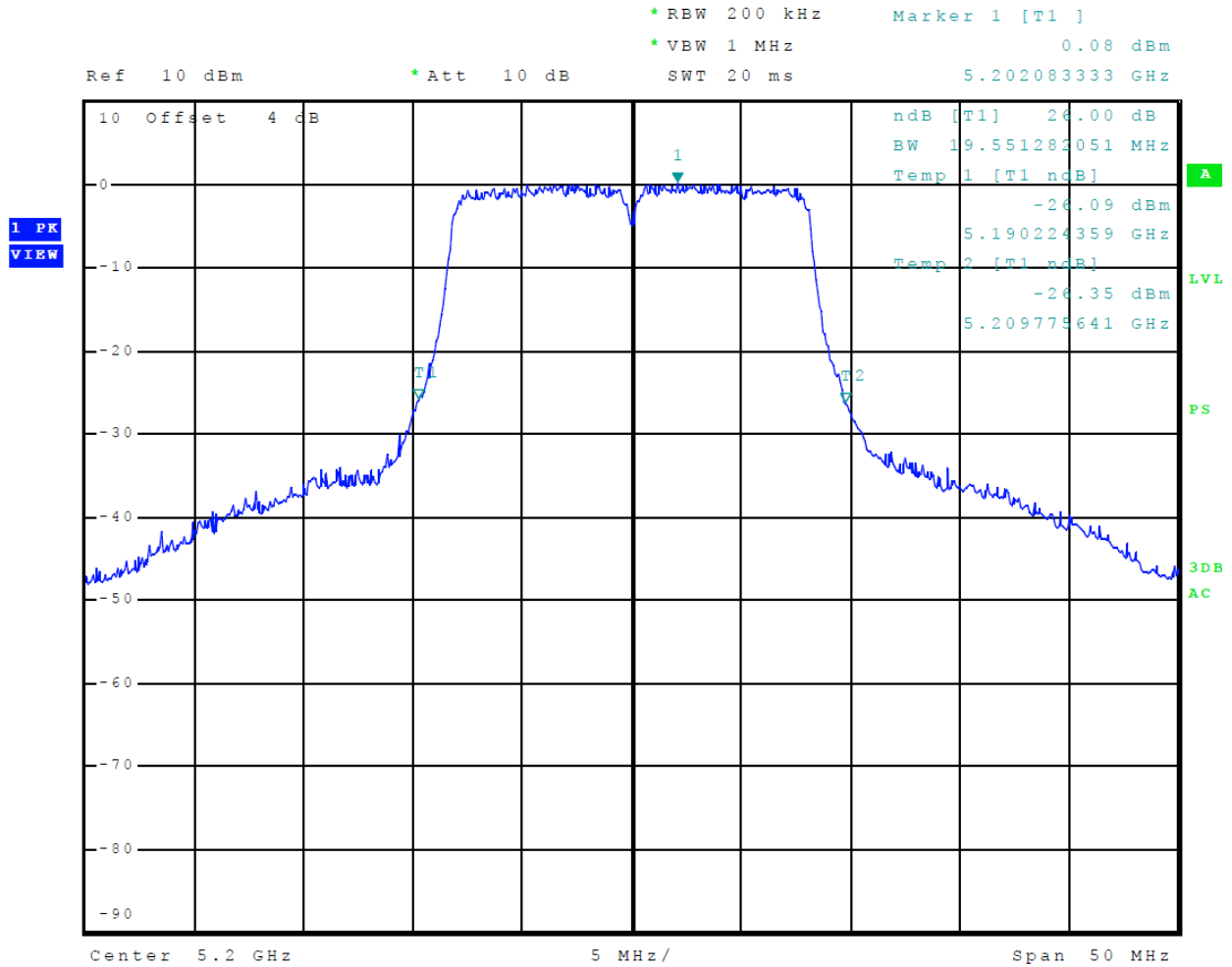
Figure 29 Plot of Transmitter Emissions (5150-5250 MHz Band, 802.11a, Chain 0, 26 dB OBW)
