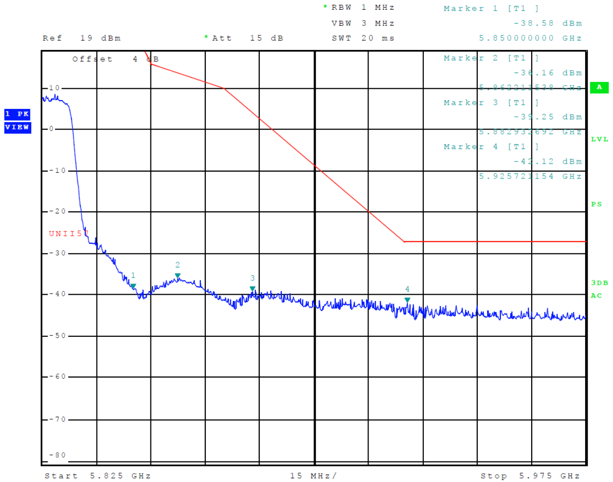
Figure 59 Plot of Transmitter High Band Edge (5725-5850 MHz Band, Chain 0, 802.11a)
