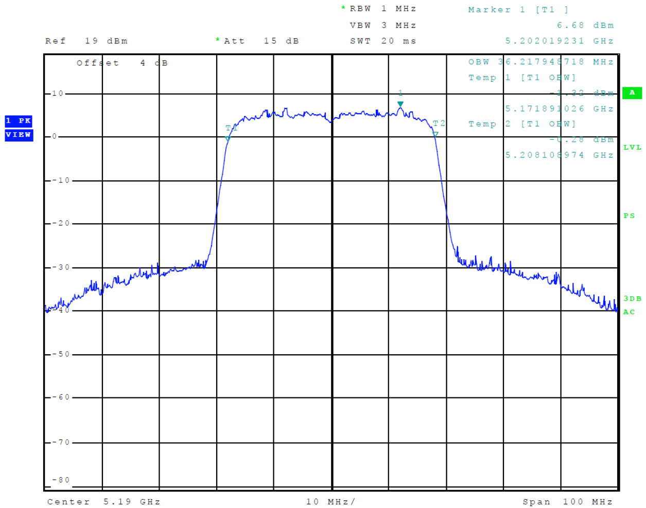
Figure 36 Plot of Transmitter Emissions (5150-5250 MHz Band, 802.11n40, Chain 1, 99% OBW)
