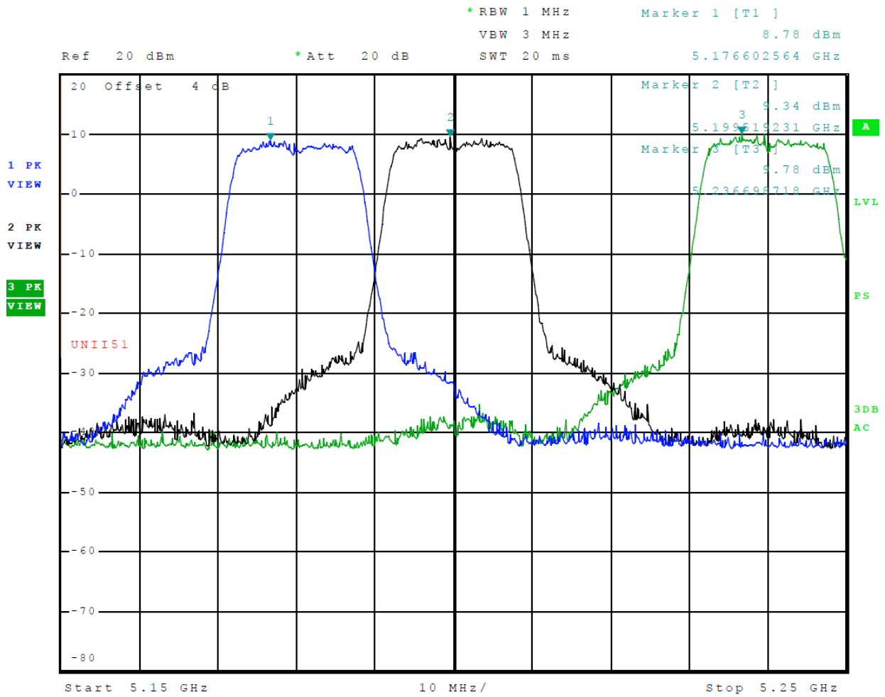
Figure 6 Plot of Transmitter Emissions (Across 5150-5250 MHz Band, Chain 1, 802.11n)
