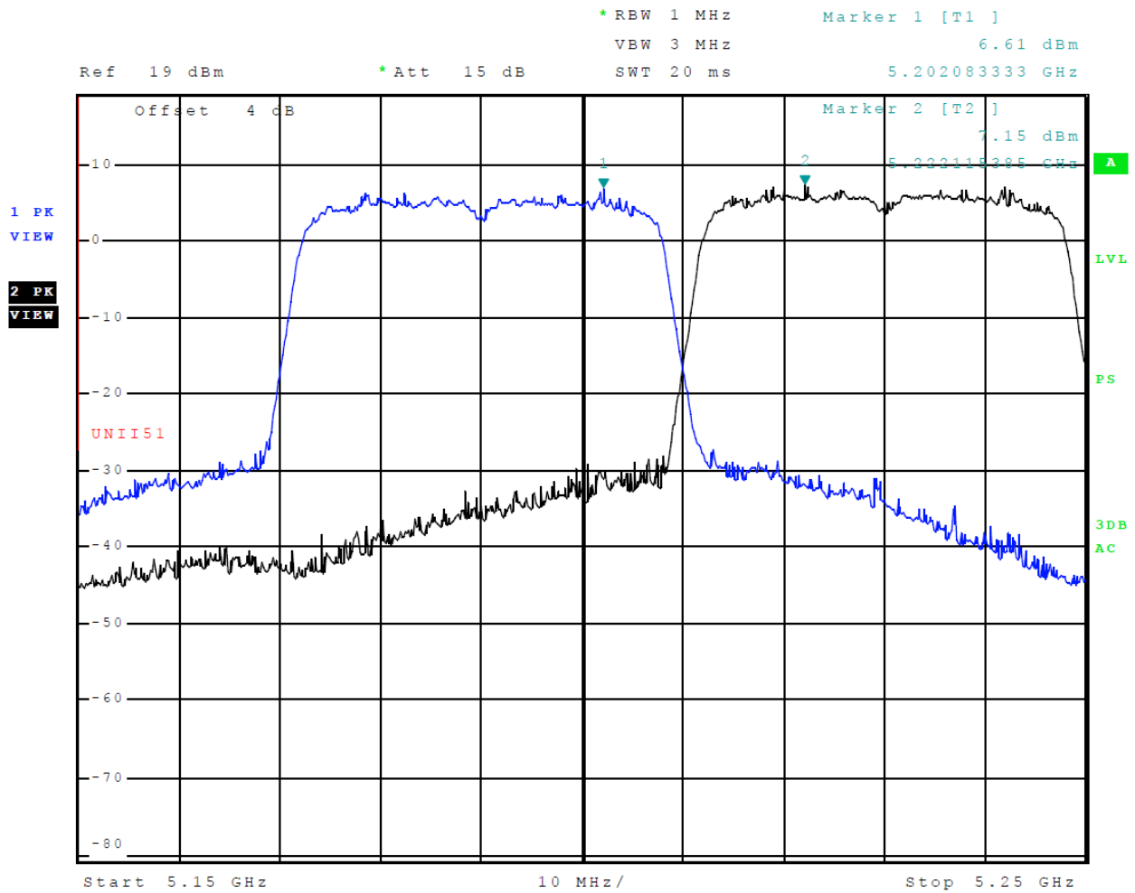
Figure 8 Plot of Transmitter Emissions (Across 5150-5250 MHz Band, Chain 1, 802.11n40)
