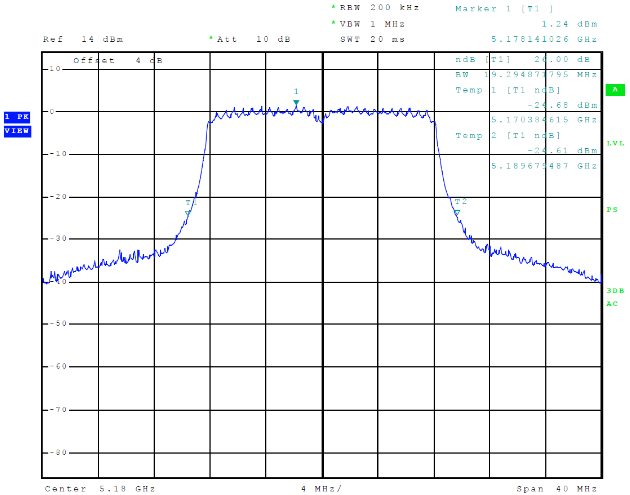
Figure 34 Plot of Transmitter Emissions (5150-5250 MHz Band, 802.11n, Chain 1, 26 dB OBW)
