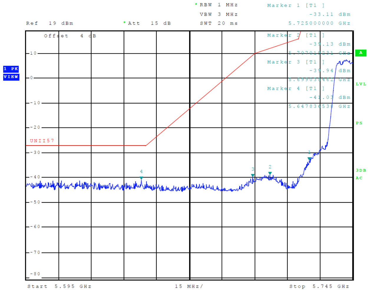
Figure 54 Plot of Transmitter Low Band Edge (5725-5850 MHz Band, Chain 1, 802.11n)
