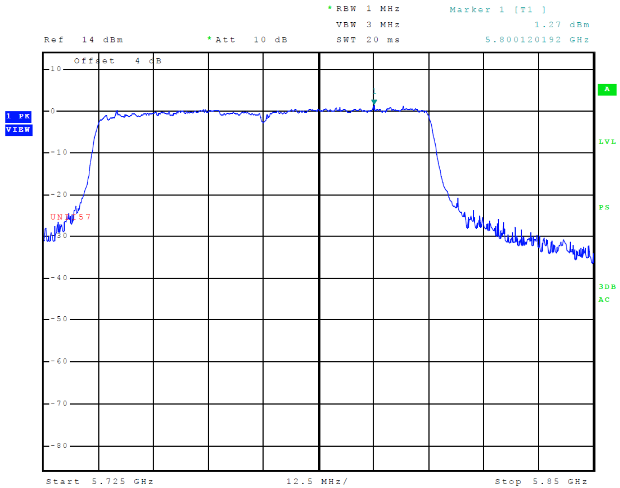
Figure 49 Plot of Transmitter Emissions (Across 5725-5850 MHz Band, Chain 0, 802.11ac)
