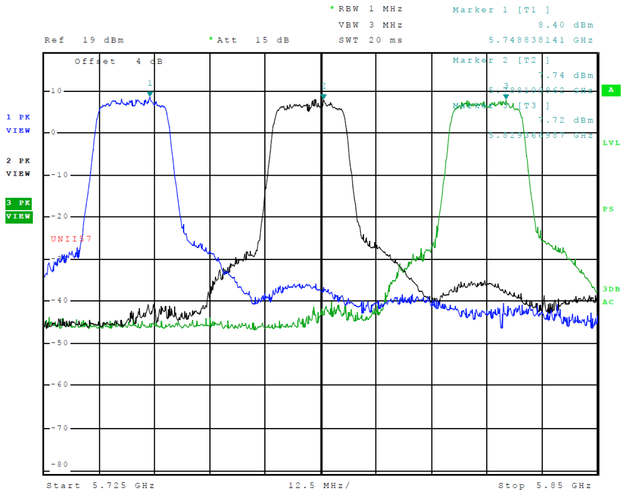
Figure 45 Plot of Transmitter Emissions (Across 5725-5850 MHz Band, Chain 0, 802.11n)
