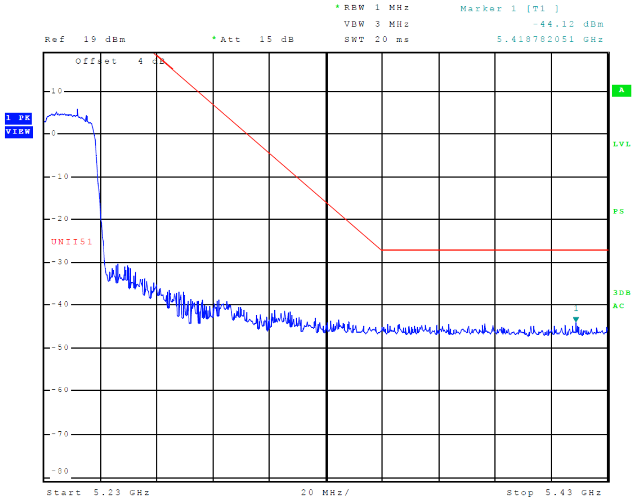
Figure 23 Plot of Transmitter High Band Edge (5150-5250 MHz Band, Chain 0, 802.11n40)
