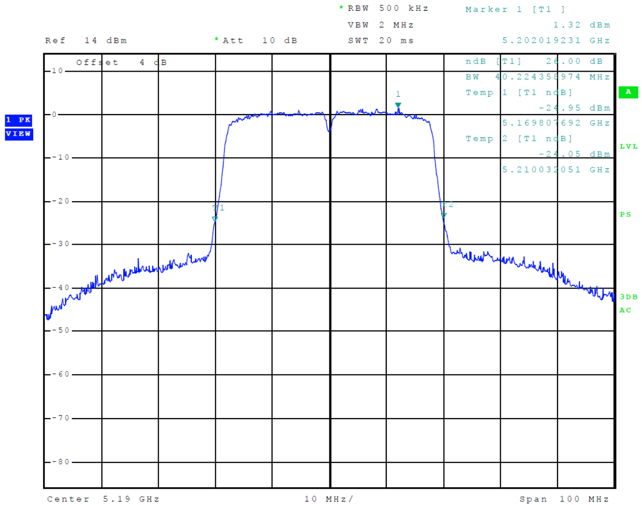
Figure 37 Plot of Transmitter Emissions (5150-5250 MHz Band, 802.11n40, Chain 0, 26 dB OBW)
