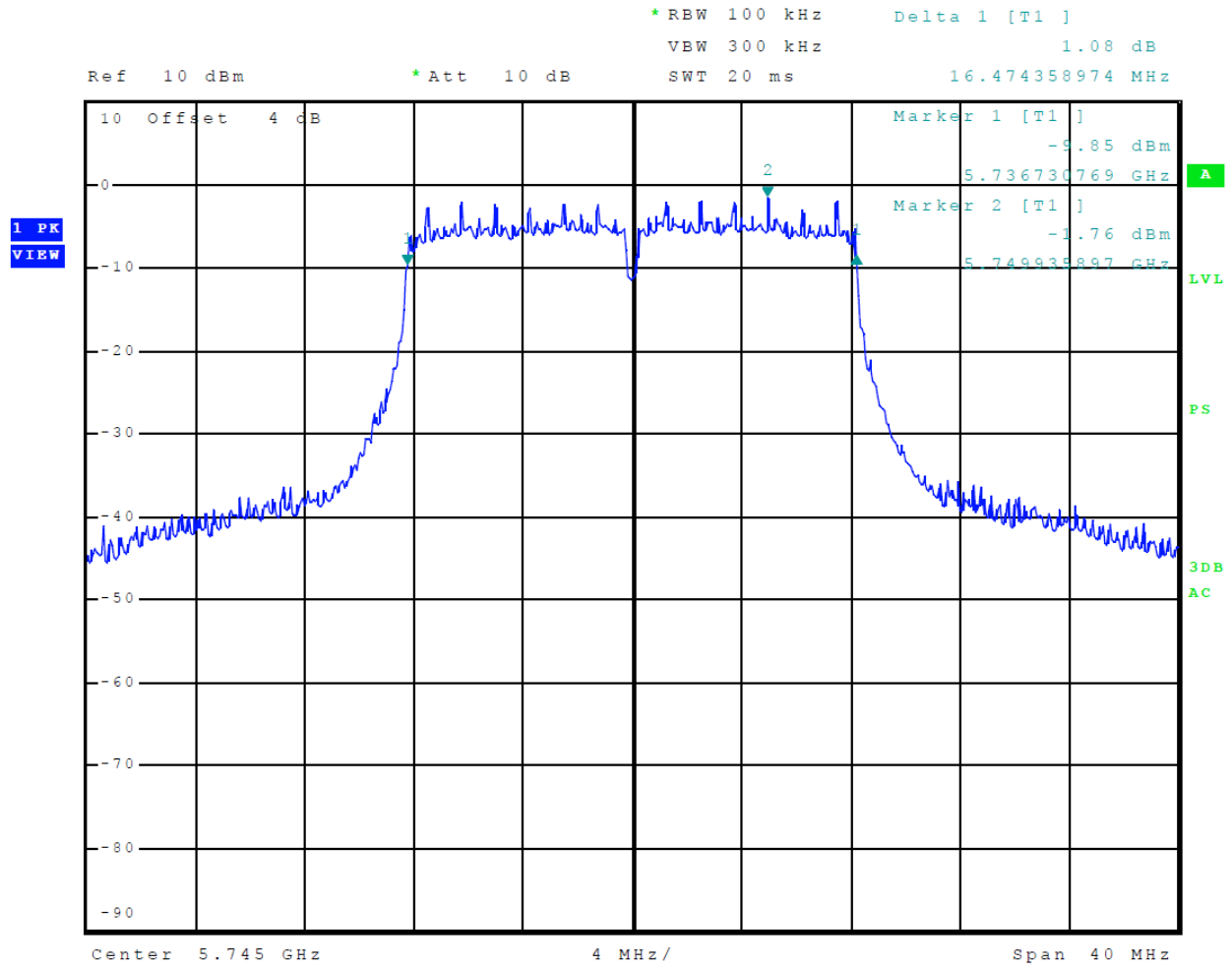
Figure 73 Plot of Transmitter Emissions (5725-5850 MHz Band, 802.11n, Chain 0, 6-dB OBW)
