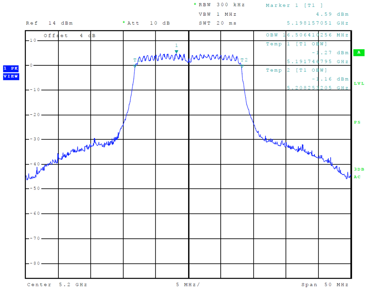
Figure 28 Plot of Transmitter Emissions (5150-5250 MHz Band, 802.11a, Chain 1, 99% OBW)
