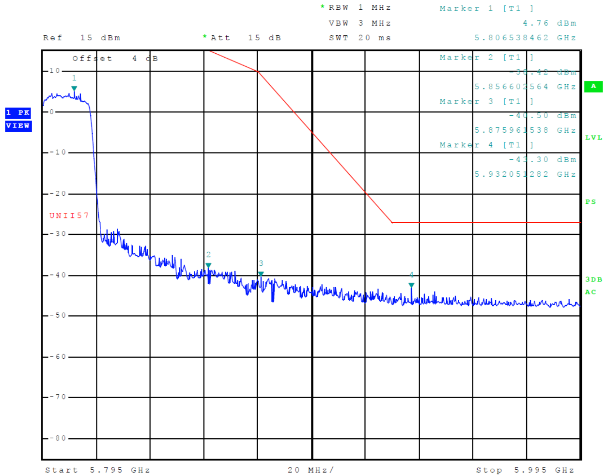
Figure 63 Plot of Transmitter High Band Edge (5725-5850 MHz Band, Chain 0, 802.11n40)
