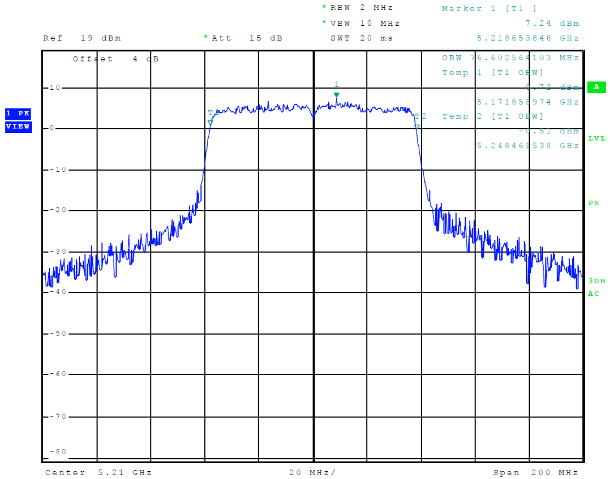
Figure 40 Plot of Transmitter Emissions (5150-5250 MHz Band, 802.11ac, Chain 1, 99% OBW)
