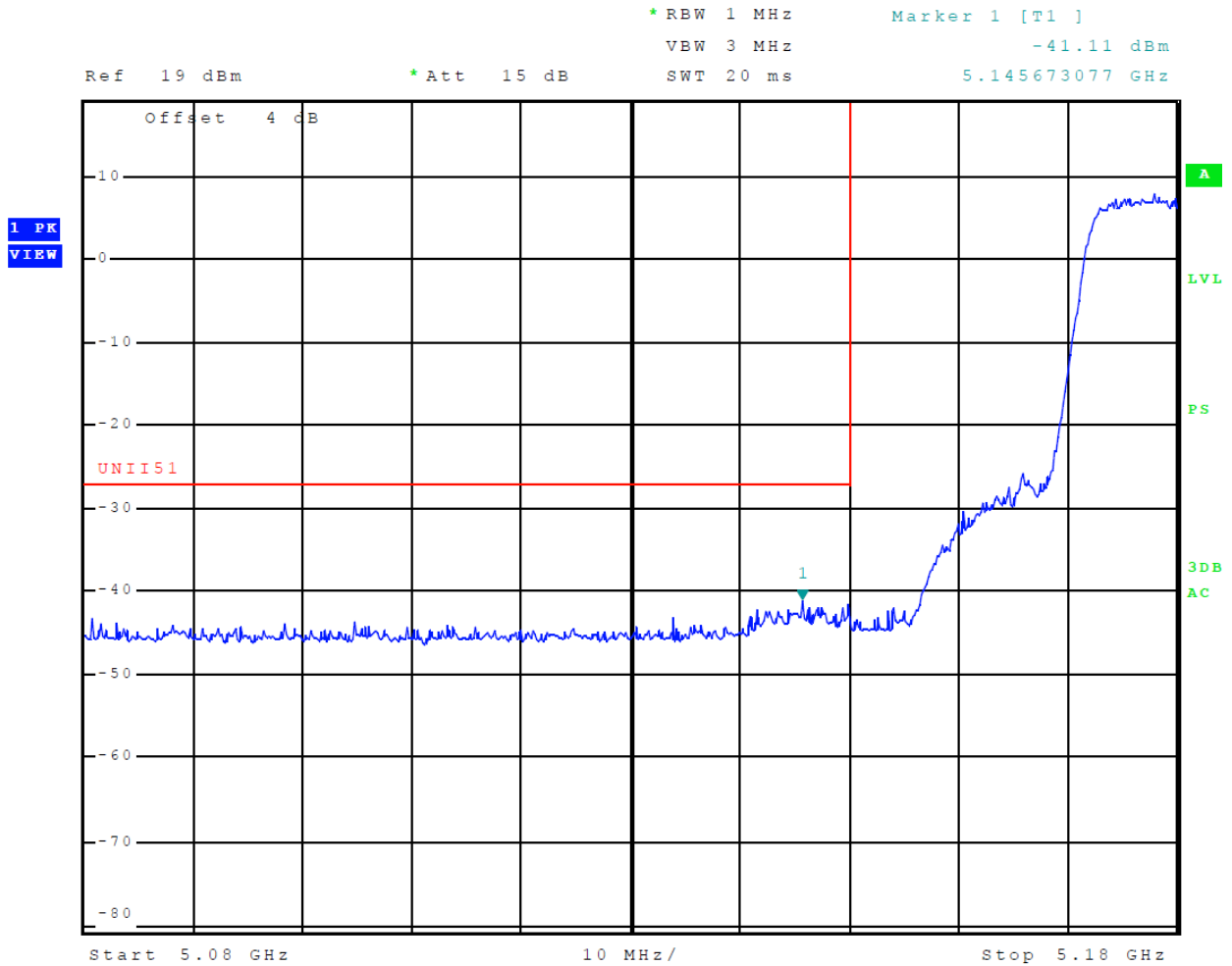
Figure 13 Plot of Transmitter Low Band Edge (5150-5250 MHz Band, Chain 0, 802.11n)
