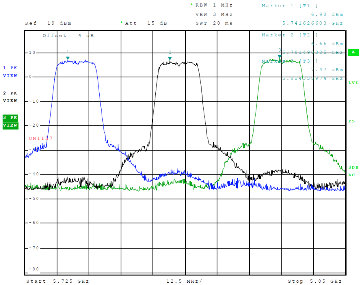
Figure 44 Plot of Transmitter Emissions (Across 5725-5850 MHz Band, Chain 1, 802.11a)
