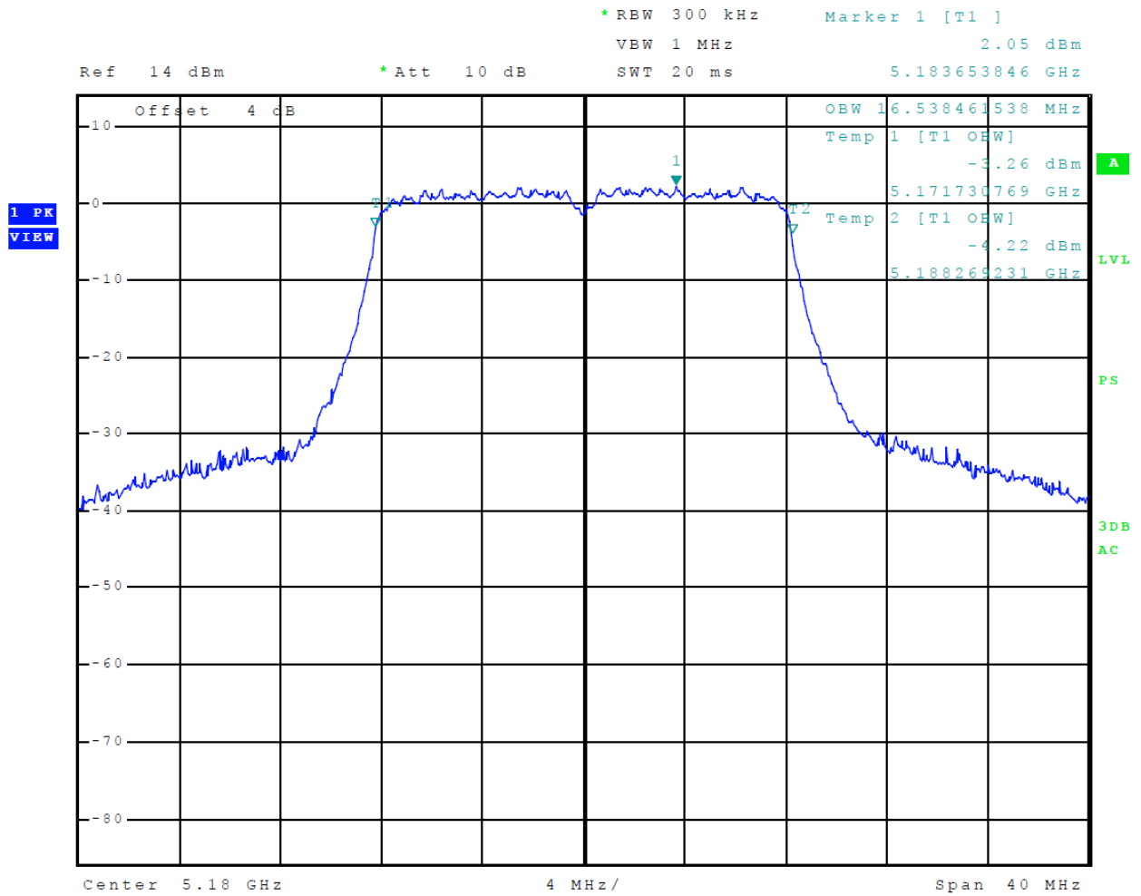
Figure 27 Plot of Transmitter Emissions (5150-5250 MHz Band, 802.11a, Chain 0, 99% OBW)
