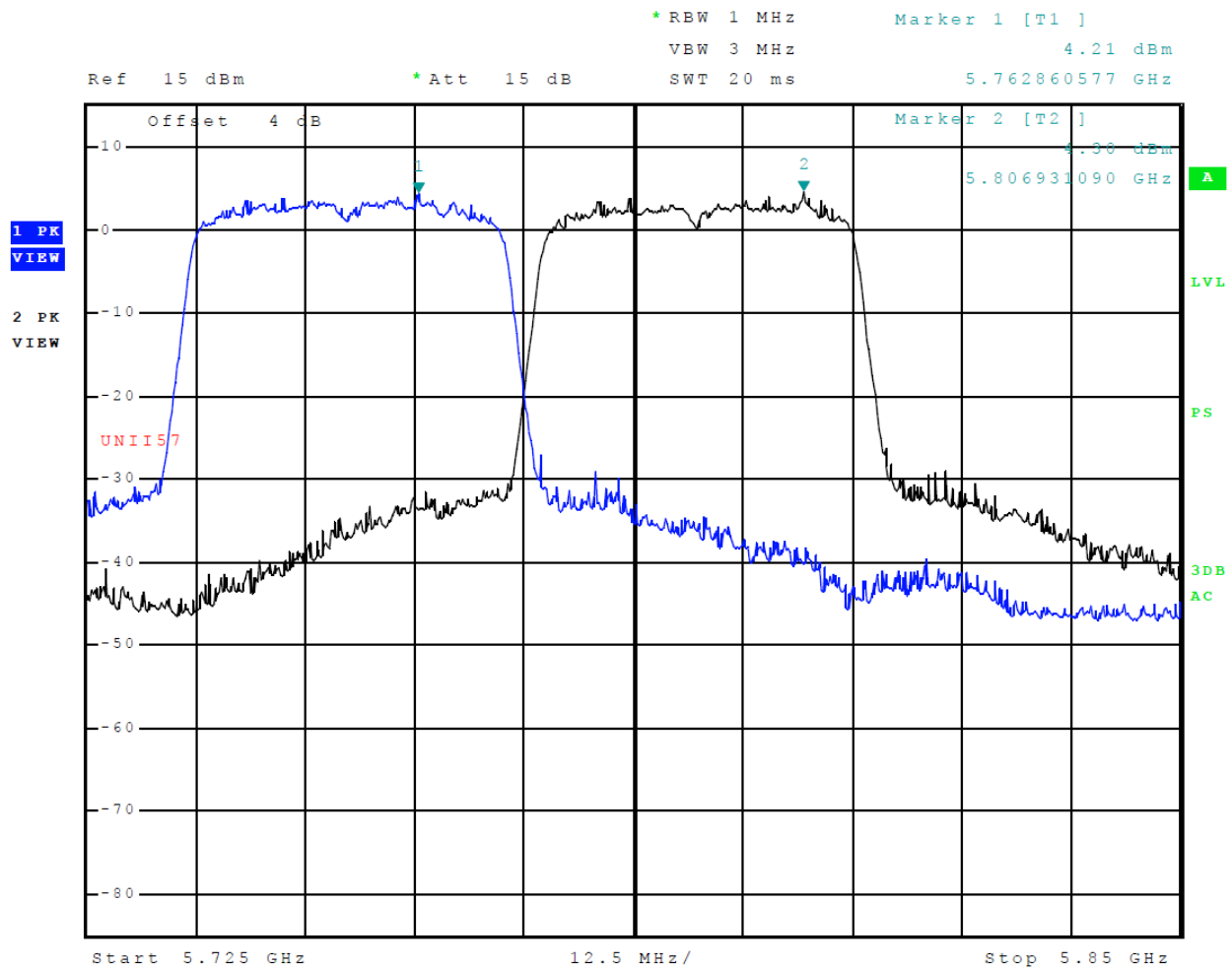
Figure 48 Plot of Transmitter Emissions (Across 5725-5850 MHz Band, Chain 1, 802.11n40)
