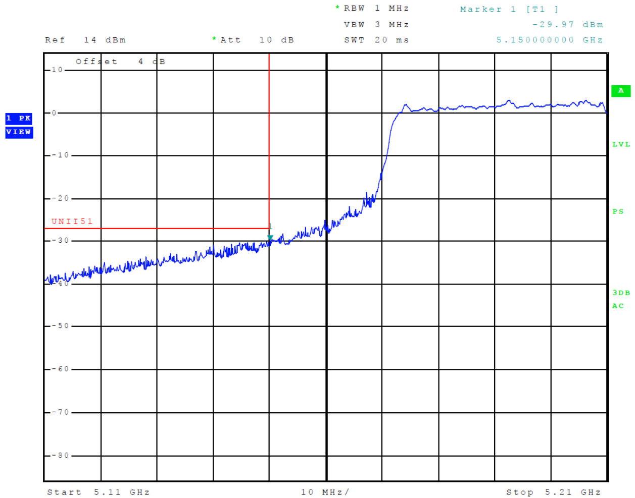
Figure 18 Plot of Transmitter Low Band Edge (5150-5250 MHz Band, Chain 1, 802.11ac)
