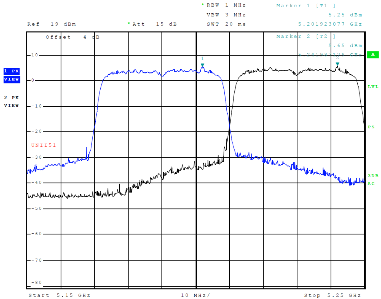
Figure 7 Plot of Transmitter Emissions (Across 5150-5250 MHz Band, Chain 0, 802.11n40)
