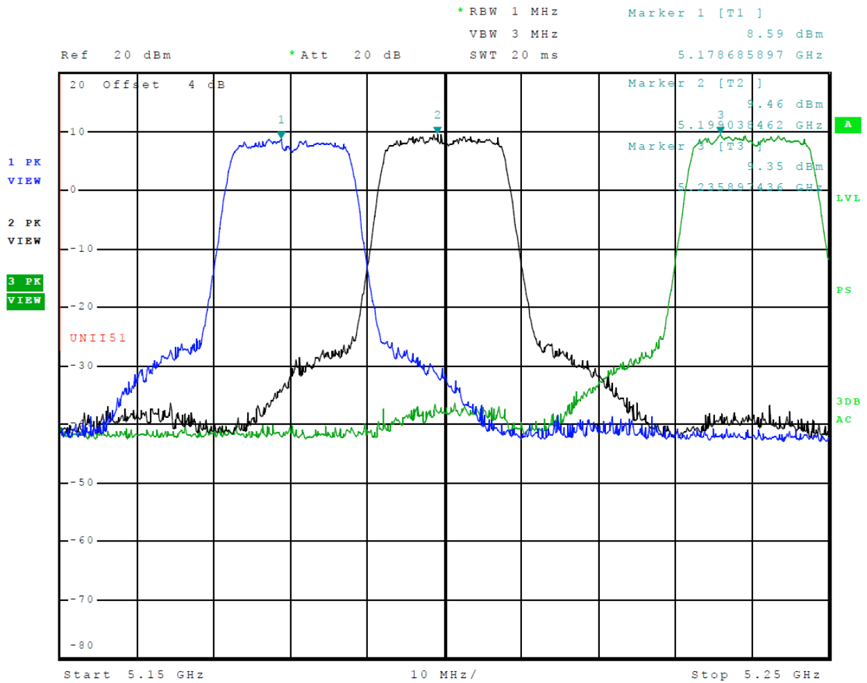
Figure 4 Plot of Transmitter Emissions (Across 5150-5250 MHz Band, Chain 1, 802.11a)
