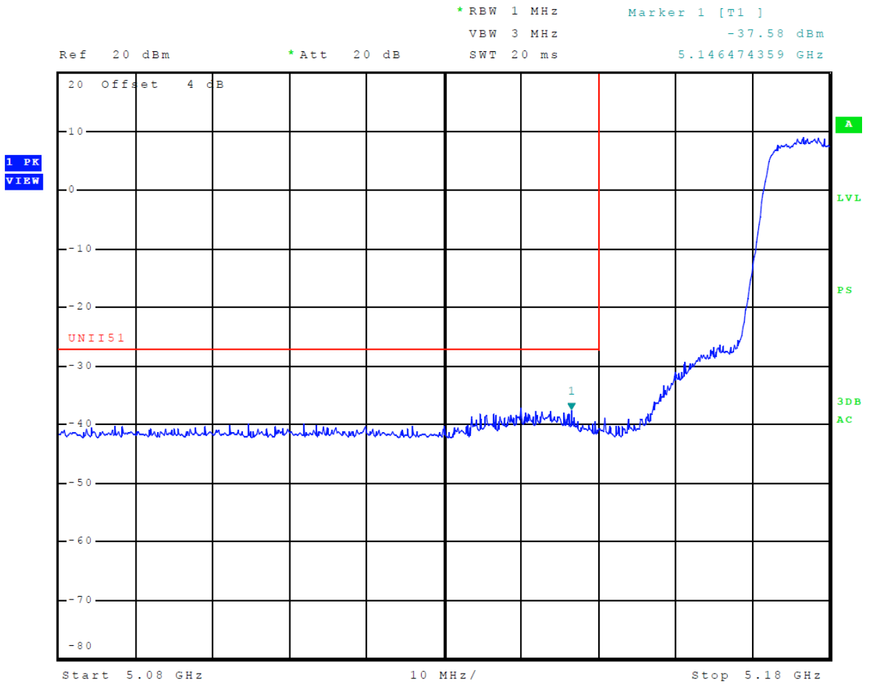
Figure 14 Plot of Transmitter Low Band Edge (5150-5250 MHz Band, Chain 1, 802.11n)
