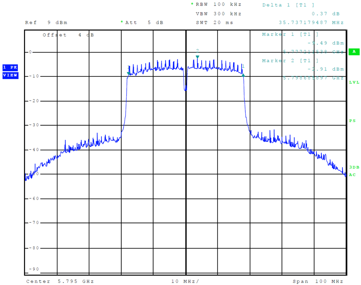
Figure 77 Plot of Transmitter Emissions (5725-5850 MHz Band, 802.11n40, Chain 0, 6-dB OBW)
