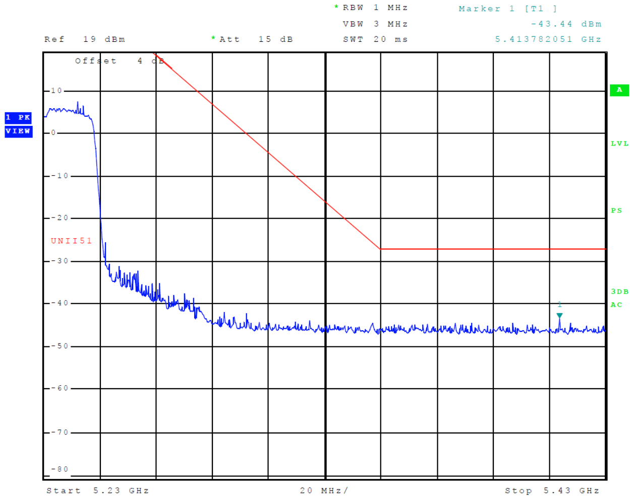
Figure 24 Plot of Transmitter High Band Edge (5150-5250 MHz Band, Chain 1, 802.11n40)
