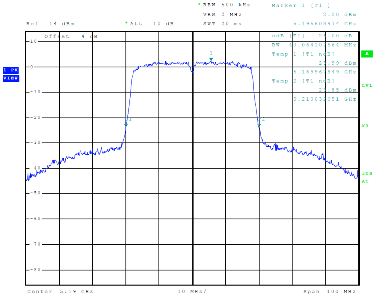
Figure 38 Plot of Transmitter Emissions (5150-5250 MHz Band, 802.11n40, Chain 1, 26 dB OBW)
