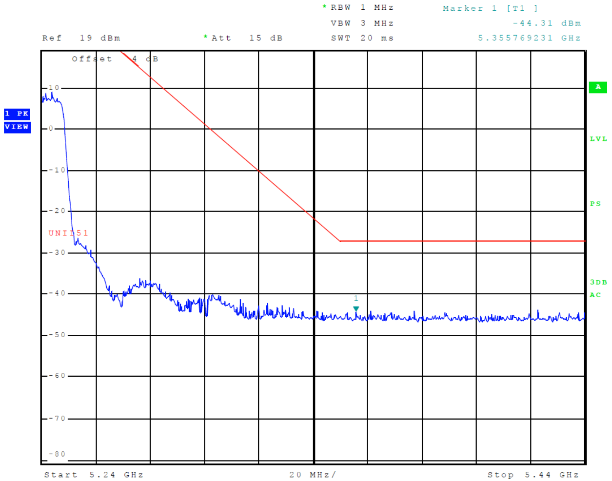
Figure 21 Plot of Transmitter High Band Edge (5150-5250 MHz Band, Chain 0, 802.11n)
