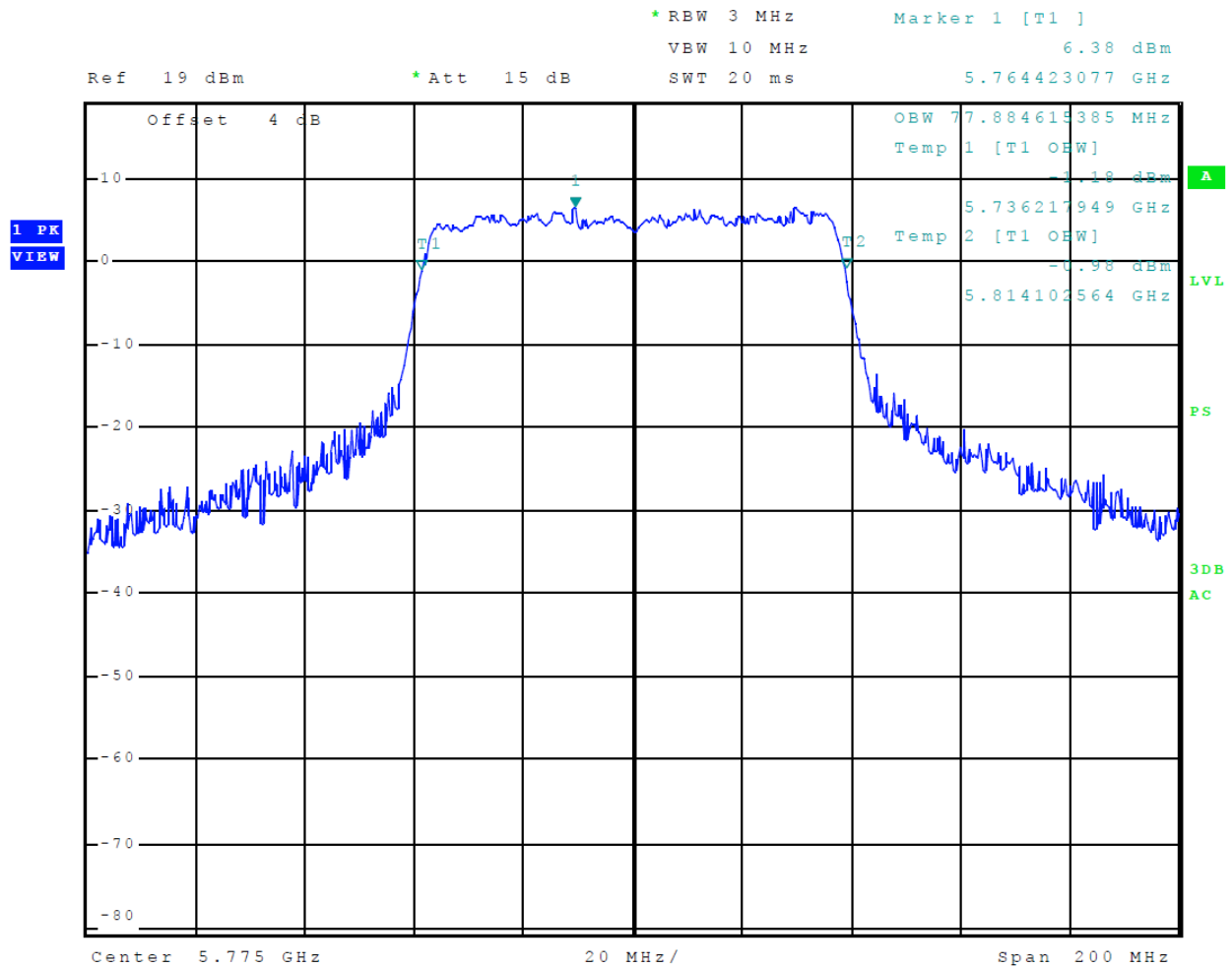
Figure 79 Plot of Transmitter Emissions (5725-5850 MHz Band, 802.11ac, Chain 0, 99% OBW)
