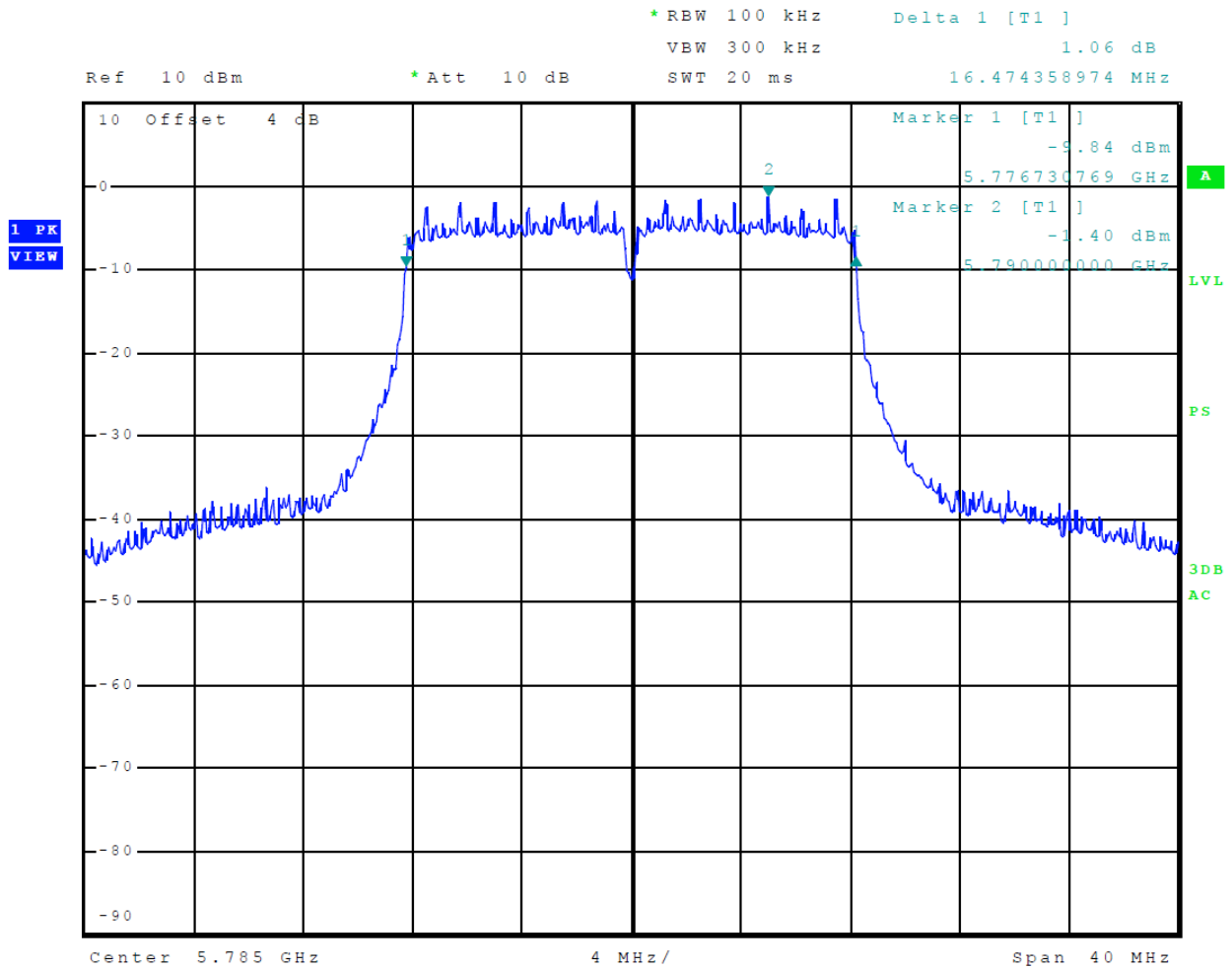
Figure 70 Plot of Transmitter Emissions (5725-5850 MHz Band, 802.11a, Chain 1, 6-dB OBW)
