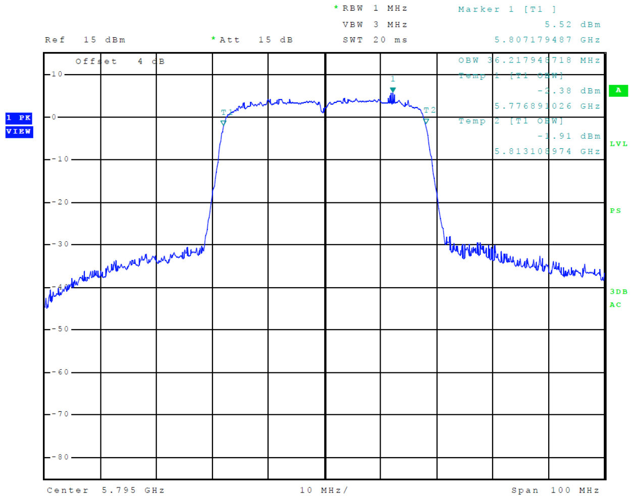
Figure 75 Plot of Transmitter Emissions (5725-5850 MHz Band, 802.11n40, Chain 0, 99% OBW)
