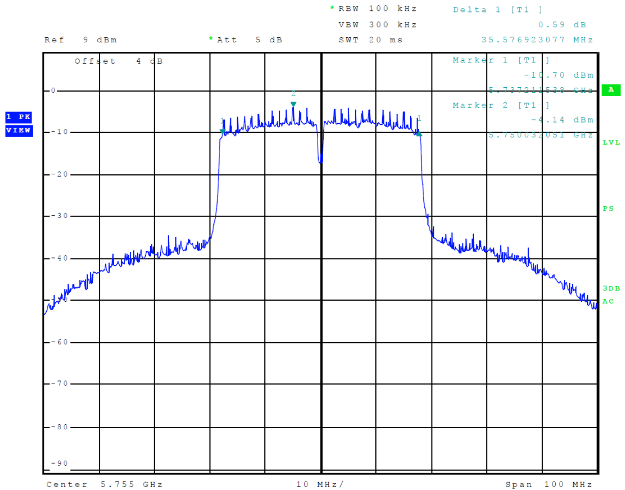
Figure 78 Plot of Transmitter Emissions (5725-5850 MHz Band, 802.11n40, Chain 1, 6-dB OBW)
