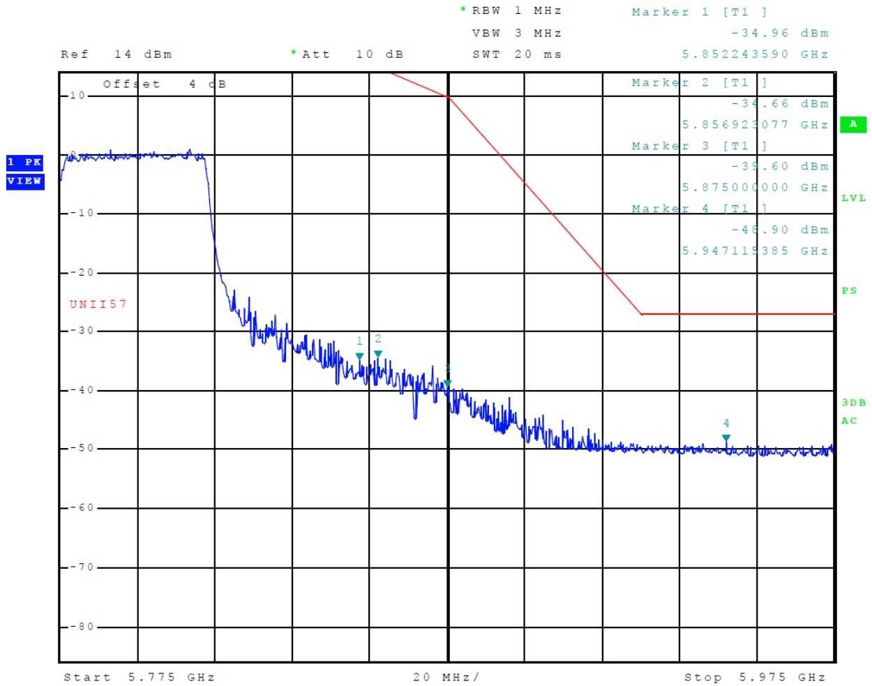
Figure 66 Plot of Transmitter High Band Edge (5725-5850 MHz Band, Chain 1, 802.11ac)
