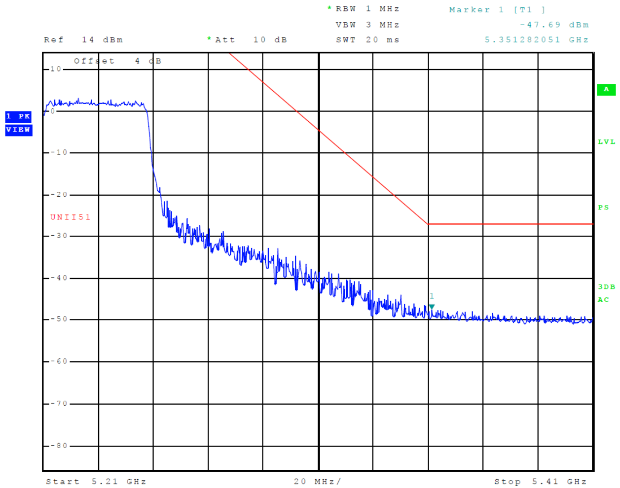
Figure 26 Plot of Transmitter High Band Edge (5150-5250 MHz Band, Chain 1, 802.11ac)
