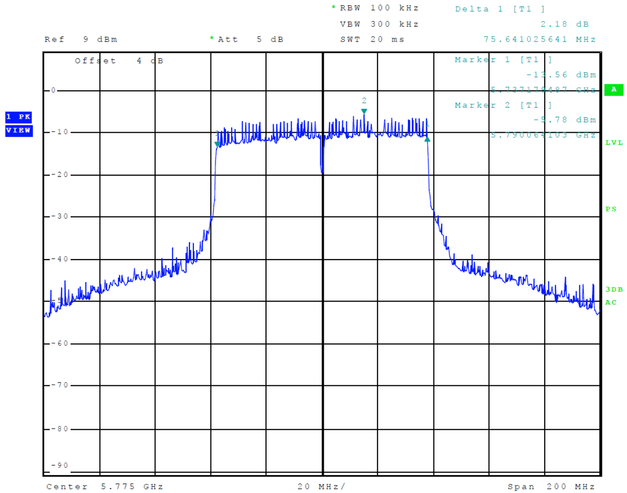
Figure 81 Plot of Transmitter Emissions (5725-5850 MHz Band, 802.11ac, Chain 0, 6-dB OBW)
