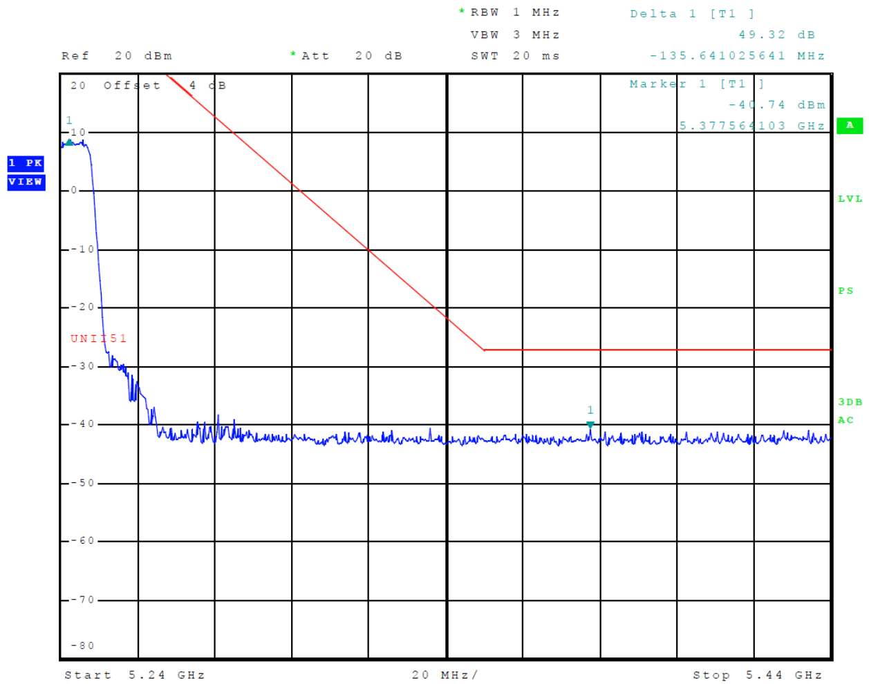
Figure 20 Plot of Transmitter High Band Edge (5150-5250 MHz Band, Chain 1, 802.11a)
