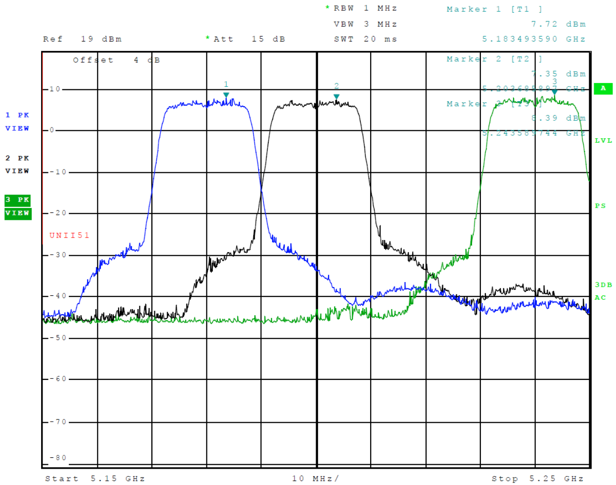
Figure 3 Plot of Transmitter Emissions (Across 5150-5250 MHz Band, Chain 0, 802.11a)
