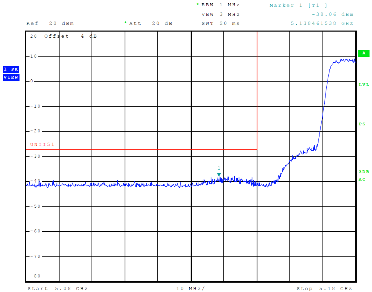
Figure 12 Plot of Transmitter Low Band Edge (5150-5250 MHz Band, Chain 1, 802.11a)
