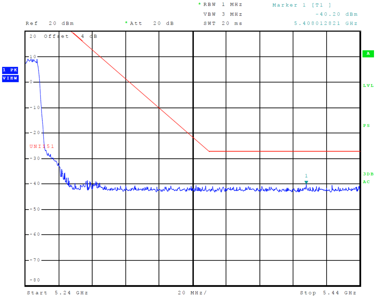
Figure 22 Plot of Transmitter High Band Edge (5150-5250 MHz Band, Chain 1, 802.11n)
