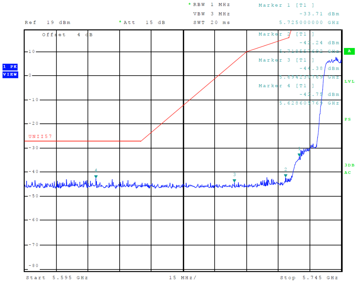
Figure 51 Plot of Transmitter Low Band Edge (5725-5850 MHz Band, Chain 0, 802.11a)
