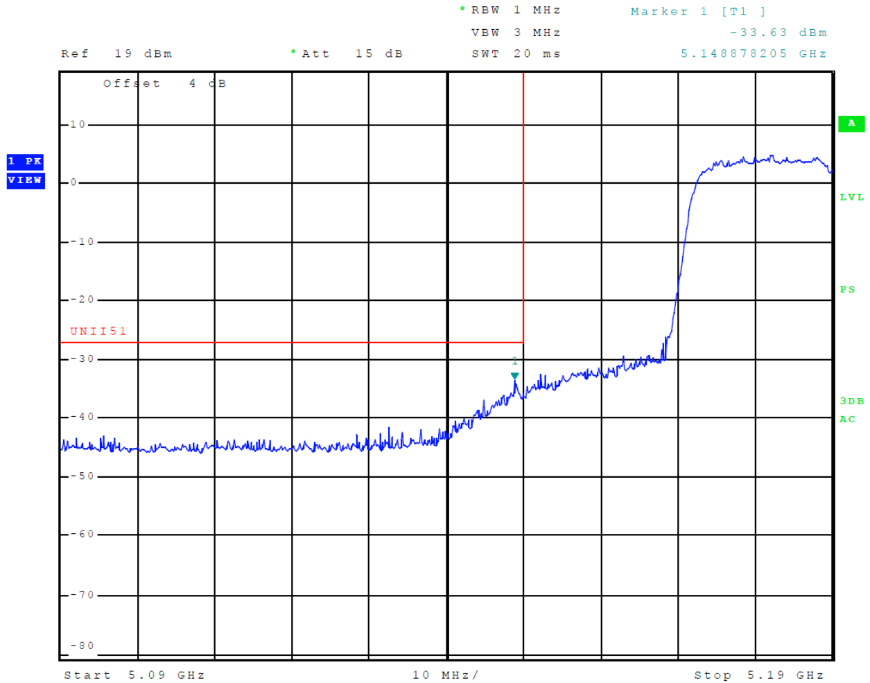
Figure 15 Plot of Transmitter Low Band Edge (5150-5250 MHz Band, Chain 0, 802.11n40)
