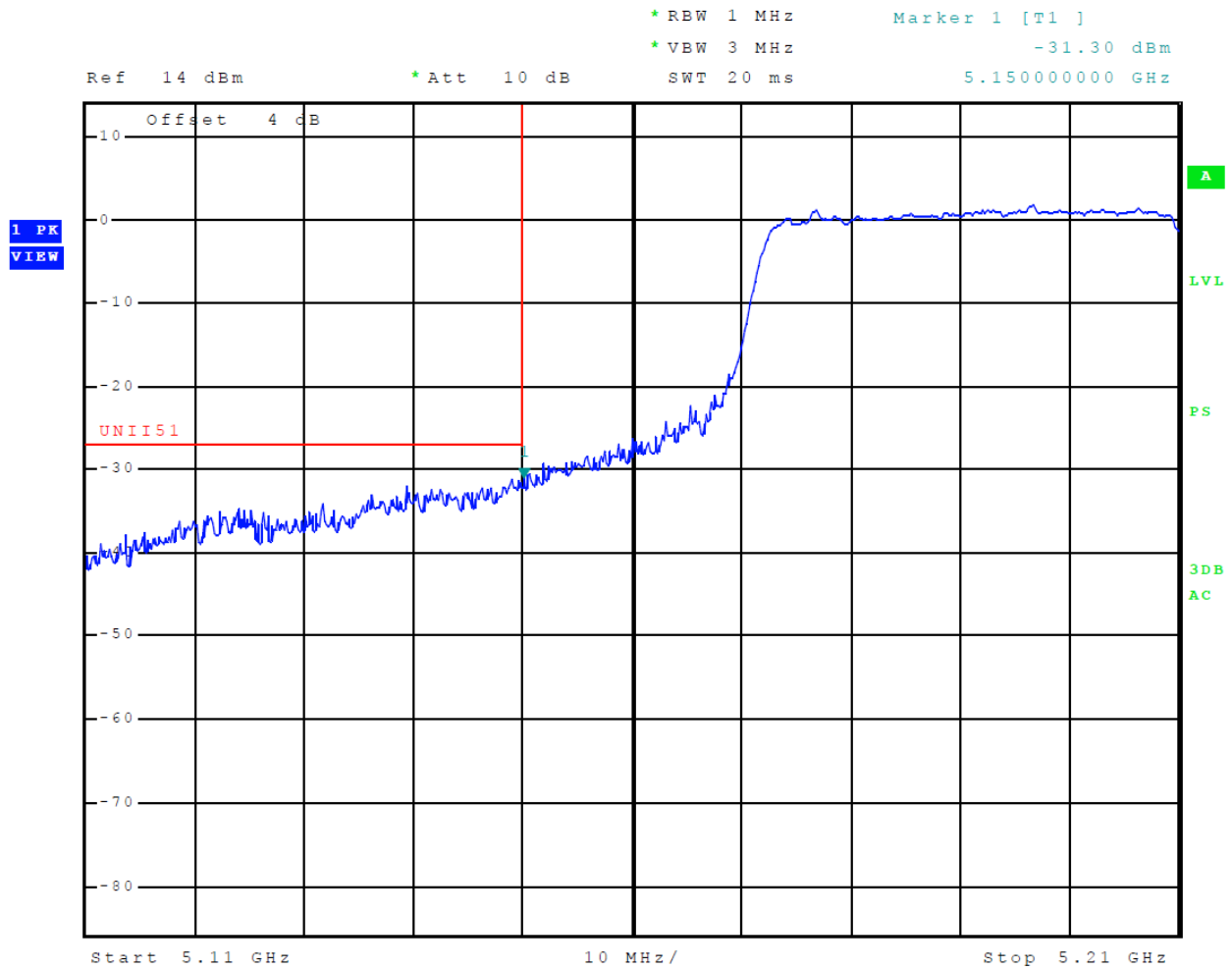
Figure 17 Plot of Transmitter Low Band Edge (5150-5250 MHz Band, Chain 0, 802.11ac)
