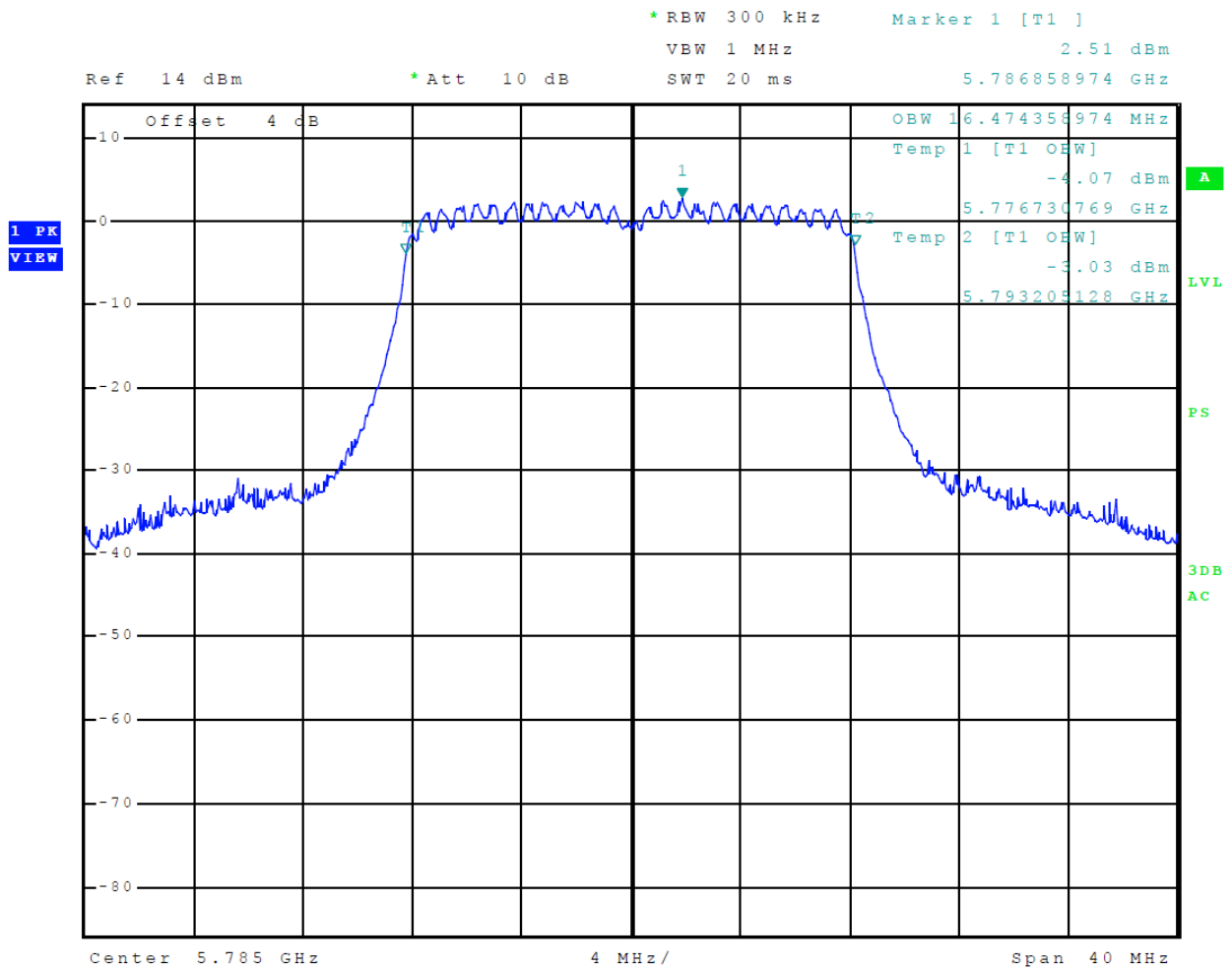
Figure 72 Plot of Transmitter Emissions (5725-5850 MHz Band, 802.11n, Chain 1, 99% OBW)
