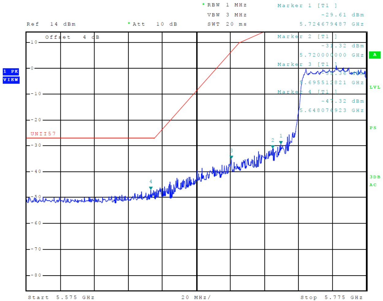
Figure 58 Plot of Transmitter Low Band Edge (5725-5850 MHz Band, Chain 1, 802.11ac)
