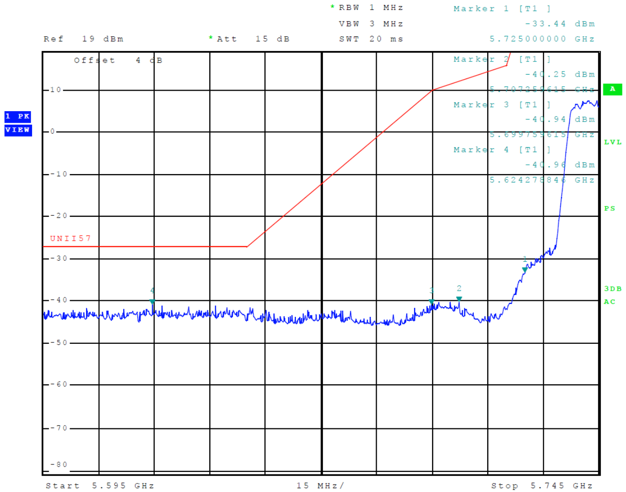
Figure 52 Plot of Transmitter Low Band Edge (5725-5850 MHz Band, Chain 1, 802.11a)
