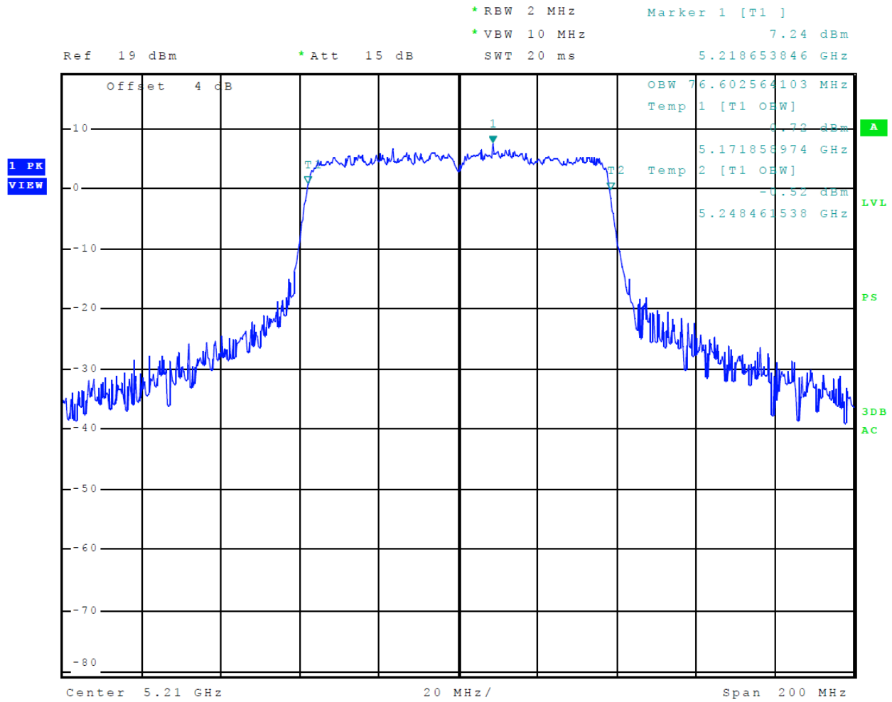
Figure 42 Plot of Transmitter Emissions (5150-5250 MHz Band, 802.11ac, Chain 1, 26 dB OBW)
