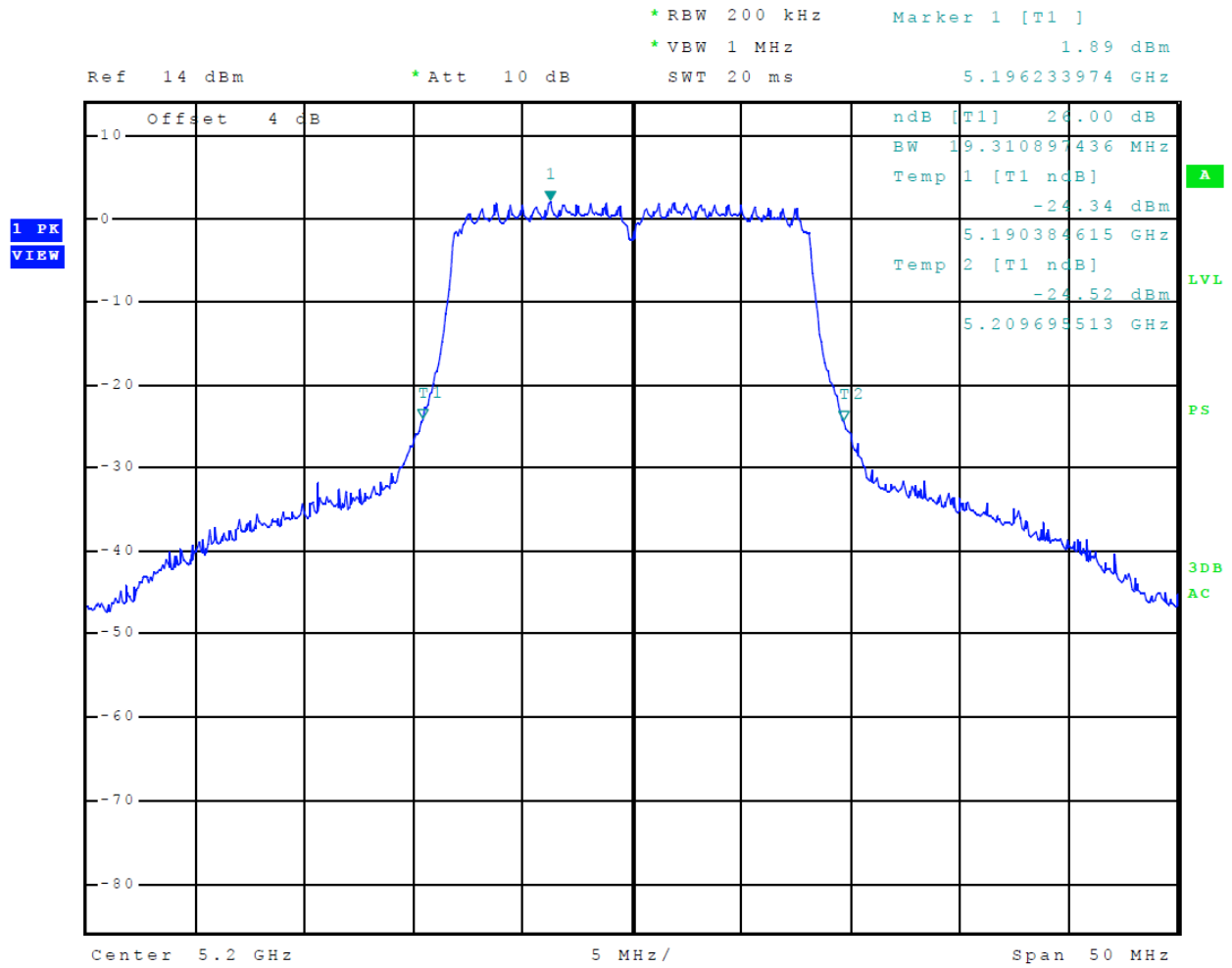
Figure 30 Plot of Transmitter Emissions (5150-5250 MHz Band, 802.11a, Chain 1, 26 dB OBW)
