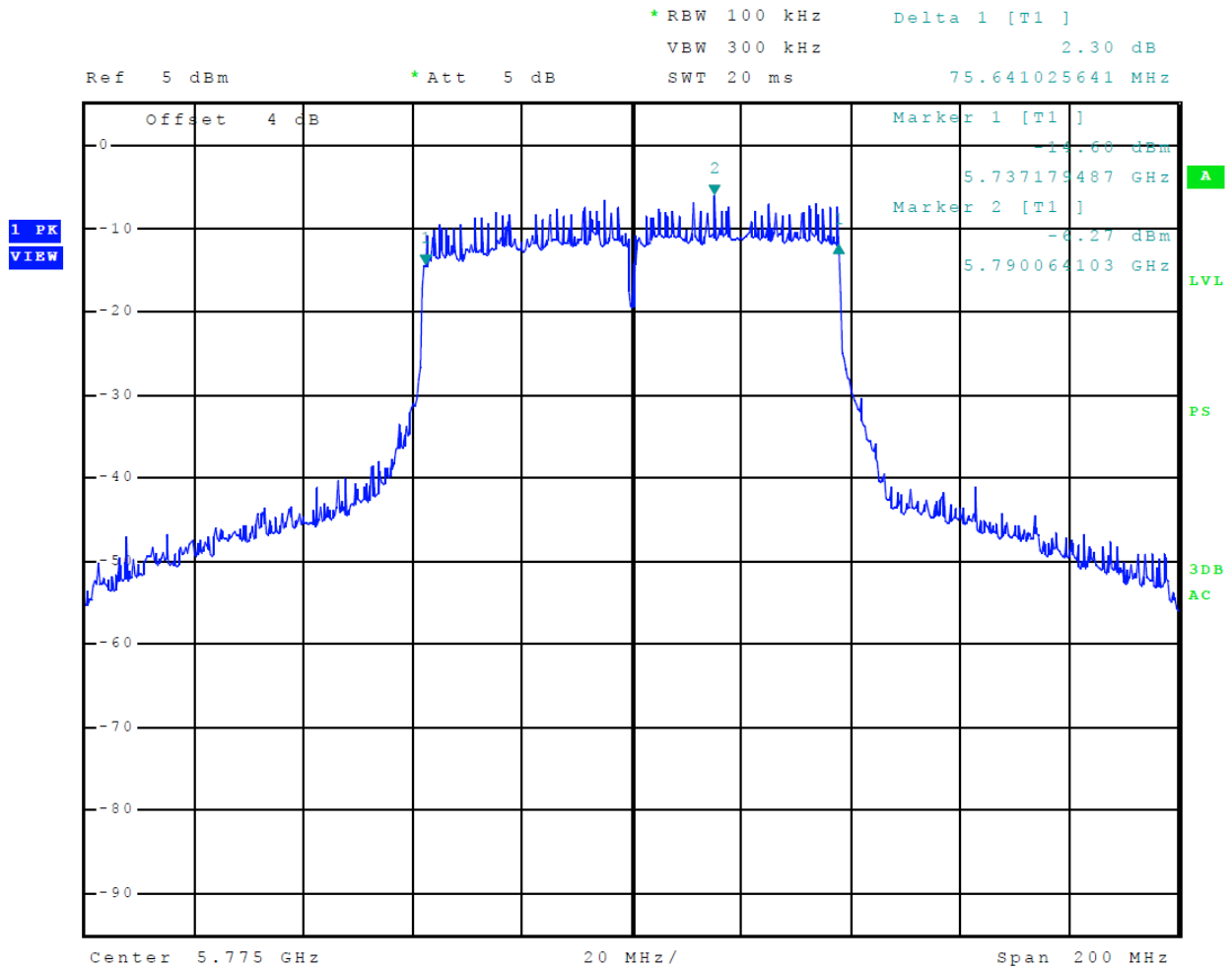
Figure 82 Plot of Transmitter Emissions (5725-5850 MHz Band, 802.11ac, Chain 1, 6-dB OBW)
