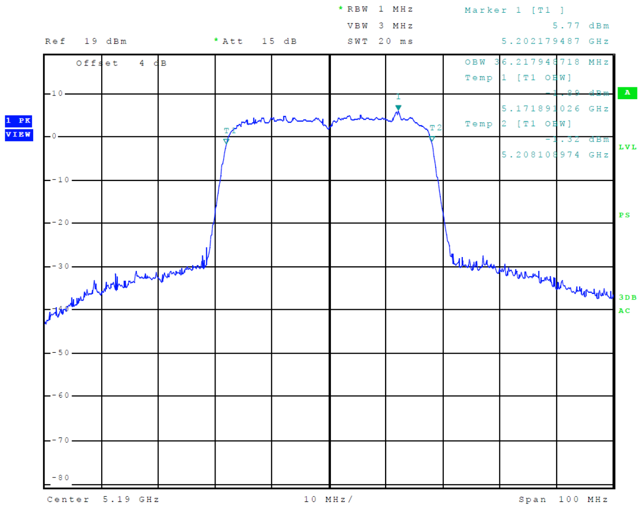
Figure 35 Plot of Transmitter Emissions (5150-5250 MHz Band, 802.11n40, Chain 0, 99% OBW)
