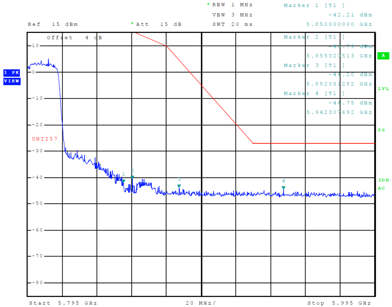
Figure 64 Plot of Transmitter High Band Edge (5725-5850 MHz Band, Chain 1, 802.11n40)
