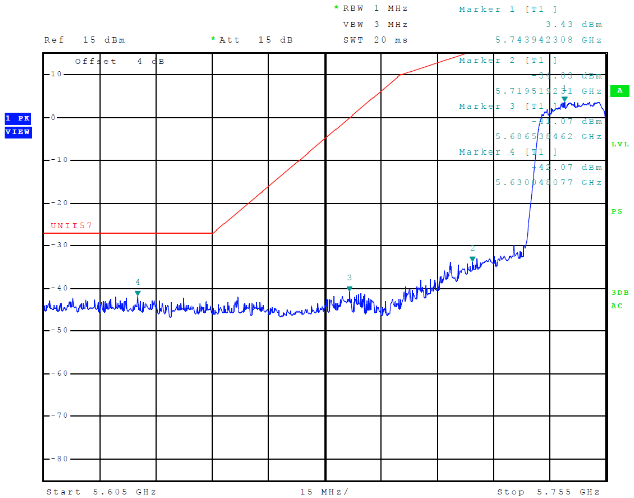
Figure 56 Plot of Transmitter Low Band Edge (5725-5850 MHz Band, Chain 1, 802.11n40)
