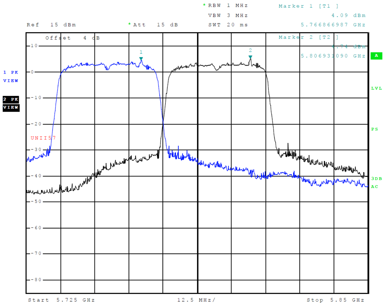
Figure 47 Plot of Transmitter Emissions (Across 5725-5850 MHz Band, Chain 0, 802.11n40)
