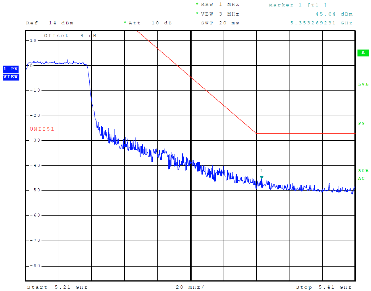
Figure 25 Plot of Transmitter High Band Edge (5150-5250 MHz Band, Chain 0, 802.11ac)
