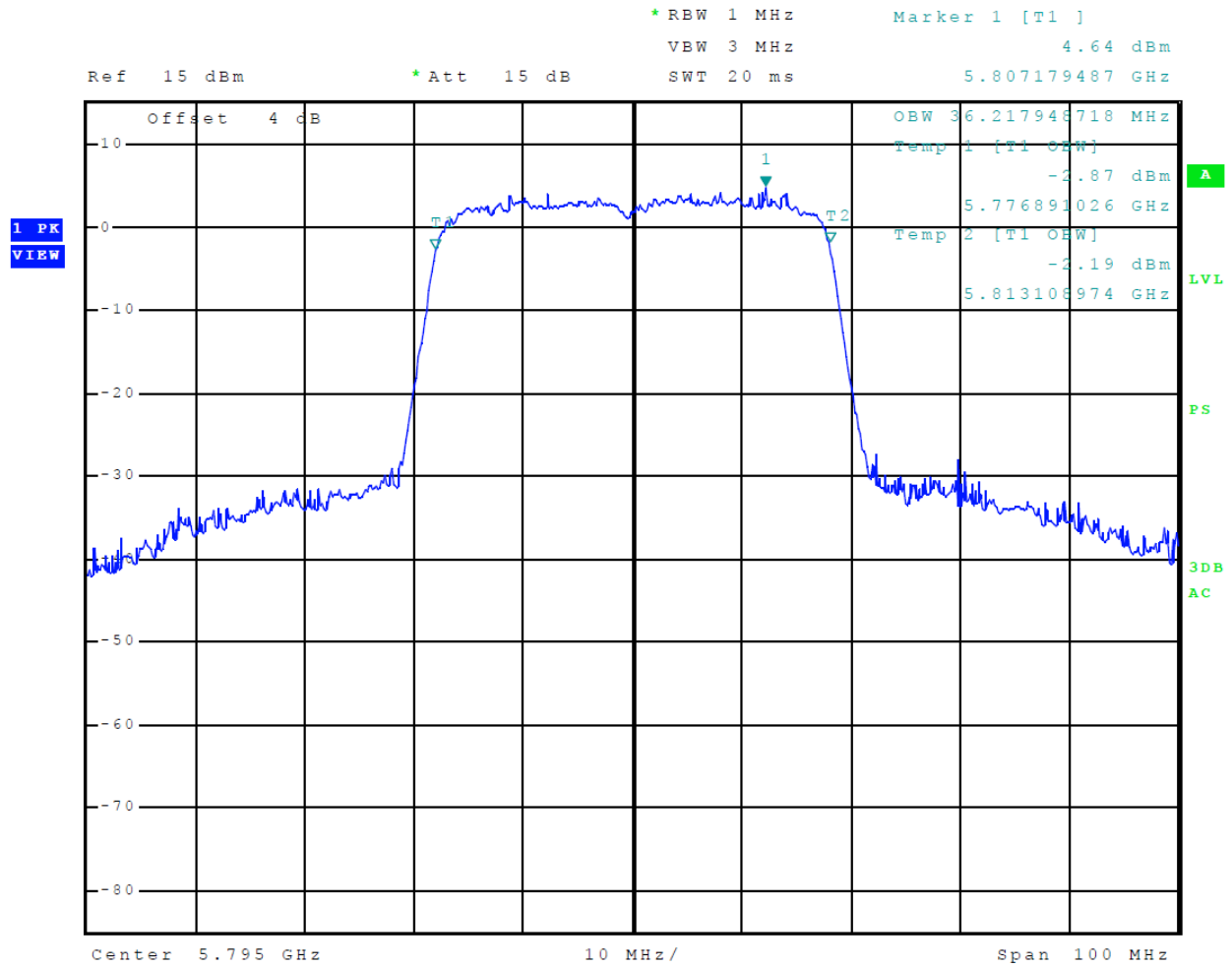
Figure 76 Plot of Transmitter Emissions (5725-5850 MHz Band, 802.11n40, Chain 1, 99% OBW)
