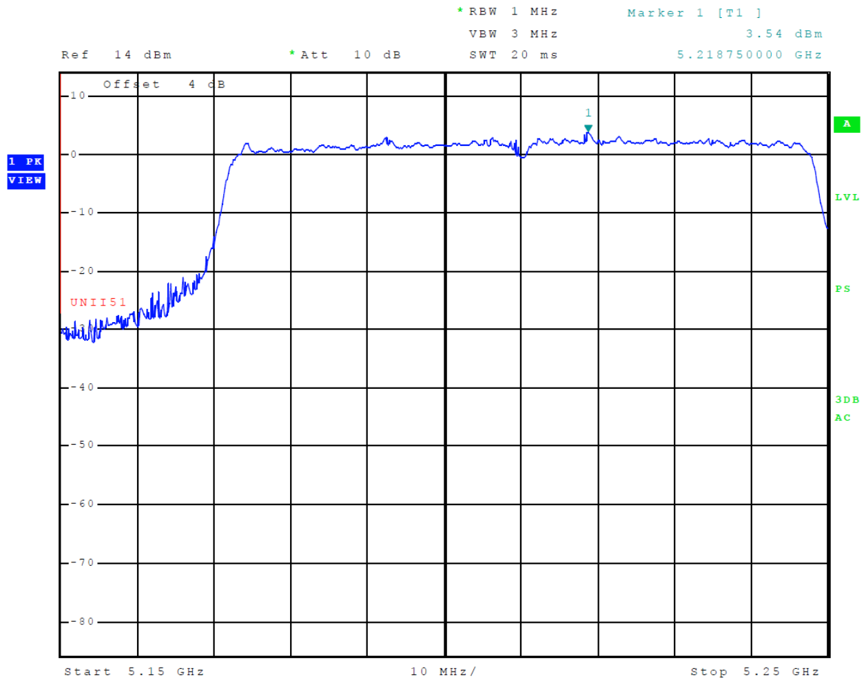
Figure 410 Plot of Transmitter Emissions (Across 5150-5250 MHz Band, Chain 1, 802.11ac)
