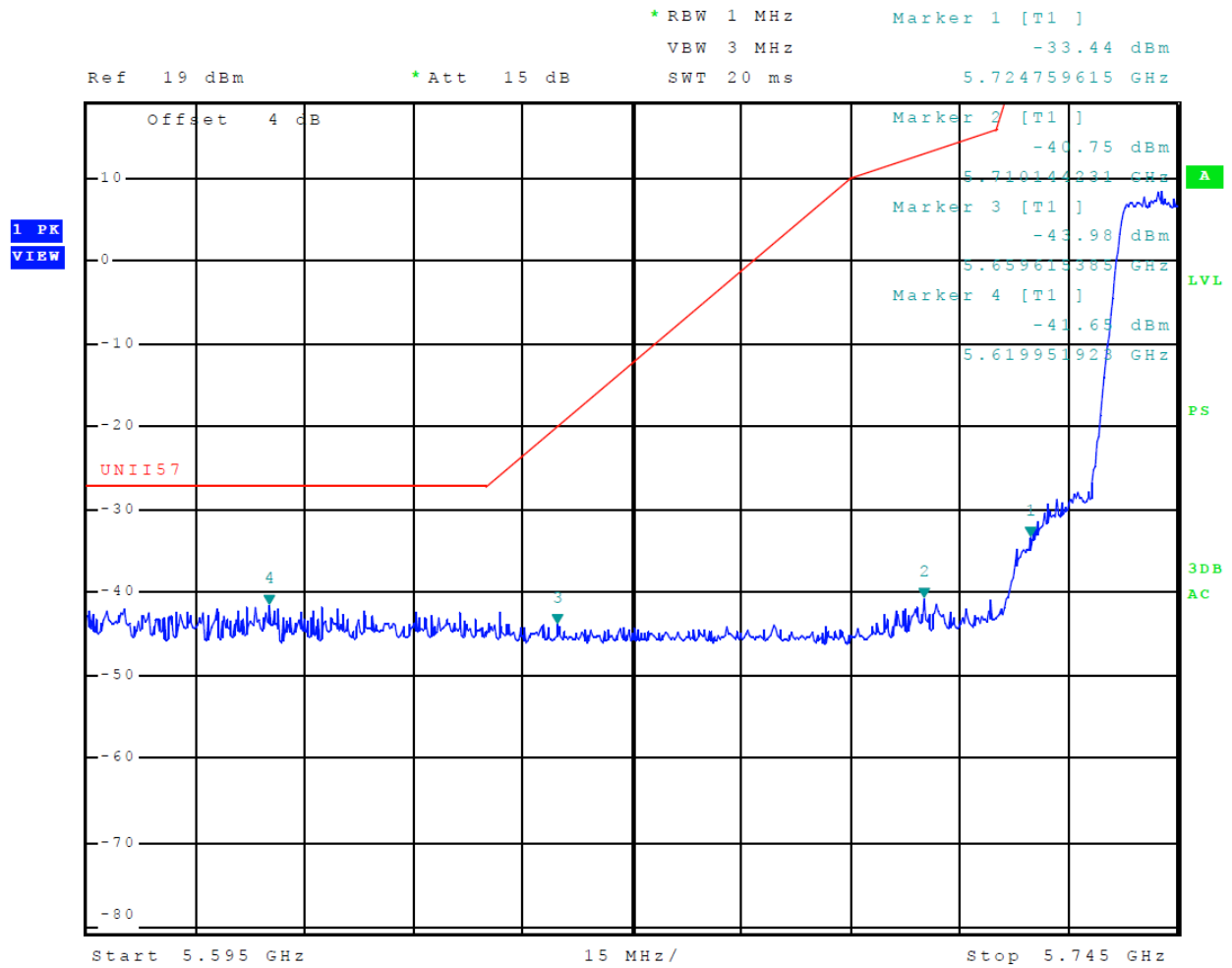
Figure 53 Plot of Transmitter Low Band Edge (5725-5850 MHz Band, Chain 0, 802.11n)
