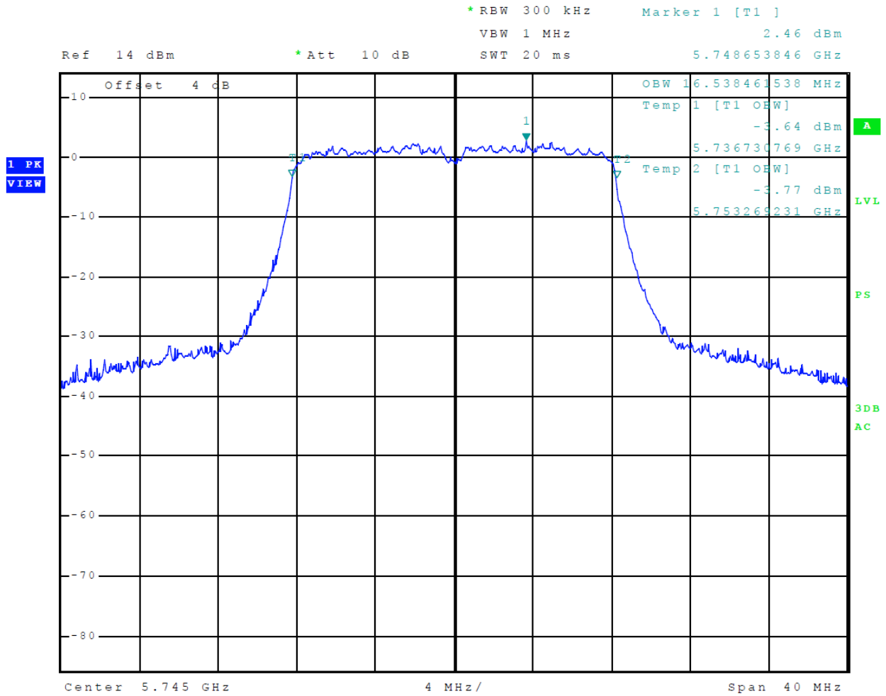
Figure 68 Plot of Transmitter Emissions (5725-5850 MHz Band, 802.11a, Chain 1, 99% OBW)
