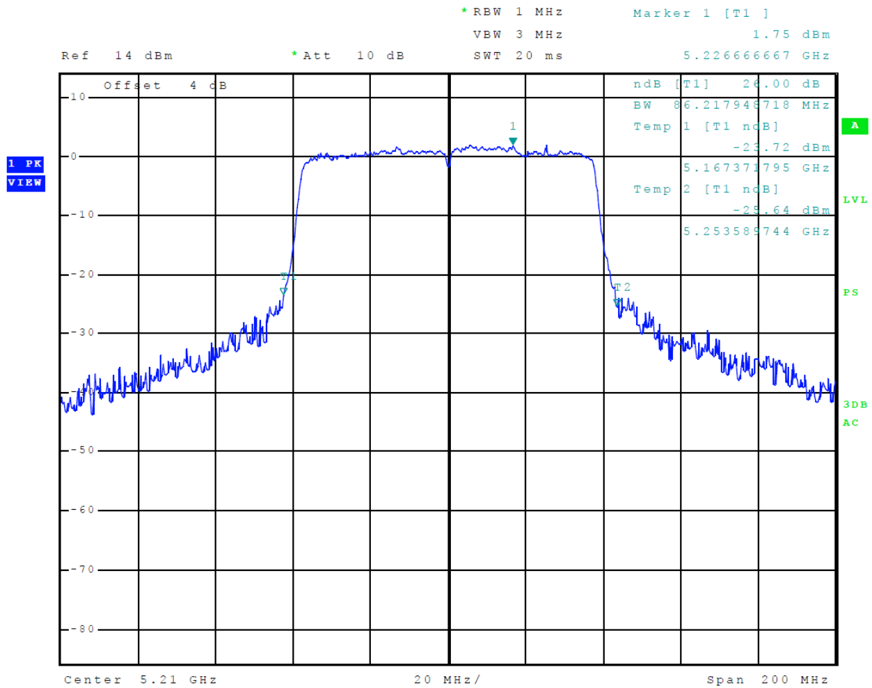
Figure 41 Plot of Transmitter Emissions (5150-5250 MHz Band, 802.11ac, Chain 0, 26 dB OBW)
