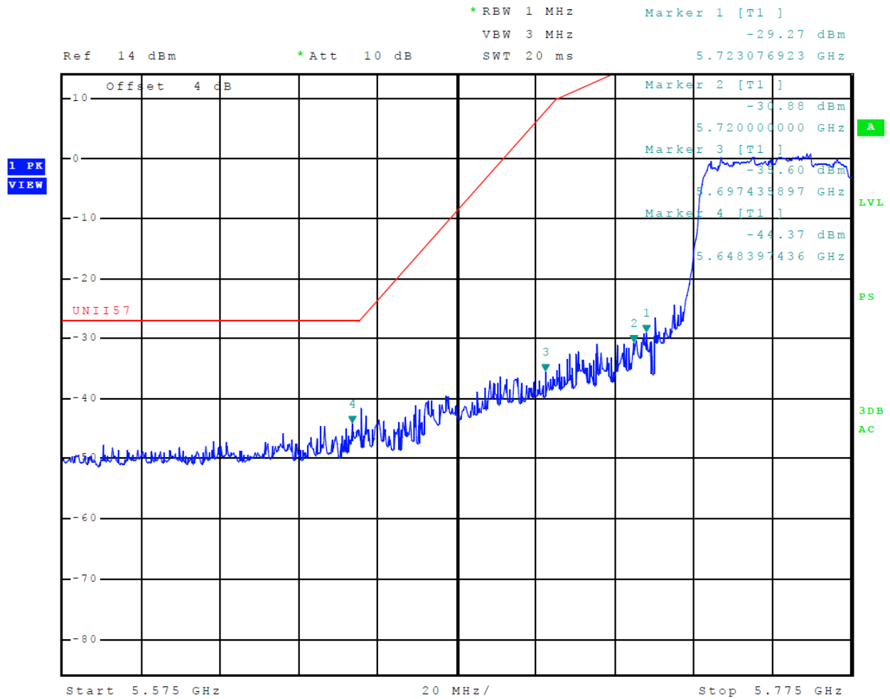
Figure 57 Plot of Transmitter Low Band Edge (5725-5850 MHz Band, Chain 0, 802.11ac)
