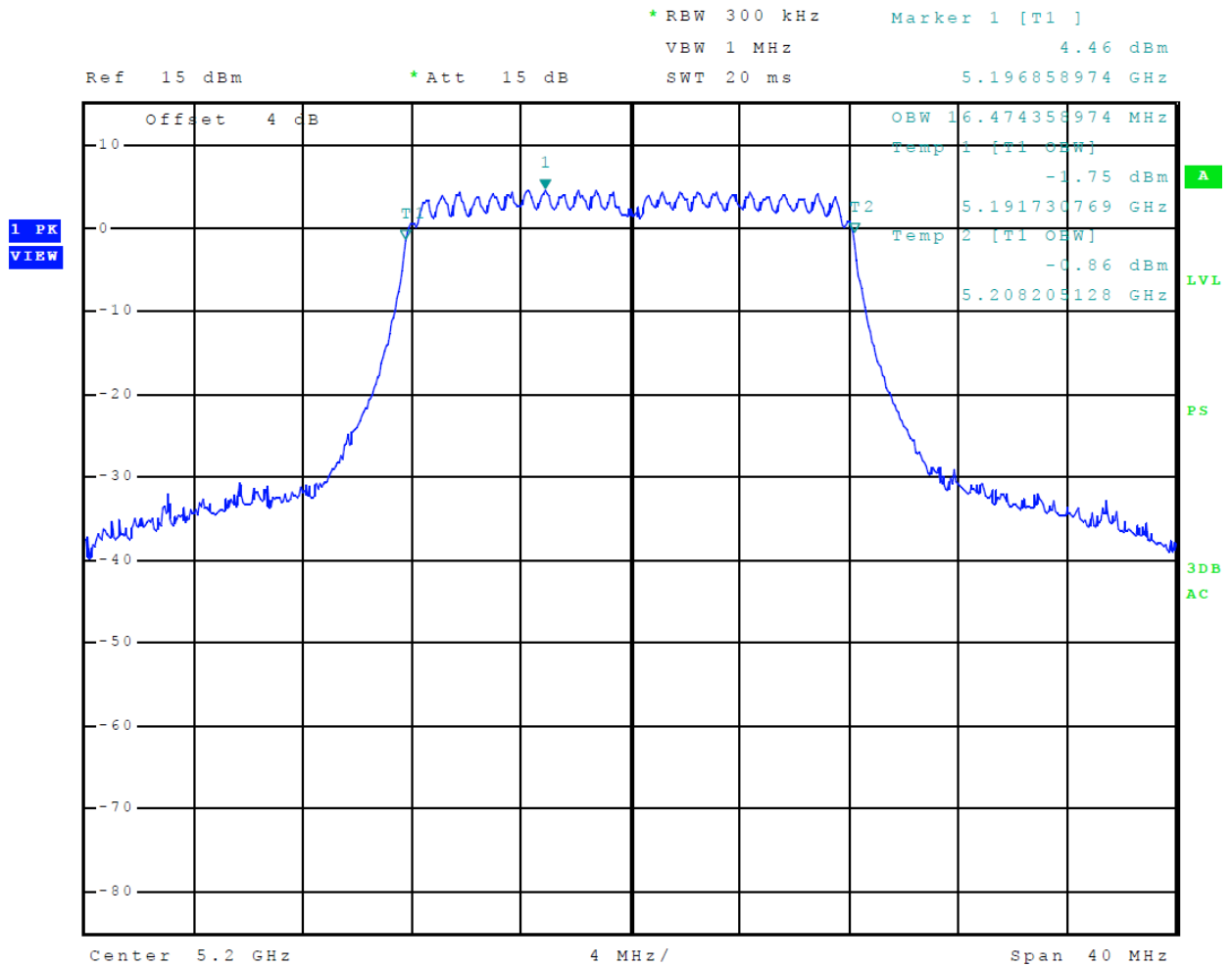
Figure 32 Plot of Transmitter Emissions (5150-5250 MHz Band, 802.11n, Chain 1, 99% OBW)
