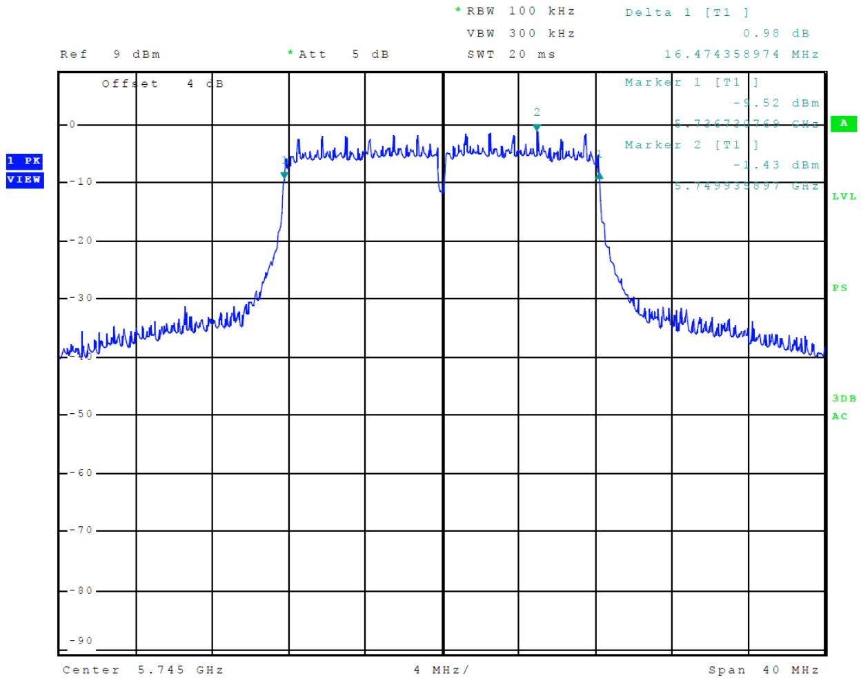
Figure 69 Plot of Transmitter Emissions (5725-5850 MHz Band, 802.11a, Chain 0, 6-dB OBW)
