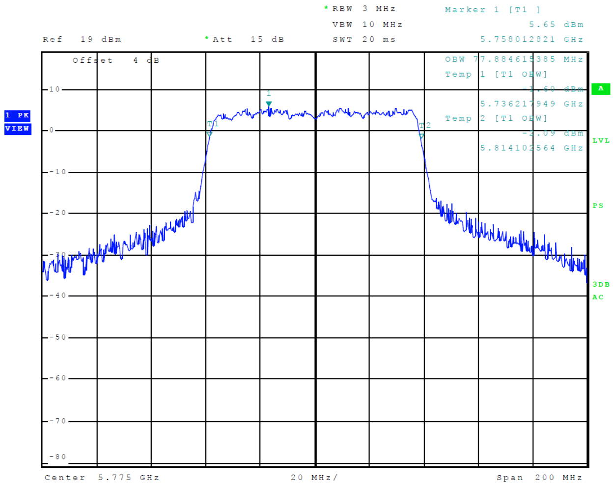
Figure 80 Plot of Transmitter Emissions (5725-5850 MHz Band, 802.11ac, Chain 1, 99% OBW)
