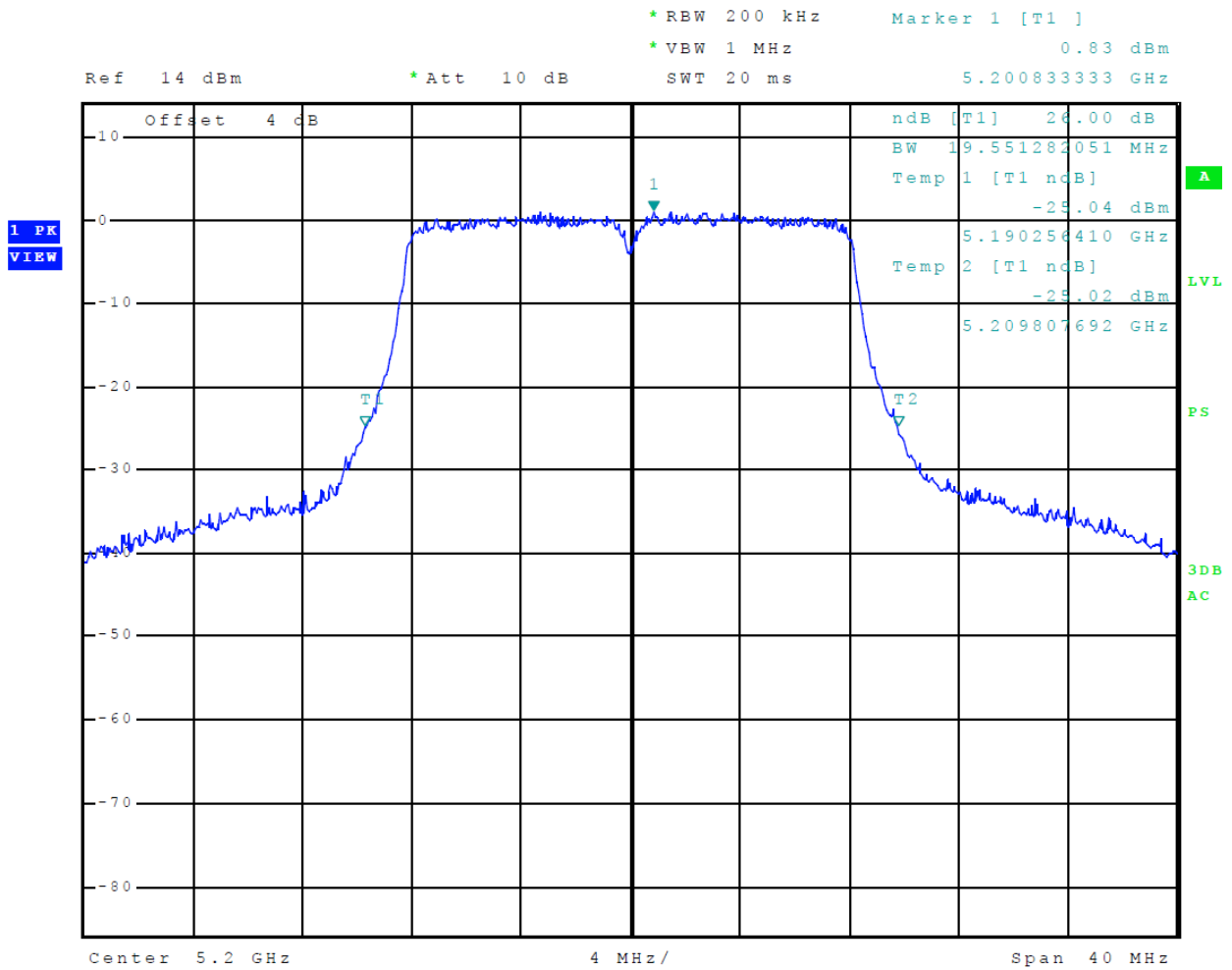
Figure 33 Plot of Transmitter Emissions (5150-5250 MHz Band, 802.11n, Chain 0, 26 dB OBW)
