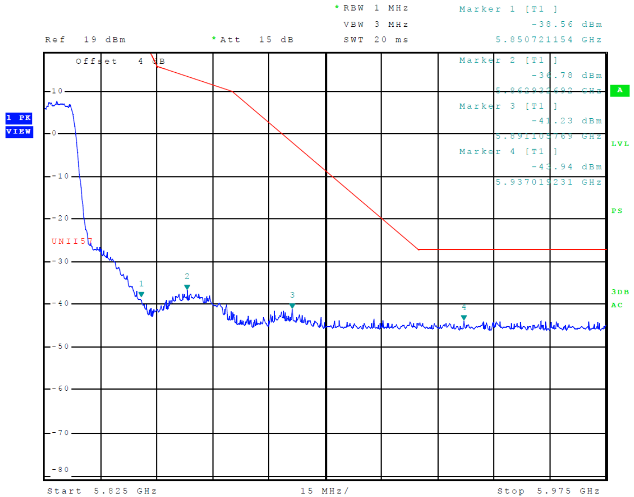
Figure 62 Plot of Transmitter High Band Edge (5725-5850 MHz Band, Chain 1, 802.11n)
