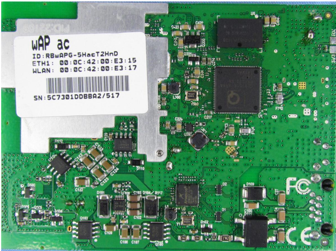
Bottom View with Shields (zoomed in)
