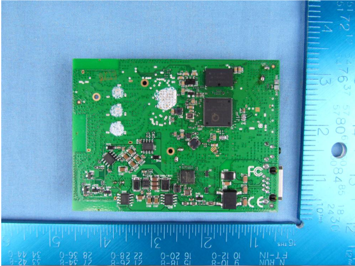
Bottom View without Shields
