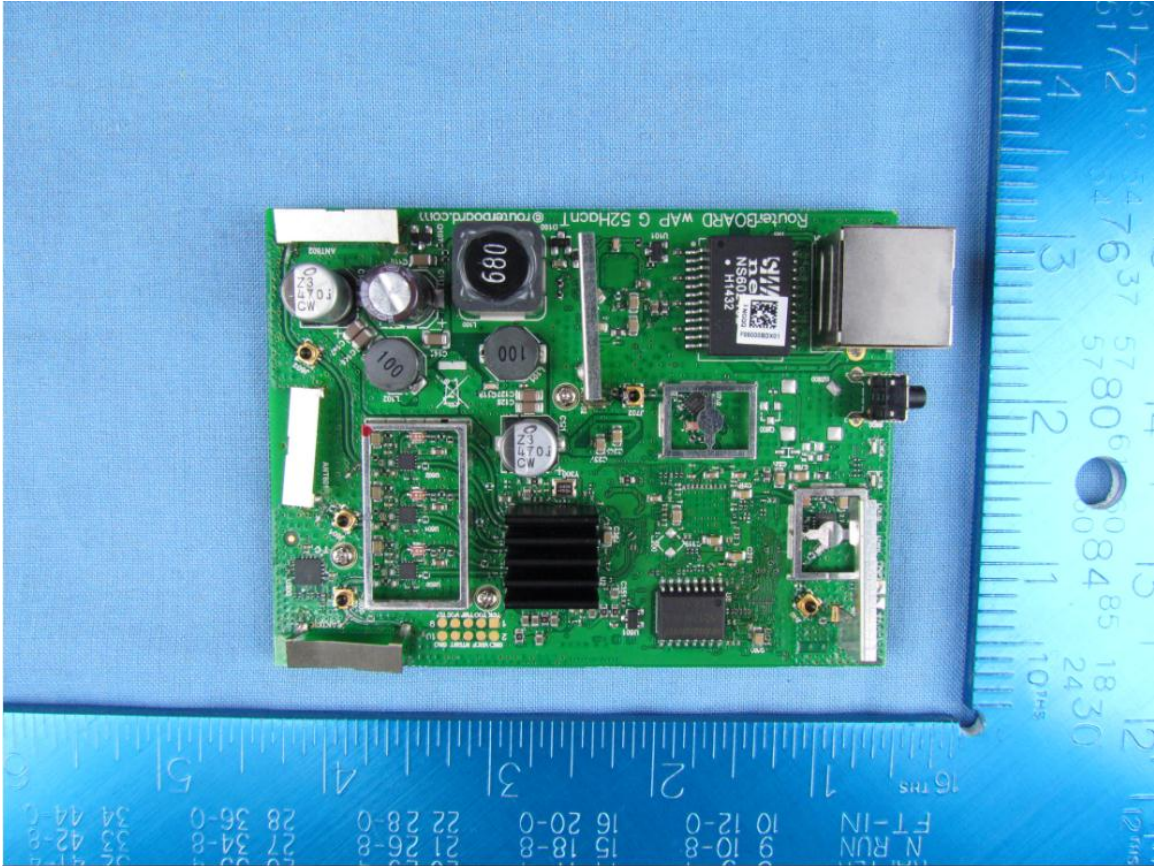
Top View without Shields
