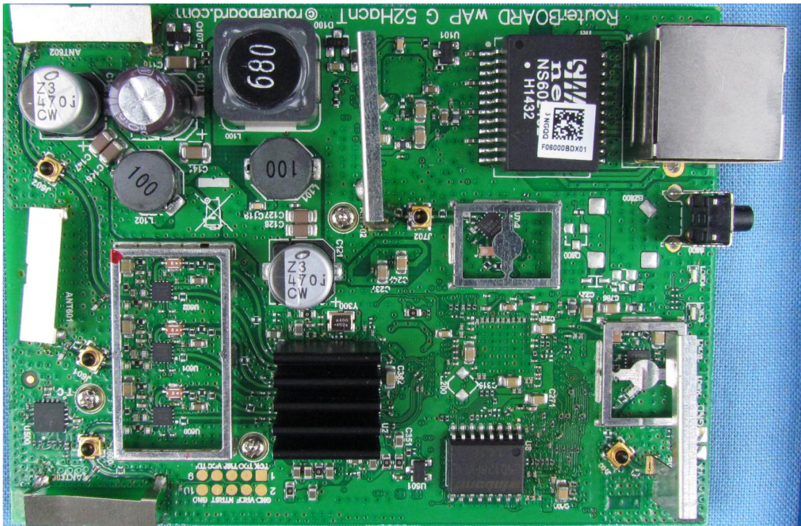
Top View without Shields (zoomed in)
