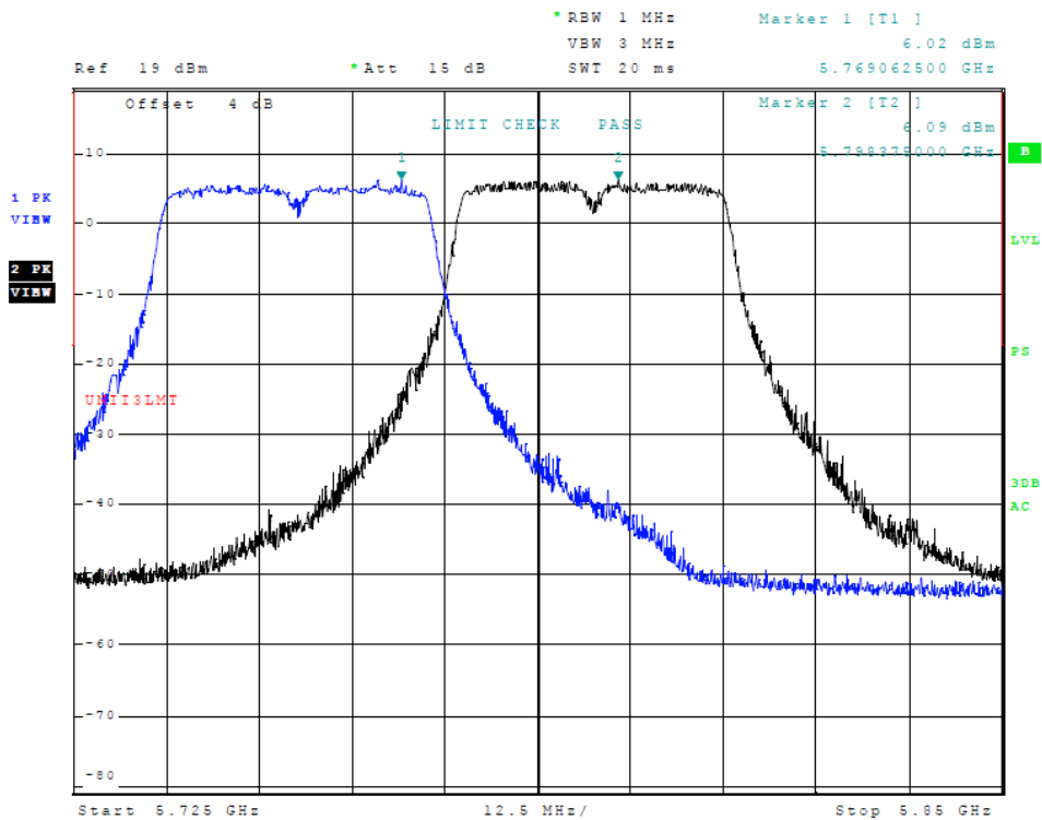
Figure 16 Plot of Transmitter Emissions (Across 5725-5850 MHz Band, 802.11n40, Chain 0)
