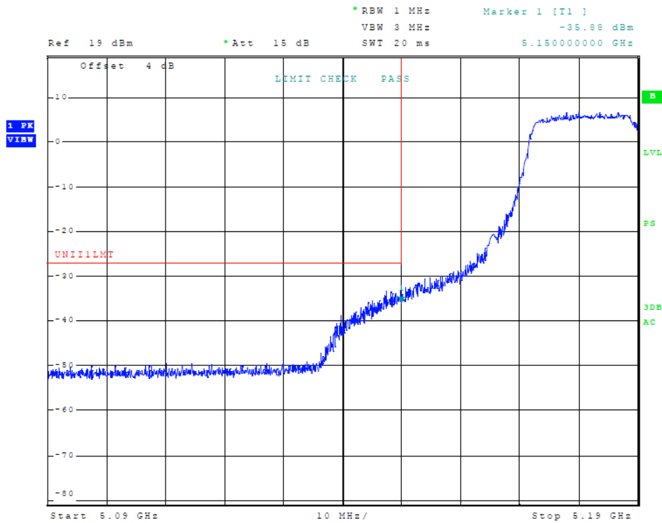
Figure 7 Plot of Transmitter Low Band Edge (5150-5250 MHz Band, 802.11n40, Chain 0)
