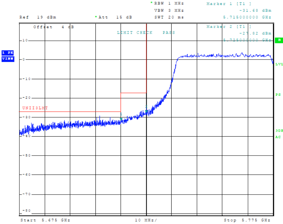
Figure 47 Plot of Transmitter Low Band Edge (5725-5850 MHz Band, 802.11ac, Chain 1)
