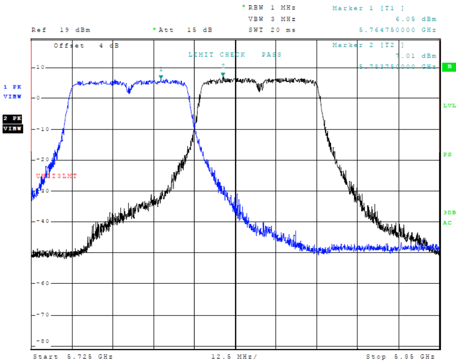
Figure 70 Plot of Transmitter Emissions (Across 5725-5850 MHz Band, 802.11n40, Chain 2)
