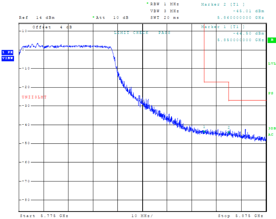
Figure 77 Plot of Transmitter High Band Edge (5725-5850 MHz Band, 802.11ac, Chain 2)
