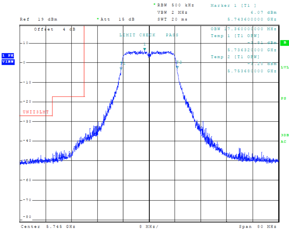
Figure 78 Plot of Transmitter Emissions (5725-5850 MHz Band, 802.11a, Chain 2, 99% OBW)
