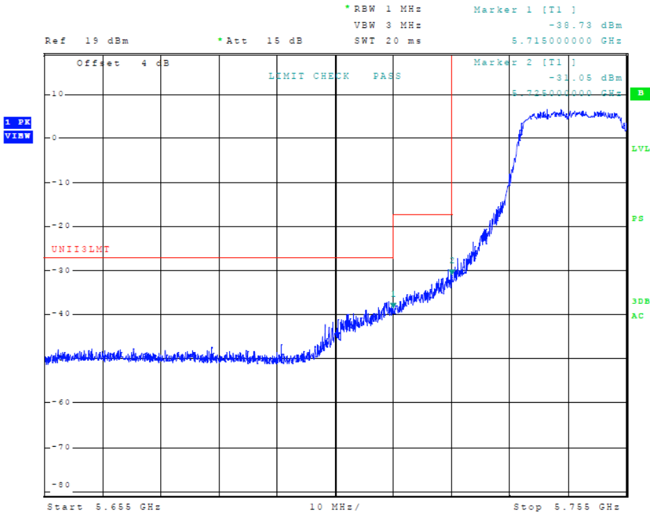
Figure 73 Plot of Transmitter Low Band Edge (5725-5850 MHz Band, 802.11n40, Chain 2)
