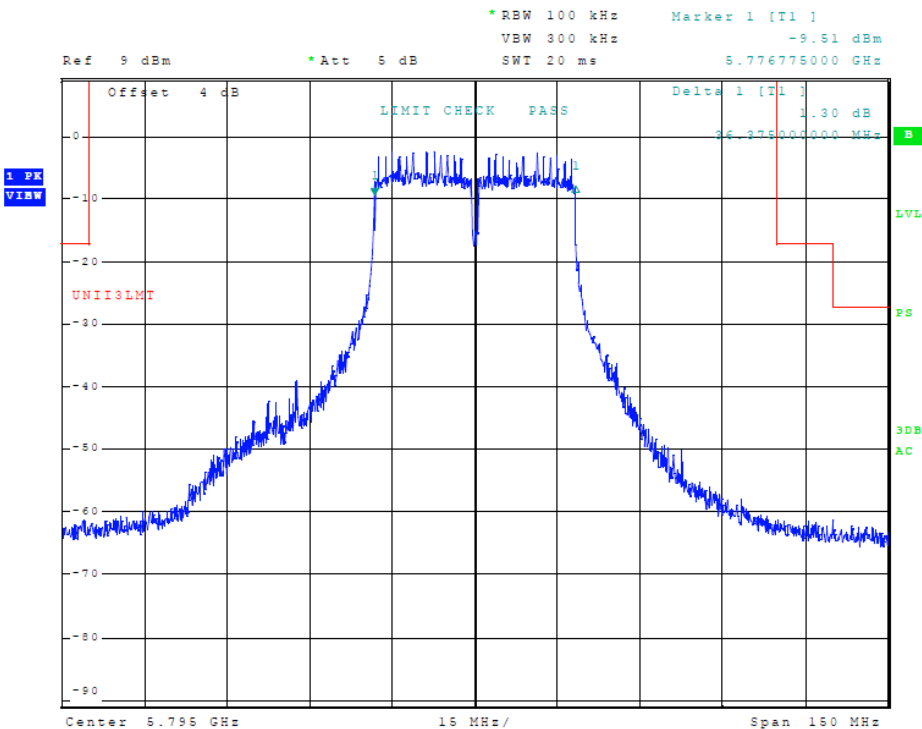
Figure 54 Plot of Transmitter Emissions (5725-5850 MHz Band, 802.11n40, Chain 1, 6-dB OBW)
