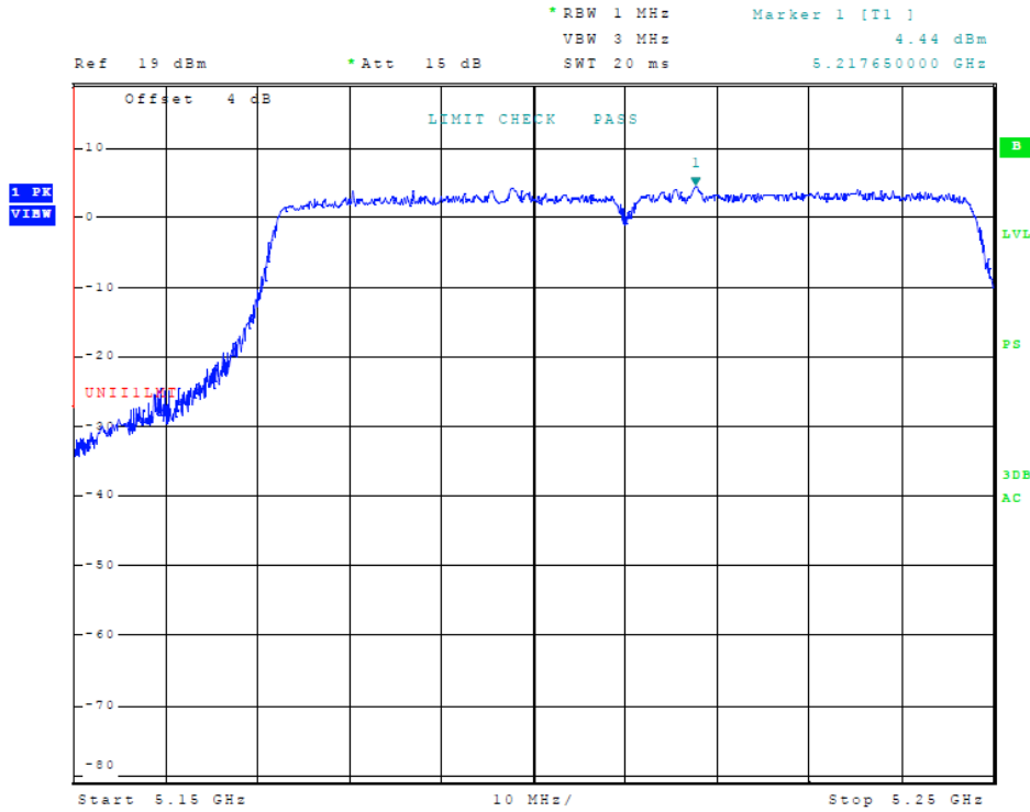
Figure 59 Plot of Transmitter Emissions (Across 5150-5250 MHz Band, 802.11ac, Chain 2)
