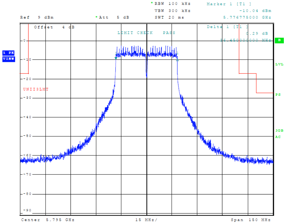
Figure 27 Plot of Transmitter Emissions (5725-5850 MHz Band, 802.11n40, Chain 0, 6-dB OBW)
