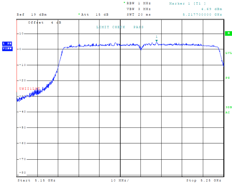
Figure 5 Plot of Transmitter Emissions (Across 5150-5250 MHz Band, 802.11ac, Chain 0)
