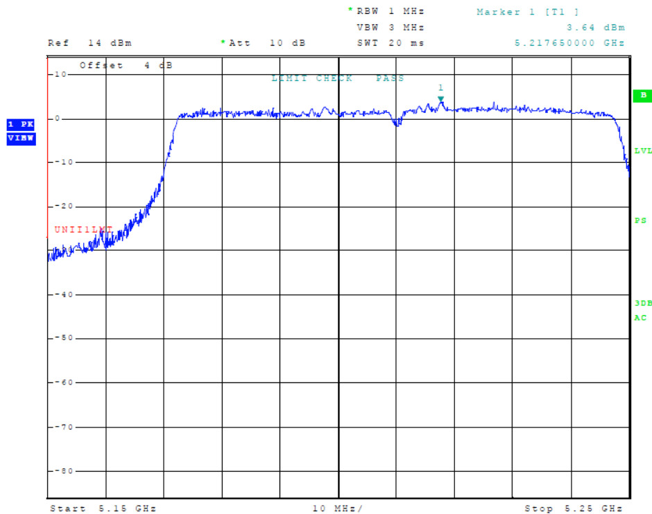
Figure 32 Plot of Transmitter Emissions (Across 5150-5250 MHz Band, 802.11ac, Chain 1)
