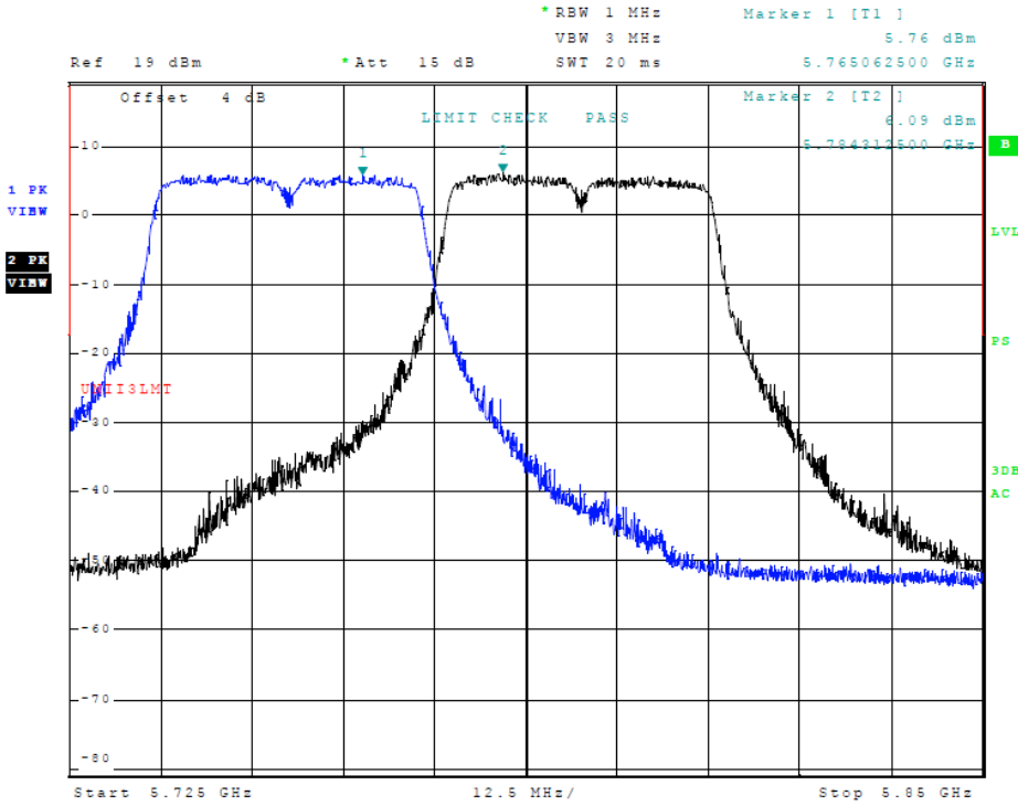
Figure 43 Plot of Transmitter Emissions (Across 5725-5850 MHz Band, 802.11n40, Chain 1)
