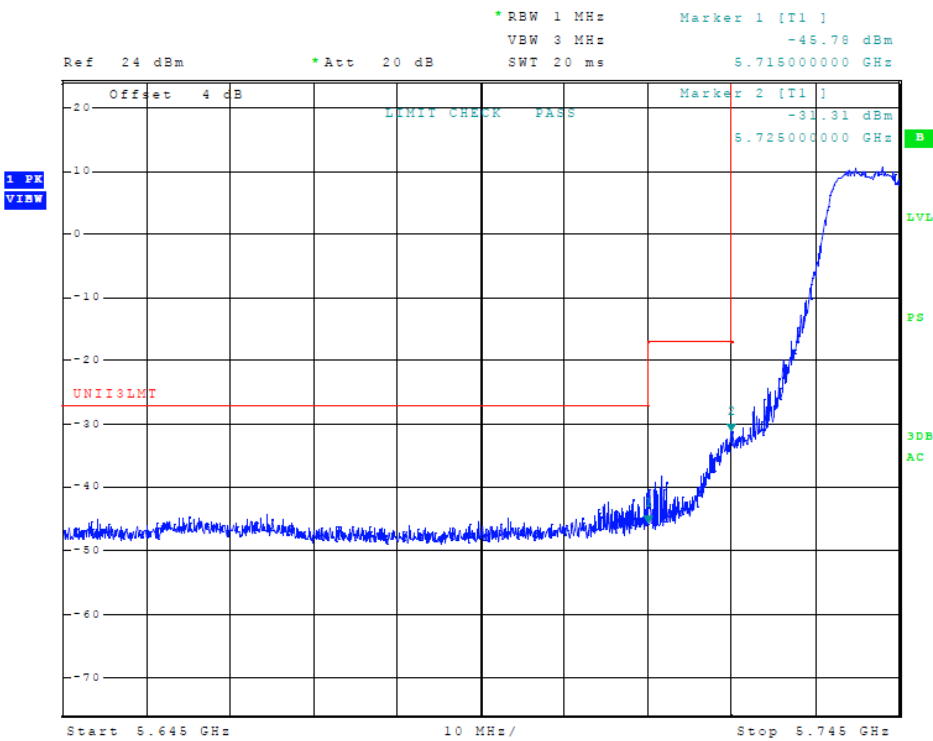
Figure 72 Plot of Transmitter Low Band Edge (5725-5850 MHz Band, 802.11a, Chain 2)
