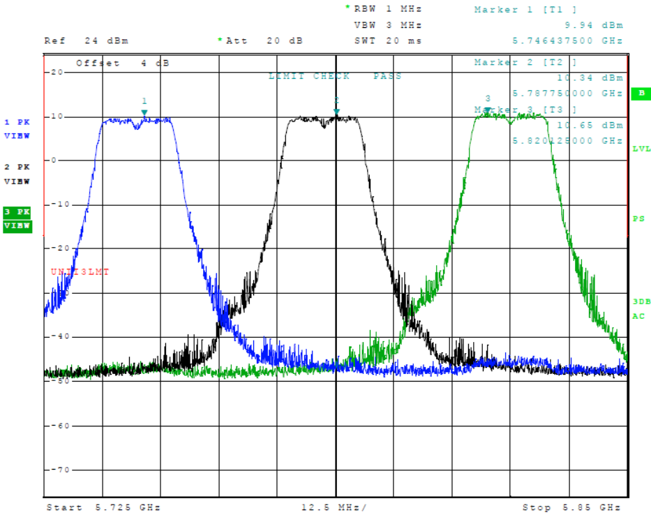
Figure 69 Plot of Transmitter Emissions (Across 5725-5850 MHz Band, 802.11a, Chain 2)
