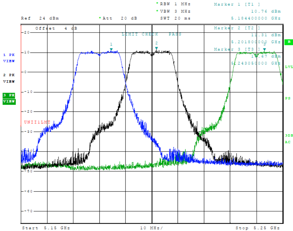
Figure 57 Plot of Transmitter Emissions (Across 5150-5250 MHz Band, 802.11a, Chain 2)
