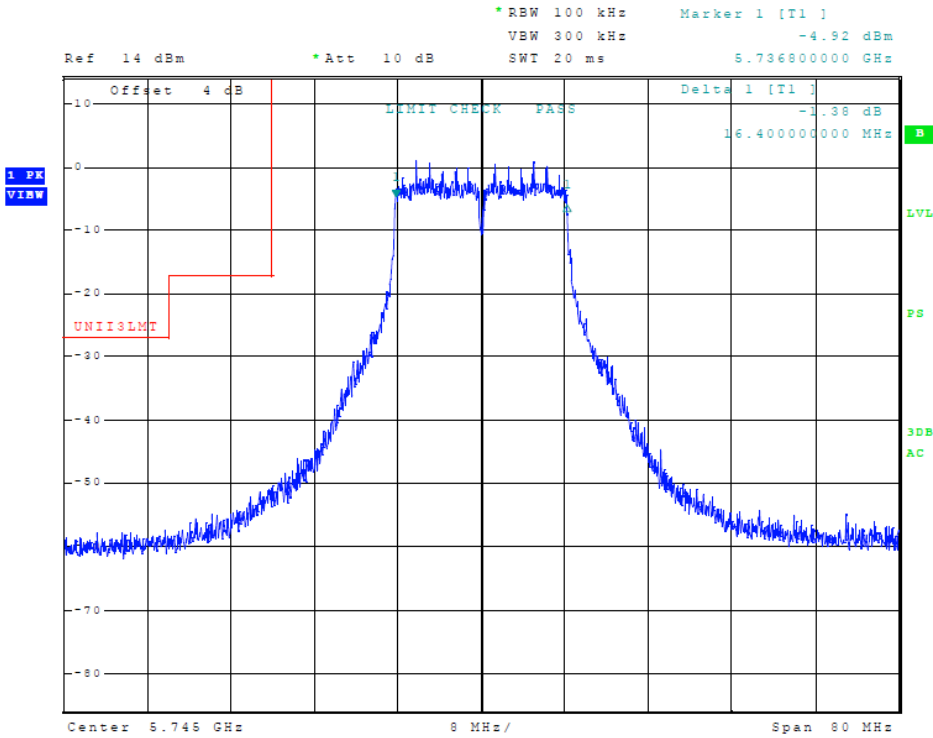
Figure 79 Plot of Transmitter Emissions (5725-5850 MHz Band, 802.11a, Chain 2, 6-dB OBW)
