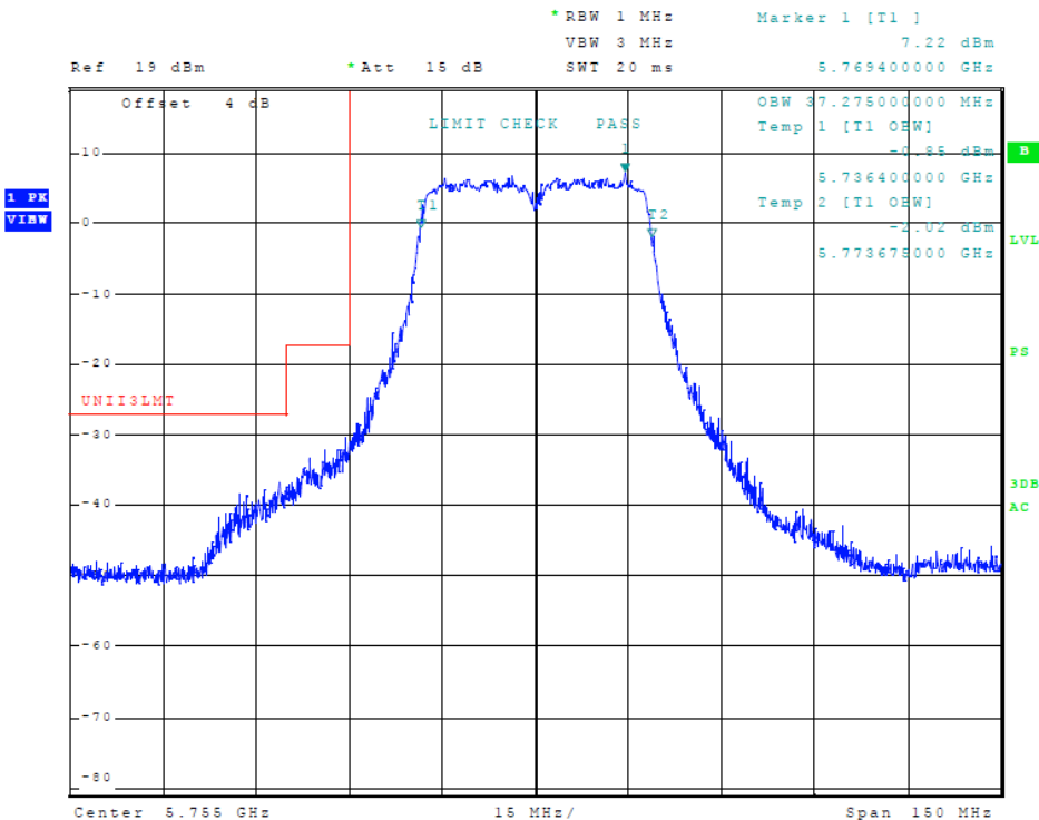
Figure 80 Plot of Transmitter Emissions (5725-5850 MHz Band, 802.11n40, Chain 2, 99% OBW)
