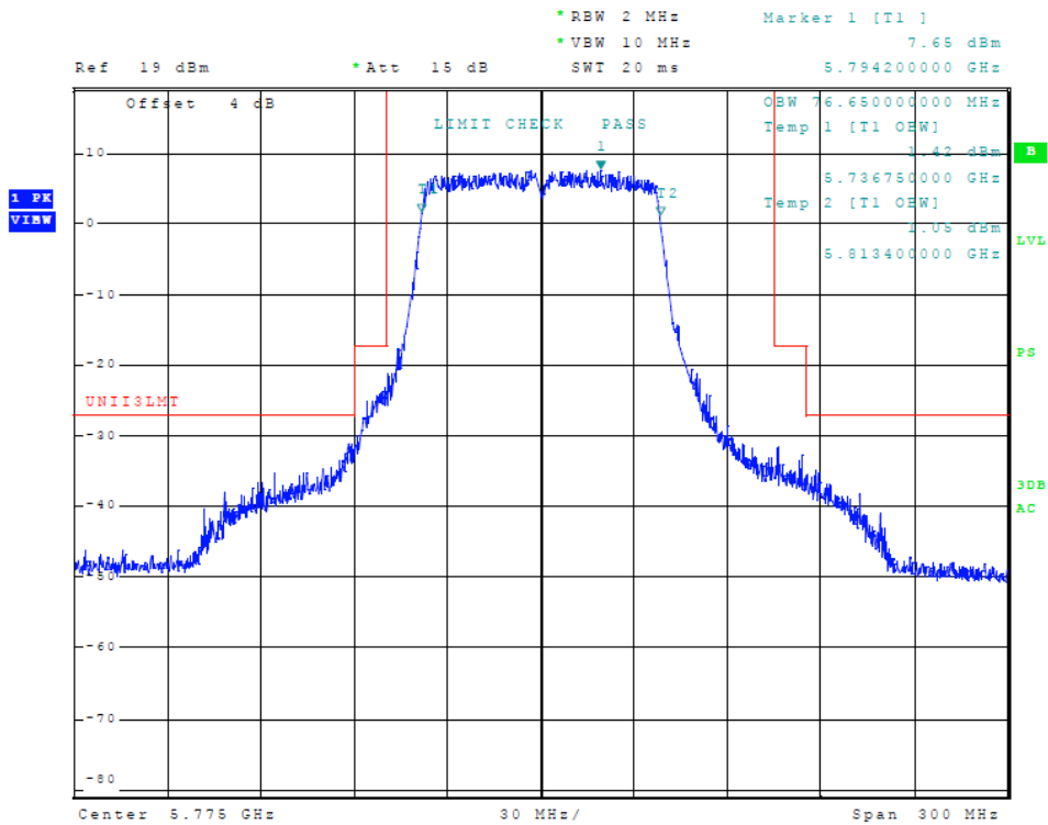
Figure 28 Plot of Transmitter Emissions (5725-5850 MHz Band, 802.11ac, Chain 0, 99% OBW)
