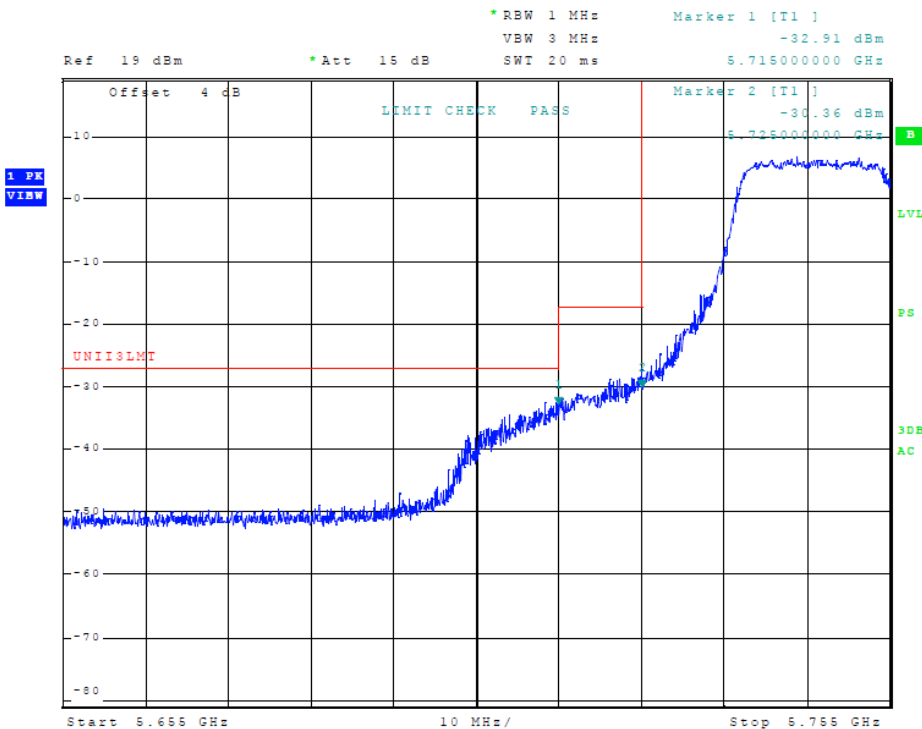
Figure 46 Plot of Transmitter Low Band Edge (5725-5850 MHz Band, 802.11n40, Chain 1)
