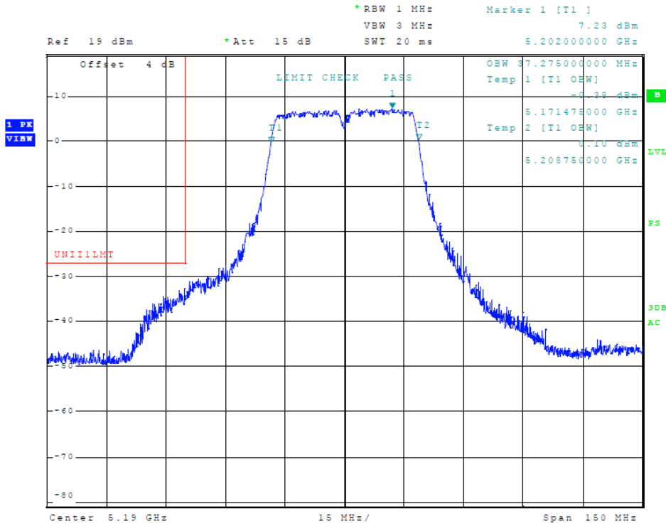
Figure 67 Plot of Transmitter Emissions (5150-5250 MHz Band, 822.11n40, Chain 2, 99% OBW)
