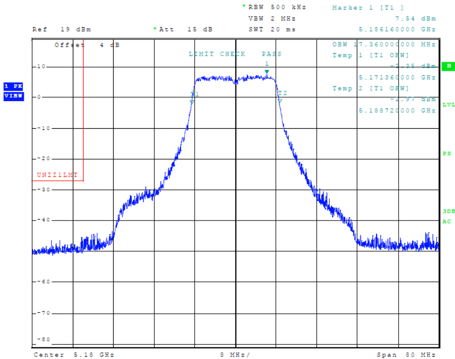
Figure 66 Plot of Transmitter Emissions (5150-5250 MHz Band, 802.11a, Chain 2, 99% OBW)
