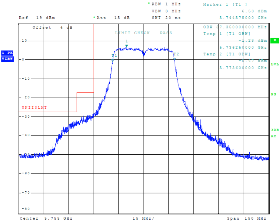
Figure 53 Plot of Transmitter Emissions (5725-5850 MHz Band, 802.11n40, Chain 1, 99% OBW)
