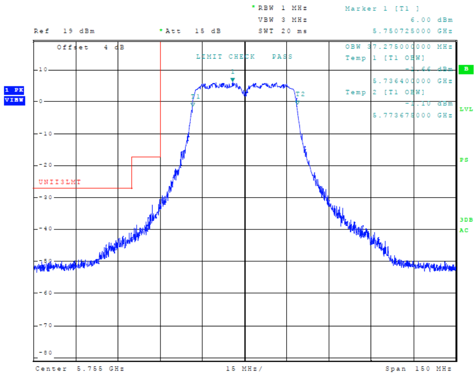
Figure 26 Plot of Transmitter Emissions (5725-5850 MHz Band, 802.11n40, Chain 0, 99% OBW)
