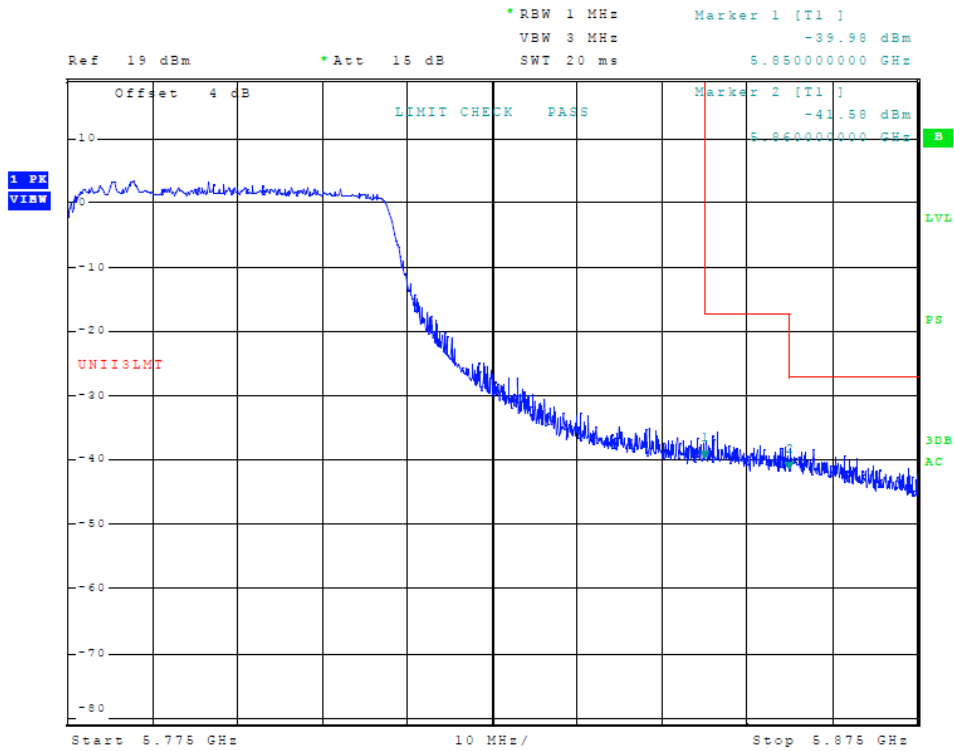
Figure 23 Plot of Transmitter High Band Edge (5725-5850 MHz Band, 802.11ac, Chain 0)
