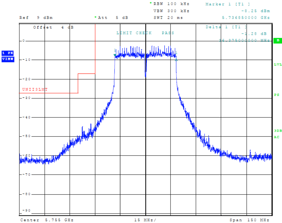
Figure 81 Plot of Transmitter Emissions (5725-5850 MHz Band, 802.11n40, Chain 2, 6-dB OBW)
