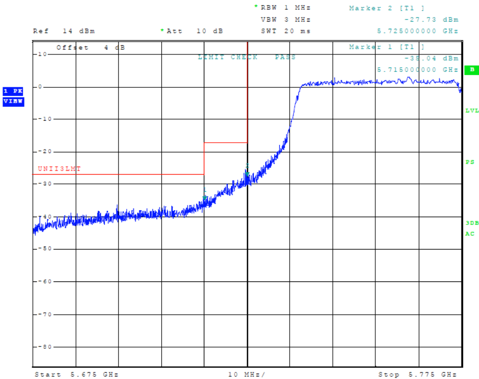
Figure 74 Plot of Transmitter Low Band Edge (5725-5850 MHz Band, 802.11ac, Chain 2)
