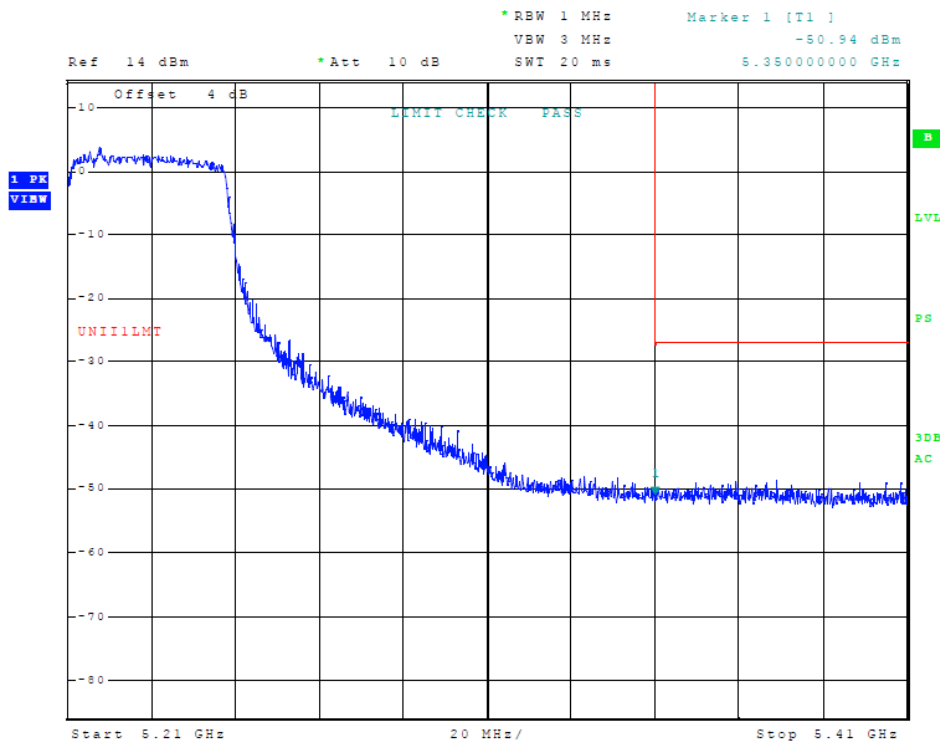
Figure 38 Plot of Transmitter High Band Edge (5150-5250 MHz Band, 802.11ac, Chain 1)
