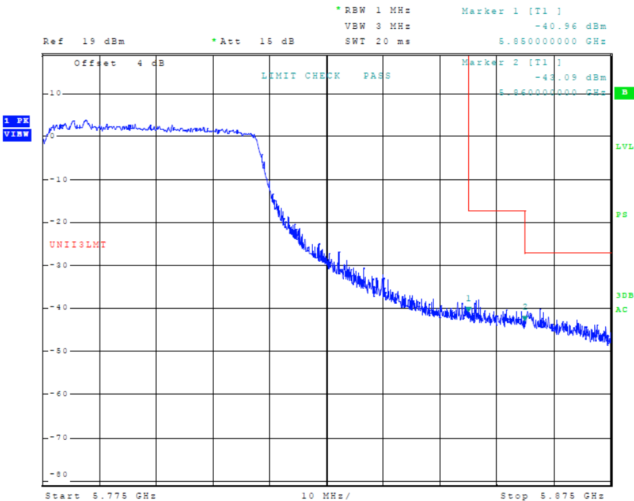
Figure 50 Plot of Transmitter High Band Edge (5725-5850 MHz Band, 802.11ac, Chain 1)
