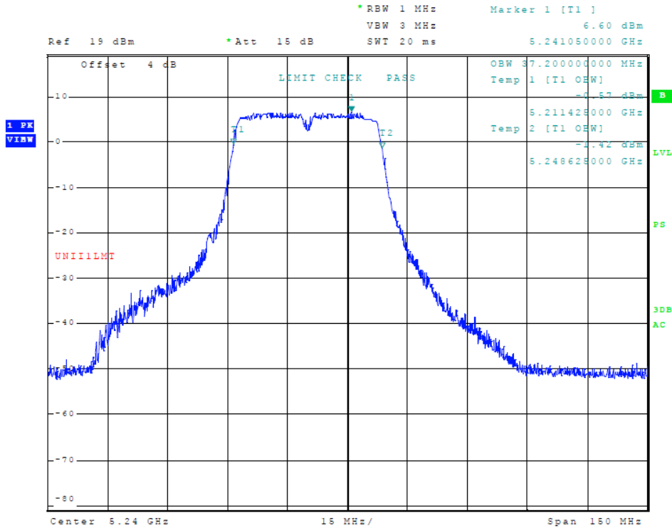
Figure 13 Plot of Transmitter Emissions (5150-5250 MHz Band, 802.11n40, Chain 0, 99% OBW)
