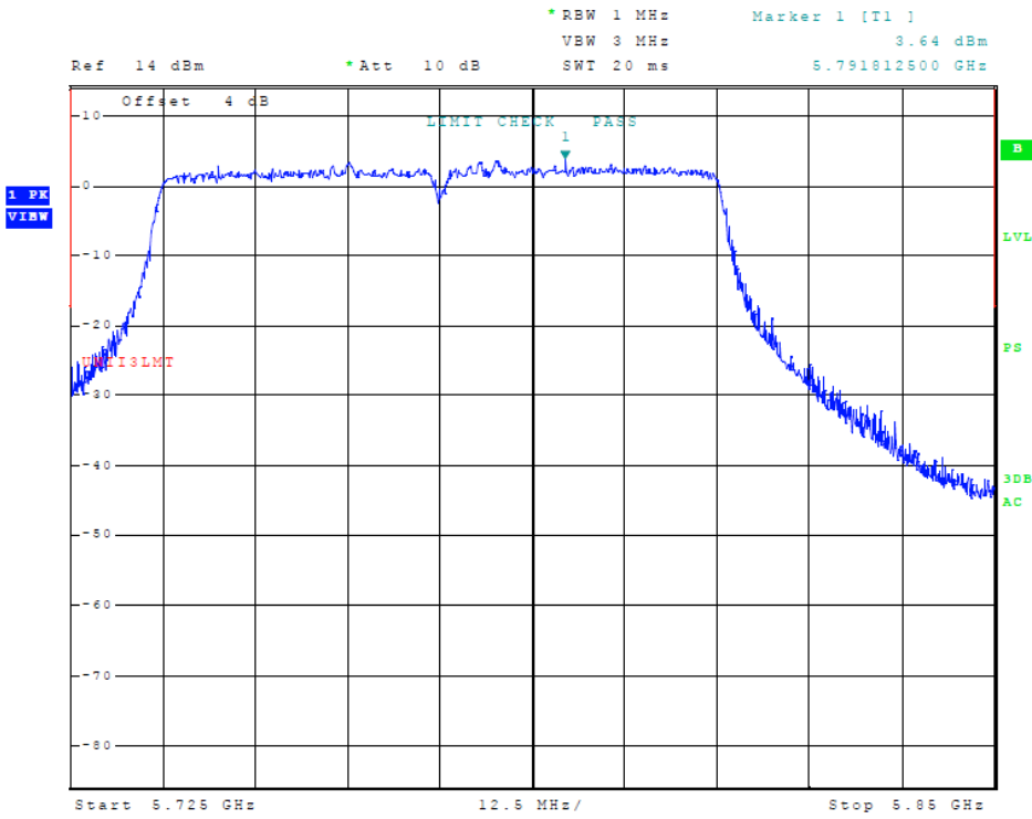
Figure 71 Plot of Transmitter Emissions (Across 5725-5850 MHz Band, 802.11ac, Chain 2)
