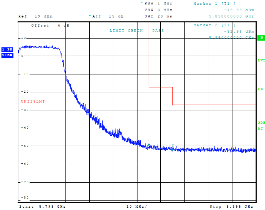
Figure 49 Plot of Transmitter High Band Edge (5725-5850 MHz Band, 802.11n40, Chain 1)
