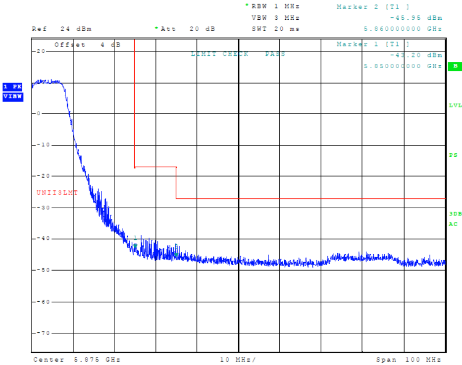
Figure 75 Plot of Transmitter High Band Edge (5725-5850 MHz Band, 802.11a, Chain 2)
