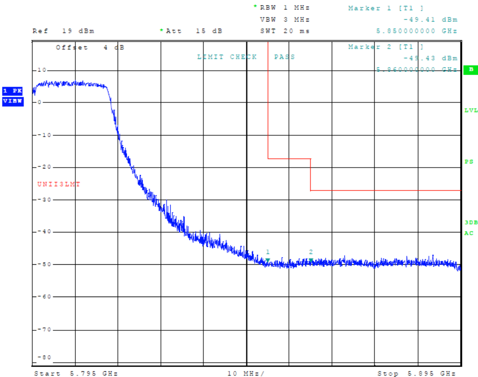
Figure 76 Plot of Transmitter High Band Edge (5725-5850 MHz Band, 802.11n40, Chain 2)
