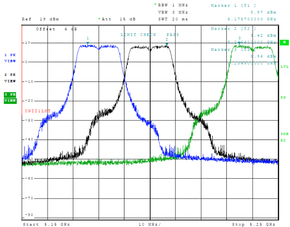
Figure 30 Plot of Transmitter Emissions (Across 5150-5250 MHz Band, 802.11a, Chain 1)
