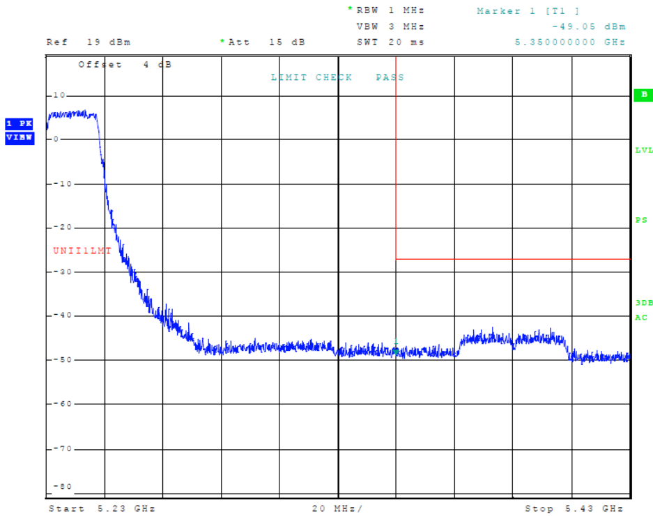
Figure 64 Plot of Transmitter High Band Edge (5150-5250 MHz Band, 802.11n40, Chain 2)
