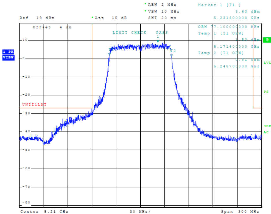
Figure 68 Plot of Transmitter Emissions (5150-5250 MHz Band, 822.11ac, Chain 2, 99% OBW)
