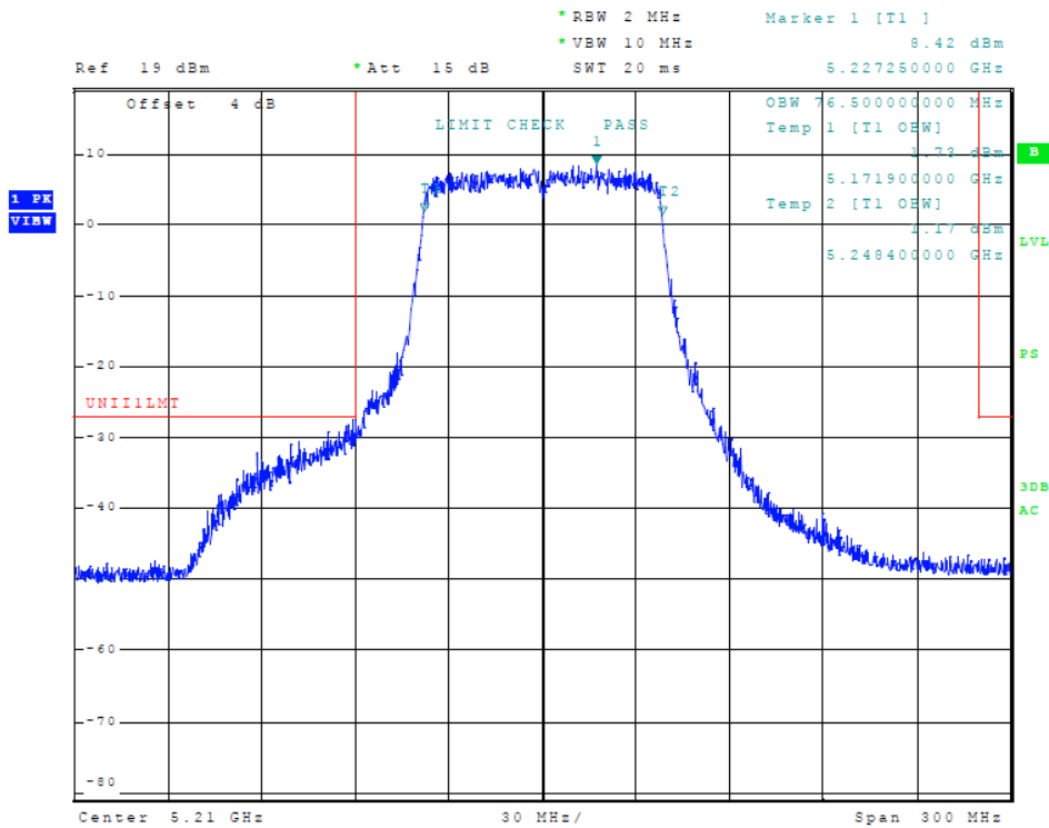
Figure 14 Plot of Transmitter Emissions (5150-5250 MHz Band, 802.11ac, Chain 0, 99% OBW)
