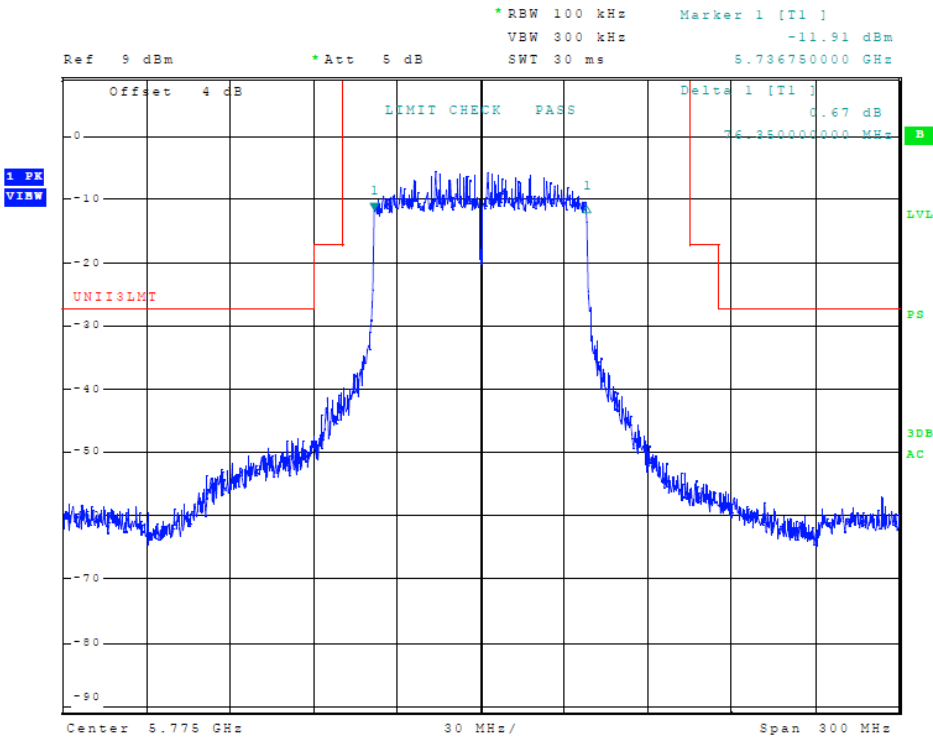
Figure 83 Plot of Transmitter Emissions (5725-5850 MHz Band, 802.11ac, Chain 2, 6-dB OBW)
