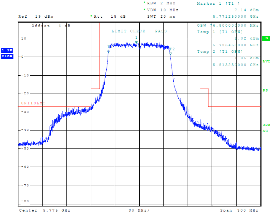
Figure 55 Plot of Transmitter Emissions (5725-5850 MHz Band, 802.11ac, Chain 1, 99% OBW)
