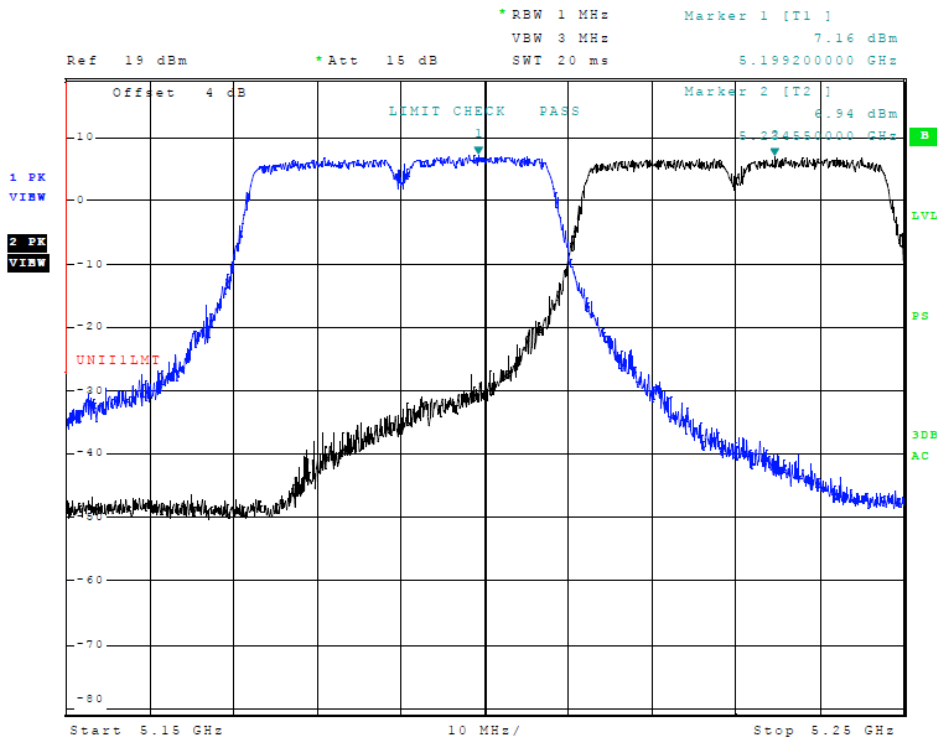
Figure 58 Plot of Transmitter Emissions (Across 5150-5250 MHz Band, 802.11n40, Chain 2)
