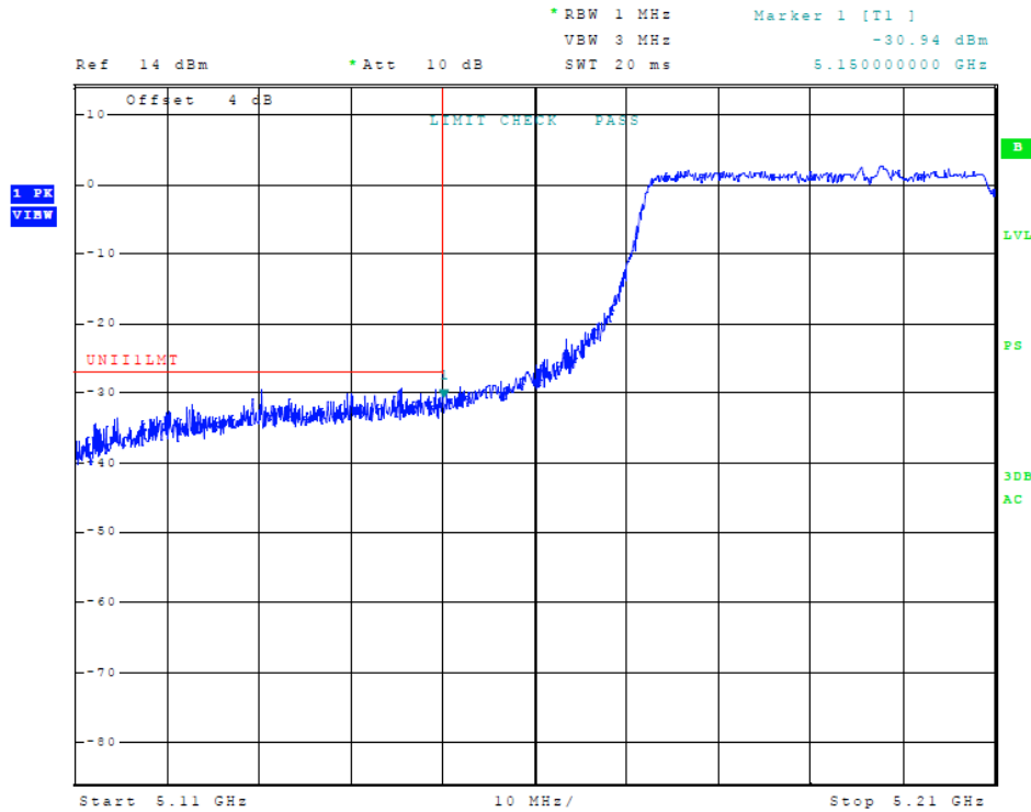
Figure 35 Plot of Transmitter Low Band Edge (5150-5250 MHz Band, 802.11ac, Chain 1)
