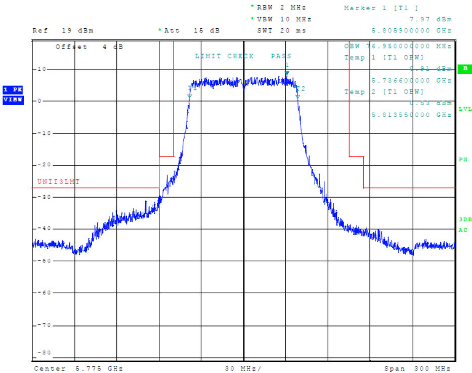
Figure 82 Plot of Transmitter Emissions (5725-5850 MHz Band, 802.11ac, Chain 2, 99% OBW)
