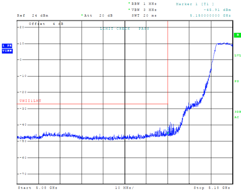
Figure 60 Plot of Transmitter Low Band Edge (5150-5250 MHz Band, 802.11a, Chain 2)
