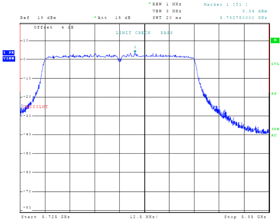
Figure 17 Plot of Transmitter Emissions (Across 5725-5850 MHz Band, 802.11ac, Chain 0)
