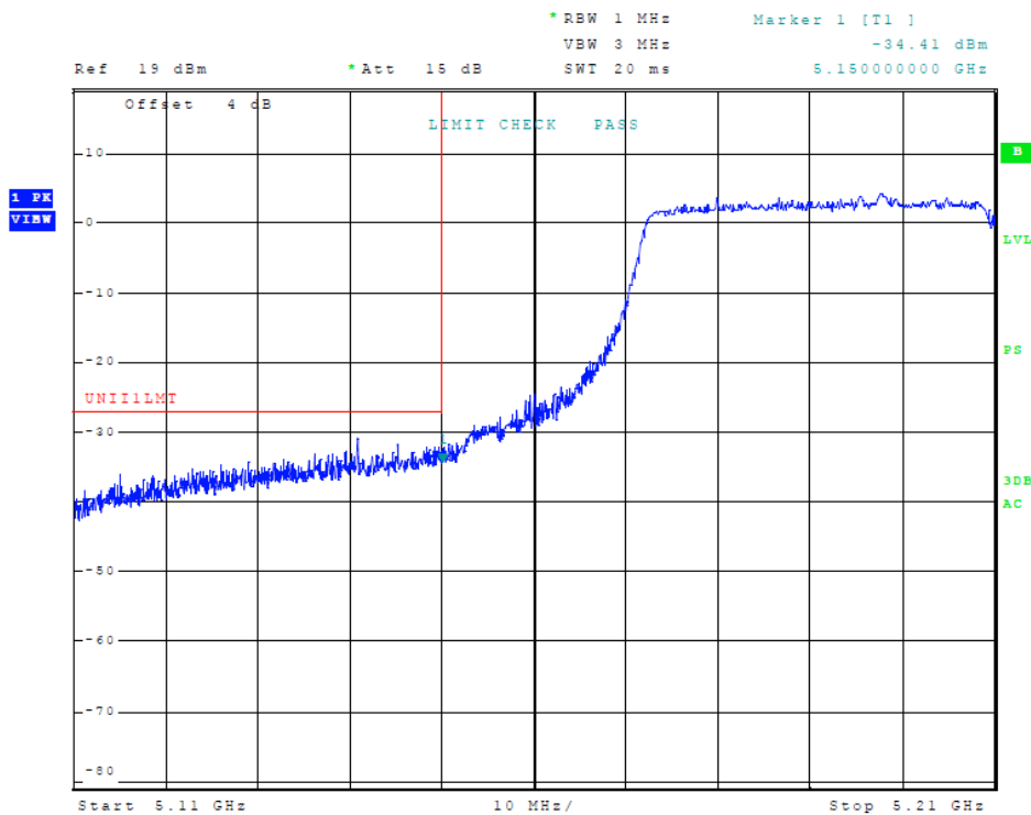
Figure 62 Plot of Transmitter Low Band Edge (5150-5250 MHz Band, 802.11ac, Chain 2)
