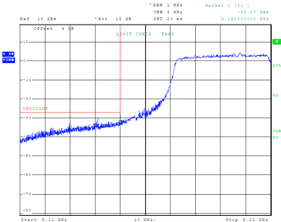
Figure 8 Plot of Transmitter Low Band Edge (5150-5250 MHz Band, 802.11ac, Chain 0)
