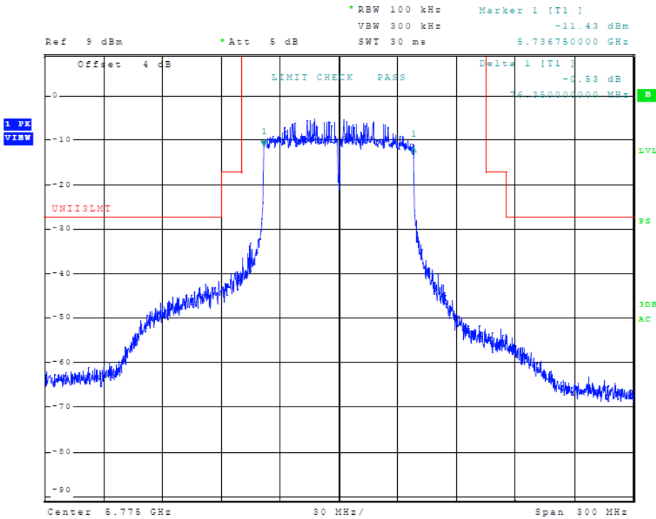
Figure 56 Plot of Transmitter Emissions (5725-5850 MHz Band, 802.11ac, Chain 1, 6-dB OBW)
