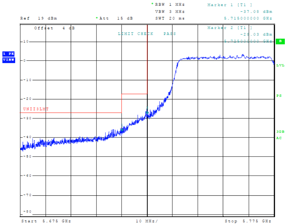
Figure 20 Plot of Transmitter Low Band Edge (5725-5850 MHz Band, 802.11ac, Chain 0)
