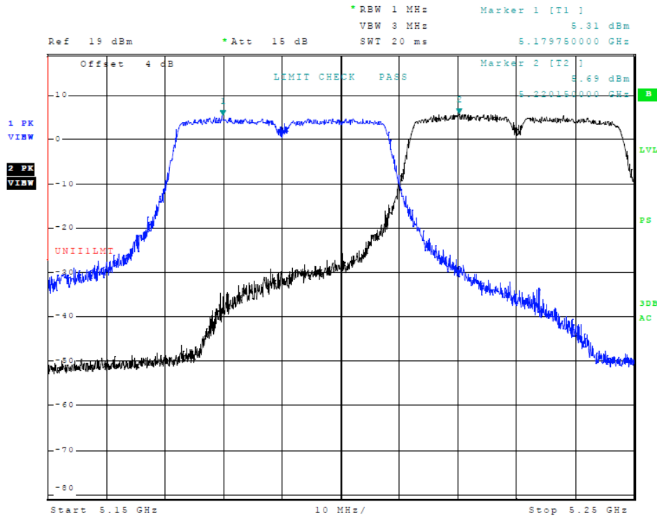
Figure 31 Plot of Transmitter Emissions (Across 5150-5250 MHz Band, 802.11n40, Chain 1)
