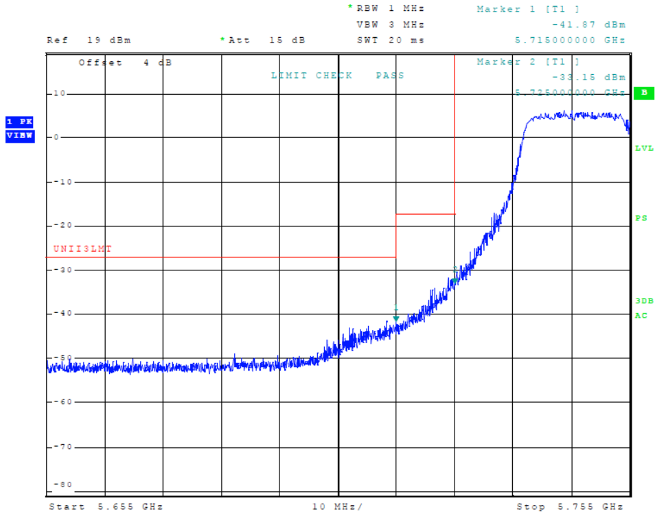
Figure 19 Plot of Transmitter Low Band Edge (5725-5850 MHz Band, 802.11n40, Chain 0)
