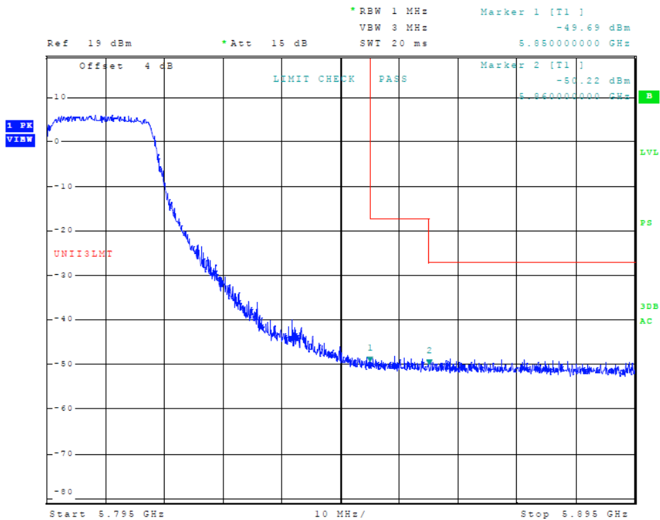
Figure 22 Plot of Transmitter High Band Edge (5725-5850 MHz Band, 802.11n40, Chain 0)
