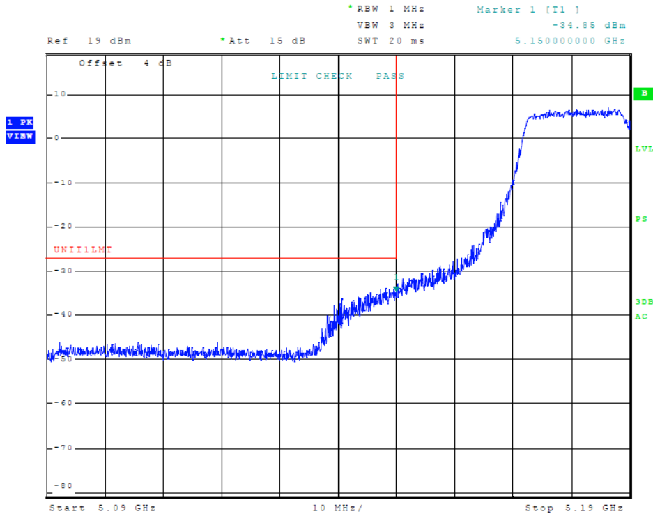
Figure 61 Plot of Transmitter Low Band Edge (5150-5250 MHz Band, 802.11n40, Chain 2)
