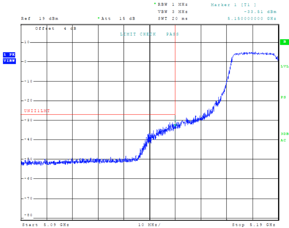
Figure 34 Plot of Transmitter Low Band Edge (5150-5250 MHz Band, 802.11n40, Chain 1)
