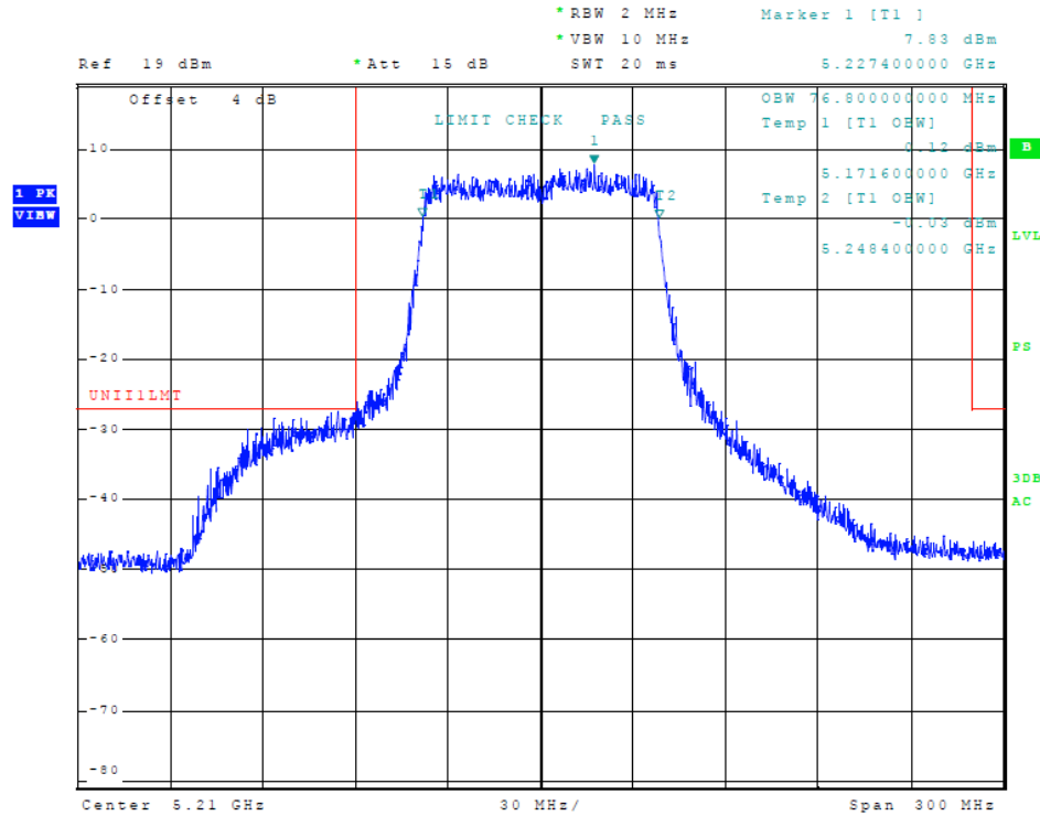
Figure 41 Plot of Transmitter Emissions (5150-5250 MHz Band, 822.11ac, Chain 1, 99% OBW)
