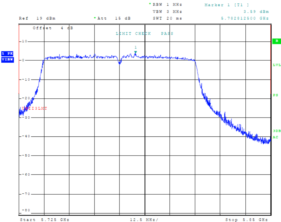
Figure 44 Plot of Transmitter Emissions (Across 5725-5850 MHz Band, 802.11ac, Chain 1)
