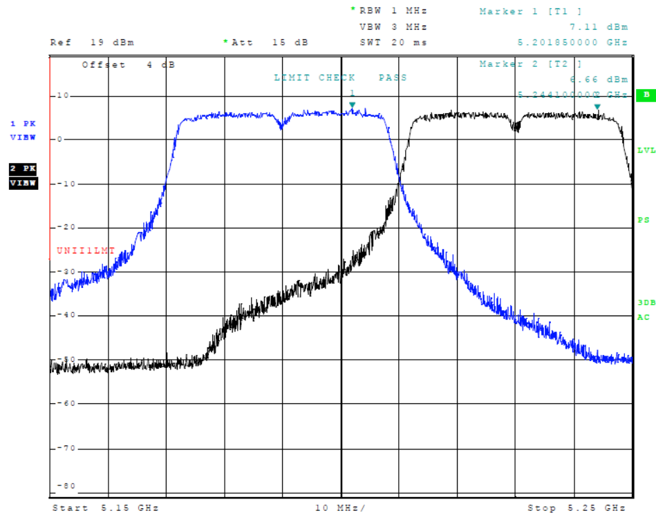
Figure 4 Plot of Transmitter Emissions (Across 5150-5250 MHz Band, 802.11n40, Chain 0)
