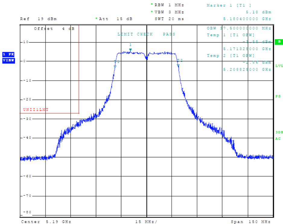
Figure 40 Plot of Transmitter Emissions (5150-5250 MHz Band, 822.11n40, Chain 1, 99% OBW)
