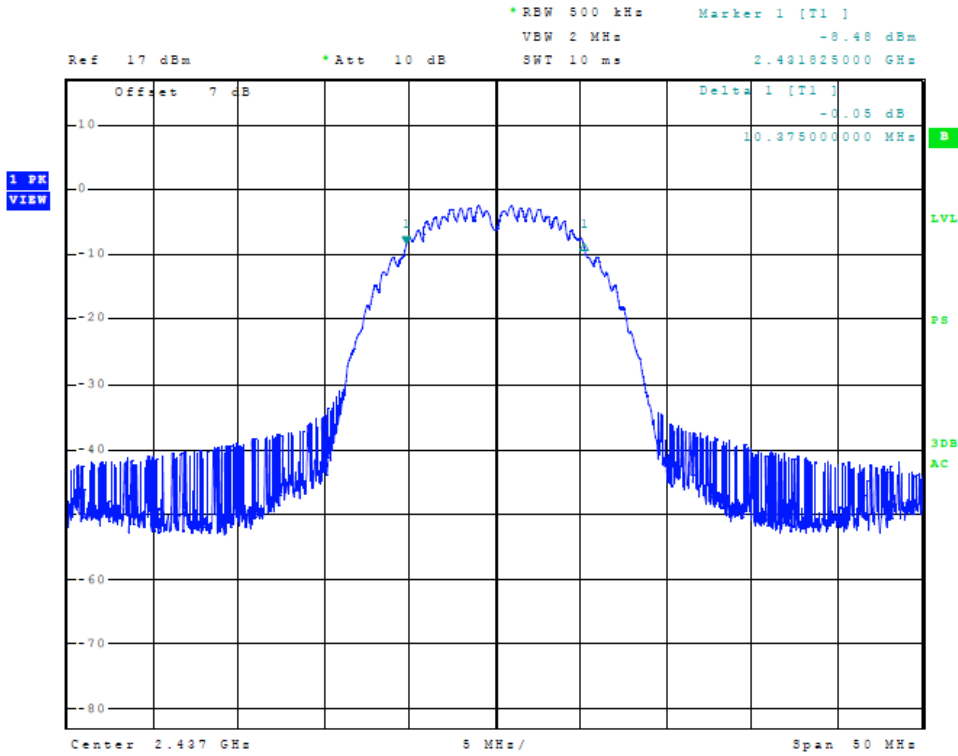
Figure 31 Plot of Transmitter 6-dB Occupied Band Width (802.11b, Chain 1)
