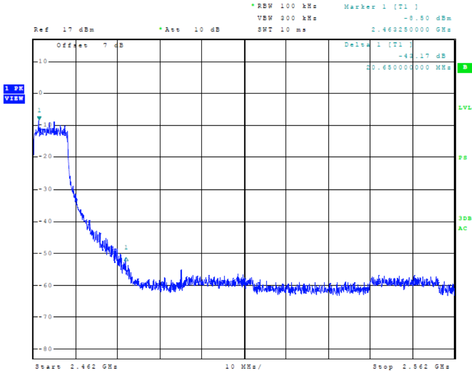
Figure 13 Plot of Transmitter High Band Edge (802.11n (20), Chain 0)
