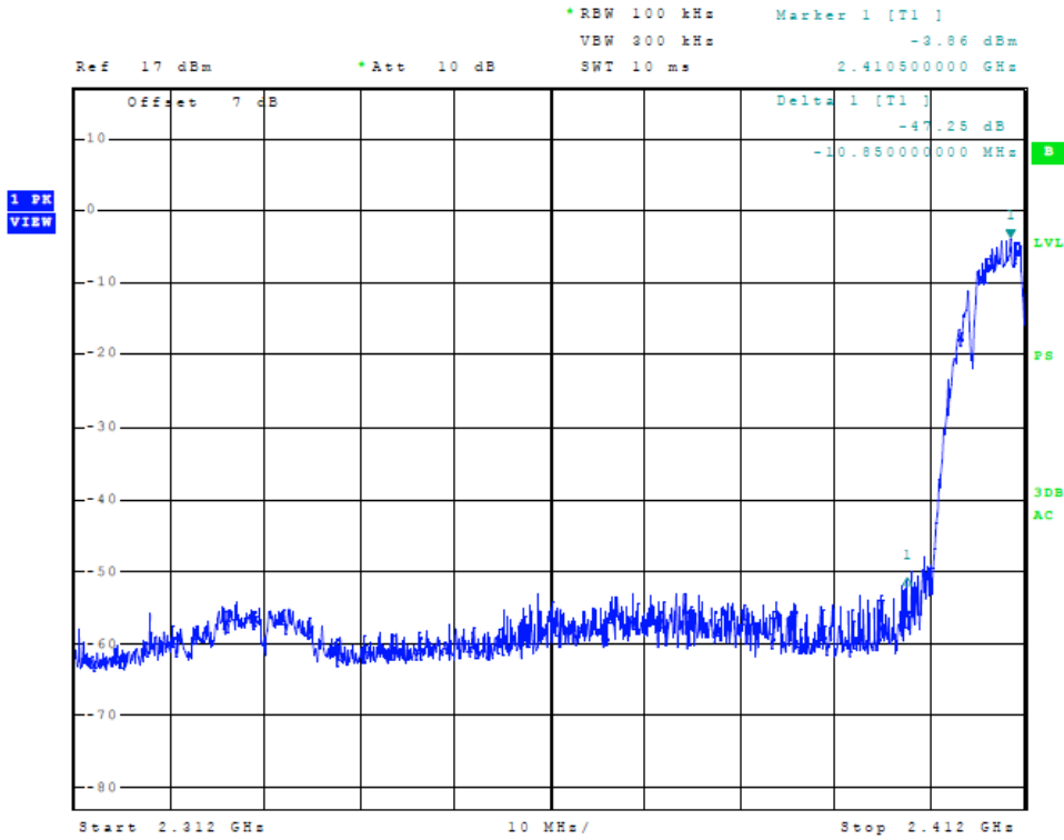
Figure 23 Plot of Transmitter Low Band Edge (802.11b, Chain 1)
