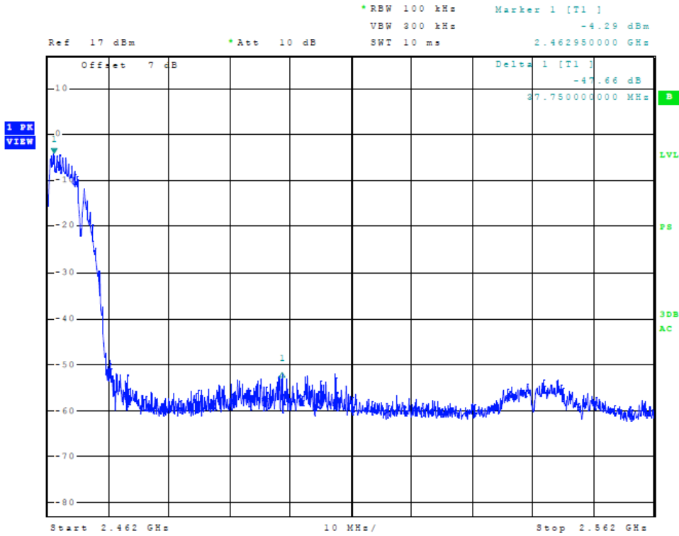
Figure 27 Plot of Transmitter High Band Edge (802.11b, Chain 1)
