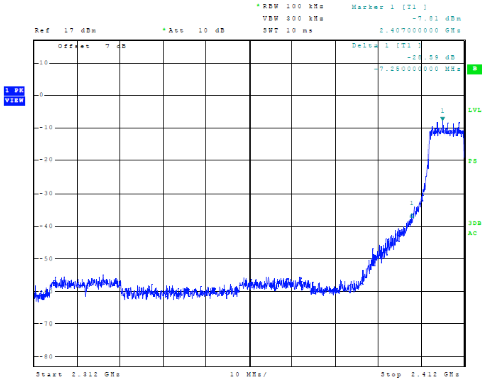
Figure 9 Plot of Transmitter Low Band Edge (802.11n (20), Chain 0)
