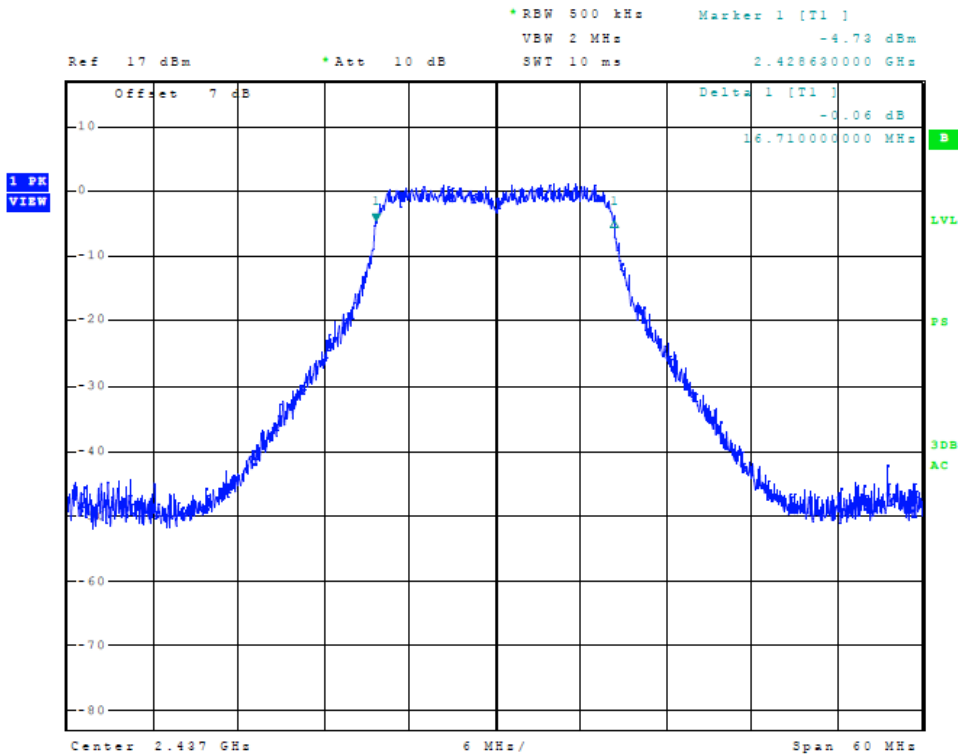
Figure 33 Plot of Transmitter 6-dB Occupied Band Width (802.11n (20), Chain 1)
