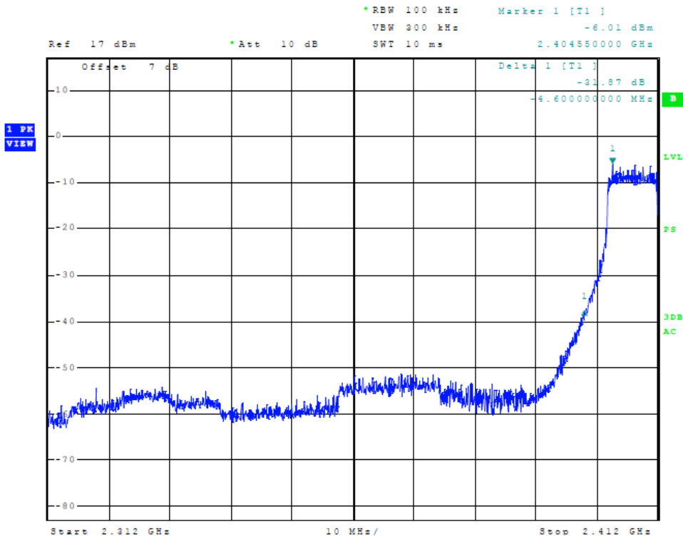
Figure 24 Plot of Transmitter Low Band Edge (802.11g, Chain 1)
