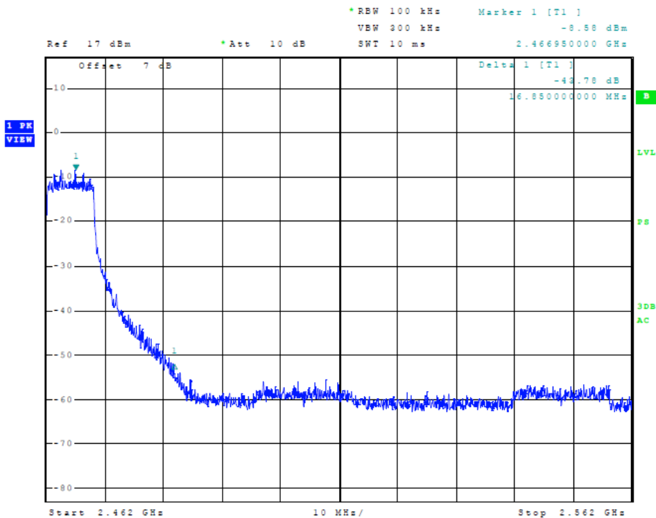
Figure 12 Plot of Transmitter High Band Edge (802.11g, Chain 0)
