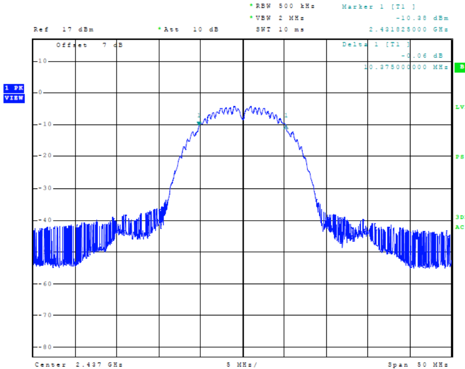
Figure 15 Plot of Transmitter 6-dB Occupied Band Width (802.11b, Chain 0)
