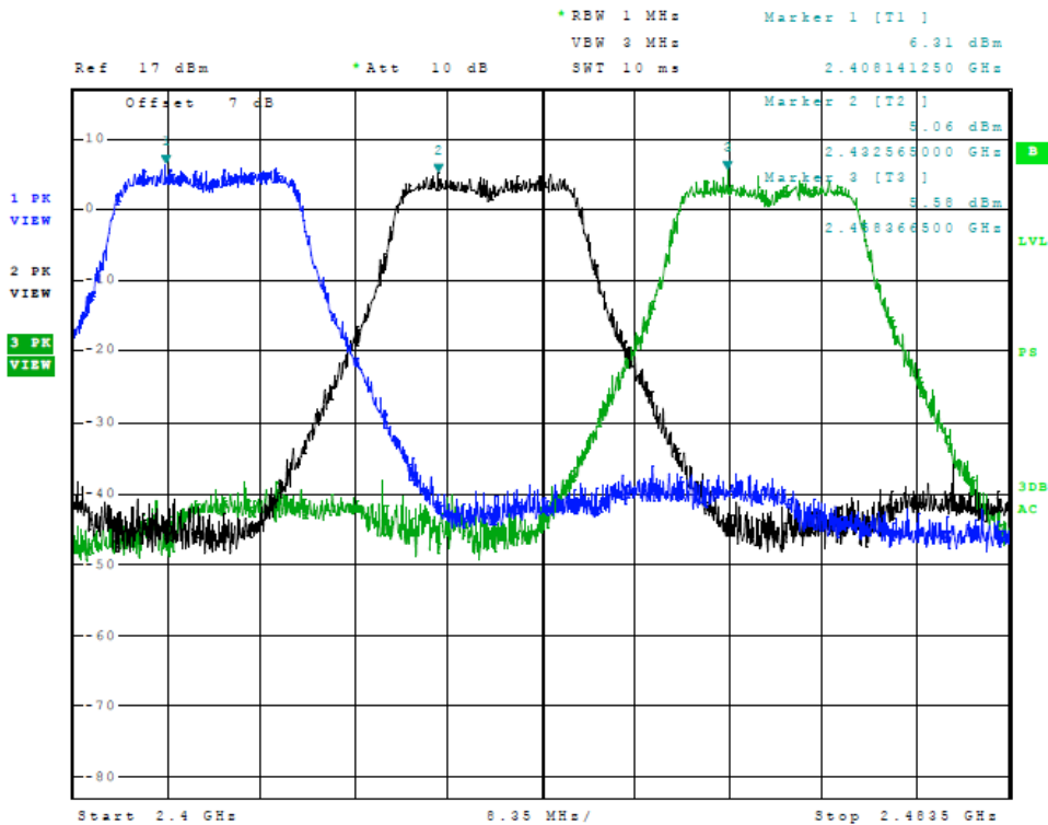
Figure 20 Plot of Transmitter Emissions (Across Operational Band, 802.11g, Chain 01)
