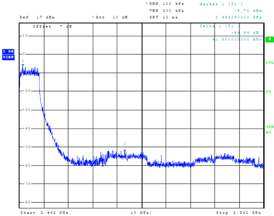
Figure 29 Plot of Transmitter High Band Edge (802.11n (20), Chain 1)
