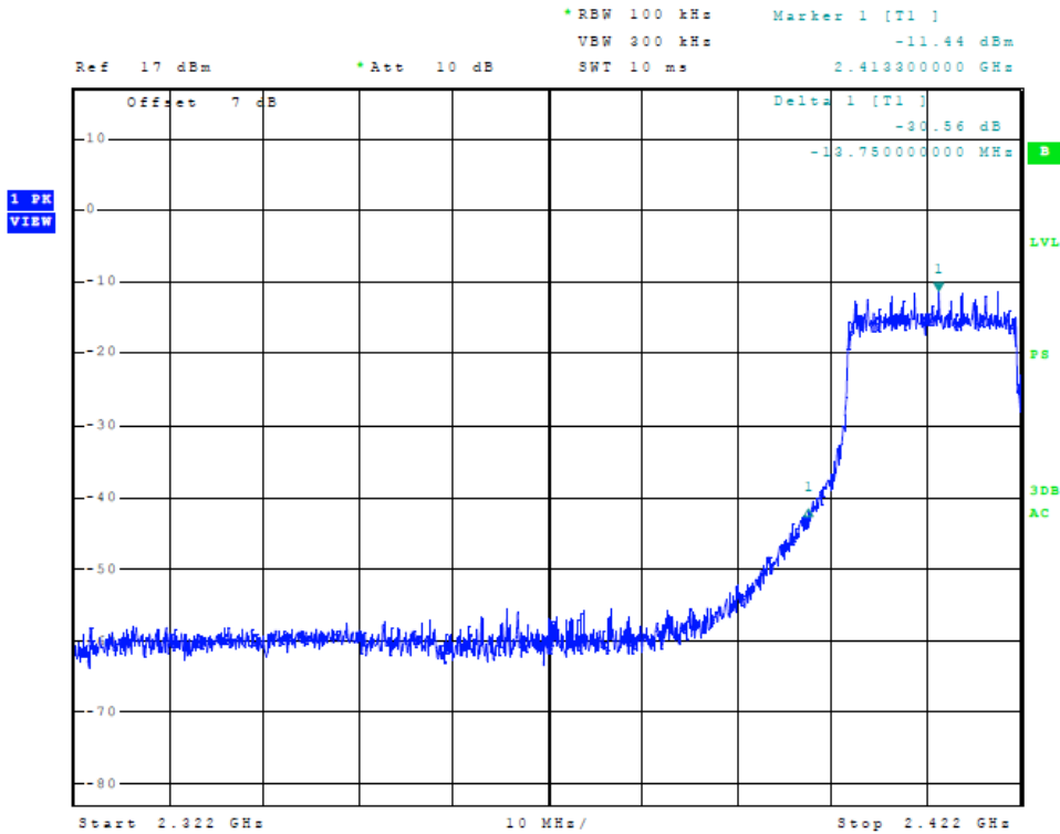
Figure 26 Plot of Transmitter Low Band Edge (802.11n (40), Chain 1)
