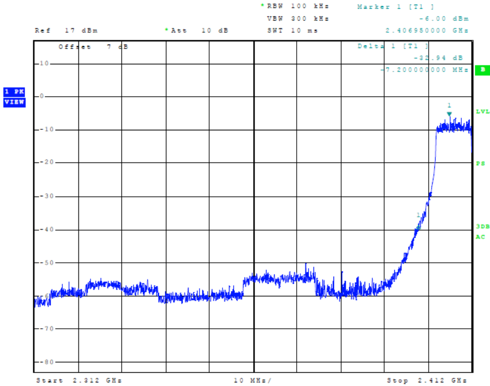
Figure 25 Plot of Transmitter Low Band Edge (802.11n (20), Chain 1)
