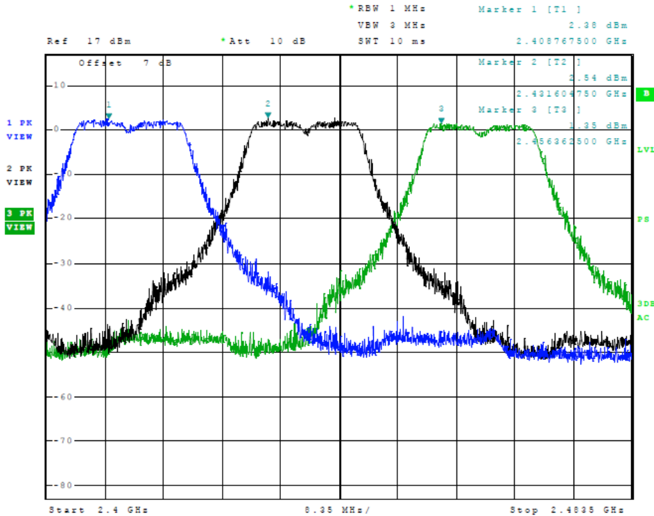
Figure 5 Plot of Transmitter Emissions (Across Operational Band, 802.11n (20), Chain 0)
