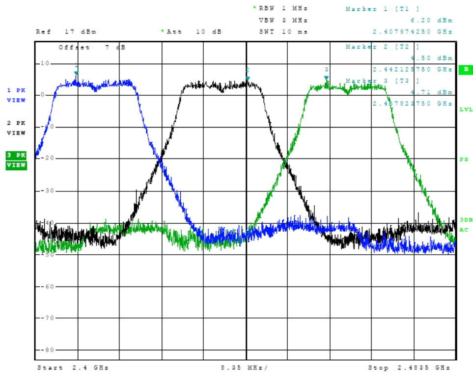
Figure 21 Plot of Transmitter Emissions (Across Operational Band, 802.11n (20), Chain 1)
