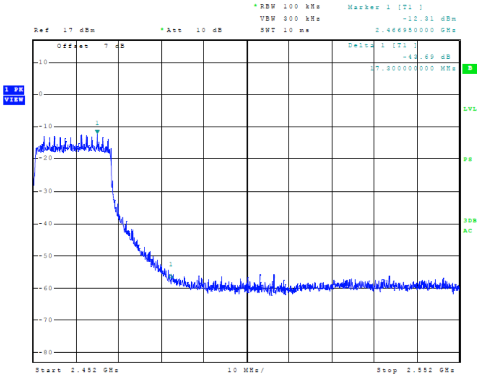
Figure 30 Plot of Transmitter High Band Edge (802.11n (40), Chain 1)
