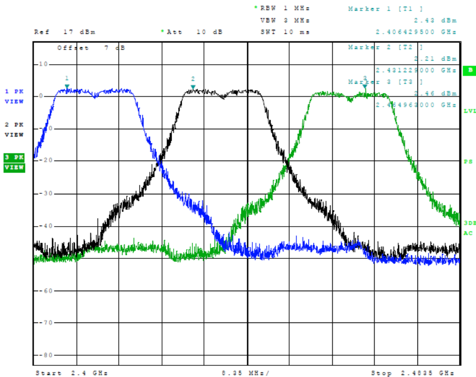
Figure 4 Plot of Transmitter Emissions (Across Operational Band, 802.11g, Chain 0)
