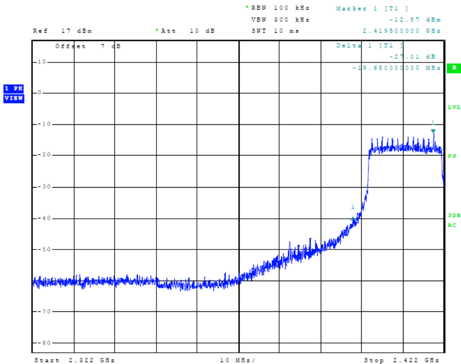
Figure 10 Plot of Transmitter Low Band Edge (802.11n (40), Chain 0)
