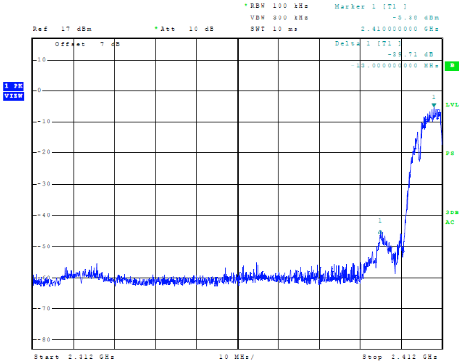
Figure 7 Plot of Transmitter Low Band Edge (802.11b, Chain 0)
