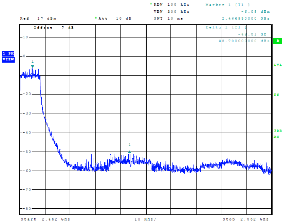
Figure 28 Plot of Transmitter High Band Edge (802.11g, Chain 1)
