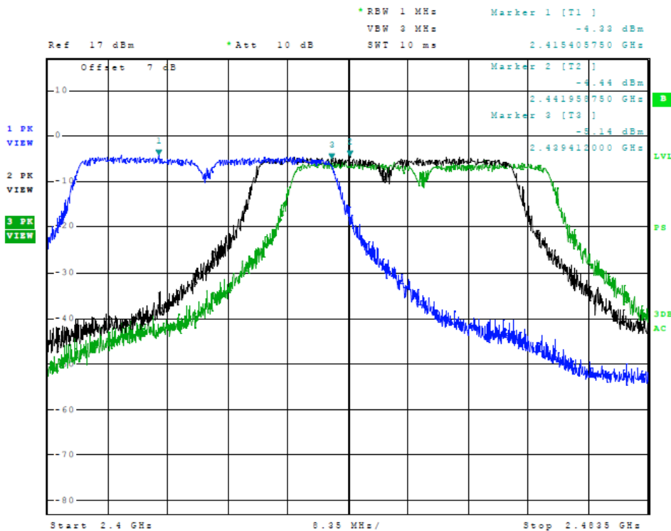
Figure 6 Plot of Transmitter Emissions (Across Operational Band, 802.11n (40), Chain 0)
