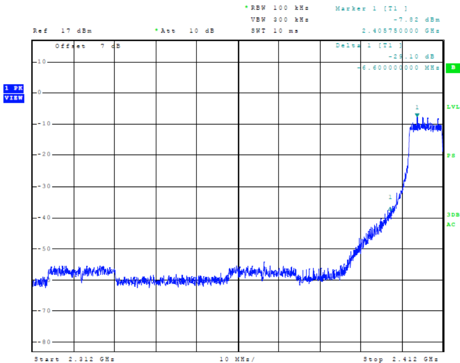
Figure 8 Plot of Transmitter Low Band Edge (802.11g, Chain 0)
