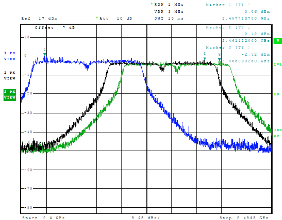
Figure 22 Plot of Transmitter Emissions (Across Operational Band, 802.11n (40), Chain 1)
