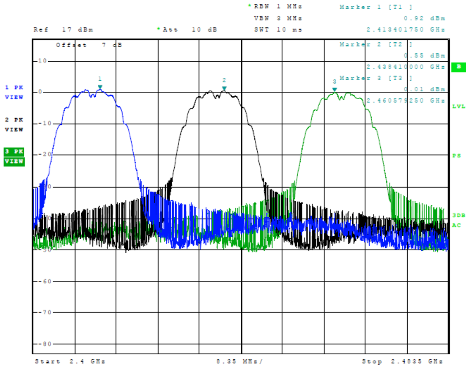
Figure 19 Plot of Transmitter Emissions (Across Operational Band 802.11b, Chain 1)
