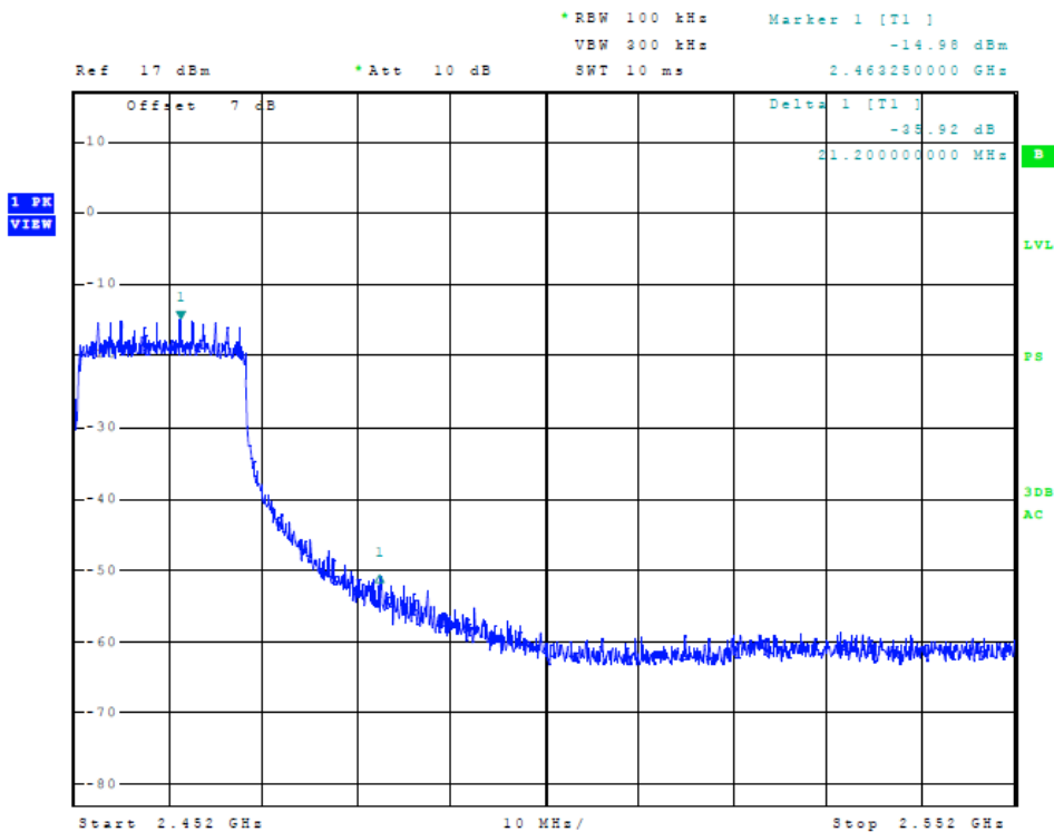
Figure 14 Plot of Transmitter High Band Edge (802.11n (40), Chain 0)
