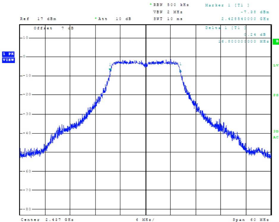
Figure 16 Plot of Transmitter 6-dB Occupied Band Width (802.11g, Chain 0)
