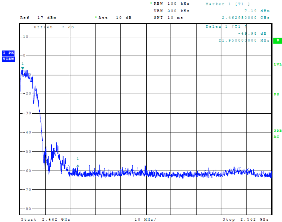
Figure 11 Plot of Transmitter High Band Edge (802.11b, Chain 0)
