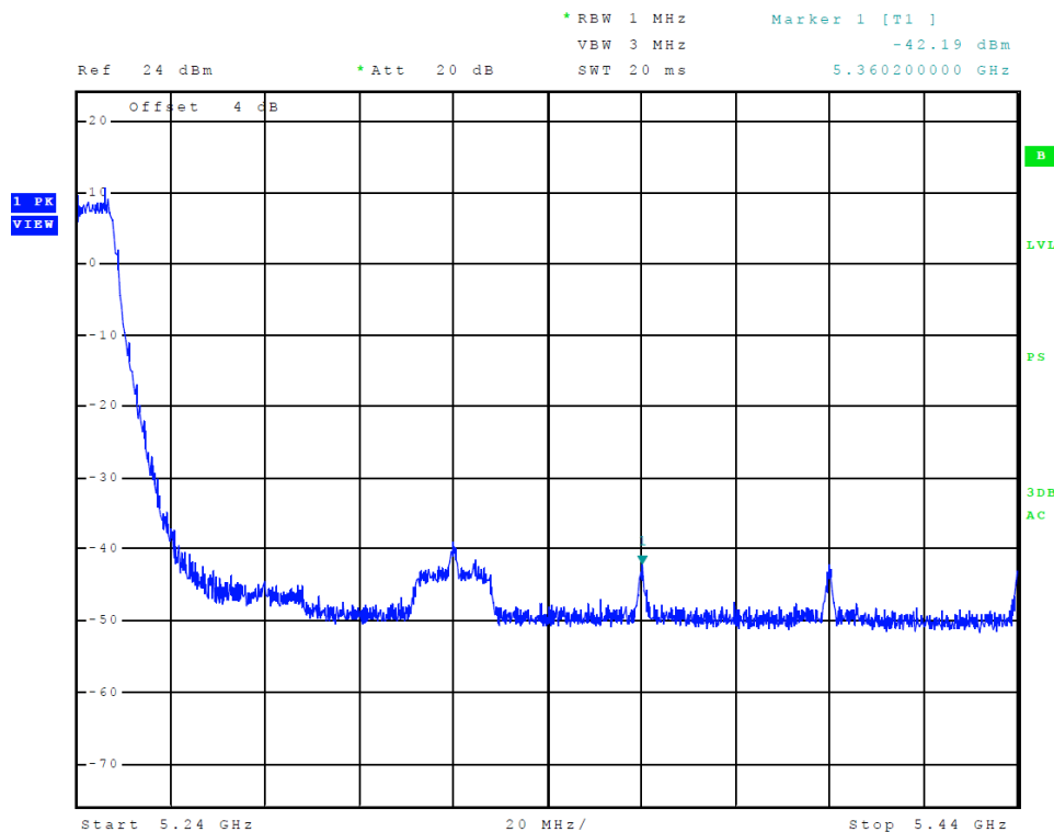
Figure 12 Plot of Transmitter High Band Edge (Chain 1, 5150-5250 MHz Band, 802.11a)
