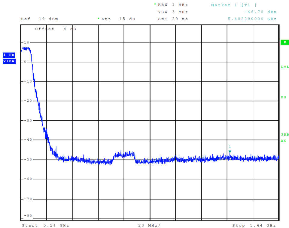
Figure 11 Plot of Transmitter High Band Edge (Chain 0, 5150-5250 MHz Band, 802.11a)
