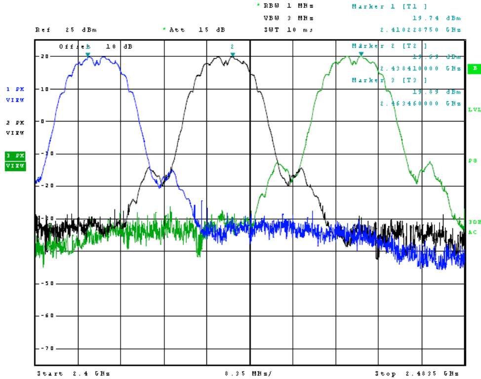
Figure 3 Plot of Transmitter Emissions (Across Operational Band, 2.4 GHz b/g/n)
