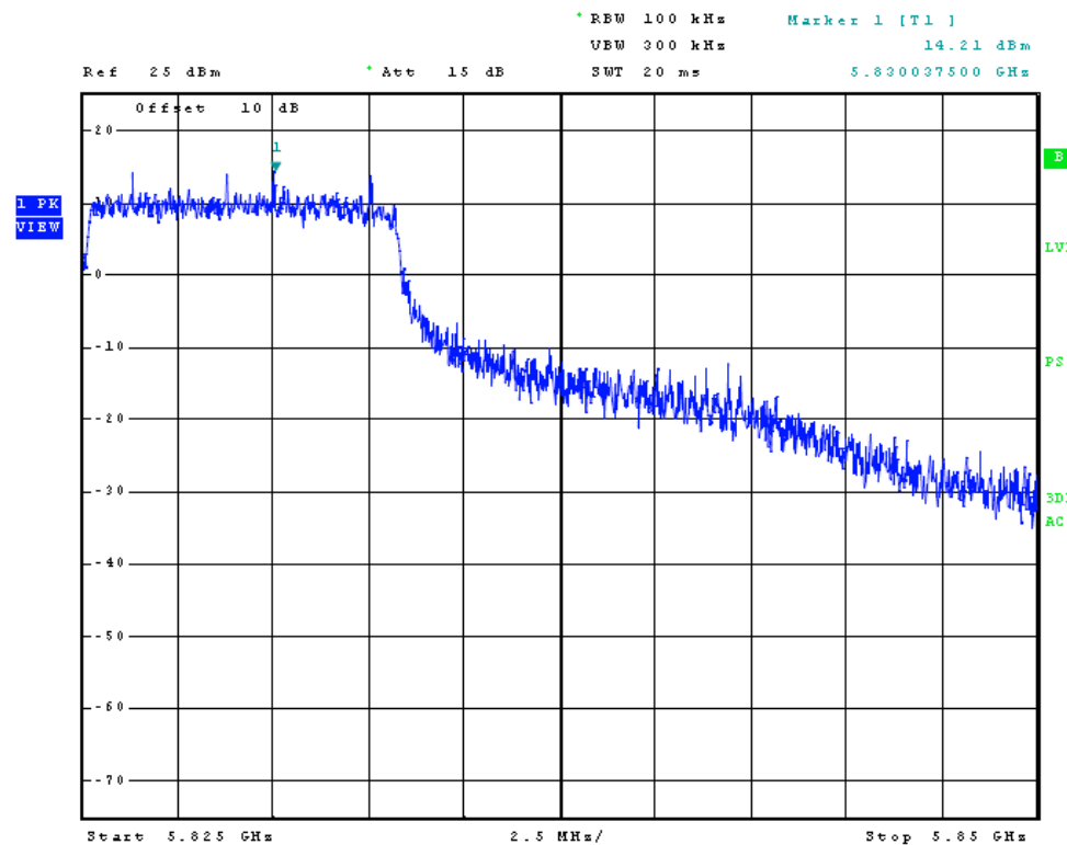
Figure 8 Plot of High Band Edge (5 GHz a/n)
