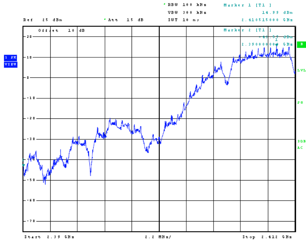
Figure 4 Plot of Low Band Edge (2.4 GHz b/g/n Mode)
