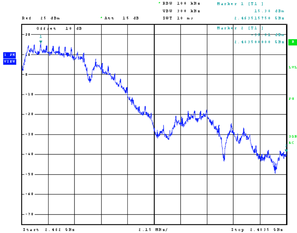
Figure 5 Plot of High Band Edge (2.4 GHz b/g/n Mode)
