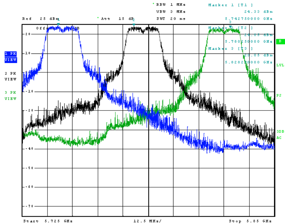
Figure 6 Plot of Transmitter Emissions (Across Operational Band, 5 GHz a/n)
