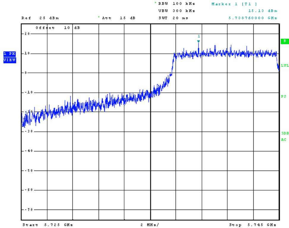
Figure 7 Plot of Low Band Edge (5 GHz a/n)
