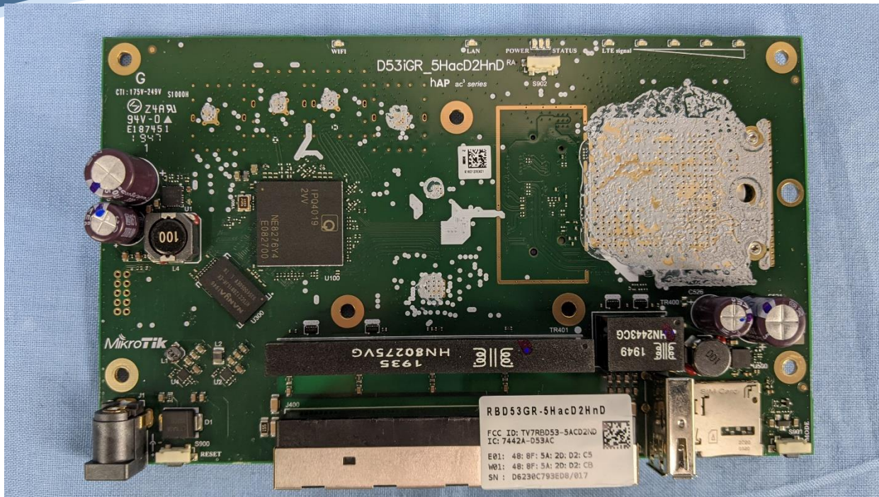
Main Board Bottom Heatsink Removed
