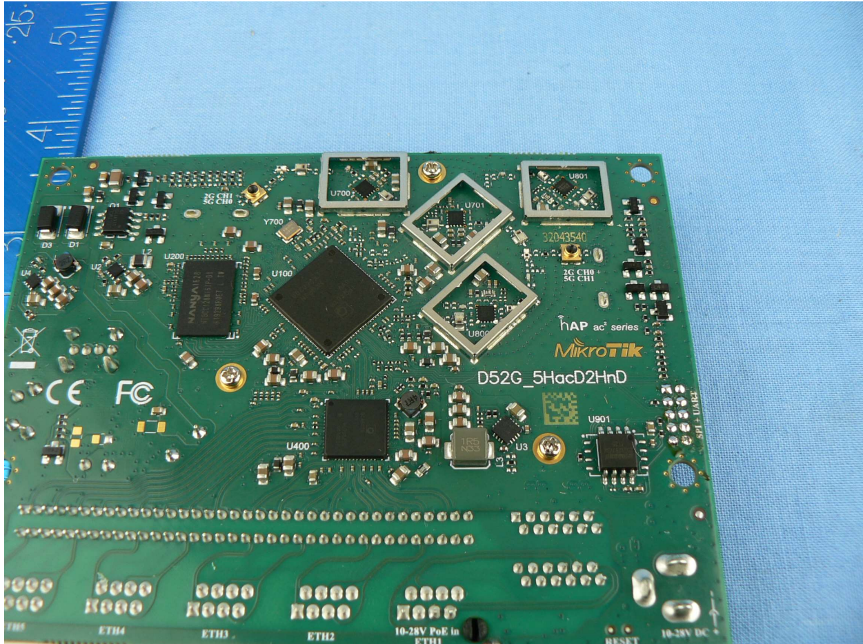
Module - Bottom Side - Cans Removed
