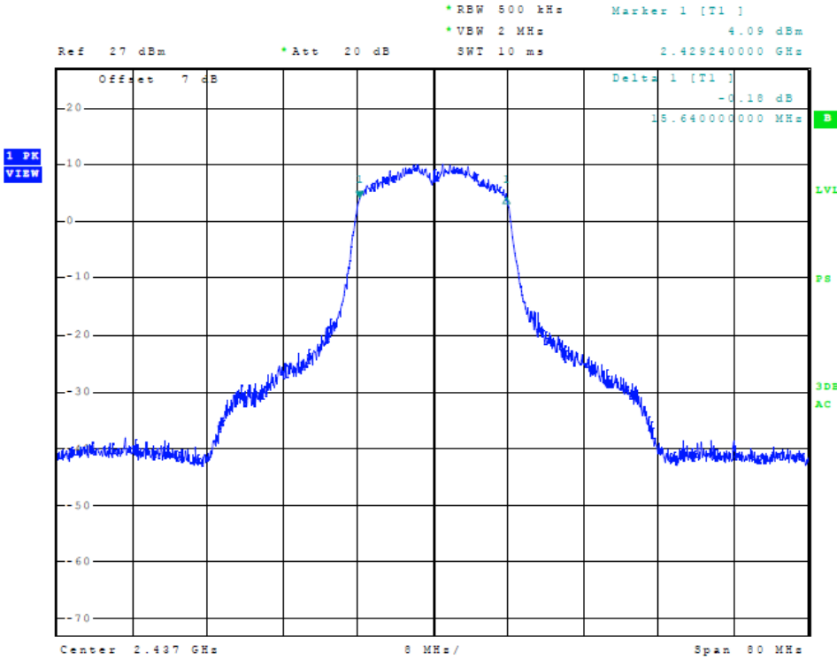
Figure 17 Plot of Transmitter 6-dB Occupied Band Width (802.11n (20), Chain 0)
