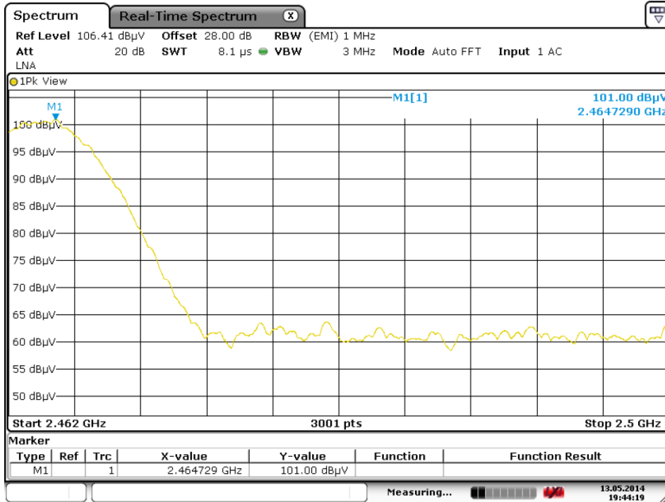
Figure 7 Plot of Transmitter High Band Edge (20 MHz Channel)
