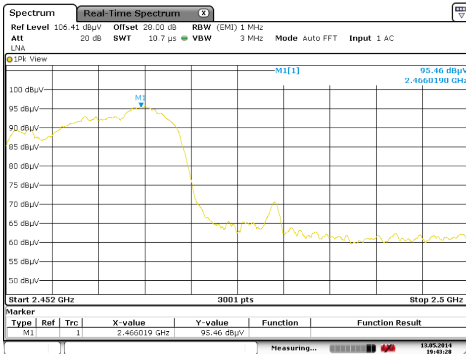
Figure 8 Plot of Transmitter High Band Edge (40 MHz Channel)
