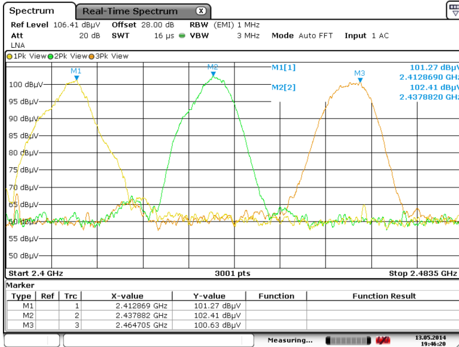
Figure 3 Plot of Transmitter Emissions (Across Operational Band, 20 MHz Channel)
