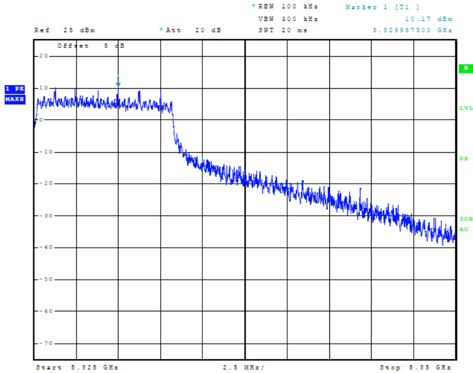
Figure 7 Plot of Transmitter High Band Edge (20 MHz Channel)
