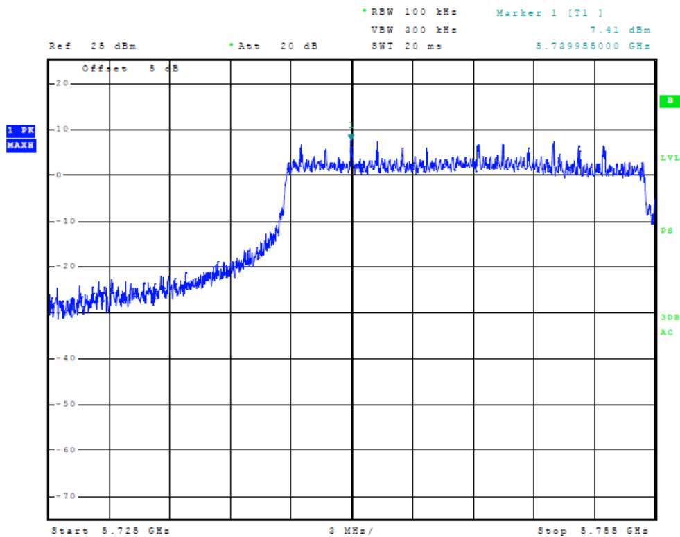
Figure 6 Plot of Transmitter Low Band Edge (40 MHz Channel)
