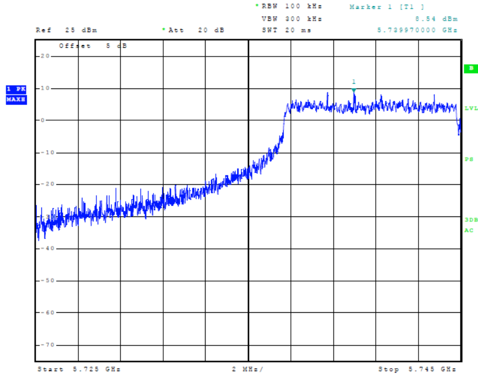
Figure 5 Plot of Transmitter Low Band Edge (20 MHz Channel)
