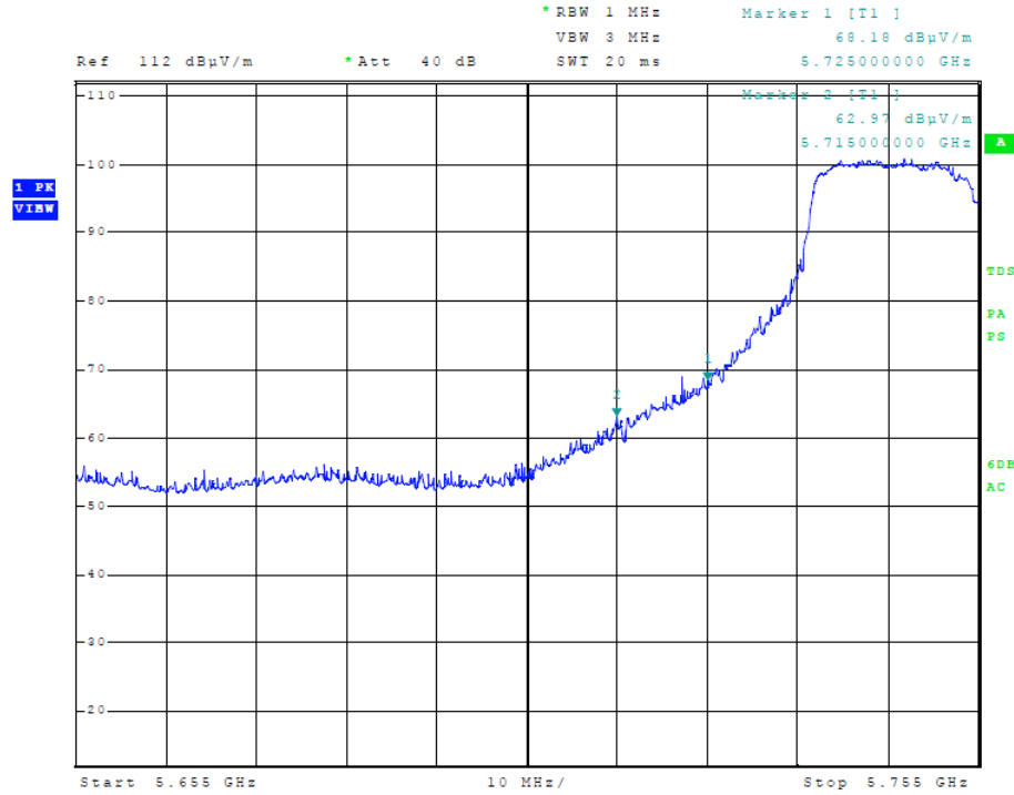
Figure 19 Plot of Transmitter Low Band Edge (5725-5850 MHz Band, 40 MHz Channel)
