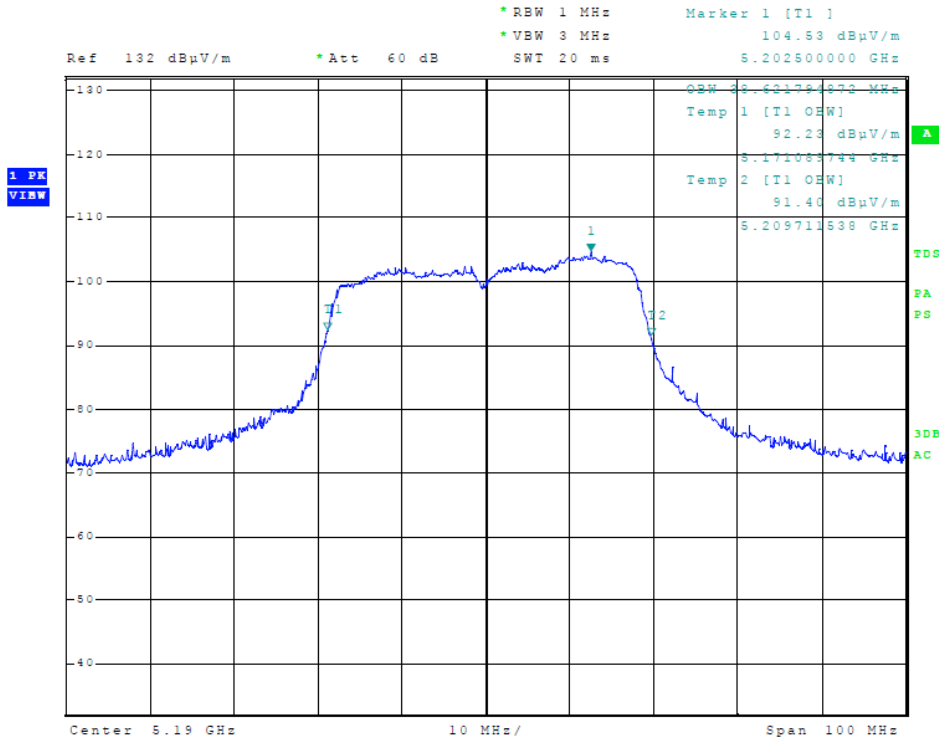
Figure 13 Plot of Transmitter Emissions (5150-5250 MHz Band, 40 MHz Channel, 99% OBW)
