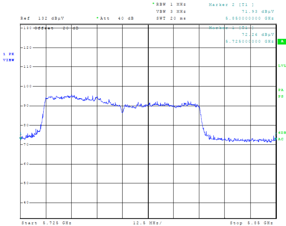
Figure 17 Plot of Transmitter Emissions (Across 5725-5850 MHz Band, 80 MHz Channel)
