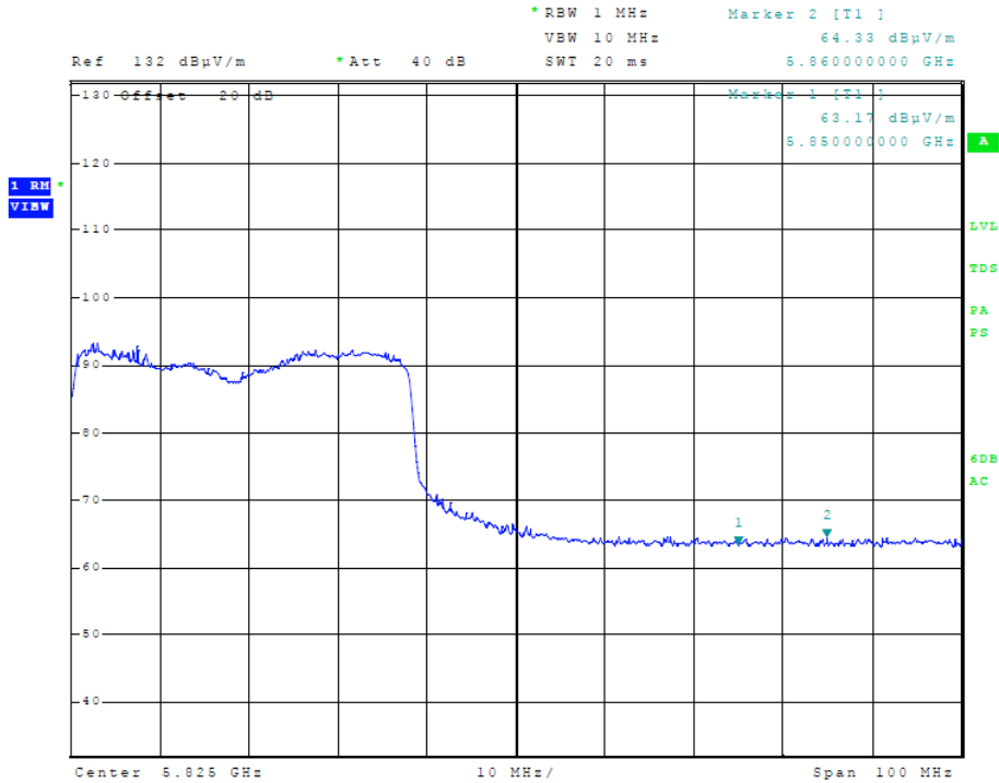
Figure 23 Plot of Transmitter High Band Edge (5725-5850 MHz Band, 80 MHz Channel)
