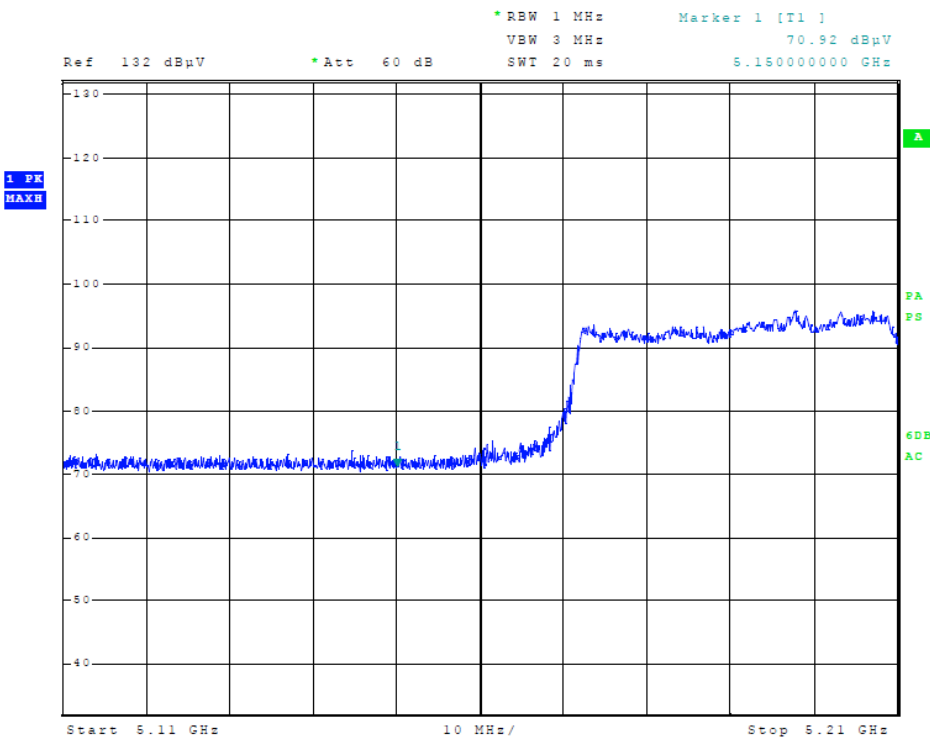
Figure 8 Plot of Transmitter Low Band Edge (5150-5250 MHz Band, 80 MHz Channel)
