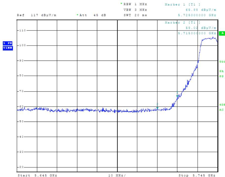
Figure 18 Plot of Transmitter Low Band Edge (5725-5850 MHz Band, 20 MHz Channel)
