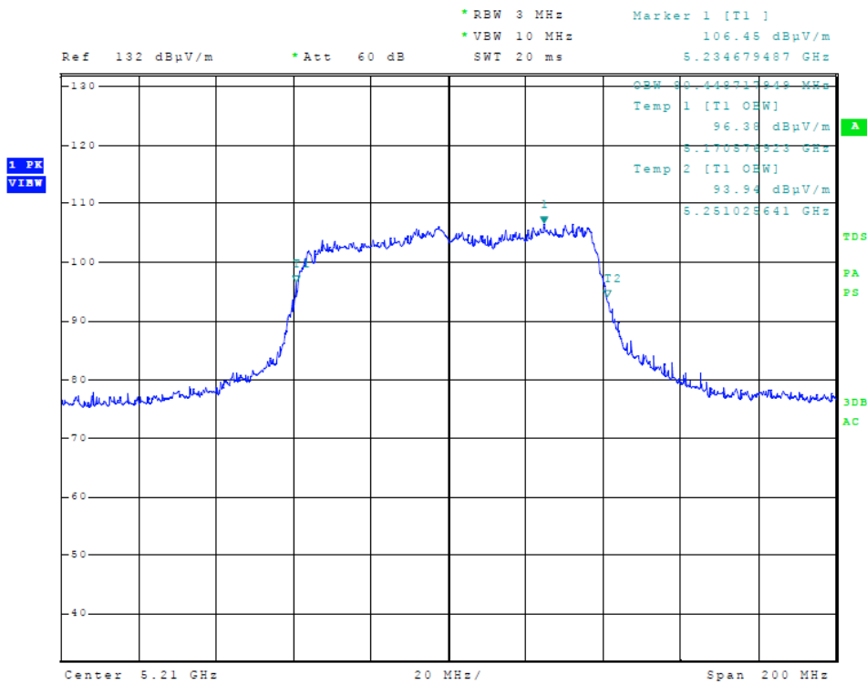
Figure 14 Plot of Transmitter Emissions (5150-5250 MHz Band, 80 MHz Channel, 99% OBW)
