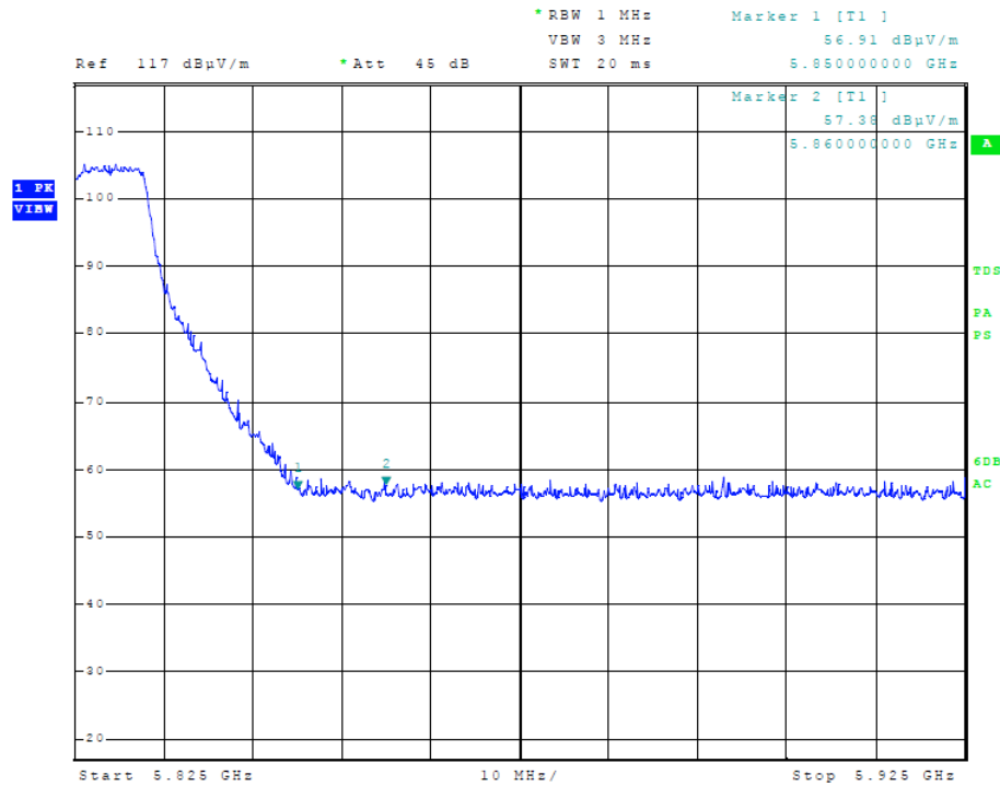
Figure 21 Plot of Transmitter High Band Edge (5725-5850 MHz Band, 20 MHz Channel)
