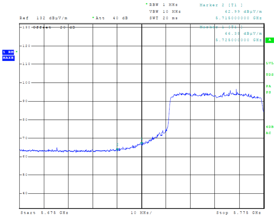
Figure 20 Plot of Transmitter Low Band Edge (5725-5850 MHz Band, 80 MHz Channel)
