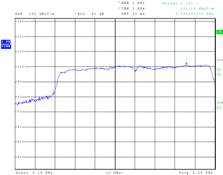
Figure 5 Plot of Transmitter Emissions (Across 5150-5250 MHz Band, 80 MHz Channel)
