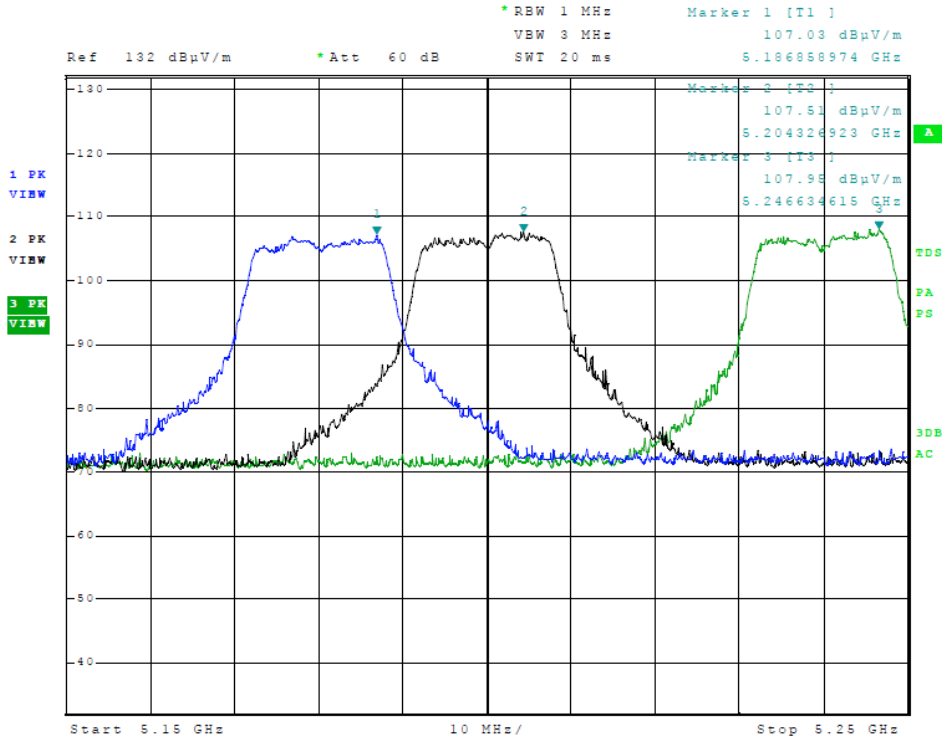
Figure 3 Plot of Transmitter Emissions (Across 5150-5250 MHz Band, 20 MHz Channel)
