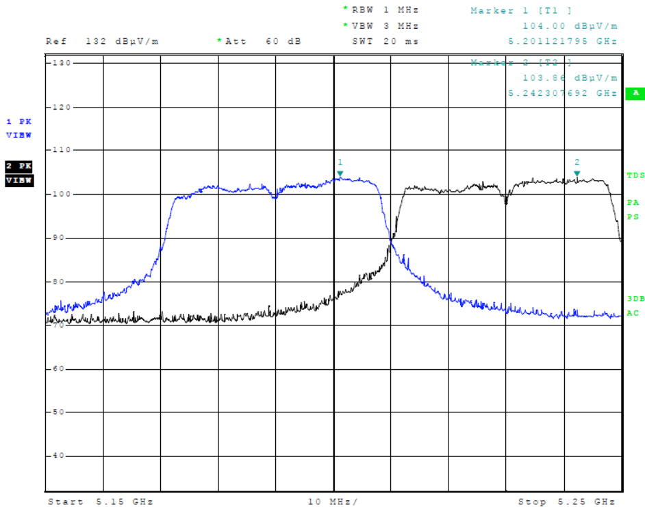
Figure 4 Plot of Transmitter Emissions (Across 5150-5250 MHz Band, 40 MHz Channel)
