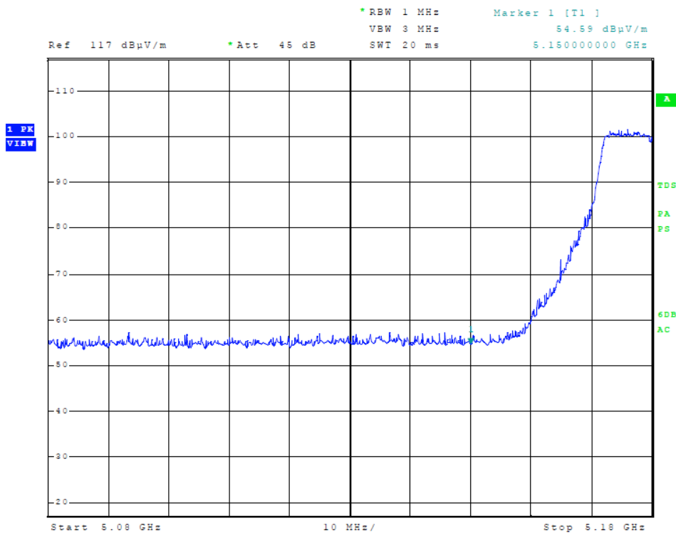
Figure 6 Plot of Transmitter Low Band Edge (5150-5250 MHz Band, 20 MHz Channel)
