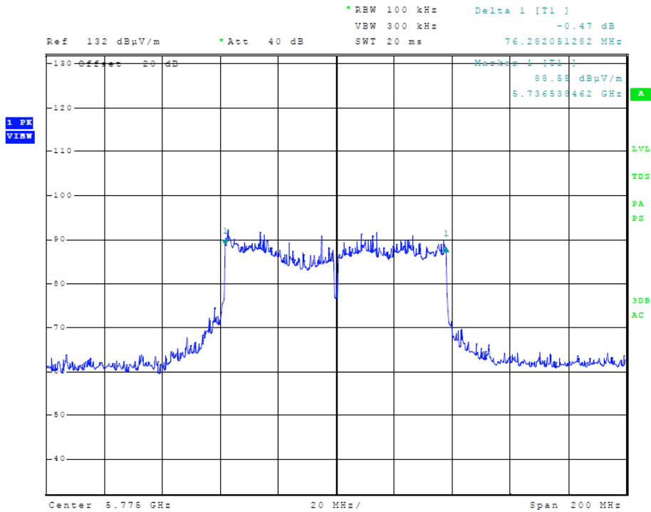
Figure 29 Plot of Transmitter Emissions (5725-5850 MHz Band, 80 MHz Channel, 6-dB OBW)
