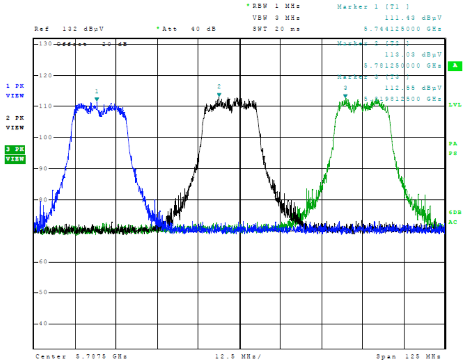
Figure 15 Plot of Transmitter Emissions (Across 5725-5850 MHz Band, 20 MHz Channel)
