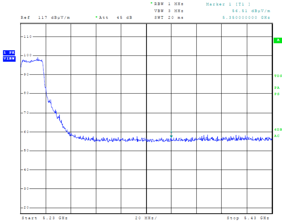
Figure 9 Plot of Transmitter High Band Edge (5150-5250 MHz Band, 20 MHz Channel)
