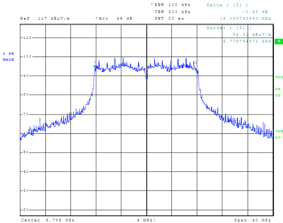
Figure 27 Plot of Transmitter Emissions (5725-5850 MHz Band, 20 MHz Channel, 6-dB OBW)
