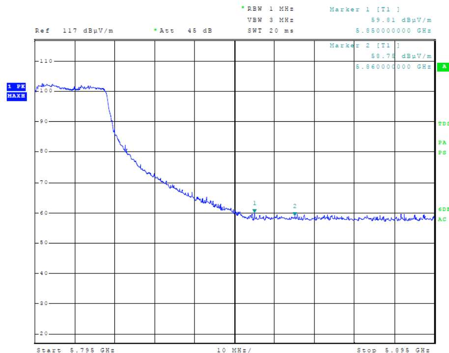
Figure 22 Plot of Transmitter High Band Edge (5725-5850 MHz Band, 40 MHz Channel)
