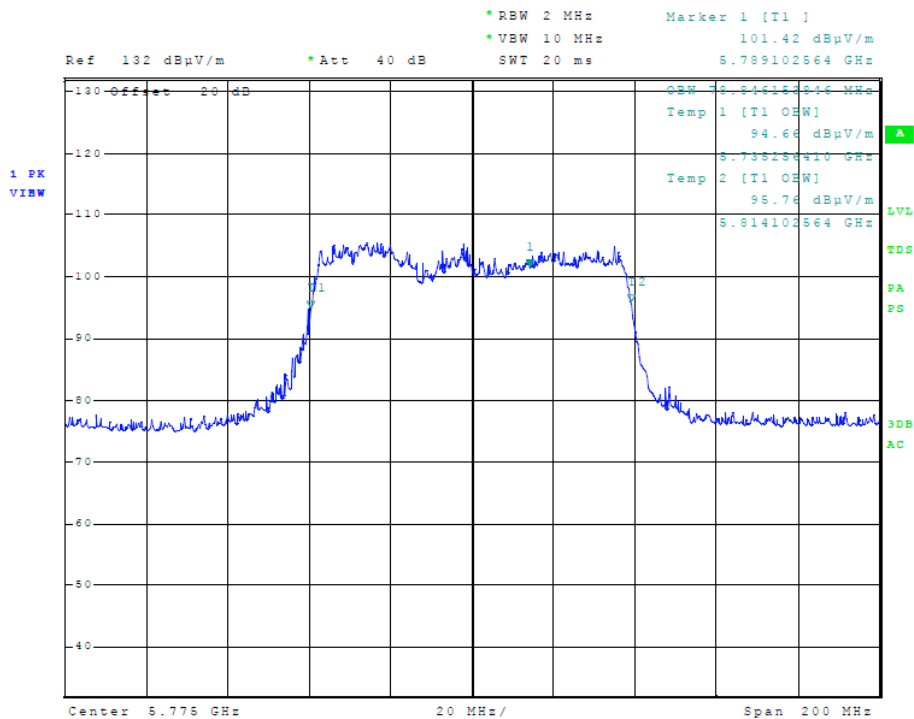
Figure 26 Plot of Transmitter Emissions (5725-5850 MHz Band, 80 MHz Channel, 99% OBW)
