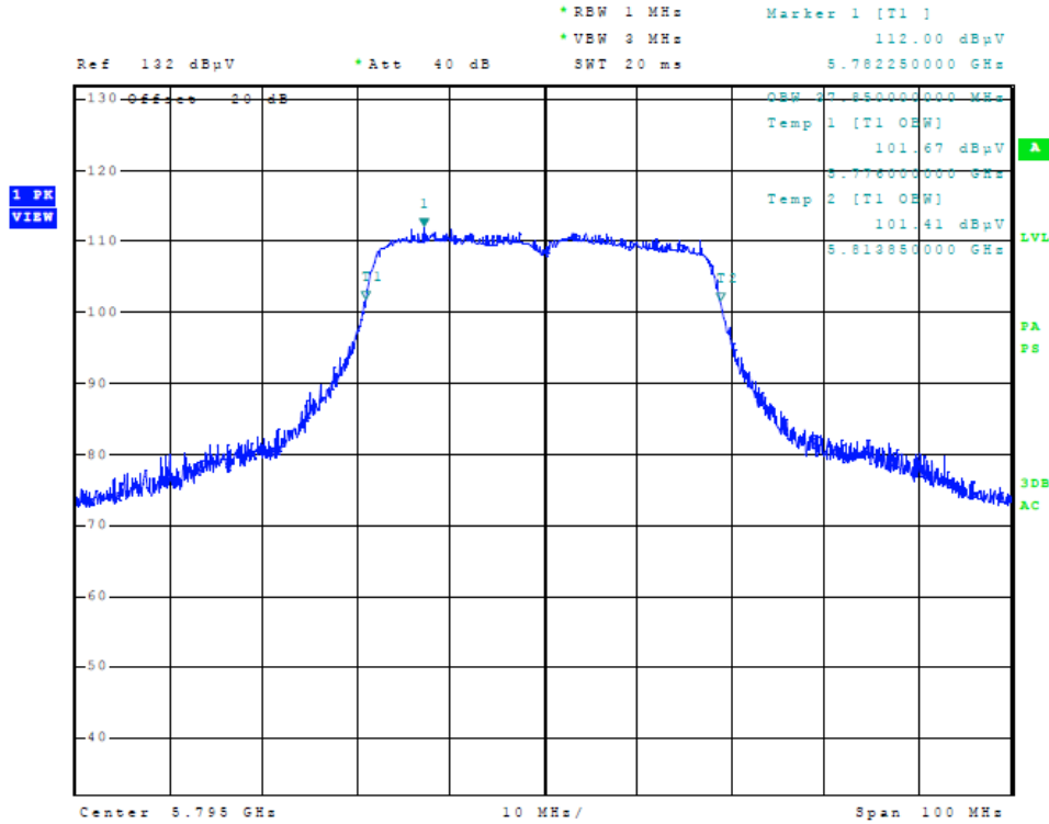
Figure 25 Plot of Transmitter Emissions (5725-5850 MHz Band, 40 MHz Channel, 99% OBW)
