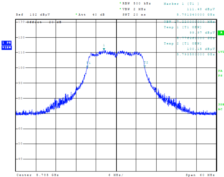
Figure 24 Plot of Transmitter Emissions (5725-5850 MHz Band, 20 MHz Channel, 99% OBW)
