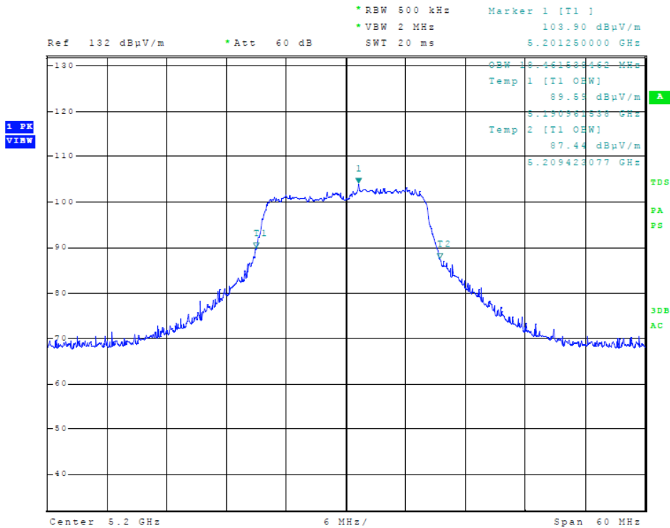
Figure 12 Plot of Transmitter Emissions (5150-5250 MHz Band, 20 MHz Channel, 99% OBW)
