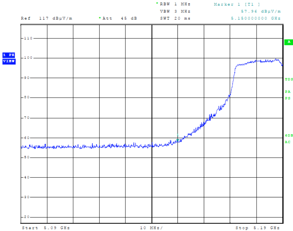
Figure 7 Plot of Transmitter Low Band Edge (5150-5250 MHz Band, 40 MHz Channel)
