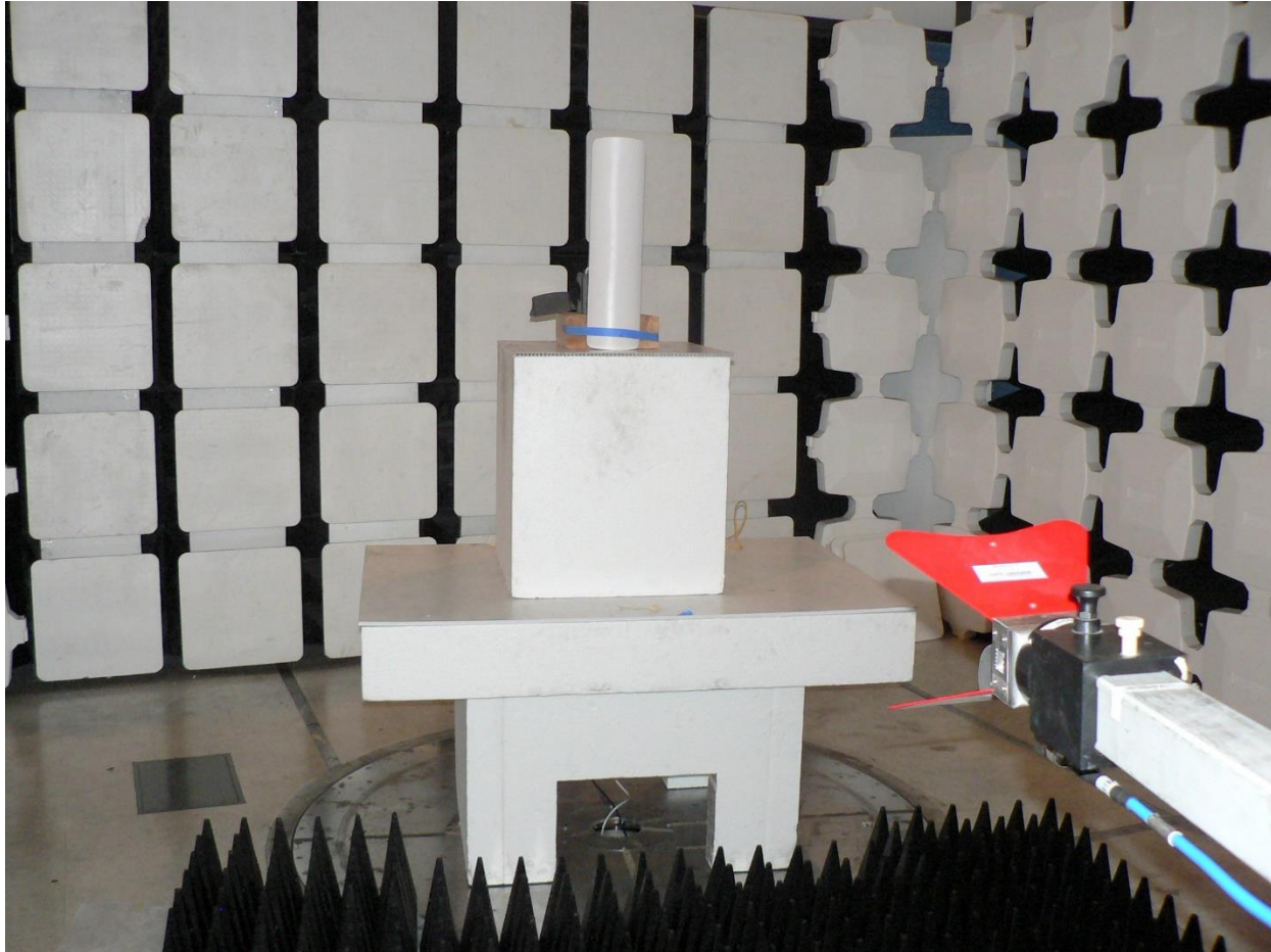
19 dBi antenna TX Spurious
