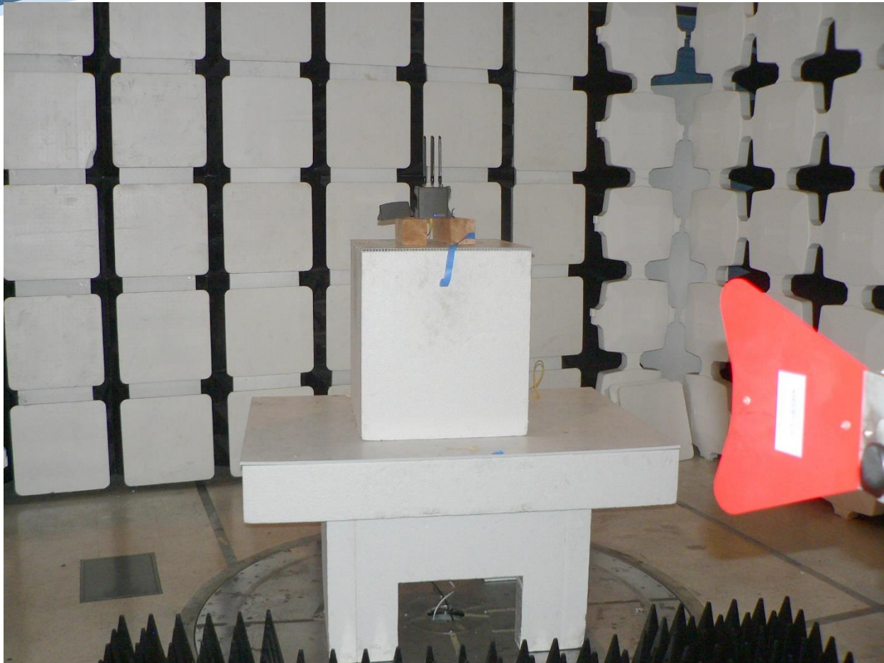
7 dBi antenna TX Spurious
