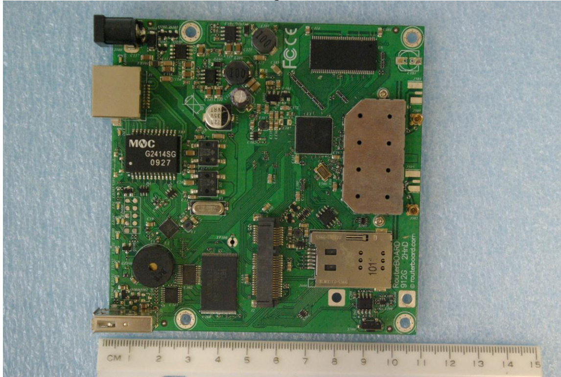
Printed Circuit Board (PCB) with shield in place
