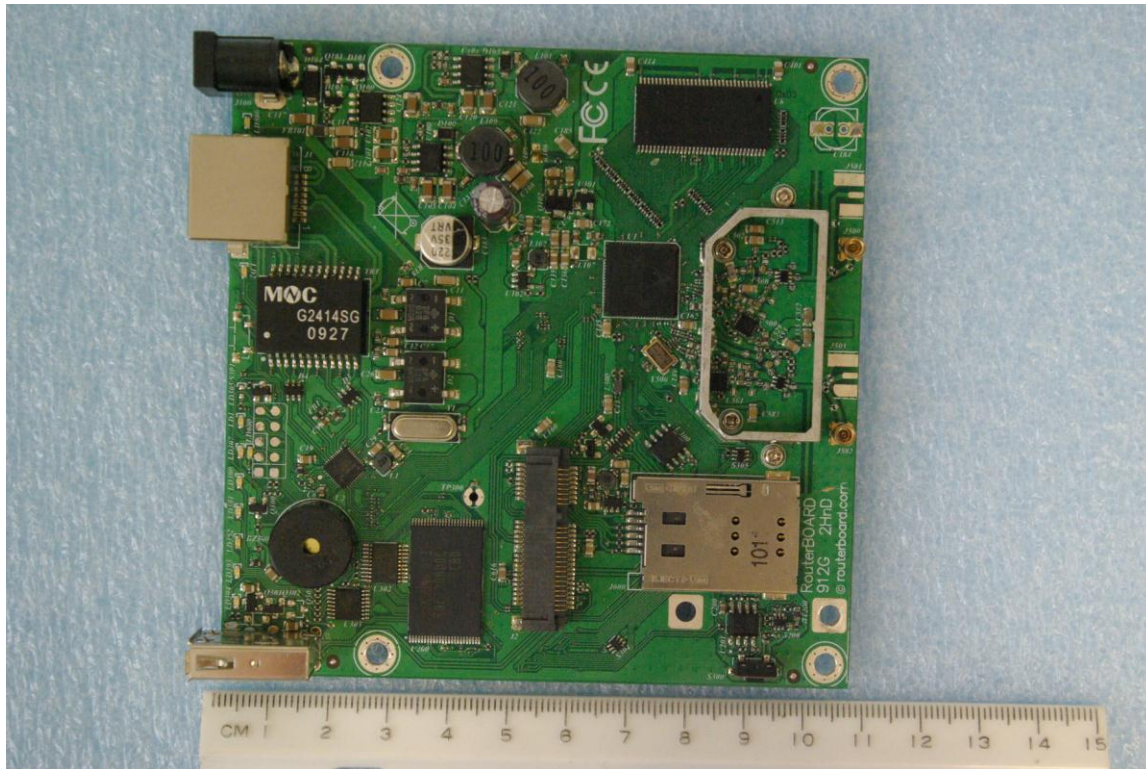
PCB Shield removed
