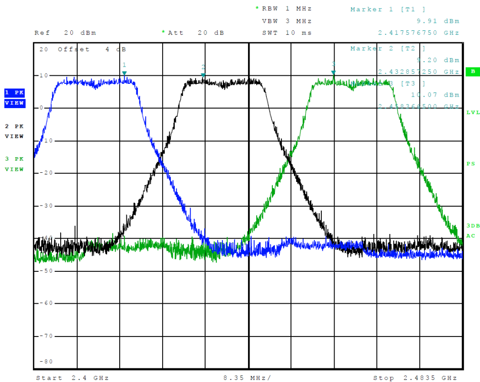
Figure 10 Plot of Transmitter Emissions (Across Operational Band, 802.11n (20), Chain 1)
