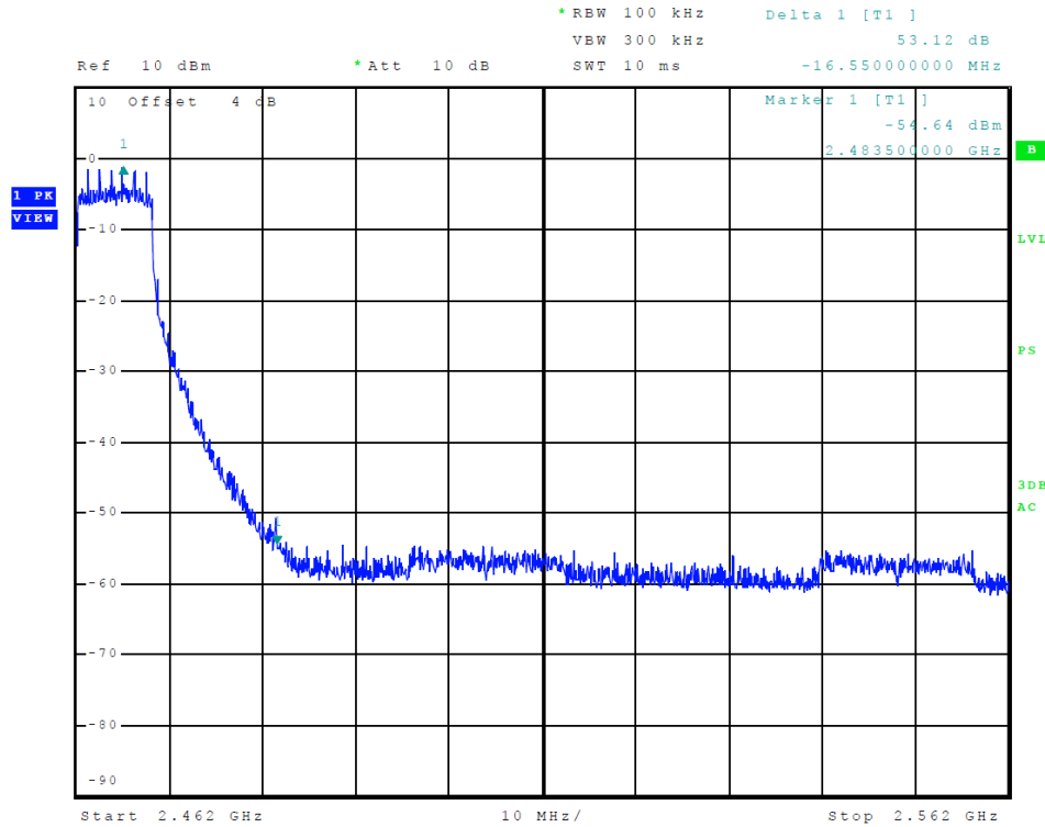
Figure 25 Plot of Transmitter High Band Edge (802.11n (20), Chain 0)
