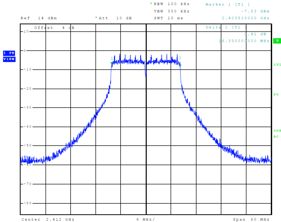
Figure 33 Plot of Transmitter 6-dB Occupied Band Width (802.11n (20), Chain 0)
