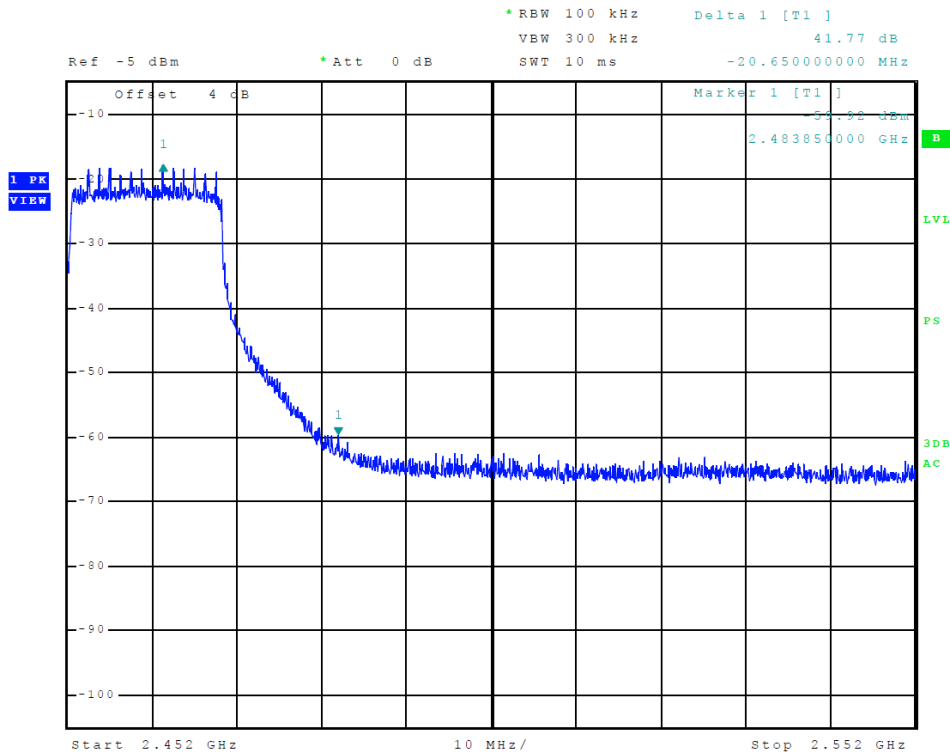
Figure 27 Plot of Transmitter High Band Edge (802.11n (40), Chain 0)
