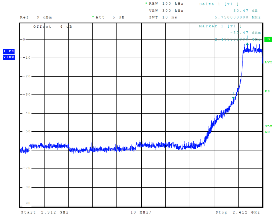
Figure 17 Plot of Transmitter Low Band Edge (802.11n (20), Chain 0)
