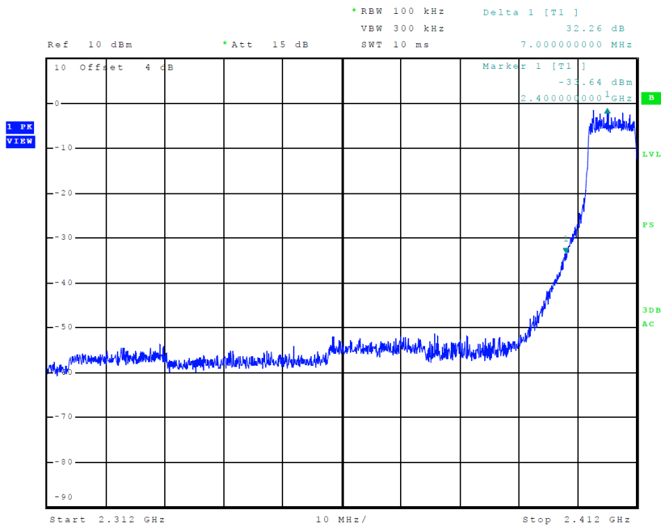
Figure 18 Plot of Transmitter Low Band Edge (802.11n (20), Chain 1)
