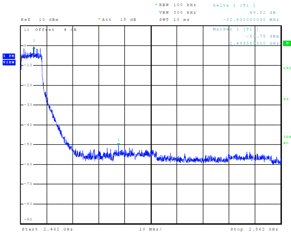
Figure 26 Plot of Transmitter High Band Edge (802.11n (20), Chain 1)
