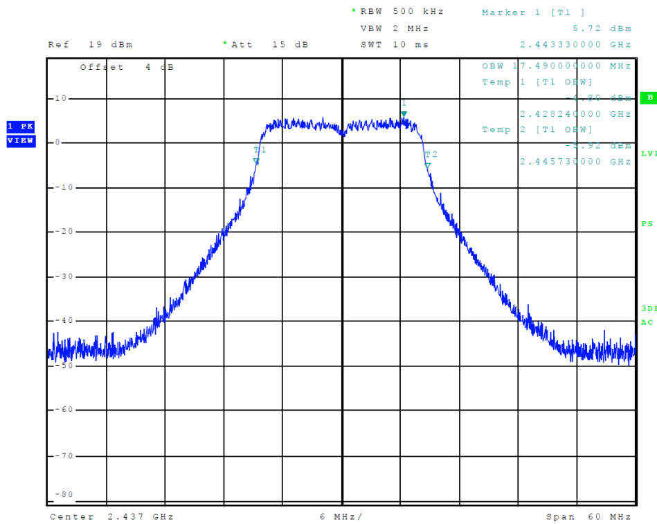
Figure 42 Plot of Transmitter 99% Occupied Band Width (802.11n (20), Chain 1)
