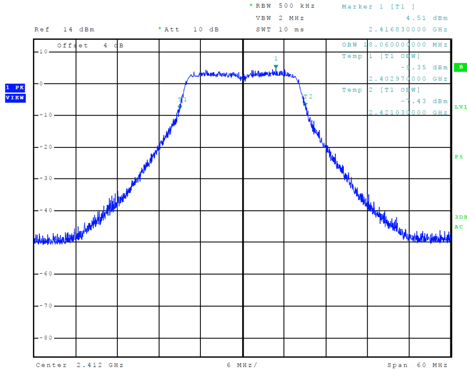
Figure 41 Plot of Transmitter 99% Occupied Band Width (802.11n (20), Chain 0)
