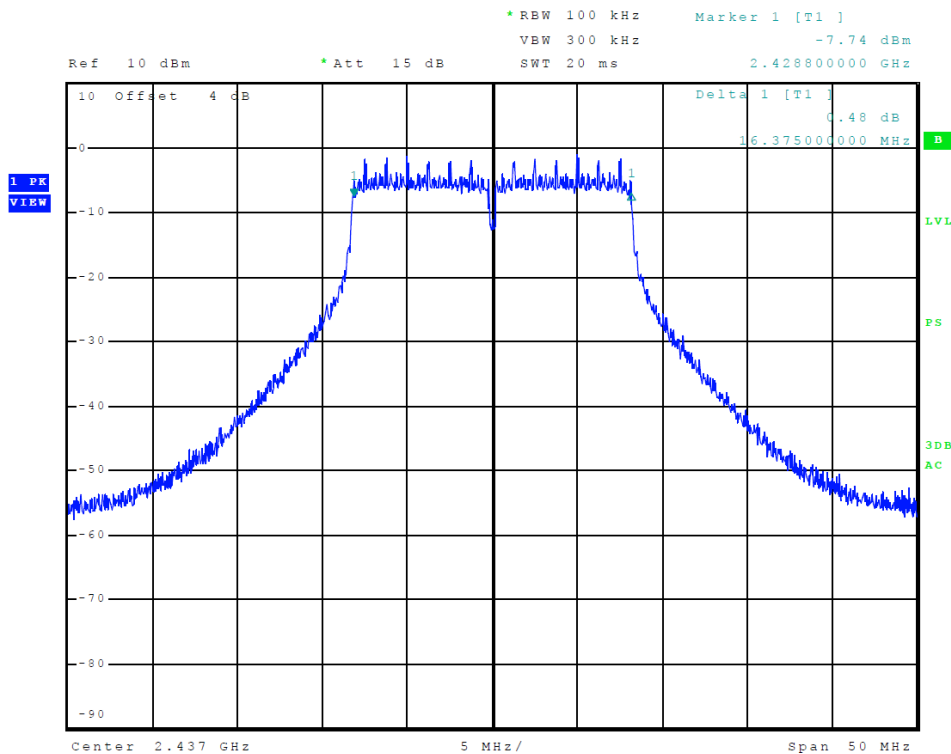
Figure 34 Plot of Transmitter 6-dB Occupied Band Width (802.11n (20), Chain 1)
