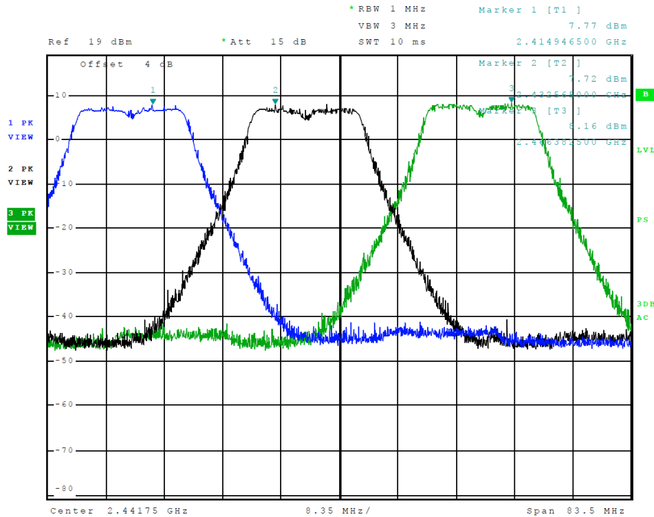
Figure 9 Plot of Transmitter Emissions (Across Operational Band, 802.11n (20), Chain 0)
