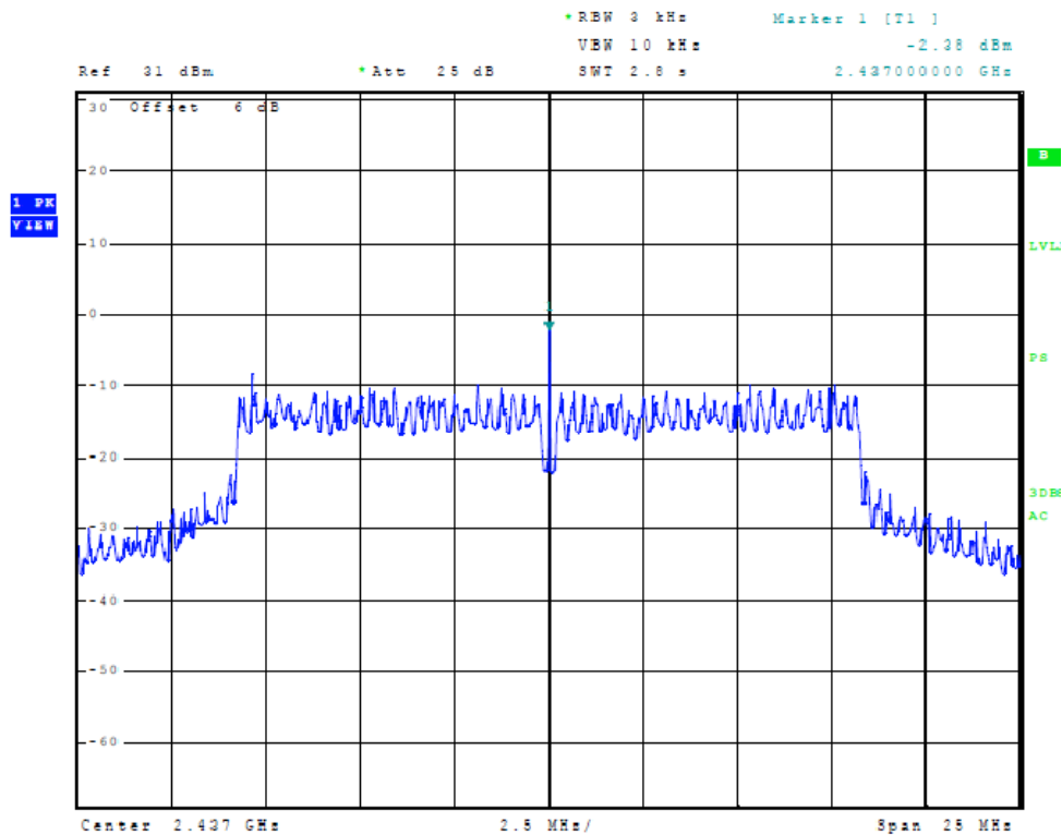
Figure 28 Plot of Power Spectral Density (20 MHz Mode, 2437 MHz)
