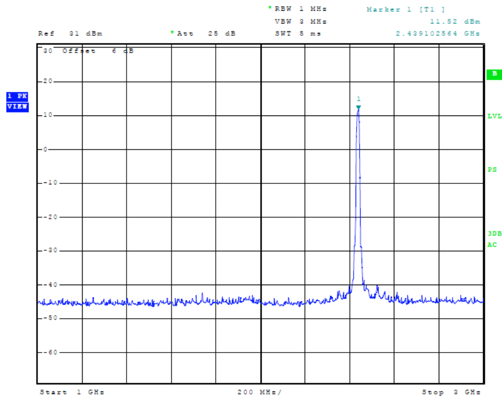
Figure 34 Plot of Antenna port conducted emissions
