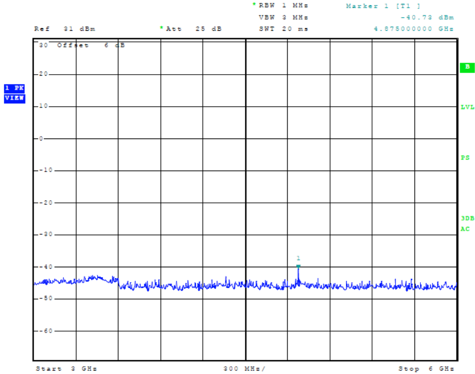
Figure 35 Plot of Antenna port conducted emissions
