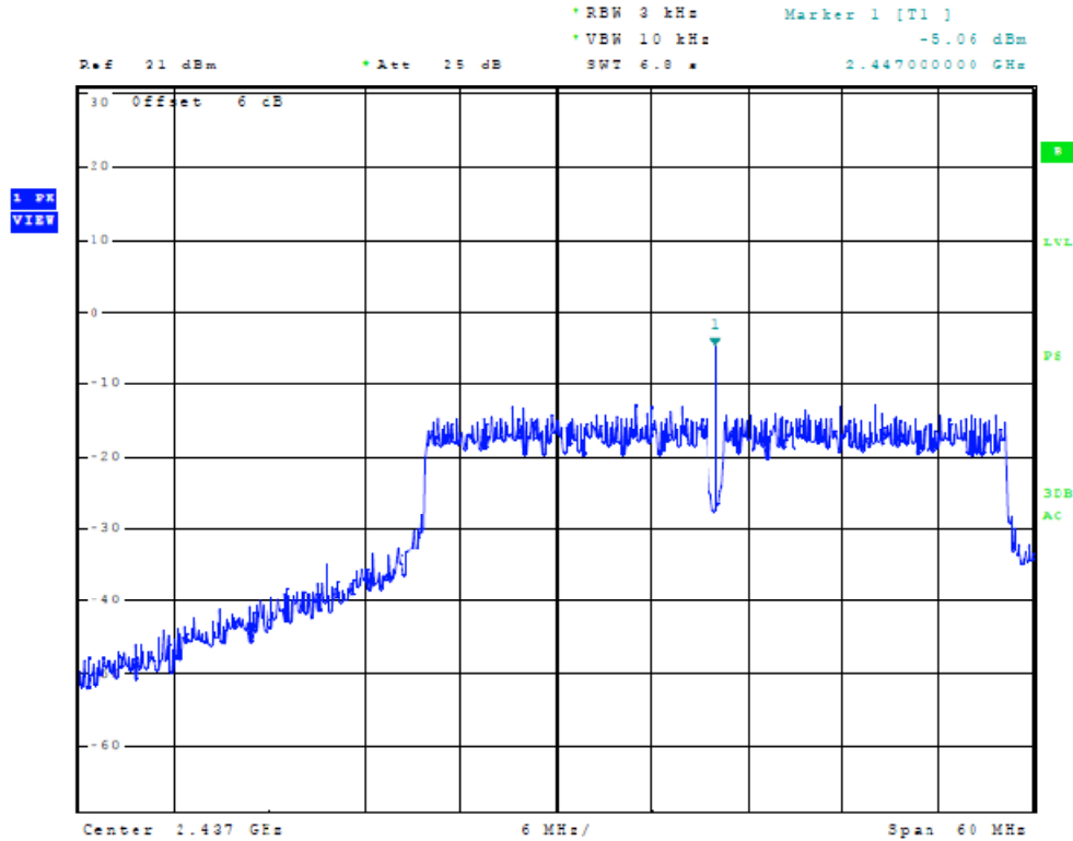
Figure 31 Plot of Power Spectral Density (40 MHz Mode, 2447 MHz)
