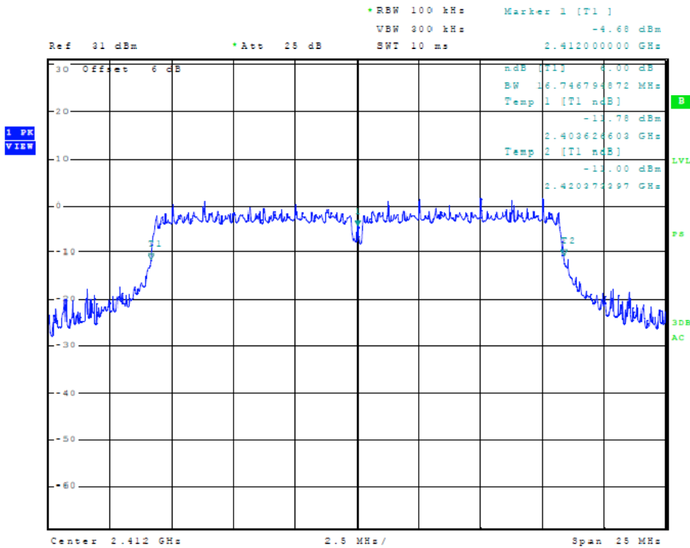
Figure 18 Plot of 6dB Band width (20 MHz Mode, 2412 MHz)
