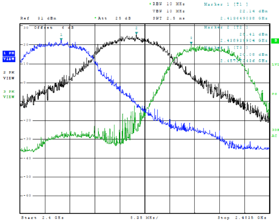
Figure 13 Plot of Antenna Port Emissions (Across Operational Band, 20MHz Mode)
