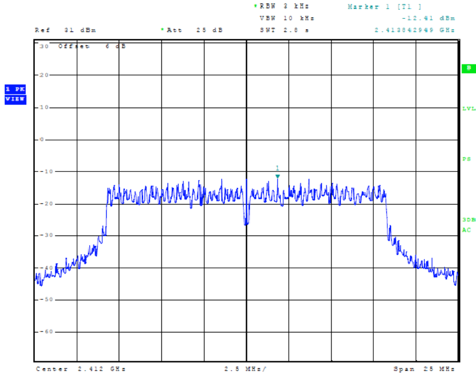
Figure 27 Plot of Power Spectral Density (20 MHz Mode, 2412 MHz)
