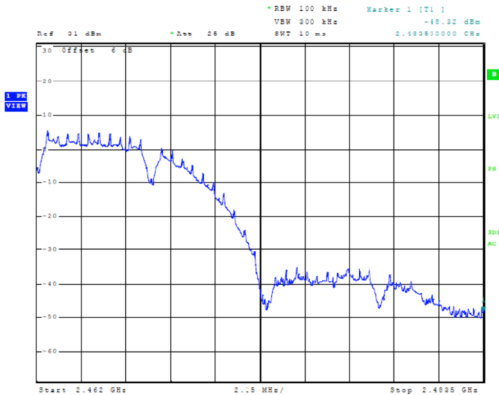
Figure 40 Plot of Band Edge Compliance at Antenna port (worst-case)
