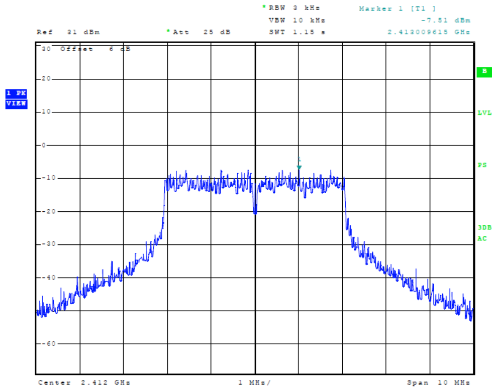
Figure 24 Plot of Power Spectral Density (5 MHz Mode, 2412 MHz)
