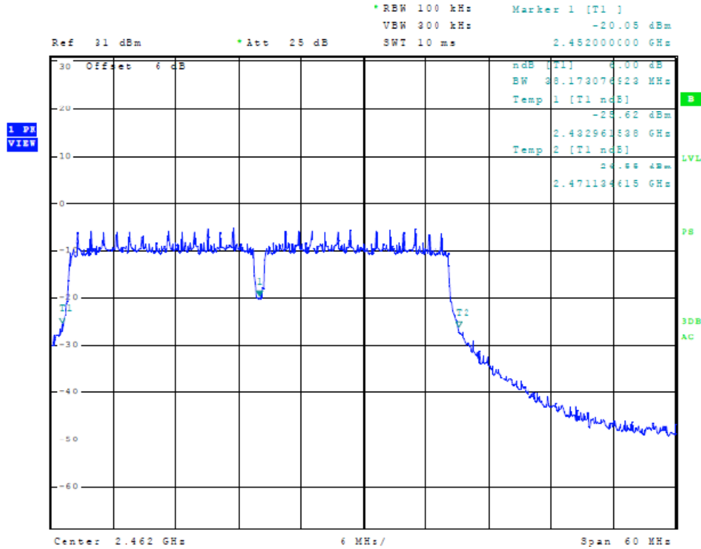
Figure 23 Plot of 6dB Band width (40 MHz Mode, 2452 MHz)
