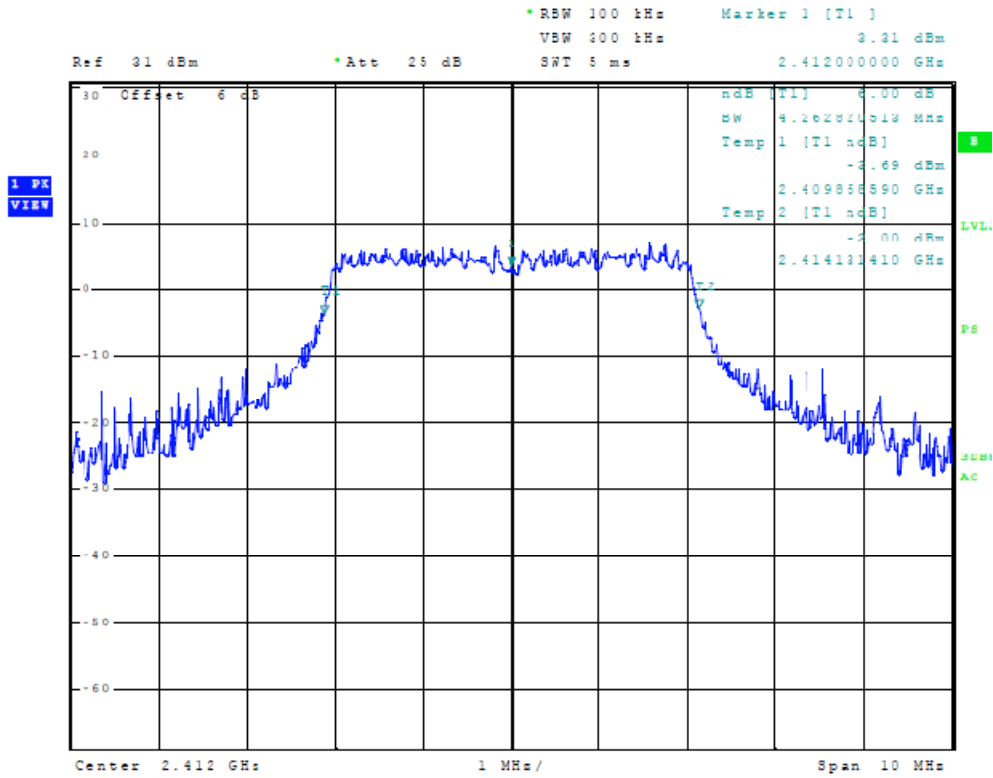
Figure 15 Plot of Plot of 6dB Band width (5 MHz Mode, 2412 MHz)
