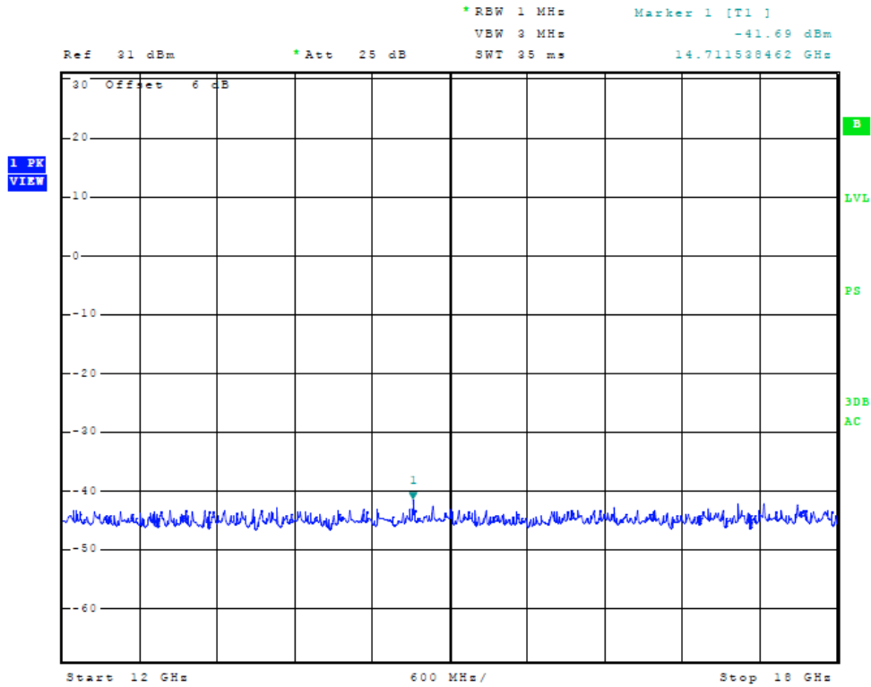
Figure 37 Plot of Antenna port conducted emissions
