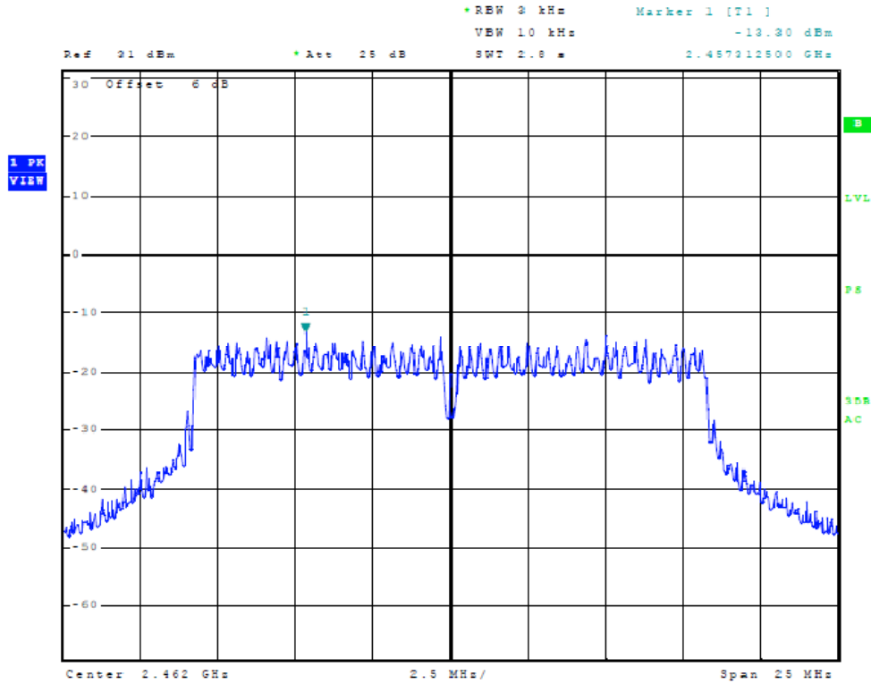
Figure 29 Plot of Power Spectral Density (20 MHz Mode, 2462 MHz)
