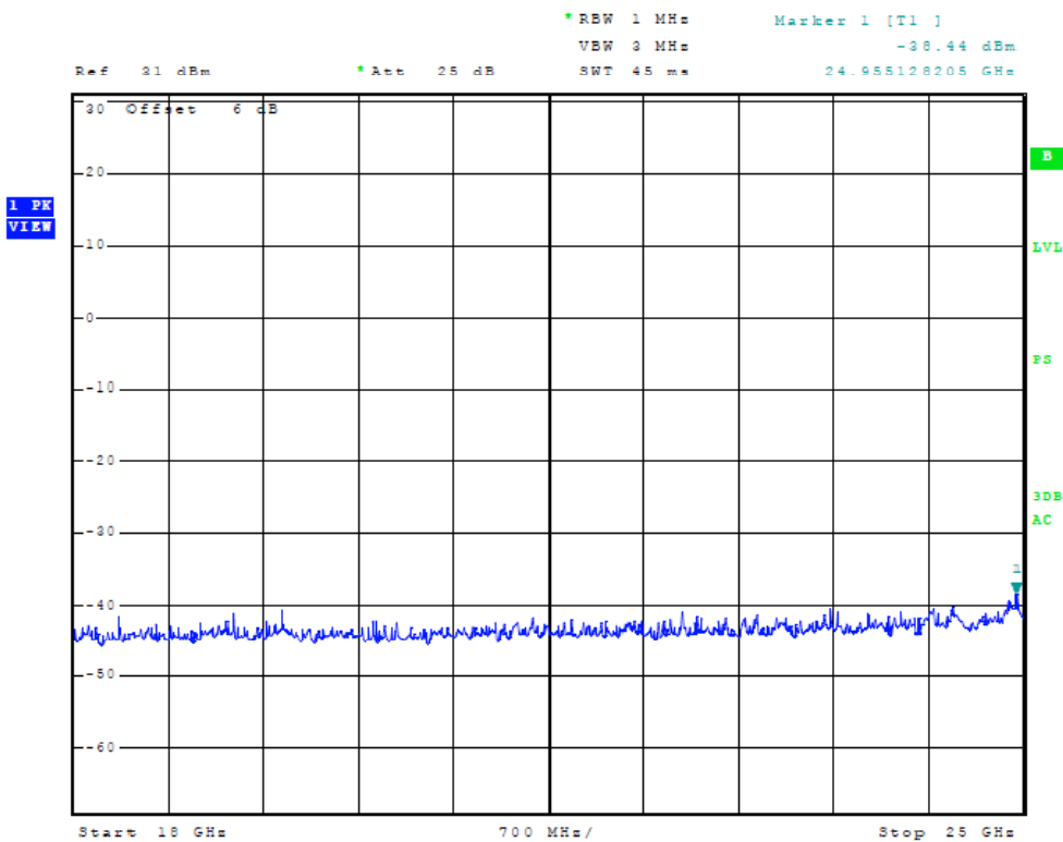
Figure 38 Plot of Antenna port conducted emissions
