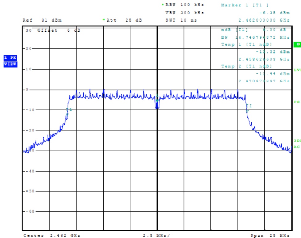
Figure 20 Plot of 6dB Band width (20 MHz Mode, 2462 MHz)
