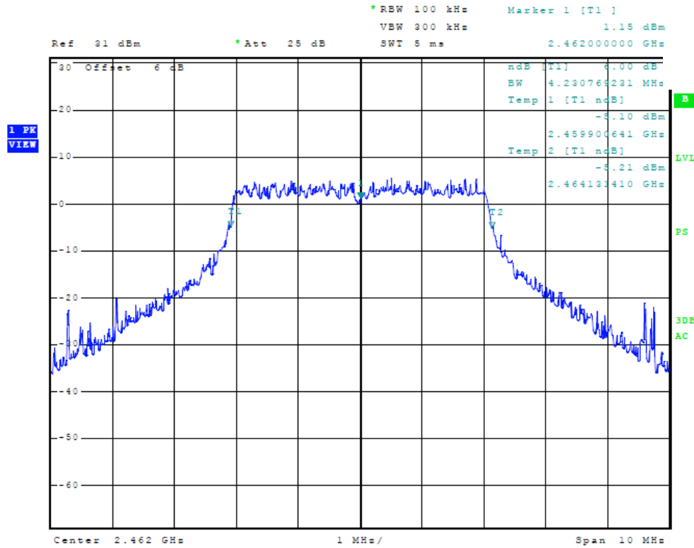
Figure 17 Plot of Plot of 6dB Band width (5 MHz Mode, 2462 MHz)
