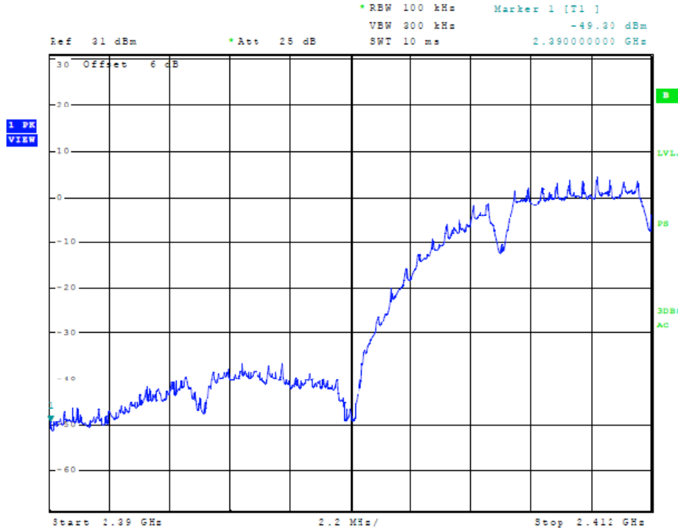
Figure 39 Plot of Band Edge Compliance at Antenna port (worst-case)
