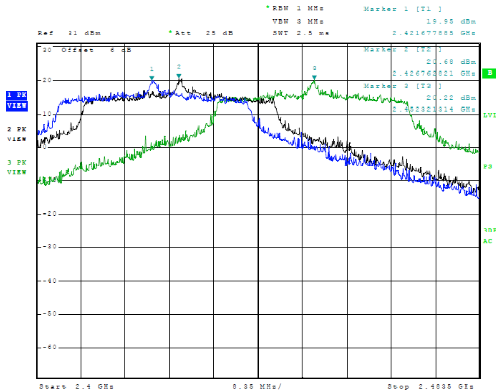
Figure 14 Plot of Antenna Port Emissions (Across Operational Band, 40MHz Mode)
