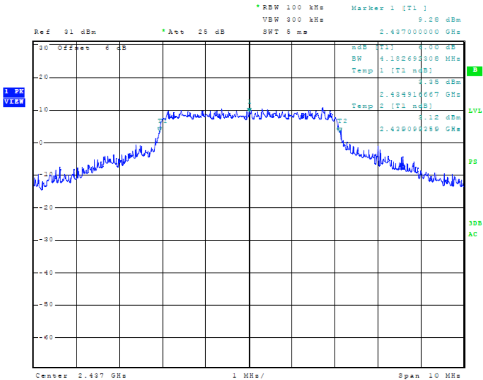
Figure 16 Plot of Plot of 6dB Band width (5 MHz Mode, 2437 MHz)
