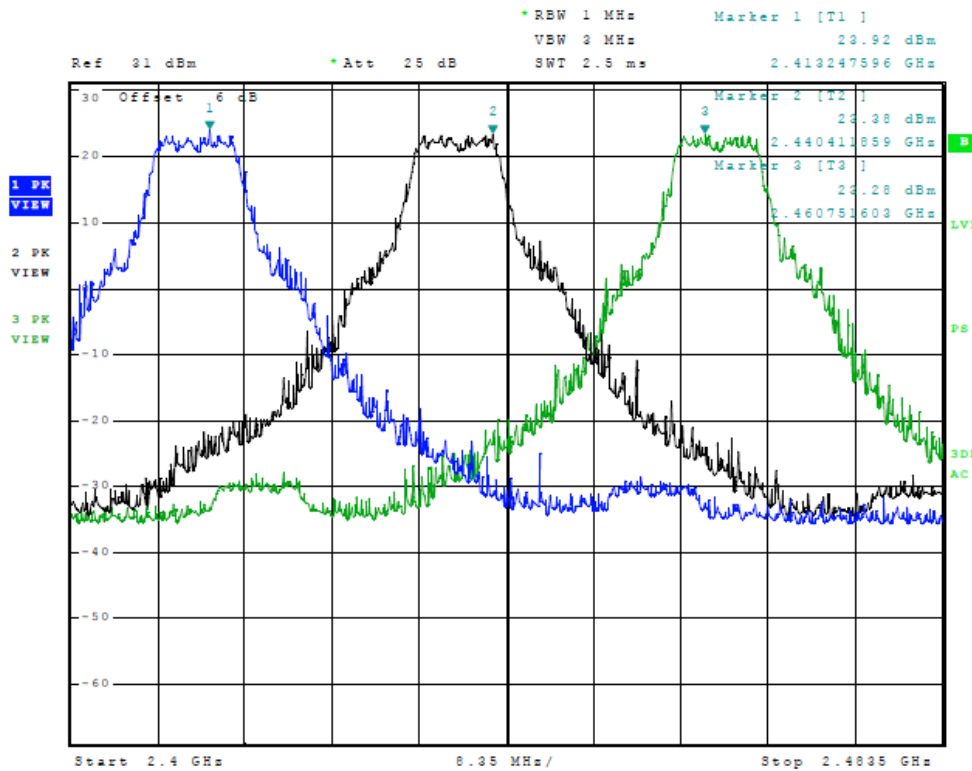
Figure 12 Plot of Antenna Port Emissions (Across Operational Band, 10MHz Mode)
