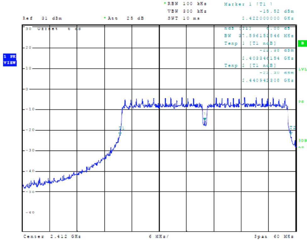
Figure 21 Plot of 6dB Band width (40 MHz Mode, 2422 MHz)
