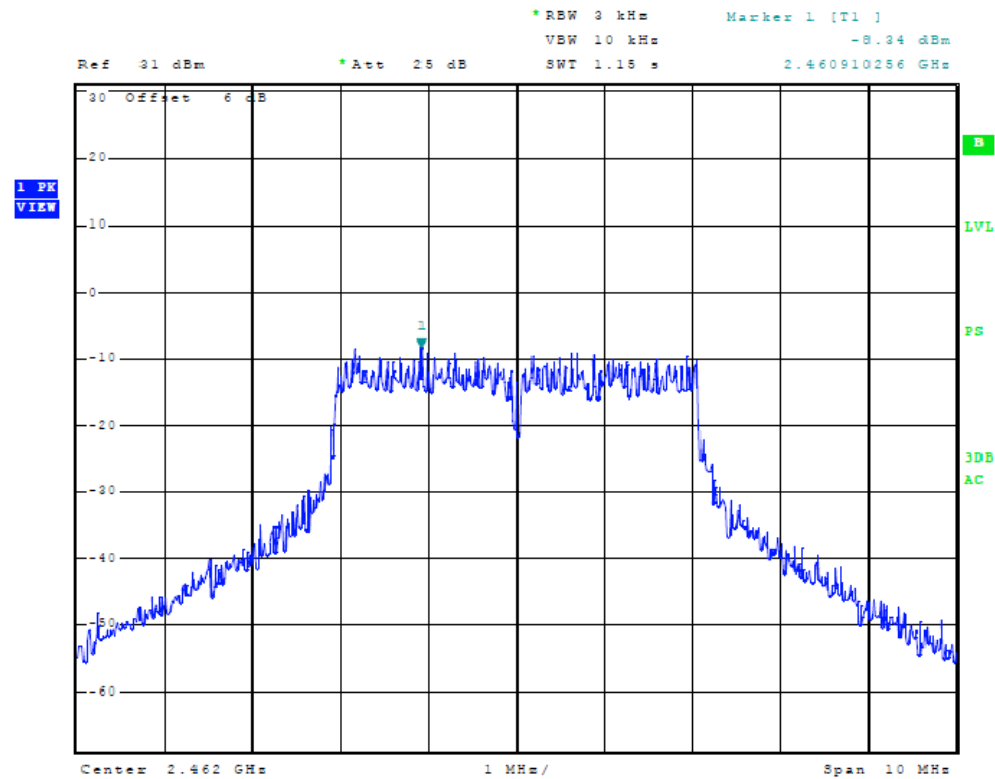
Figure 26 Plot of Power Spectral Density (5 MHz Mode, 2462 MHz)
