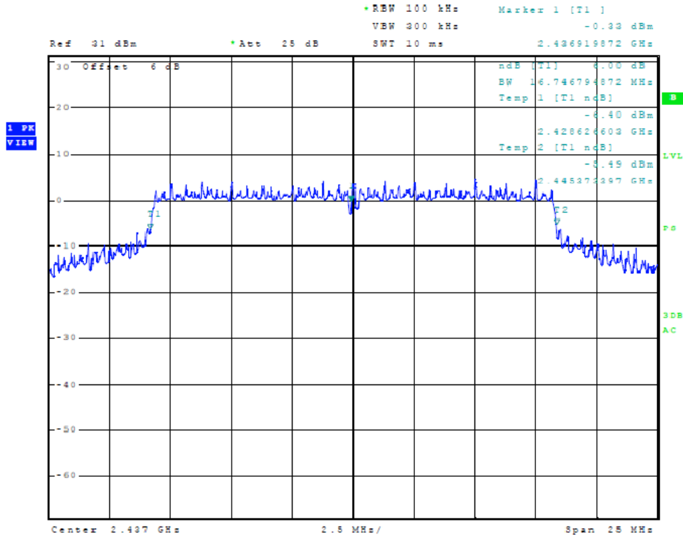
Figure 19 Plot of 6dB Band width (20 MHz Mode, 2437 MHz)
