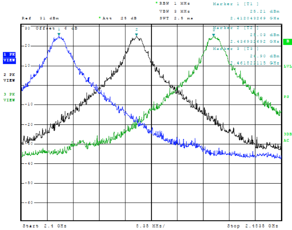
Figure 11 Plot of Antenna Port Emissions (Across Operational Band, 5MHz Mode)
