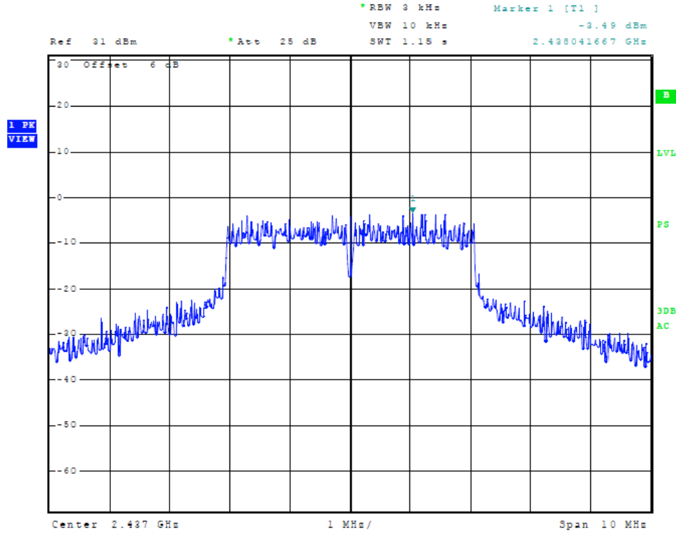
Figure 25 Plot of Power Spectral Density (5 MHz Mode, 2437 MHz)
