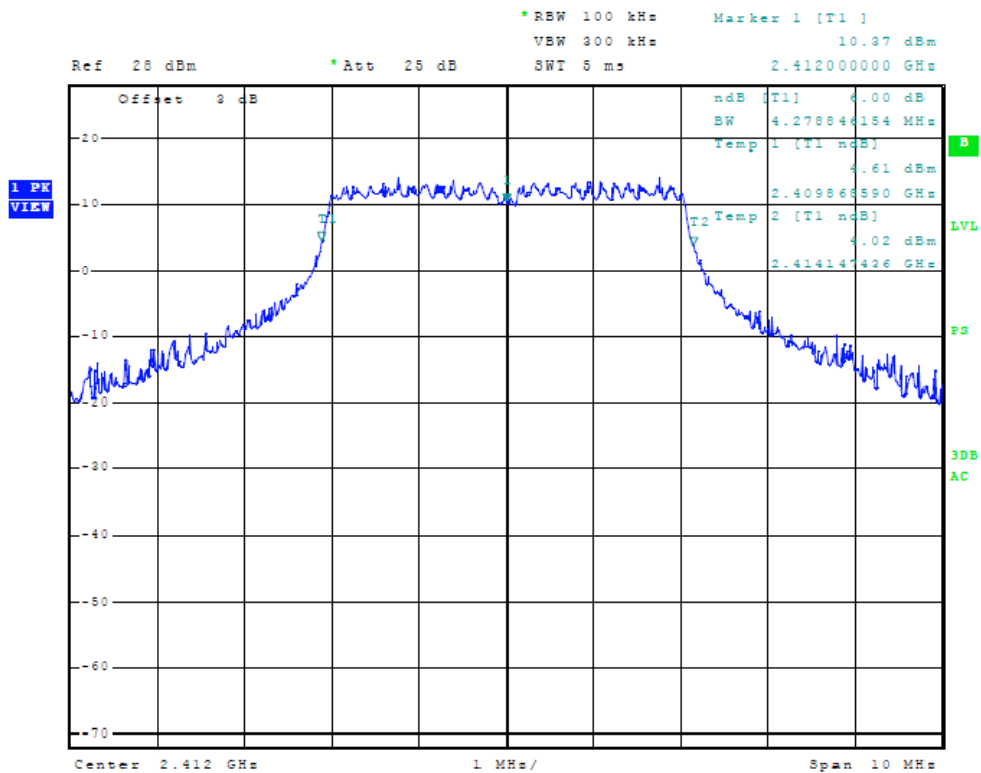
Figure Thirteen Plot of Plot of 6dB Band width (Chain 1, 5 MHz Mode, 2412 MHz)
