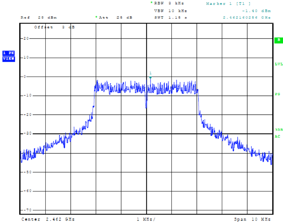
Figure Forty-two Plot of Power Spectral Density (Chain 2, 5 MHz Mode, 2462 MHz)
