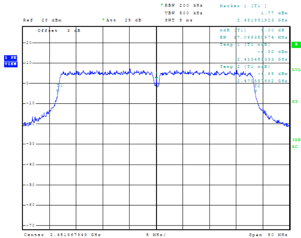
Figure Twenty-one Plot of 6dB Band width (Chain 1, 40 MHz Mode, 2452 MHz)
