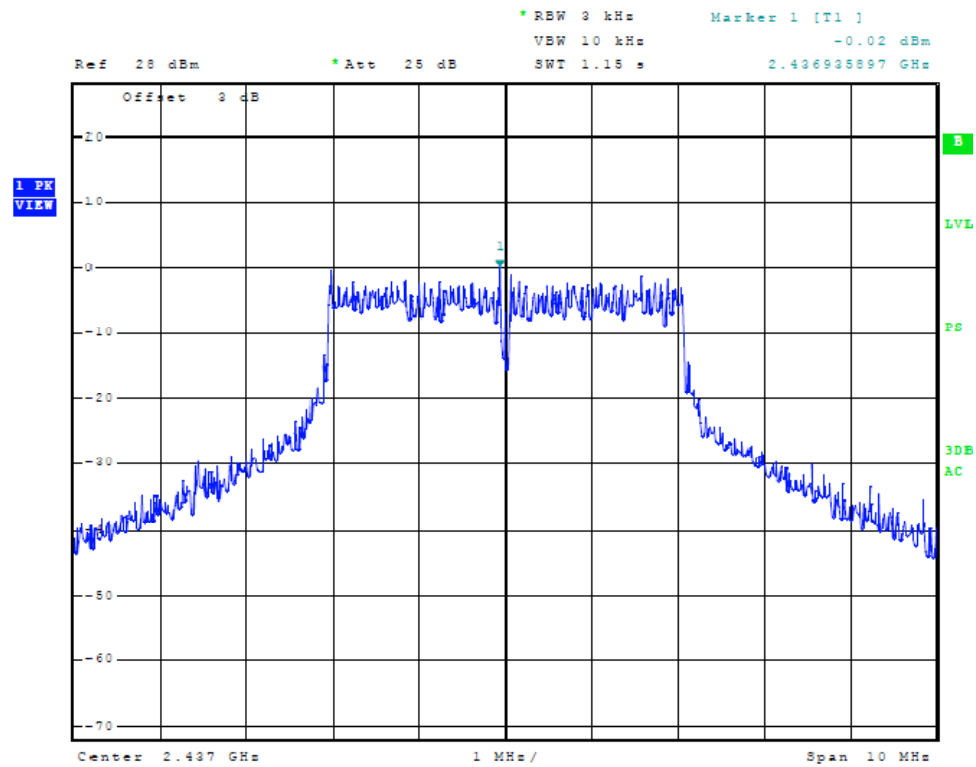
Figure Forty-one Plot of Power Spectral Density (Chain 2, 5 MHz Mode, 2437 MHz)
