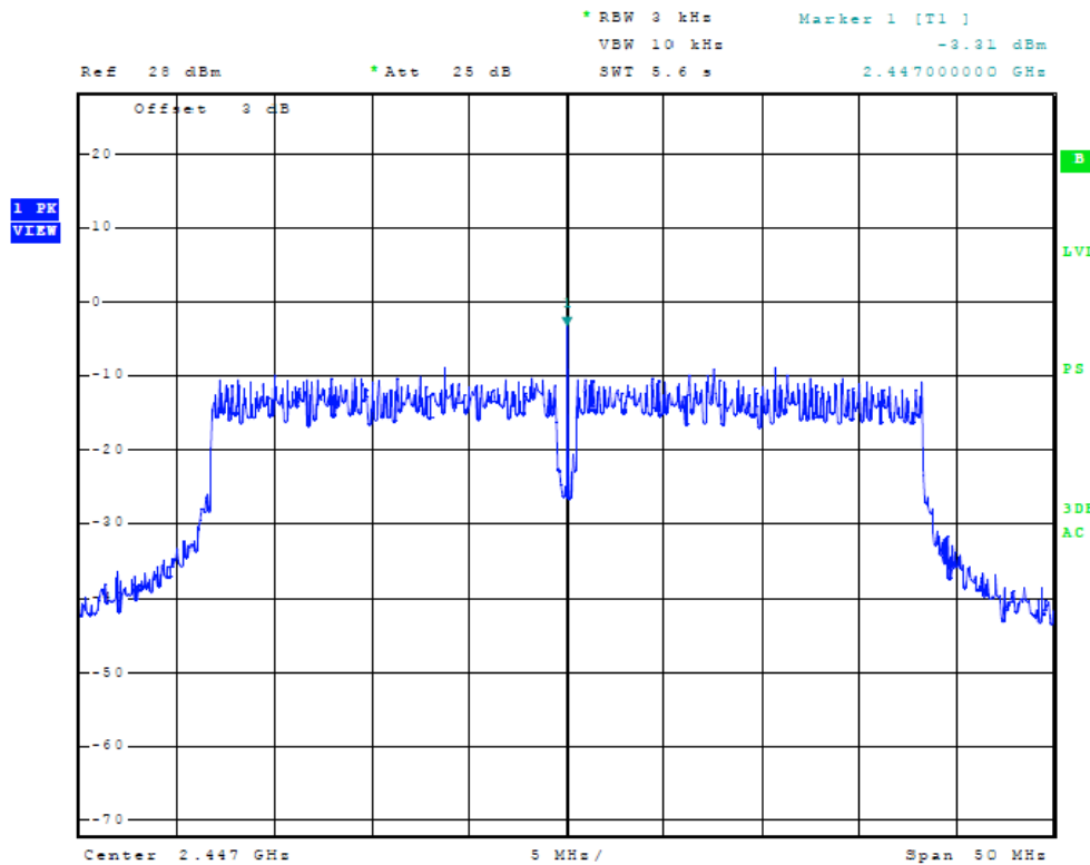
Figure Forty-seven Plot of Power Spectral Density (Chain 2, 40 MHz Mode, 2447 MHz)
