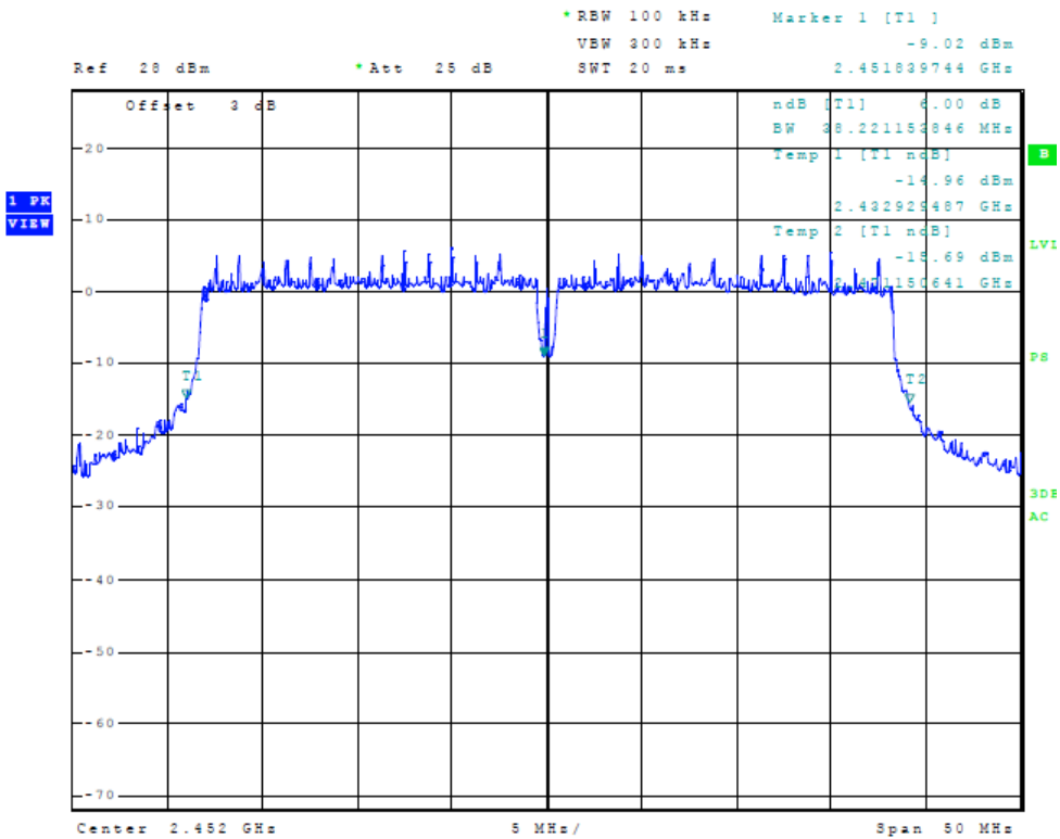
Figure Thirty-nine Plot of 6dB Band width (Chain 2, 40 MHz Mode, 2452 MHz)
