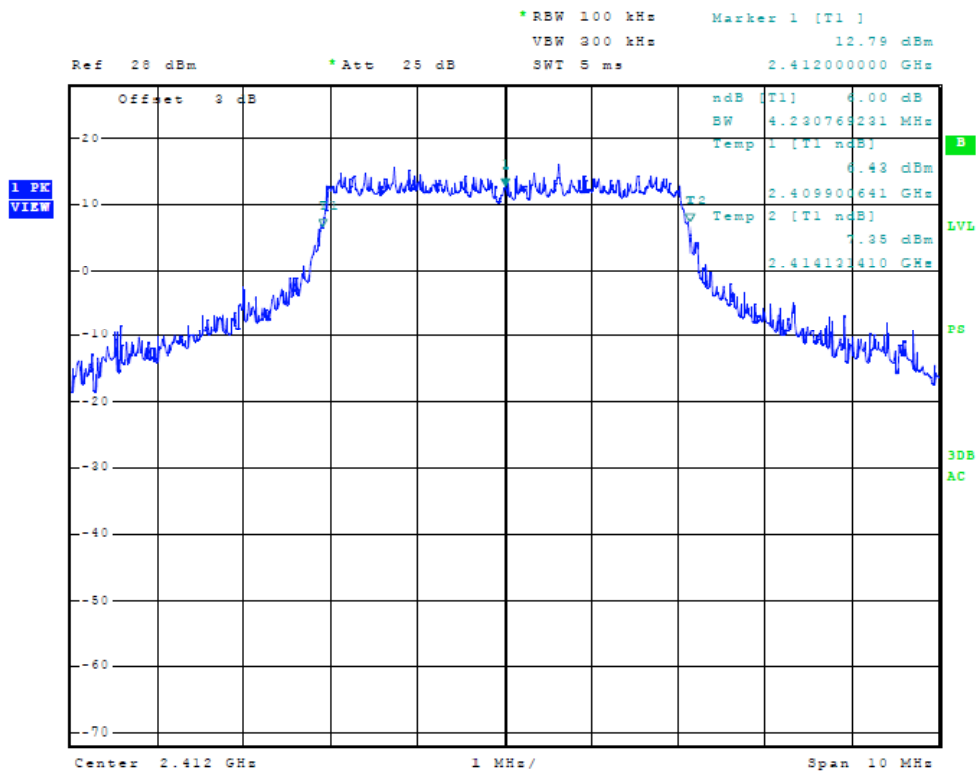
Figure Thirty-one Plot of Plot of 6dB Band width (Chain 2, 5 MHz Mode, 2412 MHz)
