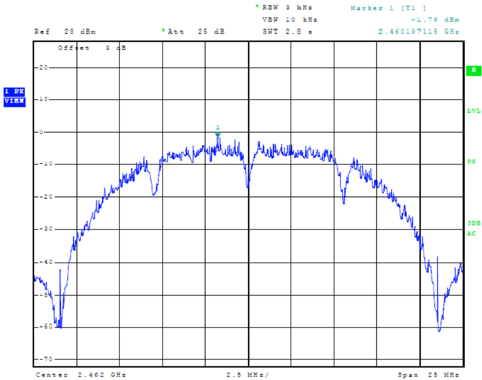
Figure Forty-five Plot of Power Spectral Density (Chain 2, 20 MHz Mode, 2462 MHz)
