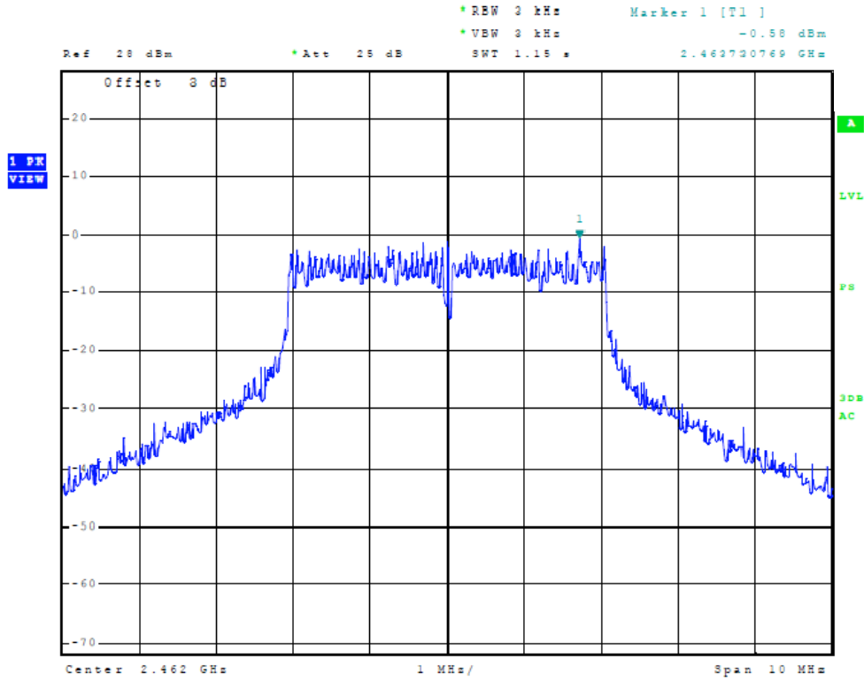
Figure Twenty-four Plot of Power Spectral Density (Chain 1, 5 MHz Mode, 2462 MHz)
