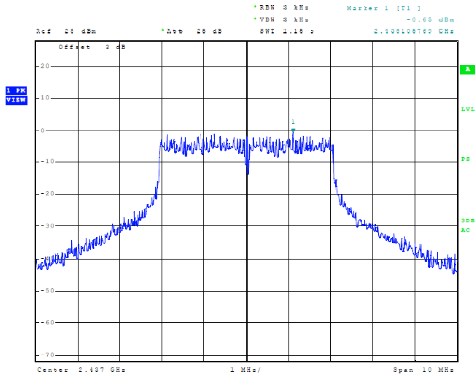
Figure Twenty-three Plot of Power Spectral Density (Chain 1, 5 MHz Mode, 2437 MHz)
