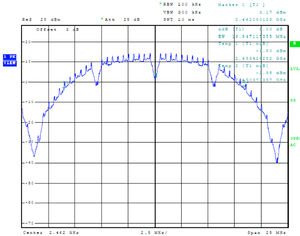
Figure Eighteen Plot of 6dB Band width (Chain 1, 20 MHz Mode, 2462 MHz)
