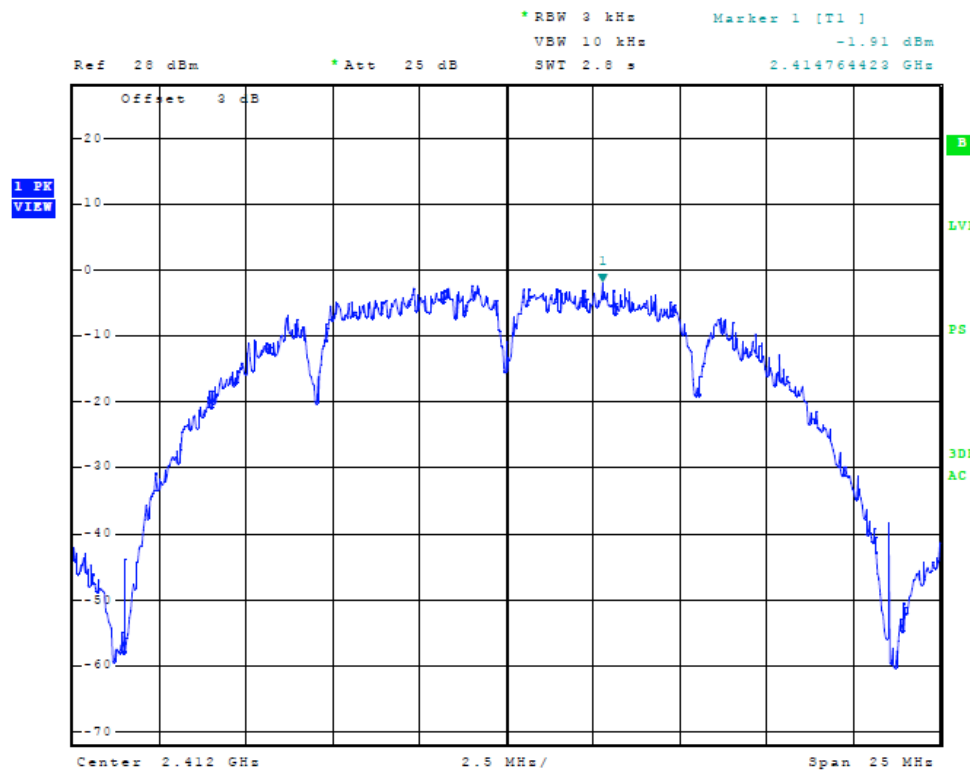
Figure Forty-three Plot of Power Spectral Density (Chain 2, 20 MHz Mode, 2412 MHz)
