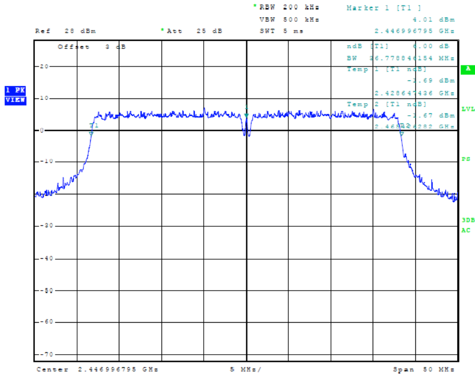
Figure Twenty Plot of 6dB Band width (Chain 1, 40 MHz Mode, 2447 MHz)
