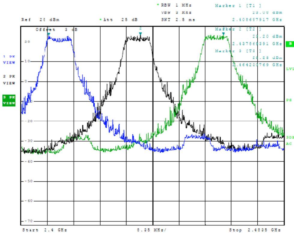
Figure Fifty-seven Plot of Radiated Emissions (Across Operational Band, 10MHz Mode)
