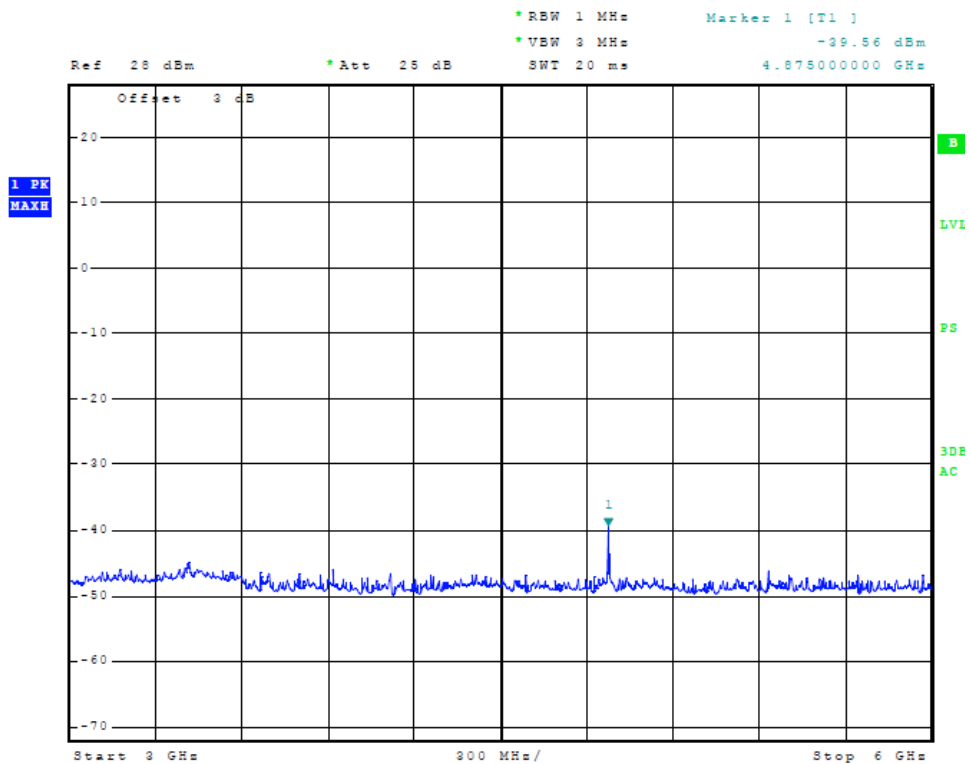
Figure Fifty-one Plot of Antenna port conducted emissions
