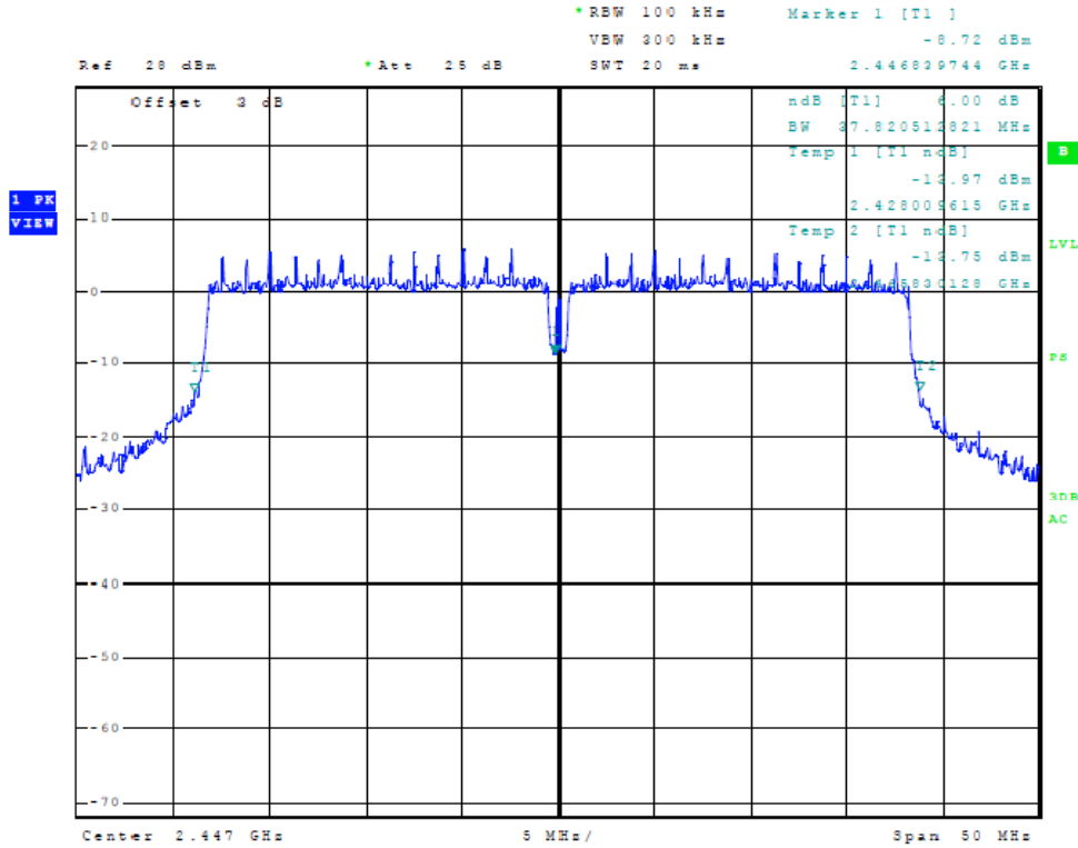
Figure Thirty-eight Plot of 6dB Band width (Chain 2, 40 MHz Mode, 2447 MHz)
