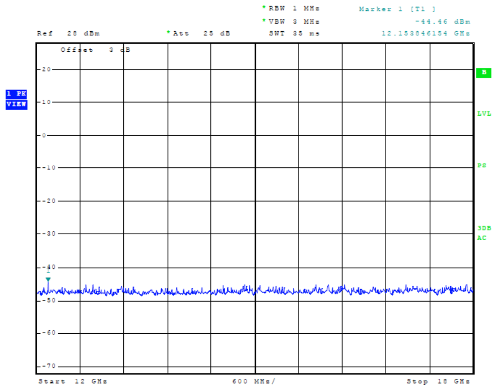
Figure Fifty-three Plot of Antenna port conducted emissions
