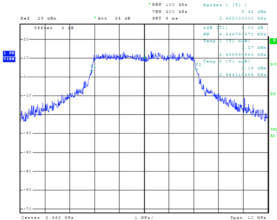
Figure Thirty-three Plot of Plot of 6dB Band width (Chain 2, 5 MHz Mode, 2462 MHz)
