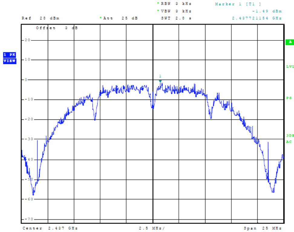
Figure Twenty-six Plot of Power Spectral Density (Chain 1, 20 MHz Mode, 2437 MHz)
