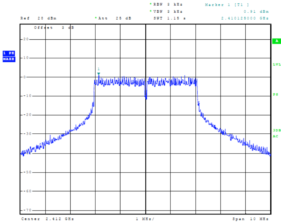
Figure Twenty-two Plot of Power Spectral Density (Chain 1, 5 MHz Mode, 2412 MHz)
