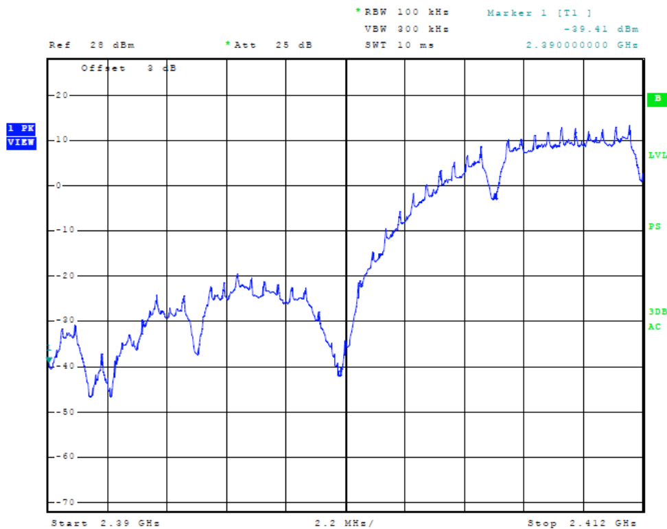
Figure Fifty-five Plot of Band Edge Compliance at Antenna port (worst-case)
