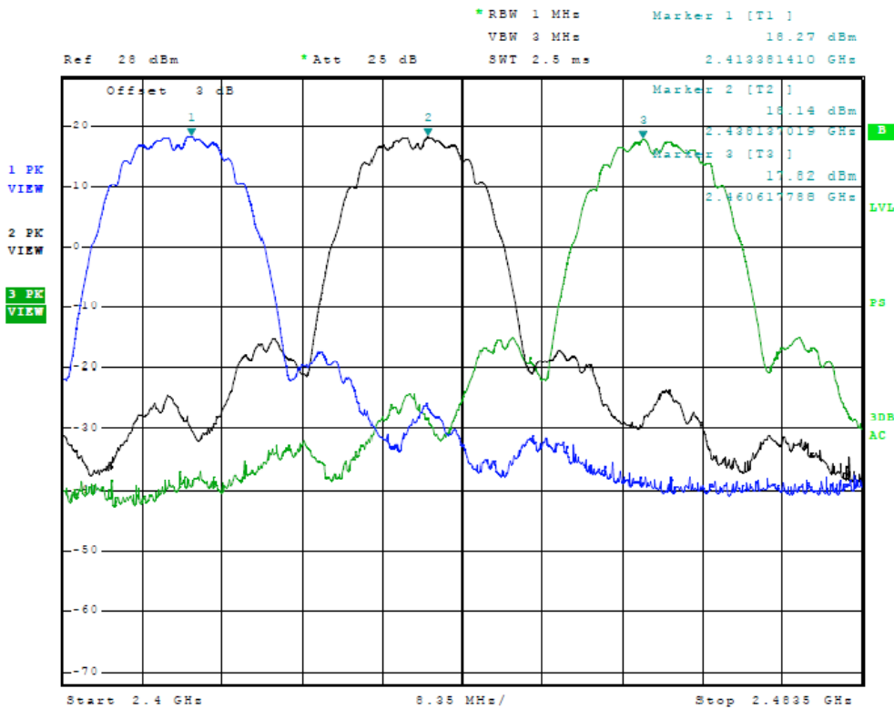
Figure Eleven Plot of Radiated Emissions (Across Operational Band, 20MHz Mode)
