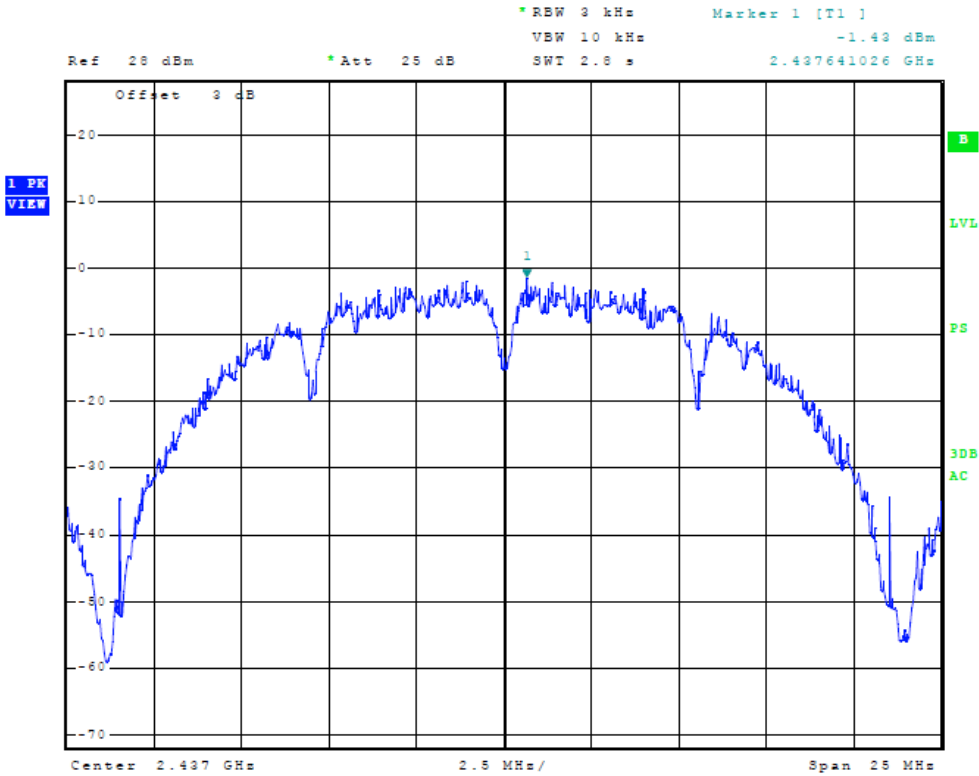
Figure Forty-four Plot of Power Spectral Density (Chain 2, 20 MHz Mode, 2437 MHz)
