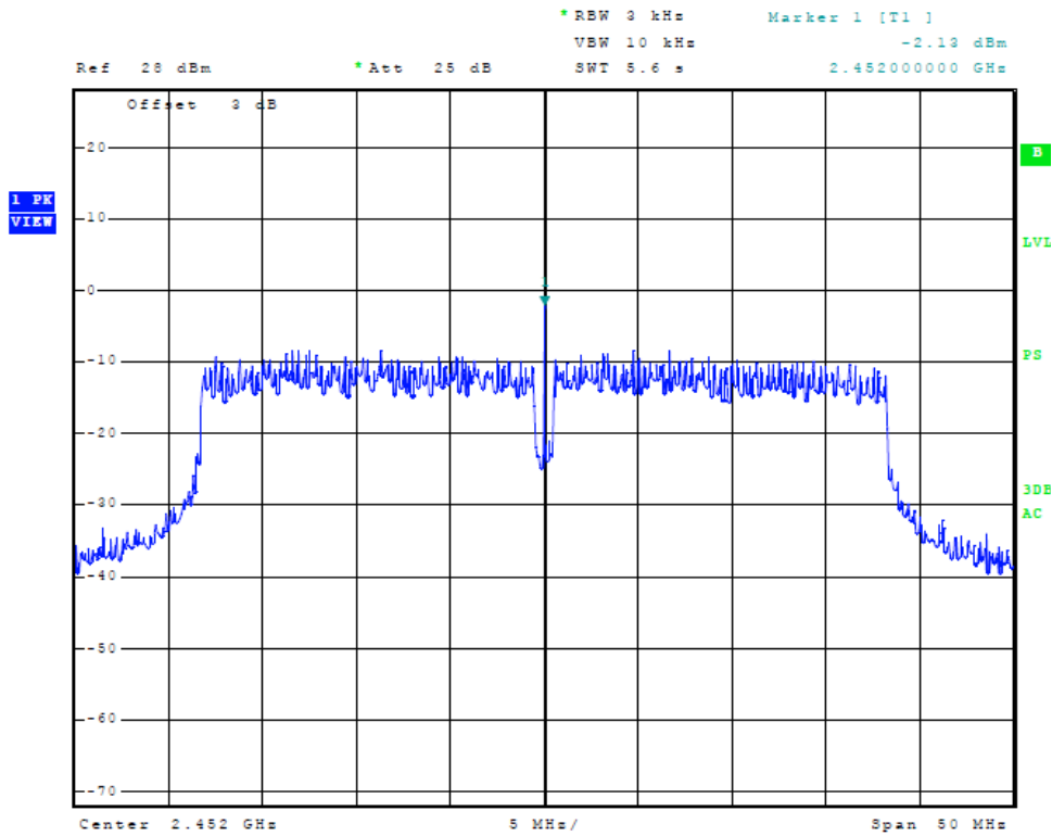
Figure Thirty Plot of Power Spectral Density (Chain 1, 40 MHz Mode, 2452 MHz)
