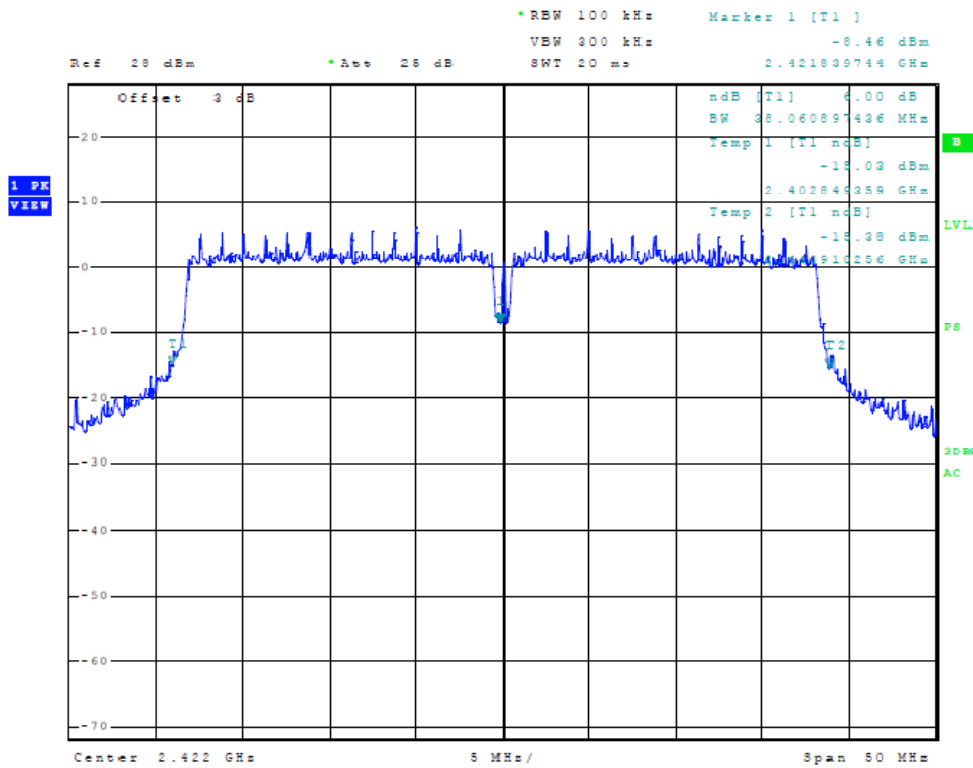
Figure Thirty-seven Plot of 6dB Band width (Chain 2, 40 MHz Mode, 2422 MHz)
