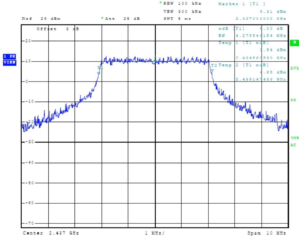
Figure Fourteen Plot of Plot of 6dB Band width (Chain 1, 5 MHz Mode, 2437 MHz)
