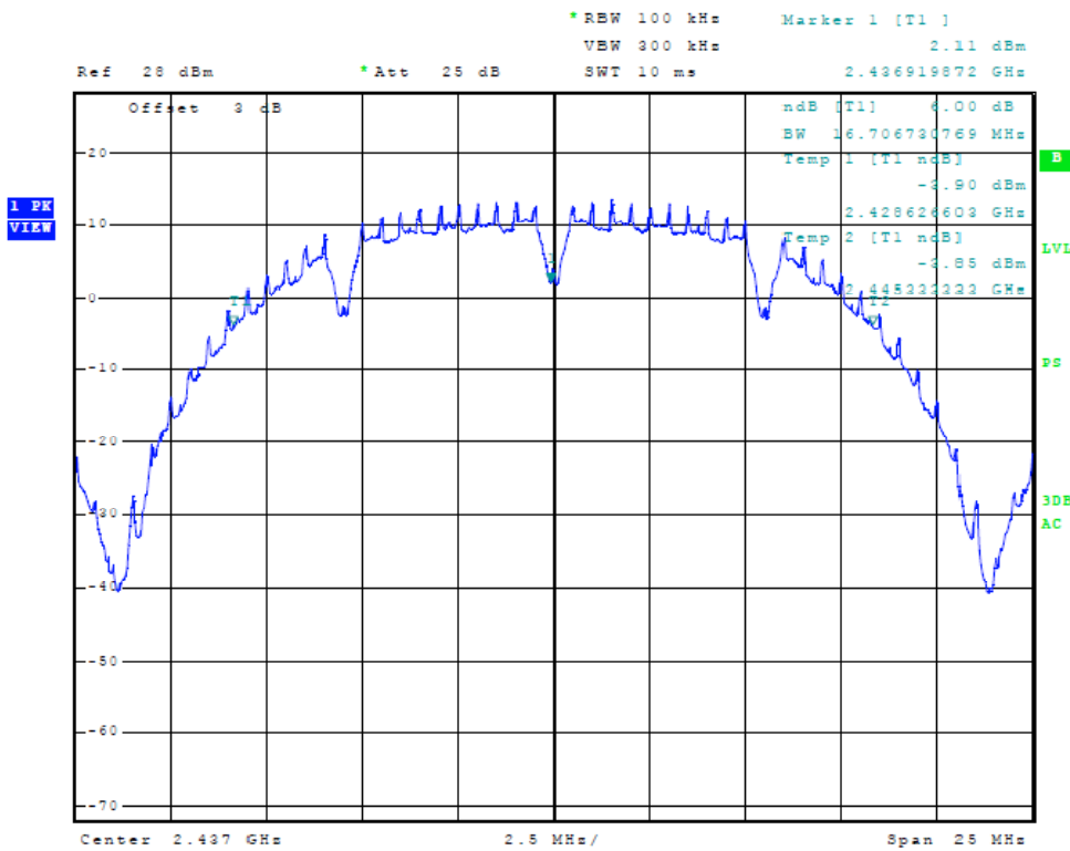
Figure Thirty-five Plot of 6dB Band width (Chain 2, 20 MHz Mode, 2437 MHz)
