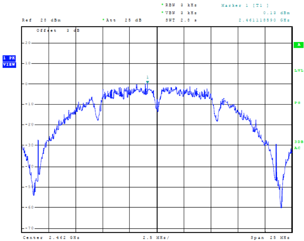
Figure Twenty-seven Plot of Power Spectral Density (Chain 1, 20 MHz Mode, 2462 MHz)
