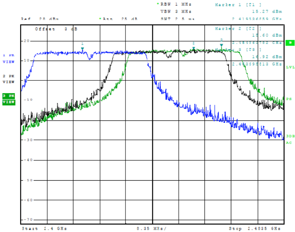
Figure Twelve Plot of Radiated Emissions (Across Operational Band, 40MHz Mode)
