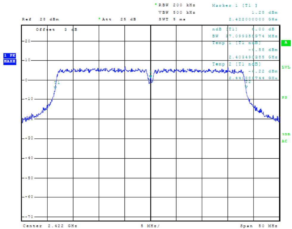
Figure Nineteen Plot of 6dB Band width (Chain 1, 40 MHz Mode, 2422 MHz)
