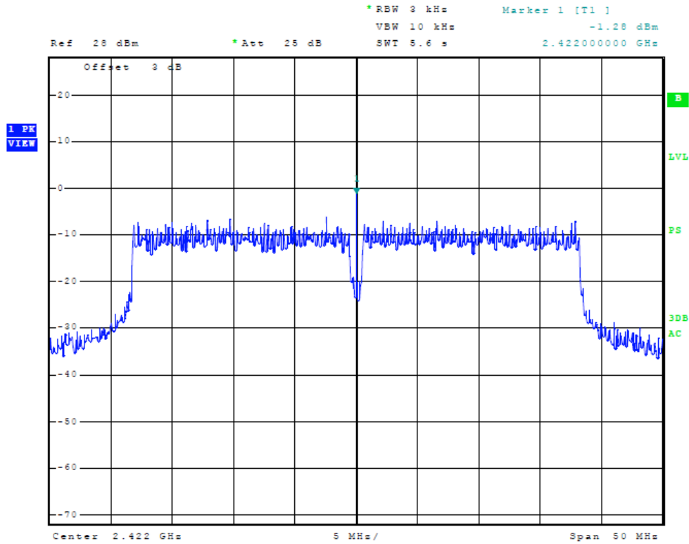
Figure Twenty-eight Plot of Power Spectral Density (Chain 1, 40 MHz Mode, 2422 MHz)
