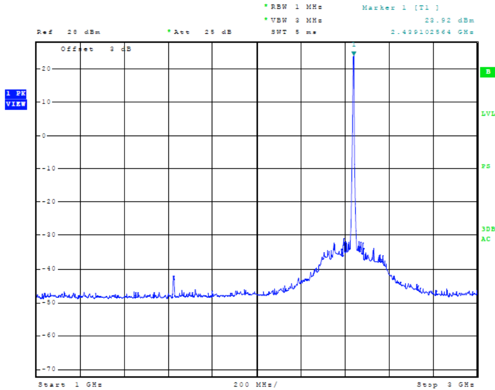
Figure Fifty Plot of Antenna port conducted emissions
