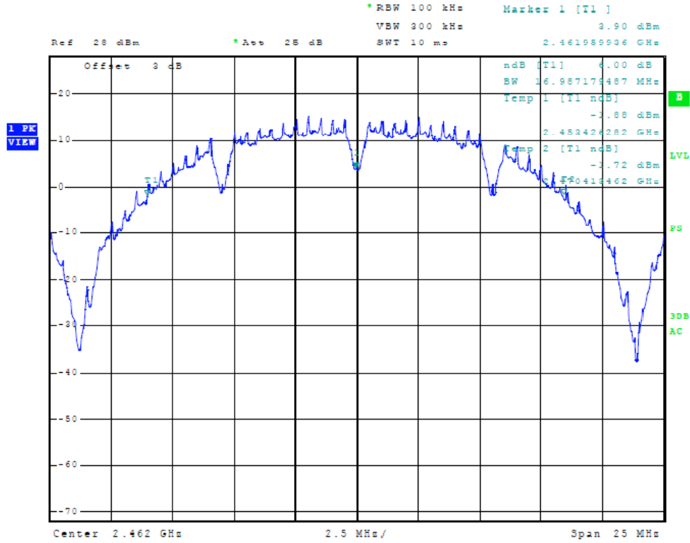
Figure Thirty-six Plot of 6dB Band width (Chain 2, 20 MHz Mode, 2462 MHz)
