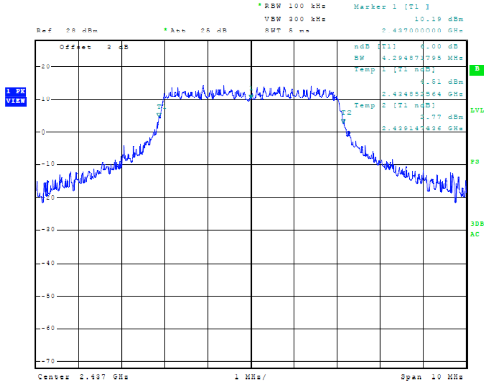
Figure Thirty-two Plot of Plot of 6dB Band width (Chain 2, 5 MHz Mode, 2437 MHz)
