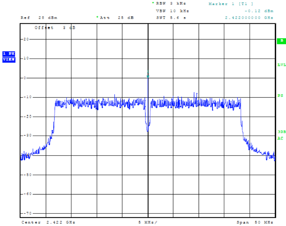
Figure Forty-six Plot of Power Spectral Density (Chain 2, 40 MHz Mode, 2422 MHz)
