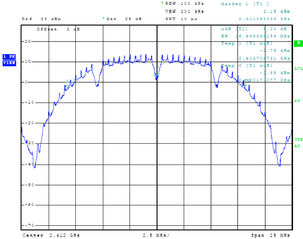
Figure Thirty-four Plot of 6dB Band width (Chain 2, 20 MHz Mode, 2412 MHz)
