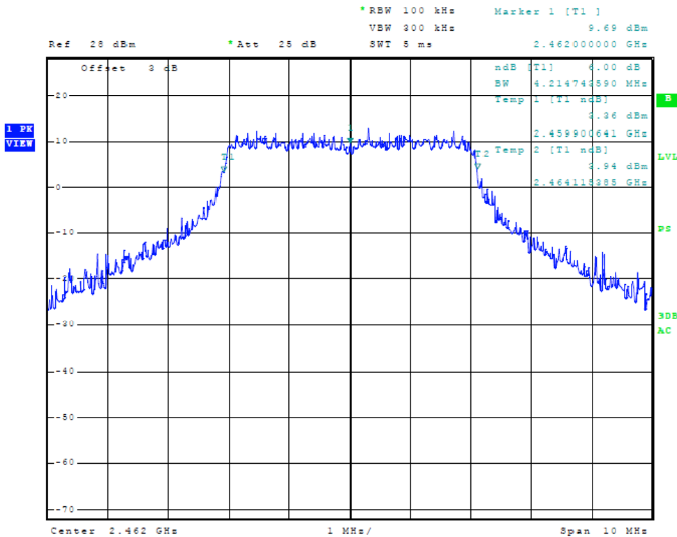
Figure Fifteen Plot of Plot of 6dB Band width (Chain 1, 5 MHz Mode, 2462 MHz)
