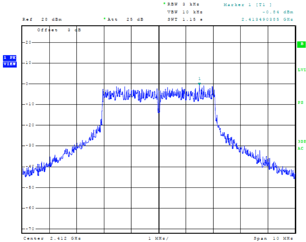
Figure Forty Plot of Power Spectral Density (Chain 2, 5 MHz Mode, 2412 MHz)
