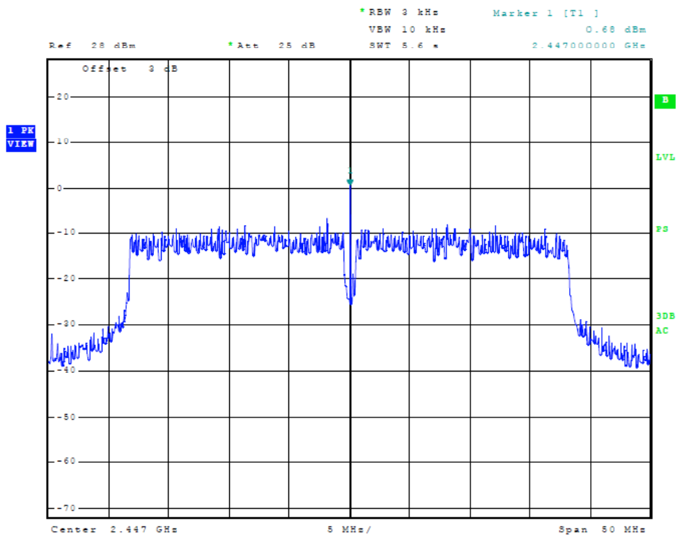
Figure Twenty-nine Plot of Power Spectral Density (Chain 1, 40 MHz Mode, 2447 MHz)
