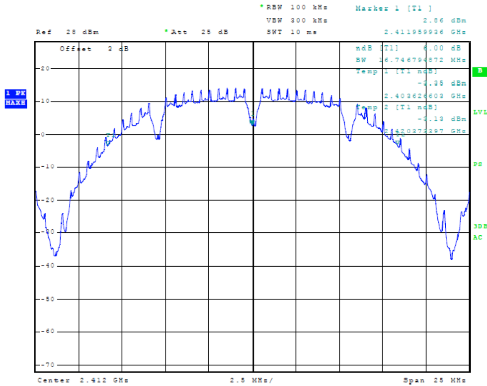
Figure Sixteen Plot of 6dB Band width (Chain 1, 20 MHz Mode, 2412 MHz)
