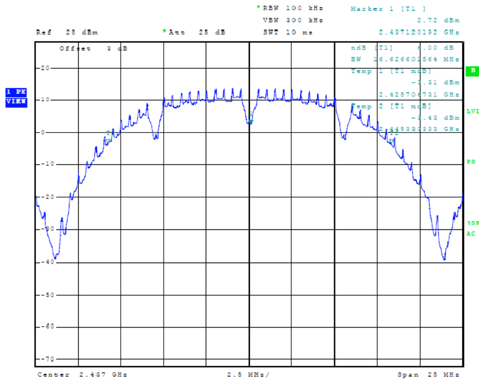
Figure Seventeen Plot of 6dB Band width (Chain 1, 20 MHz Mode, 2437 MHz)
