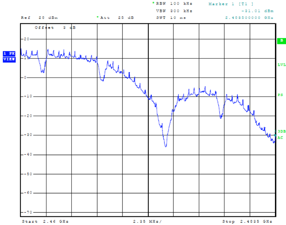
Figure Fifty-six Plot of Band Edge Compliance at Antenna port (worst-case)
