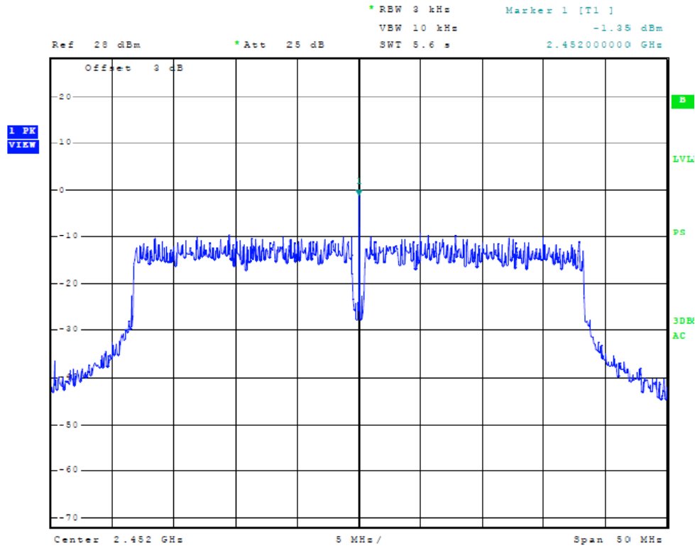
Figure Forty-eight Plot of Power Spectral Density (Chain 2, 40 MHz Mode, 2452 MHz)
