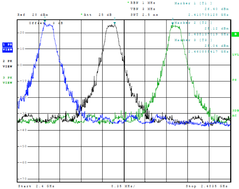
Figure Ten Plot of Radiated Emissions (Across Operational Band, 5MHz Mode)
