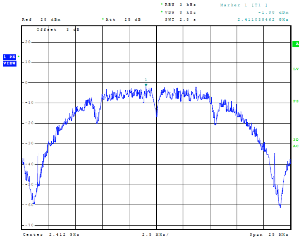
Figure Twenty-five Plot of Power Spectral Density (Chain 1, 20 MHz Mode, 2412 MHz)
