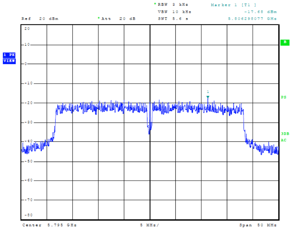
Figure Forty-nine Plot of Power Spectral Density (chain 1, 40 MHz Mode, 5795 MHz)
