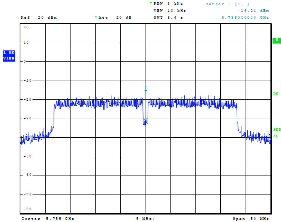
Figure Forty-eight Plot of Power Spectral Density (chain 1, 40 MHz Mode, 5755 MHz)
