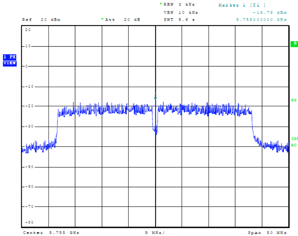
Figure Thirty Plot of Power Spectral Density (chain 1, 40 MHz Mode, 5755 MHz)
