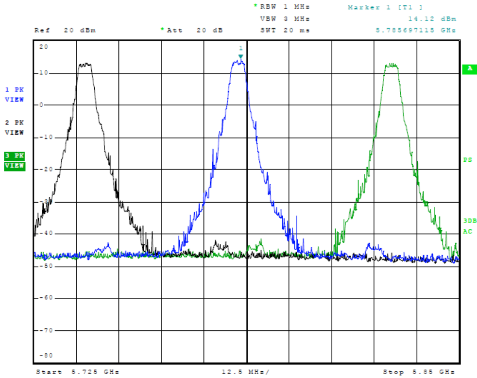
Figure Twelve Plot of Radiated Emissions (Across Operational Band, 5MHz Mode)
