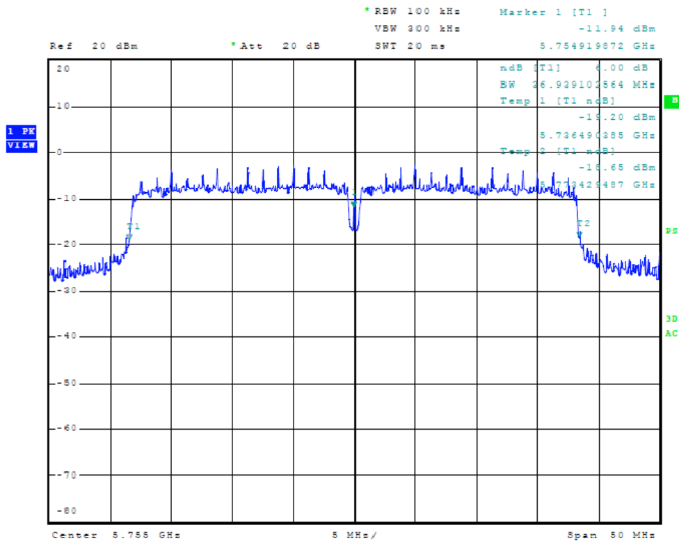
Figure Twenty-one Plot of 6dB Band width (chain 1, 40 MHz Mode, 5755 MHz)
