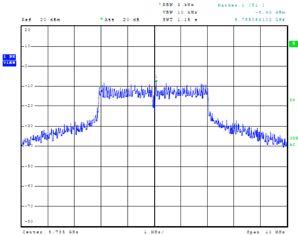
Figure Forty-three Plot of Power Spectral Density (chain 2, 5 MHz Mode, 5785 MHz)
