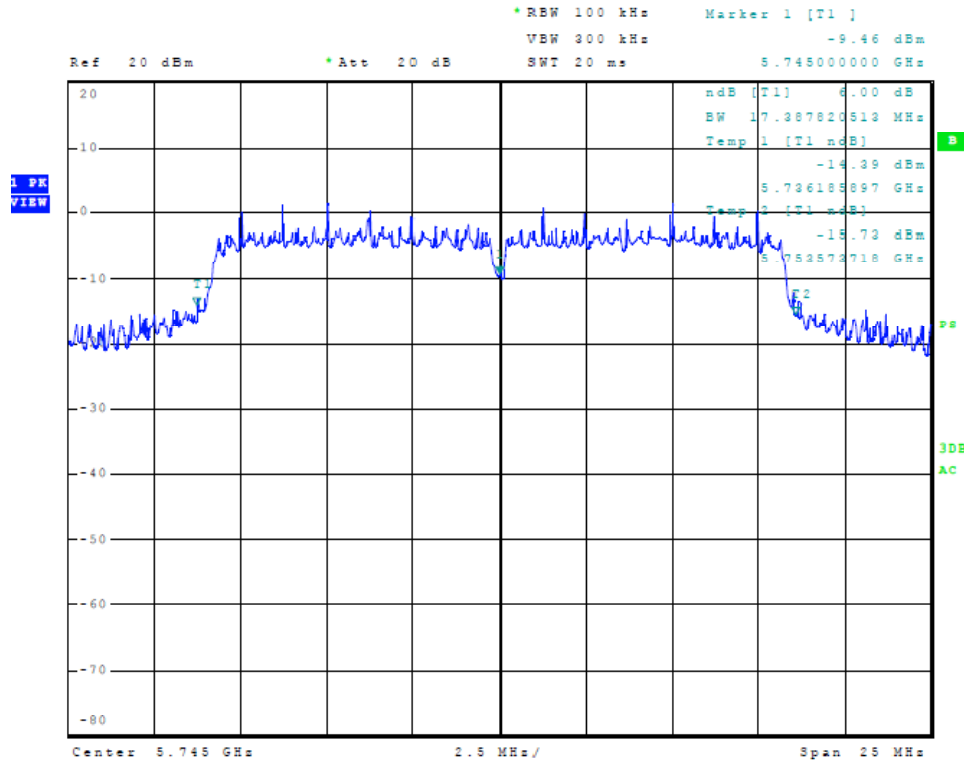
Figure Thirty-six Plot of 6dB Band width (chain 2, 20 MHz Mode, 5745 MHz)
