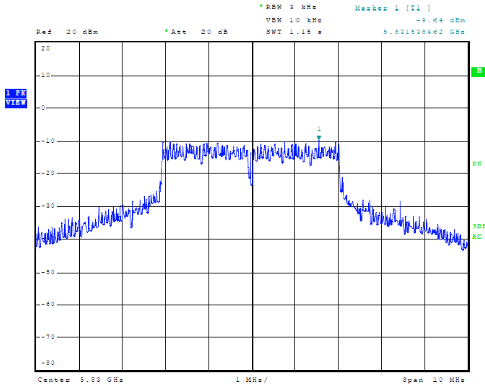
Figure Forty-four Plot of Power Spectral Density (chain 2, 5 MHz Mode, 5830 MHz)
