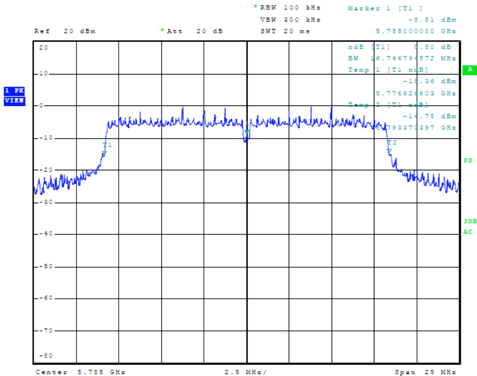
Figure Nineteen Plot of 6dB Band width (chain 1, 20 MHz Mode, 5785 MHz)
