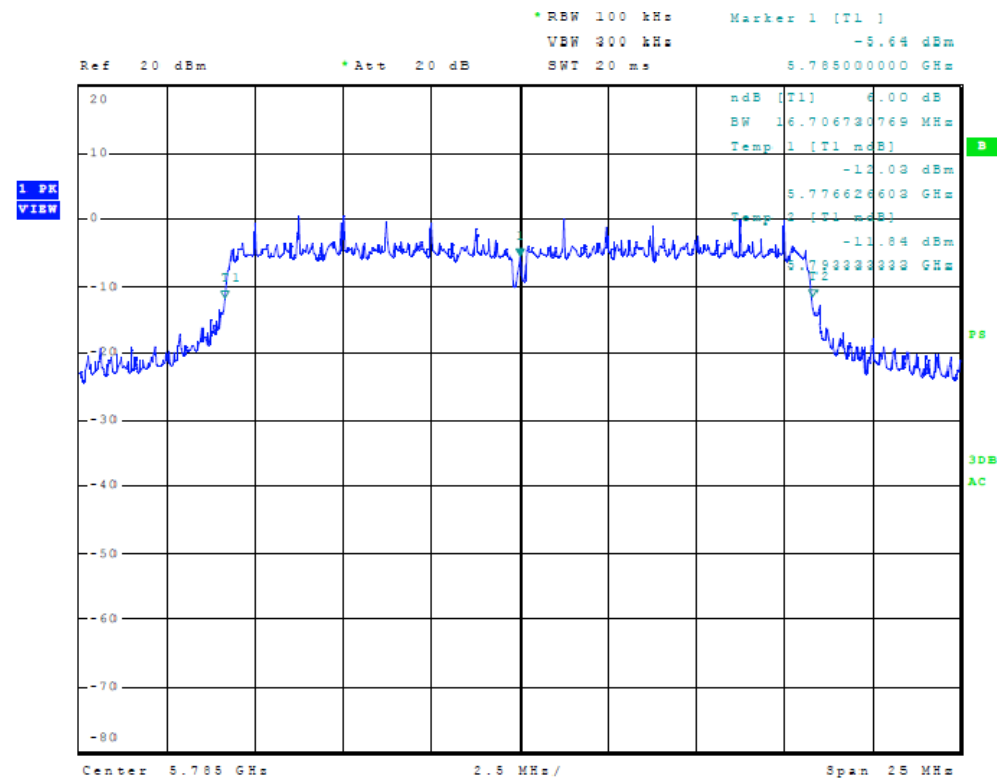
Figure Thirty-seven Plot of 6dB Band width (chain 2, 20 MHz Mode, 5785 MHz)
