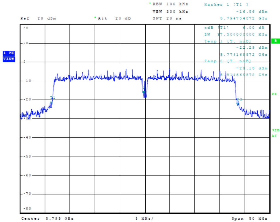
Figure Forty Plot of 6dB Band width (chain 2, 40 MHz Mode, 5795 MHz)
