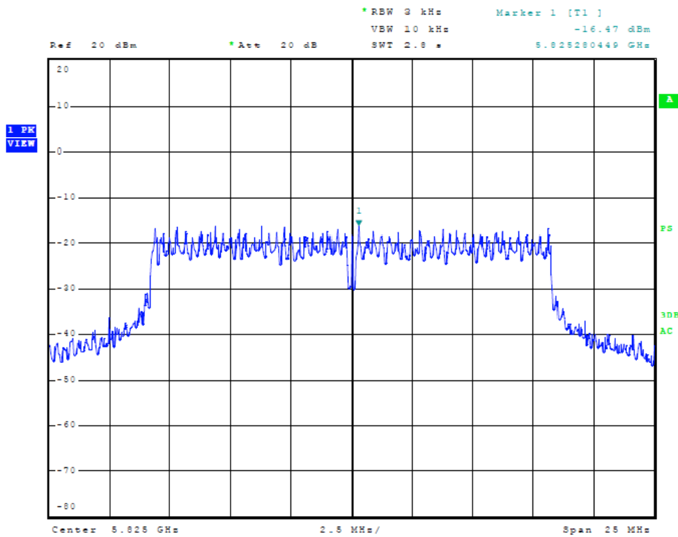
Figure Twenty-nine Plot of Power Spectral Density (chain 1, 20 MHz Mode, 5825 MHz)
