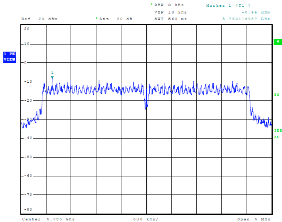
Figure Twenty-five Plot of Power Spectral Density (chain 1, 5 MHz Mode, 5785 MHz)
