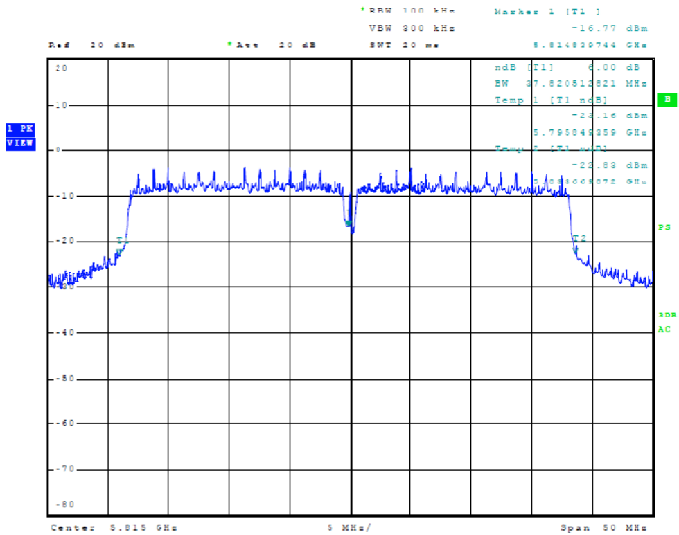
Figure Forty-one Plot of 6dB Band width (chain 2, 40 MHz Mode, 5815 MHz)
