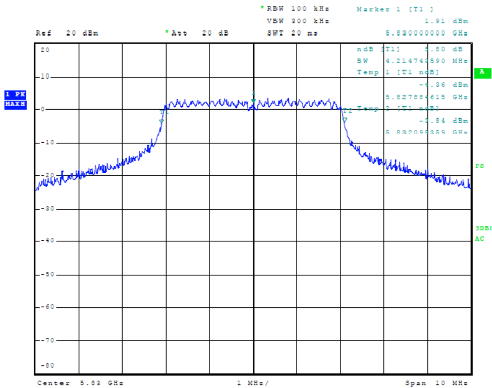
Figure Seventeen Plot of Plot of 6dB Band width (chain 1, 5 MHz Mode, 5830 MHz)
