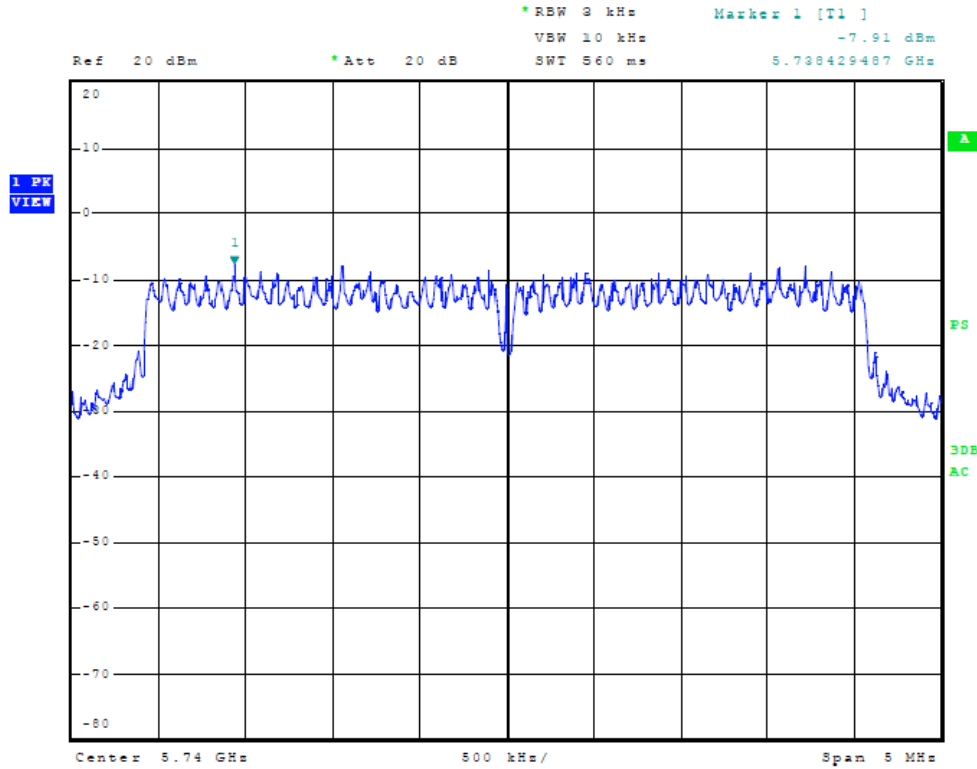
Figure Twenty-four Plot of Power Spectral Density (chain 1, 5 MHz Mode, 5740 MHz)
