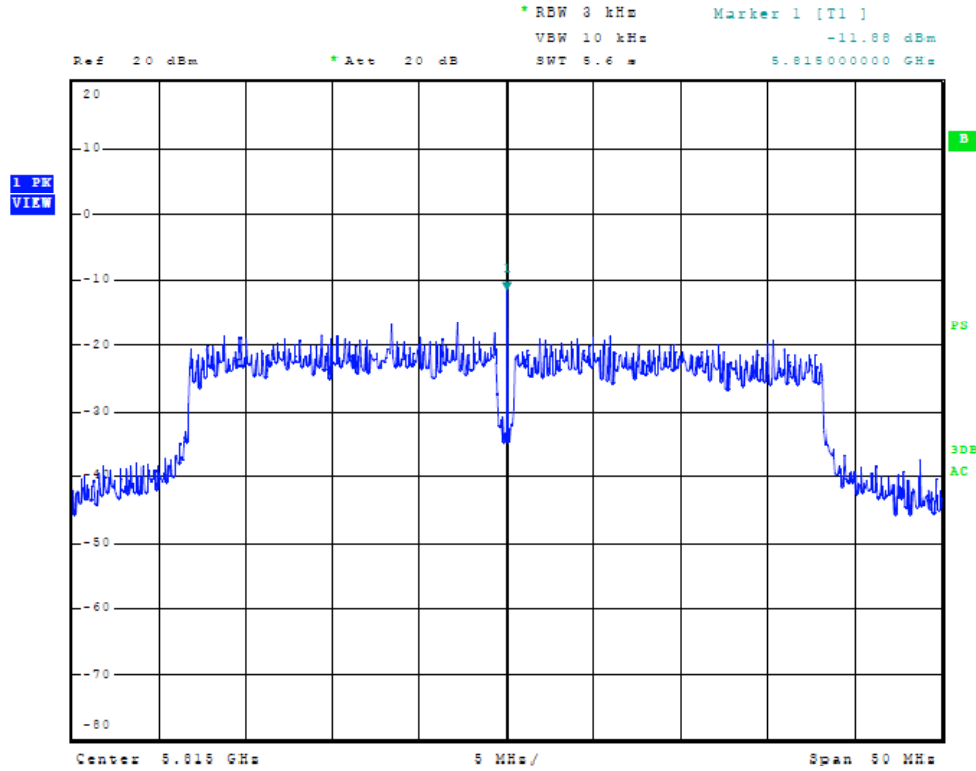
Figure Thirty-two Plot of Power Spectral Density (chain 1, 40 MHz Mode, 5815 MHz)
