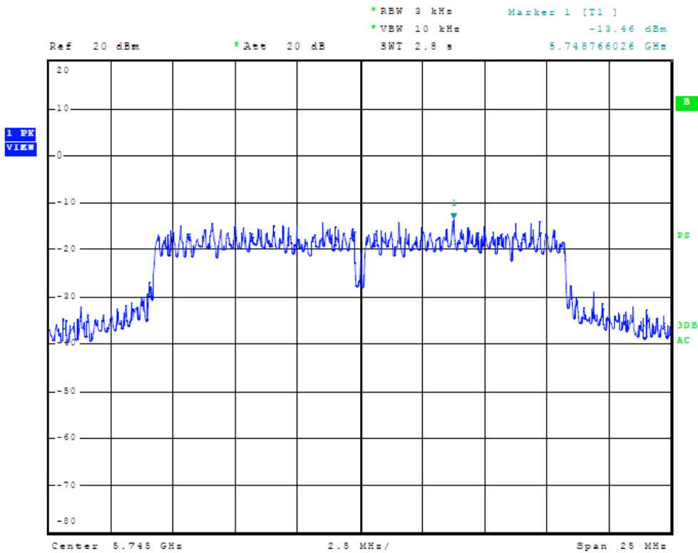
Figure Twenty-seven Plot of Power Spectral Density (chain 1, 20 MHz Mode, 5745 MHz)
