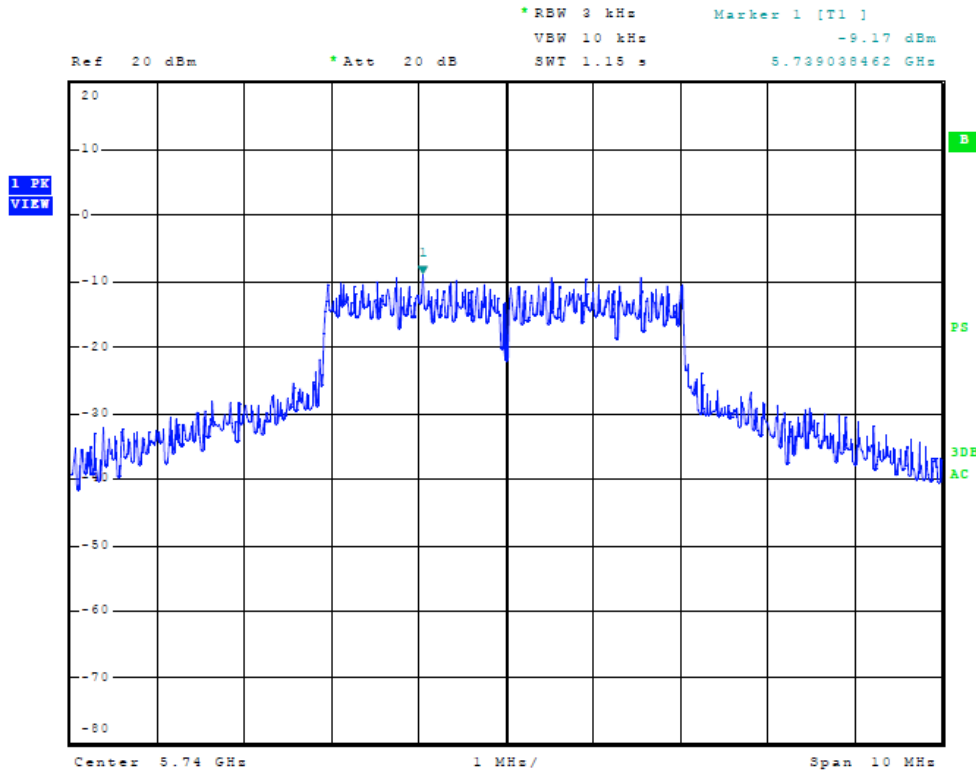
Figure Forty-two Plot of Power Spectral Density (chain 2, 5 MHz Mode, 5740 MHz)
