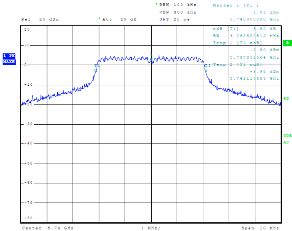
Figure Fifteen Plot of Plot of 6dB Band width (chain 1, 5 MHz Mode, 5740 MHz)
