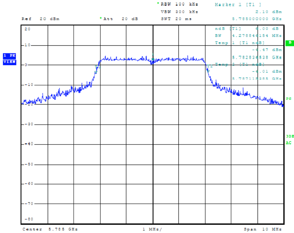
Figure Thirty-four Plot of Plot of 6dB Band width (chain 2, 5 MHz Mode, 5785 MHz)
