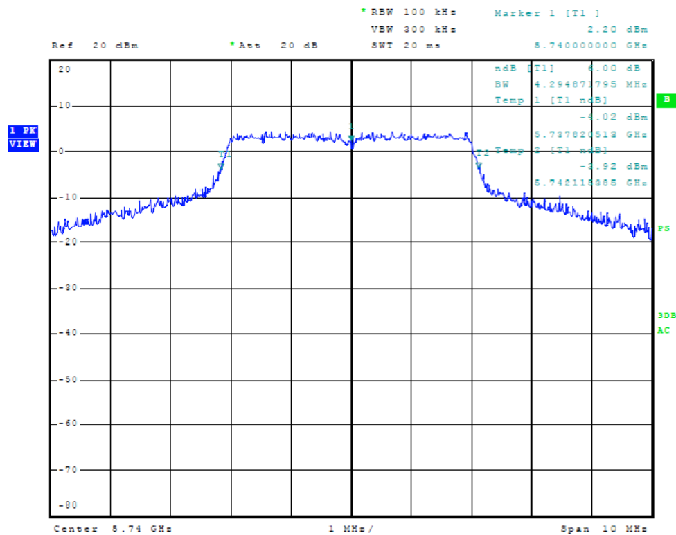
Figure Thirty-three Plot of Plot of 6dB Band width (chain 2, 5 MHz Mode, 5740 MHz)
