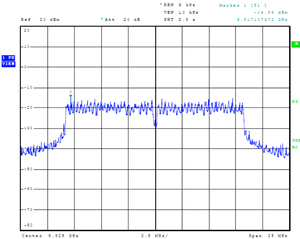
Figure Forty-seven Plot of Power Spectral Density (chain 1, 20 MHz Mode, 5825 MHz)
