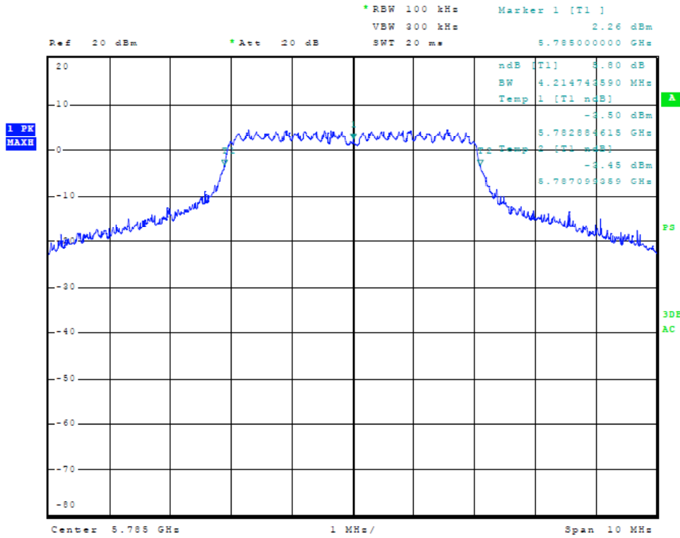
Figure Sixteen Plot of Plot of 6dB Band width (chain 1, 5 MHz Mode, 5785 MHz)
