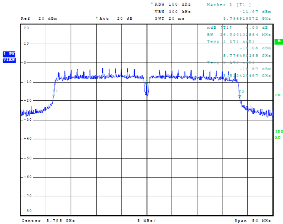
Figure Twenty-two Plot of 6dB Band width (chain 1, 40 MHz Mode, 5795 MHz)
