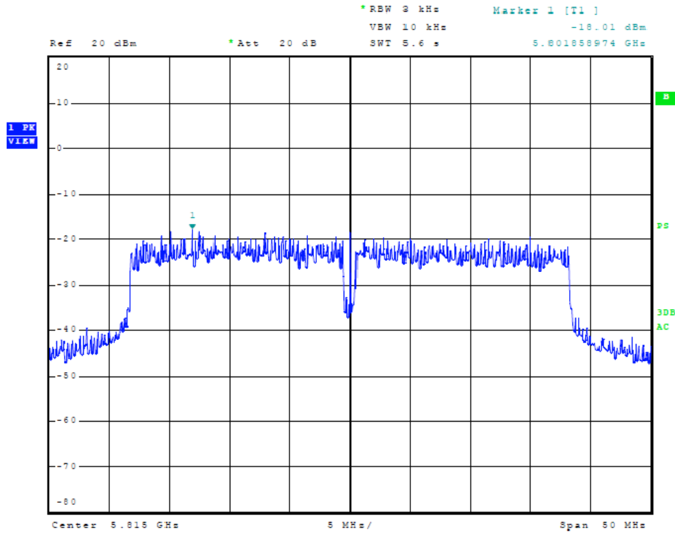
Figure Fifty Plot of Power Spectral Density (chain 1, 40 MHz Mode, 5815 MHz)
