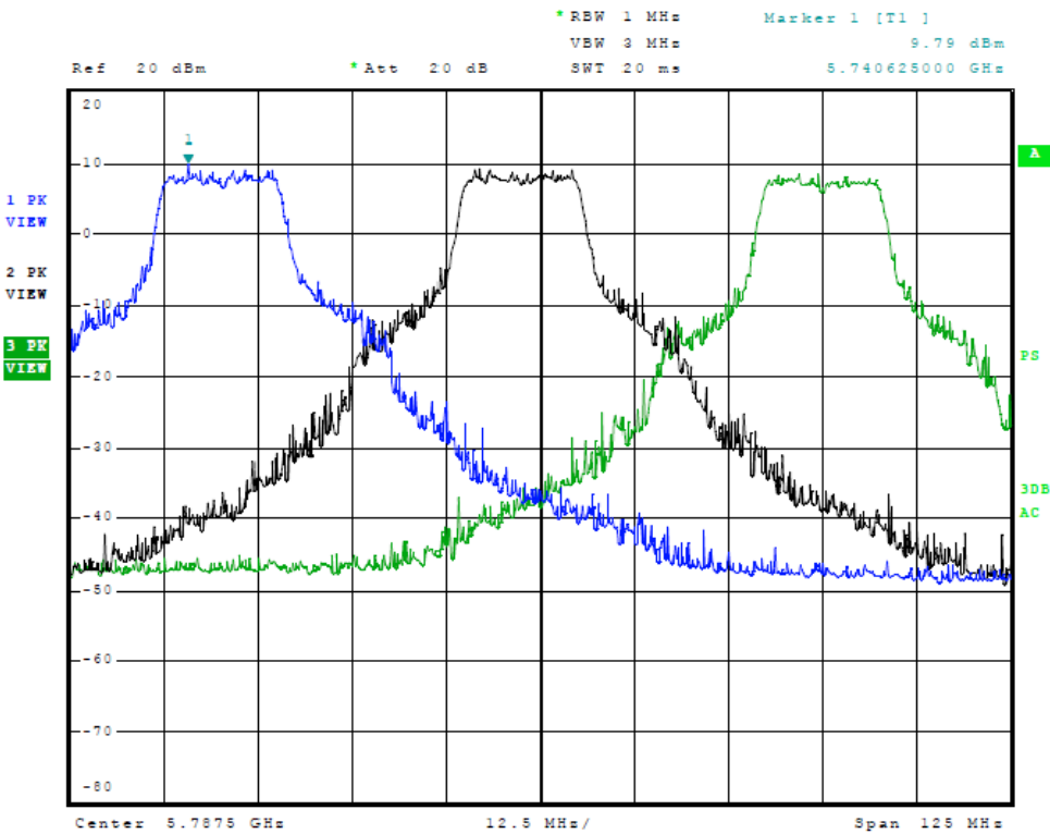
Figure Thirteen Plot of Radiated Emissions (Across Operational Band, 20MHz Mode)
