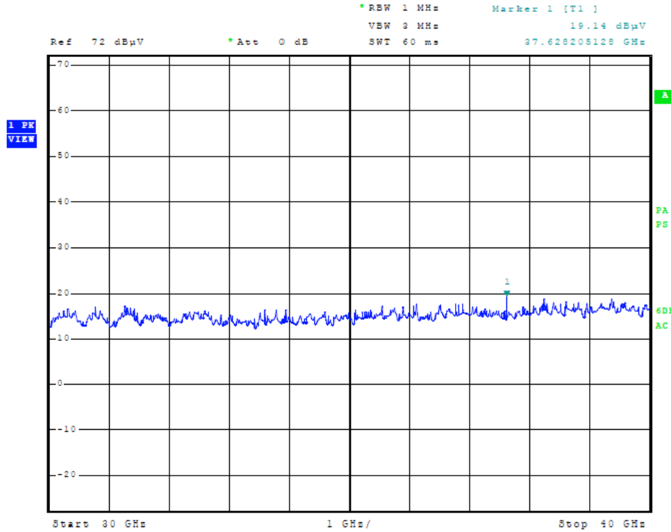
Figure Eleven General Radiated Emissions taken at 1 meter in screen room General Radiated Emissions from EUT Data (Highest Emissions)
