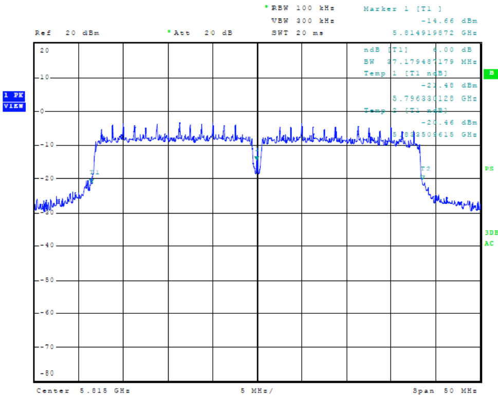
Figure Twenty-three Plot of 6dB Band width (chain 1, 40 MHz Mode, 5815 MHz)
