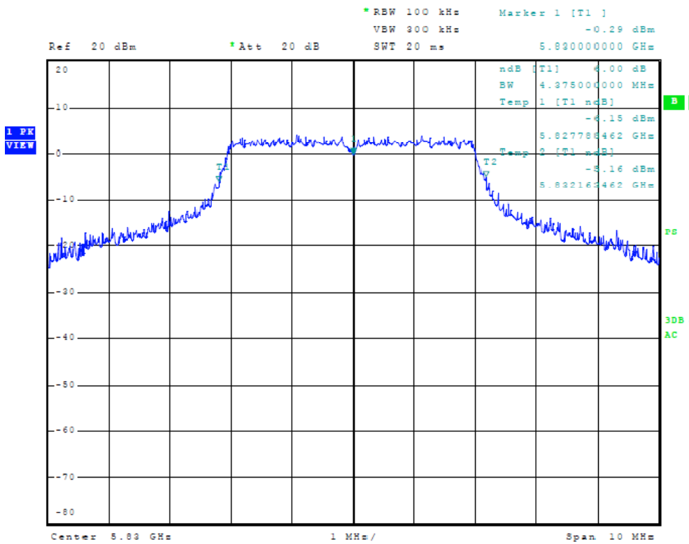
Figure Thirty-five Plot of Plot of 6dB Band width (chain 2, 5 MHz Mode, 5830 MHz)
