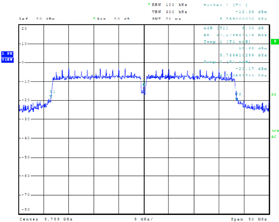
Figure Thirty-nine Plot of 6dB Band width (chain 2, 40 MHz Mode, 5755 MHz)
