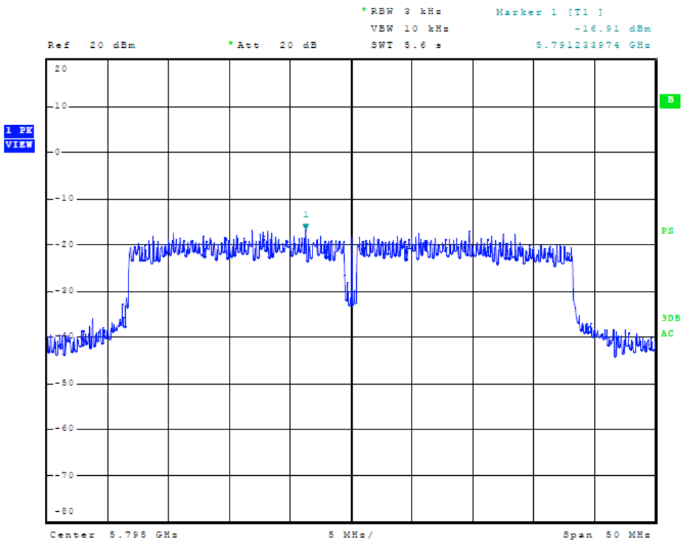
Figure Thirty-one Plot of Power Spectral Density (chain 1, 40 MHz Mode, 5795 MHz)
