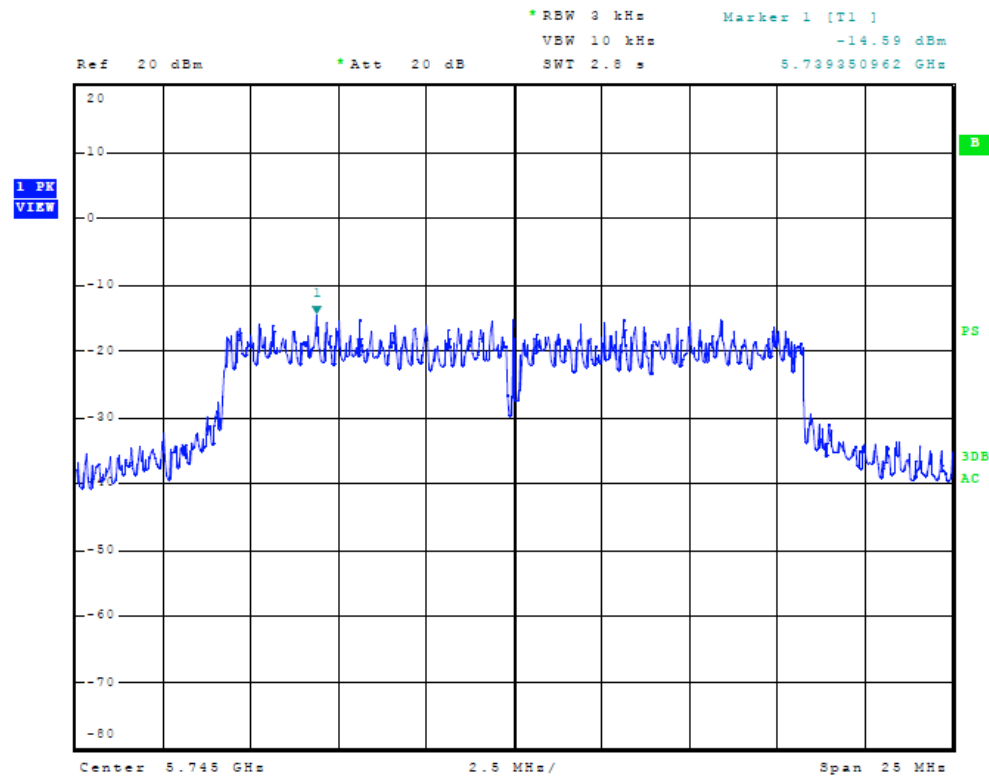
Figure Forty-five Plot of Power Spectral Density (chain 2, 20 MHz Mode, 5745 MHz)
