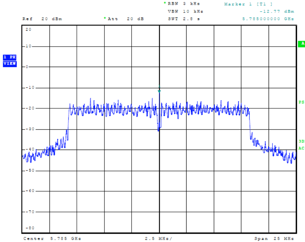
Figure Twenty-eight Plot of Power Spectral Density (chain 1, 20 MHz Mode, 5785 MHz)
