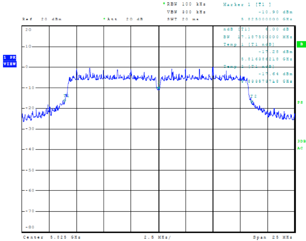
Figure Thirty-eight Plot of 6dB Band width (chain 2, 20 MHz Mode, 5825 MHz)
