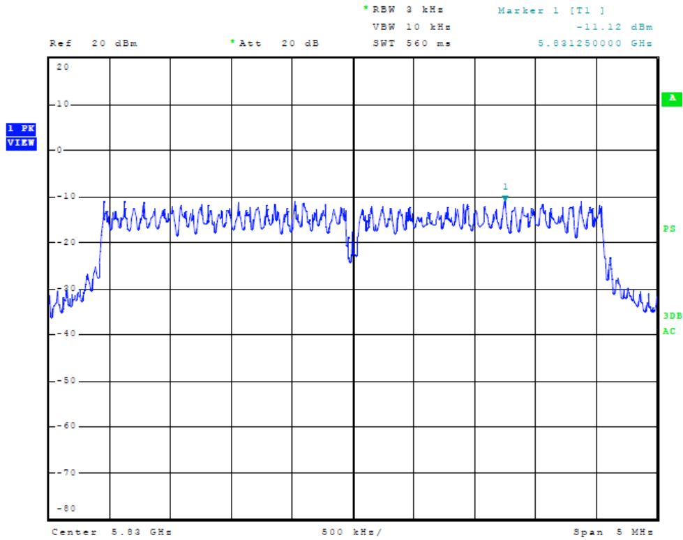
Figure Twenty-six Plot of Power Spectral Density (chain 1, 5 MHz Mode, 5830 MHz)
