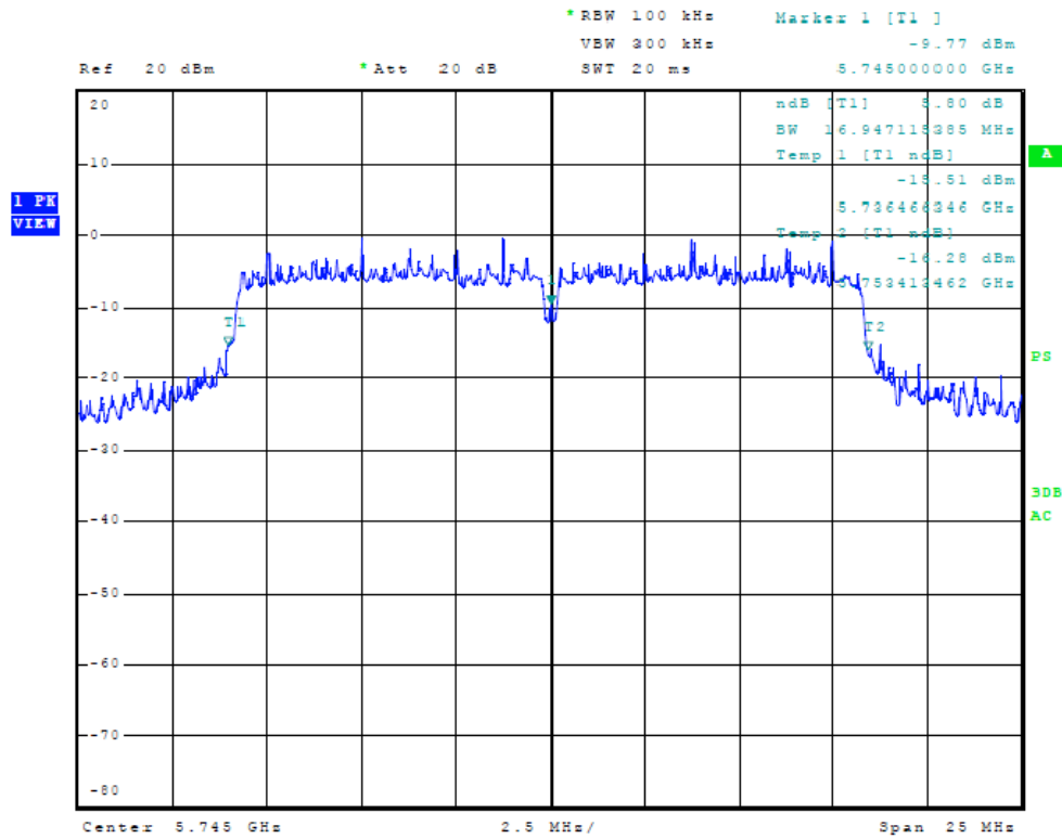
Figure Eighteen Plot of 6dB Band width (chain 1, 20 MHz Mode, 5745 MHz)
