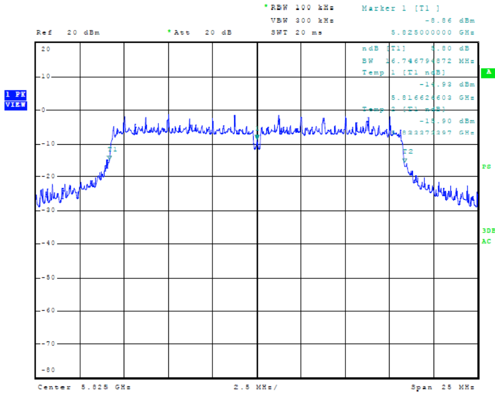
Figure Twenty Plot of 6dB Band width (chain 1, 20 MHz Mode, 5825 MHz)
