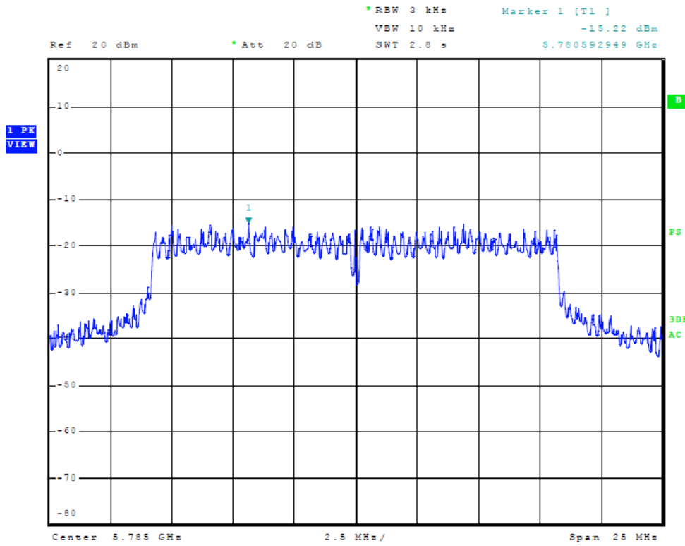
Figure Forty-six Plot of Power Spectral Density (chain 1, 20 MHz Mode, 5785 MHz)
