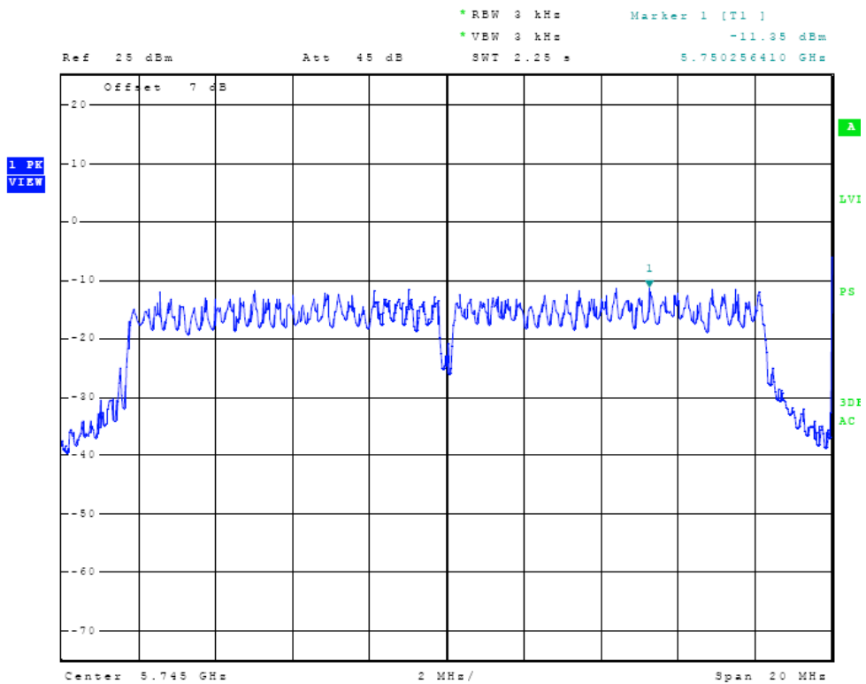
Figure Twenty-six Plot of Power Spectral Density (5745 MHz, 802.11)
