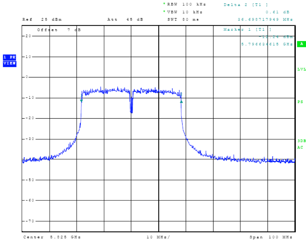
Figure Twenty-five Plot of 6dB Band width (5825 MHz, n mode)
