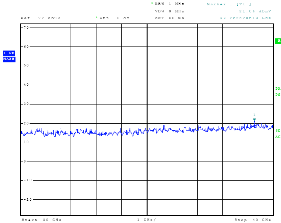
Figure Eleven General Radiated Emissions taken at 1 meter in screen room
