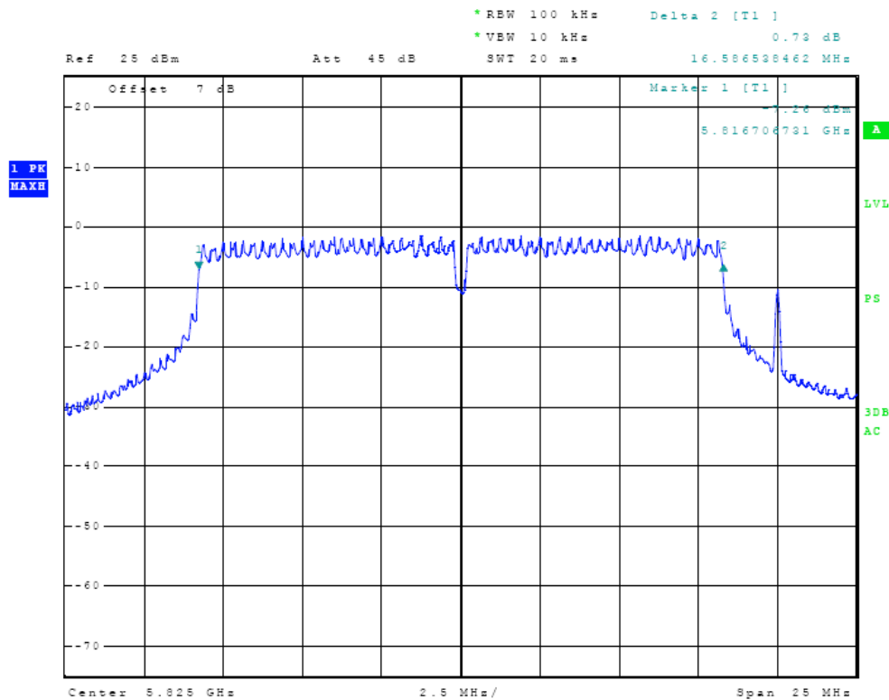
Figure Twenty-four Plot of 6dB Band width (5825 MHz, 802.11 mode)
