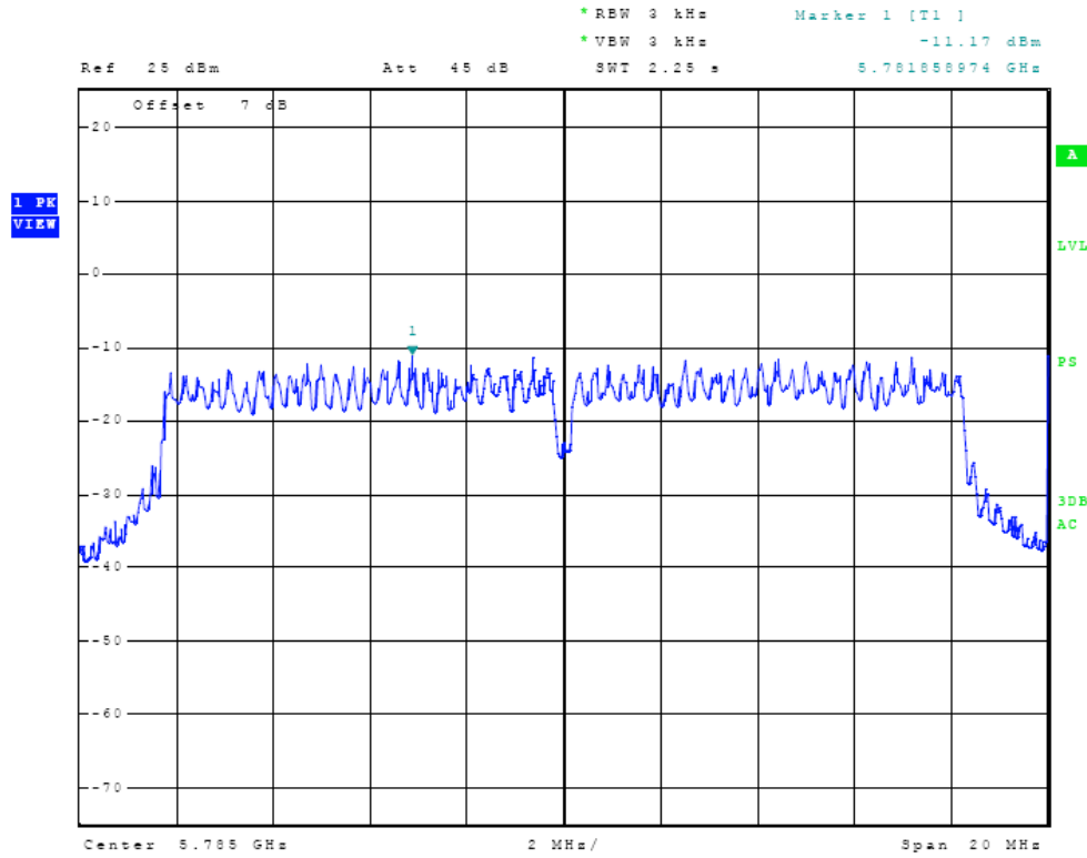
Figure Twenty-seven Plot of Power Spectral Density (5785 MHz, 802.11)
