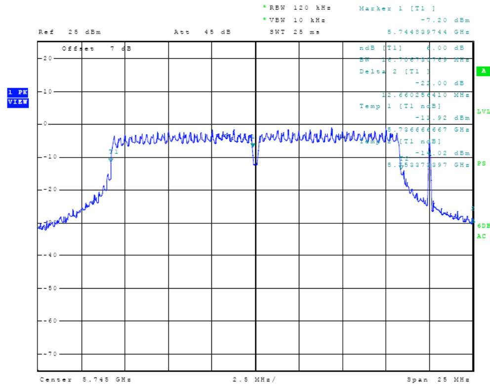
Figure Twenty Plot of 6dB Band width (5745 MHz, 802.11)
