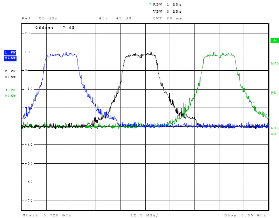
Figure Eighteen Plot of Output Across Operational Band
