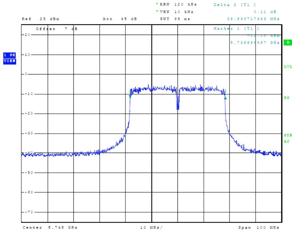
Figure Twenty-one Plot of 6dB Band width (5745 MHz, n mode)
