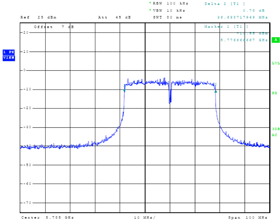
Figure Twenty-three Plot of 6dB Band width (5785 MHz, n mode)
