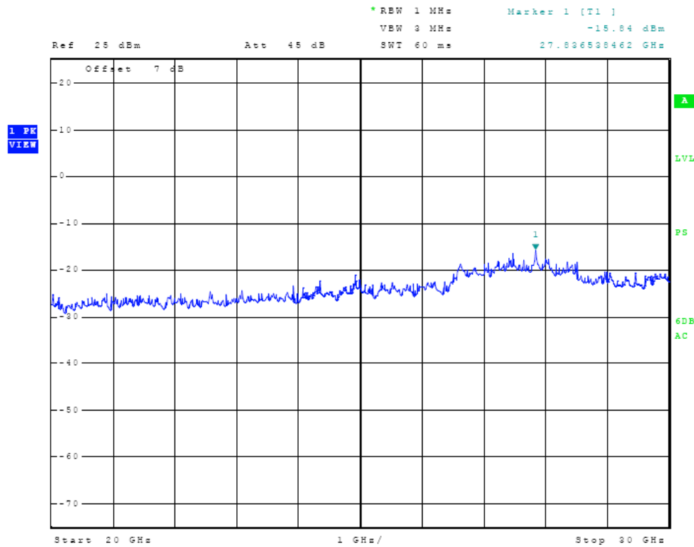
Figure Fifteen Plot of Power Antenna Port Conducted Emissions
