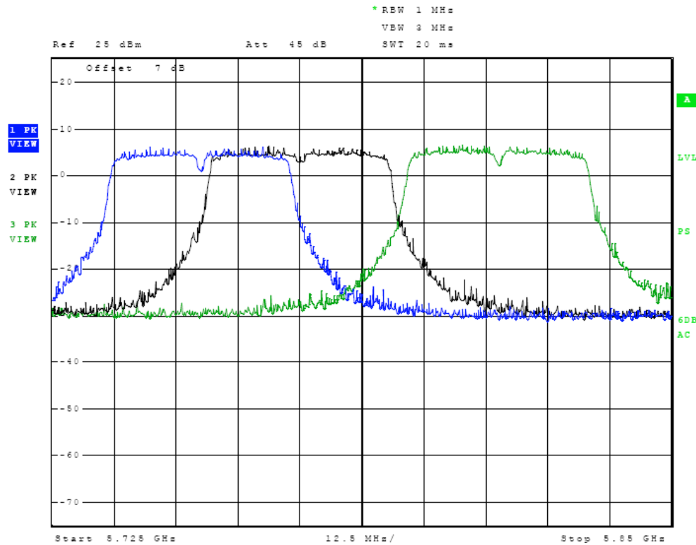
Figure Nineteen Plot of Output Across Operational Band (n mode)
