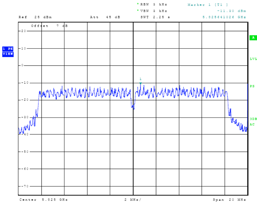
Figure Twenty-eight Plot of Power Spectral Density (5825 MHz, 802.11)
