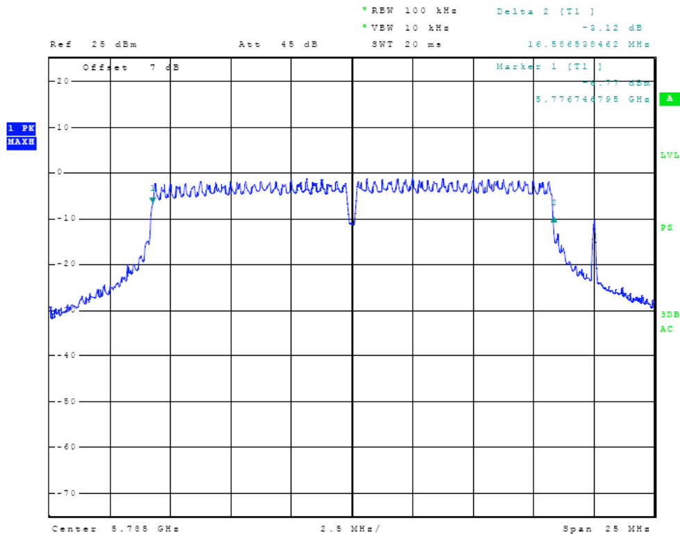
Figure Twenty-two Plot of 6dB Band width (5785 MHz, 802.11 mode)
