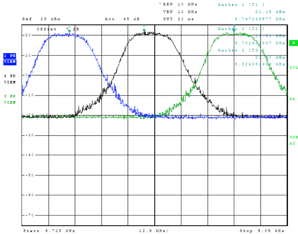
Figure Seventeen Plot of Output Across Operational Band
