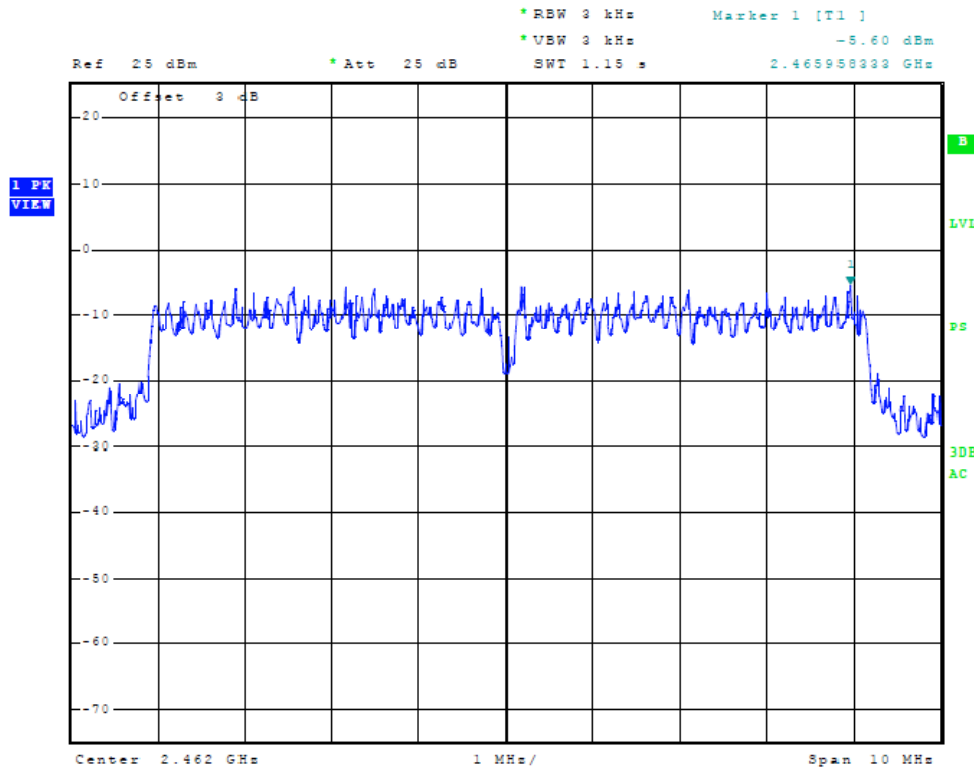
Figure Thirty-seven Plot of Power Spectral Density (10-MHz Mode, 2462 MHz)
