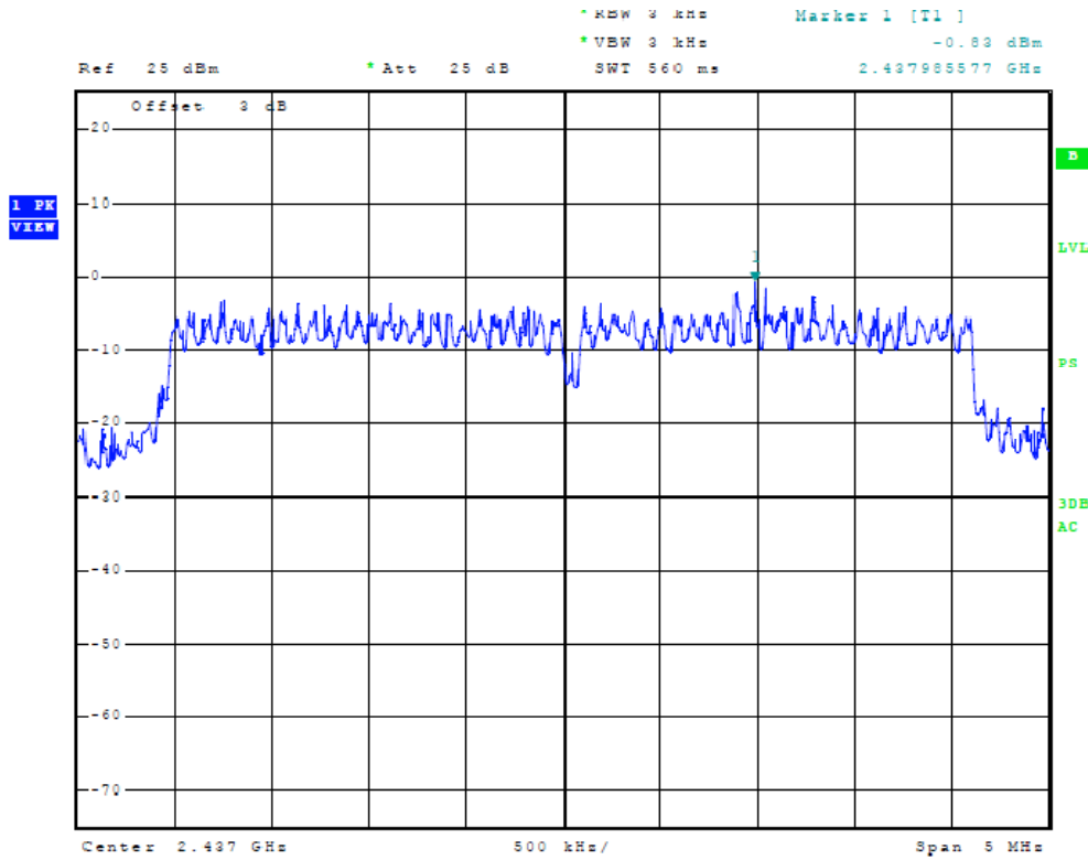
Figure Thirty-three Plot of Power Spectral Density (5-MHz Mode, 2437 MHz)
