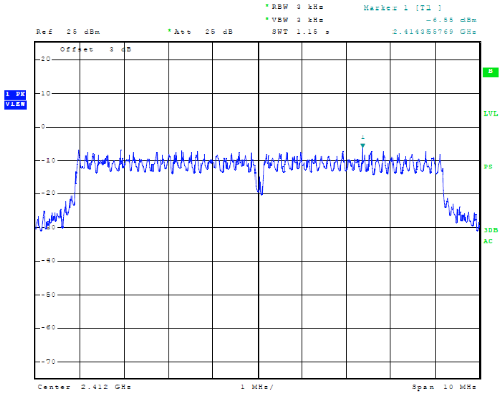
Figure Thirty-five Plot of Power Spectral Density (10-MHz Mode, 2412 MHz)
