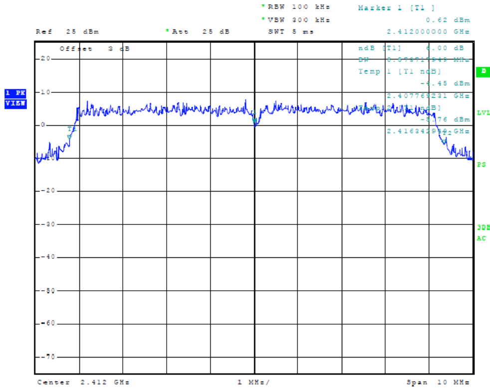
Figure Twenty-six Plot of 6dB Band width (10-MHz Mode, 2412 MHz)
