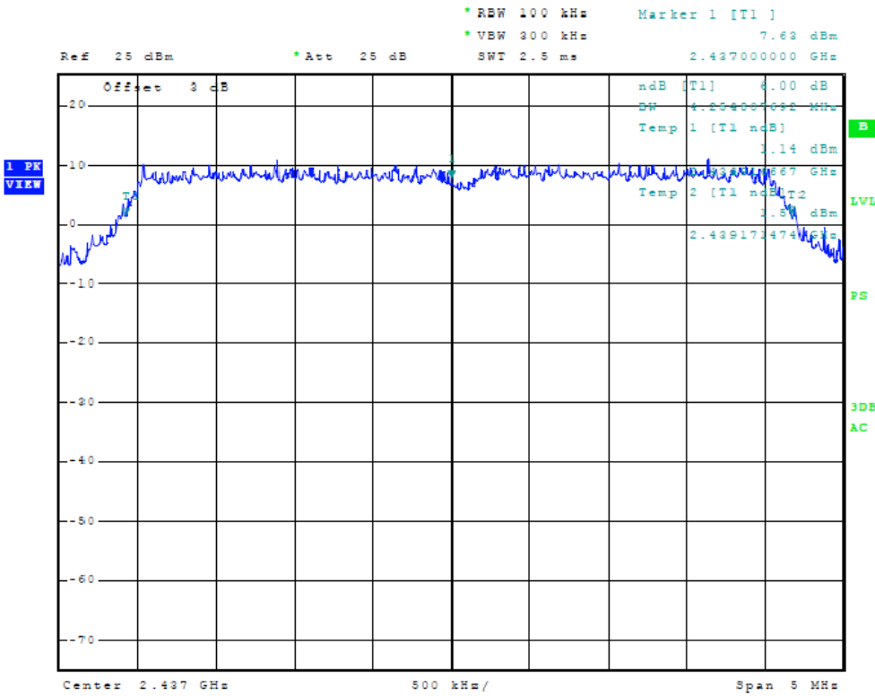
Figure Twenty-seven Plot of 6dB Band width (5-MHz Mode, 2437 MHz)
