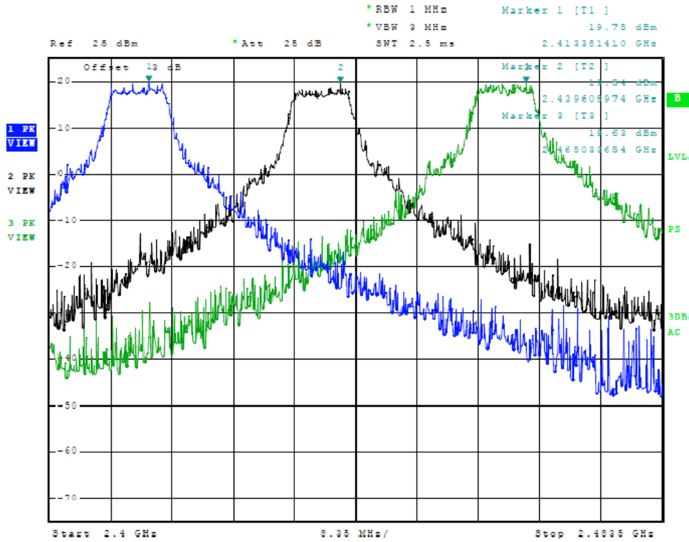
Figure Nineteen Plot of Output Across Operational Band (10-MHz mode)
