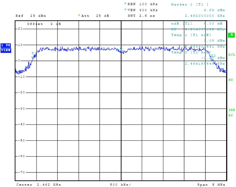
Figure Twenty-eight Plot of 6dB Band width (5-MHz Mode, 2462 MHz)
