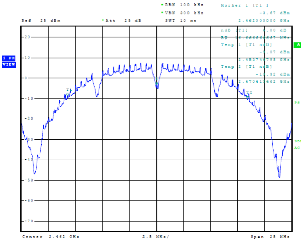
Figure Twenty-two Plot of 6dB Band width (B-Mode, 2462 MHz)
