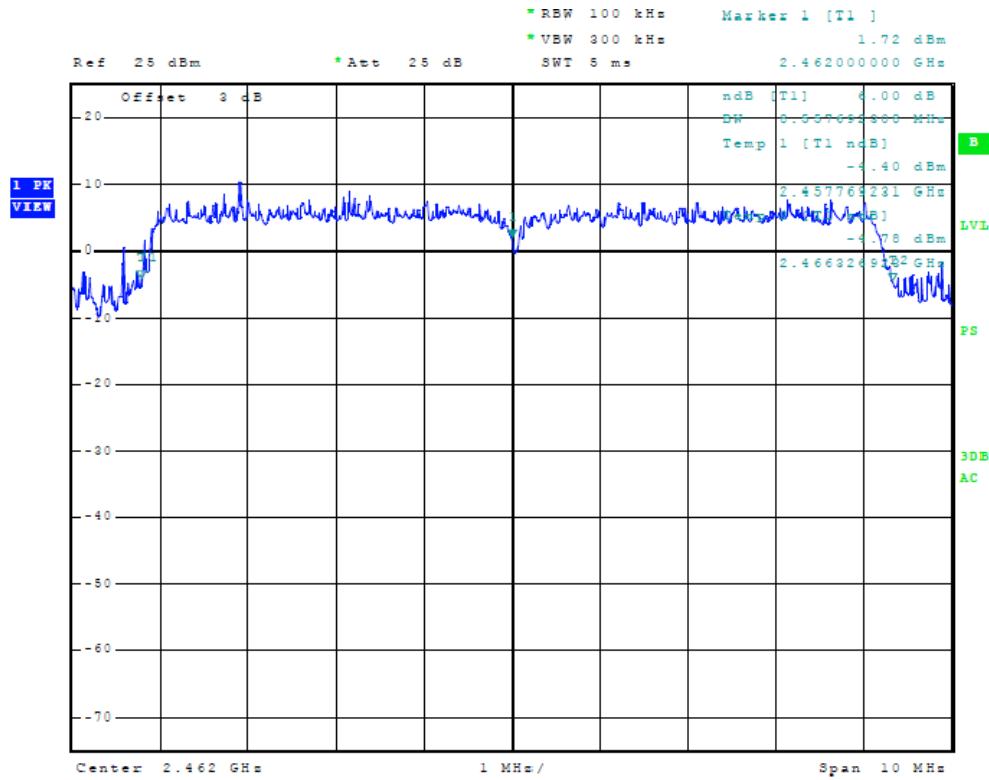
Figure Twenty-eight Plot of 6dB Band width (10-MHz Mode, 2462 MHz)
