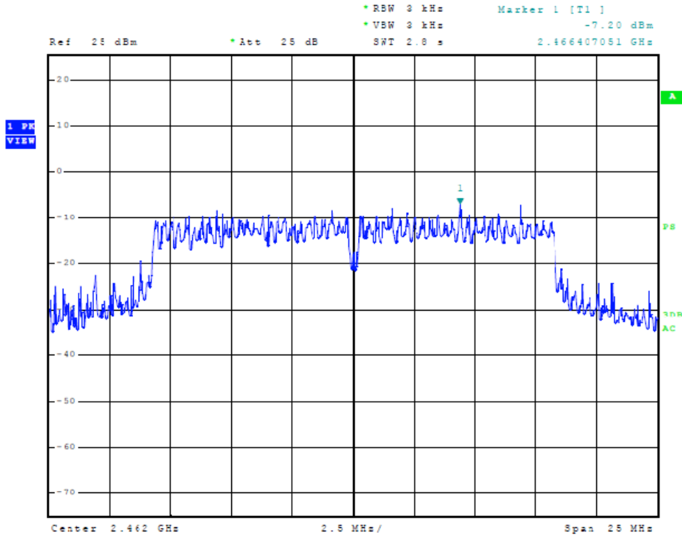
Figure Thirty-one Plot of Power Spectral Density (G-Mode, 2462 MHz)
