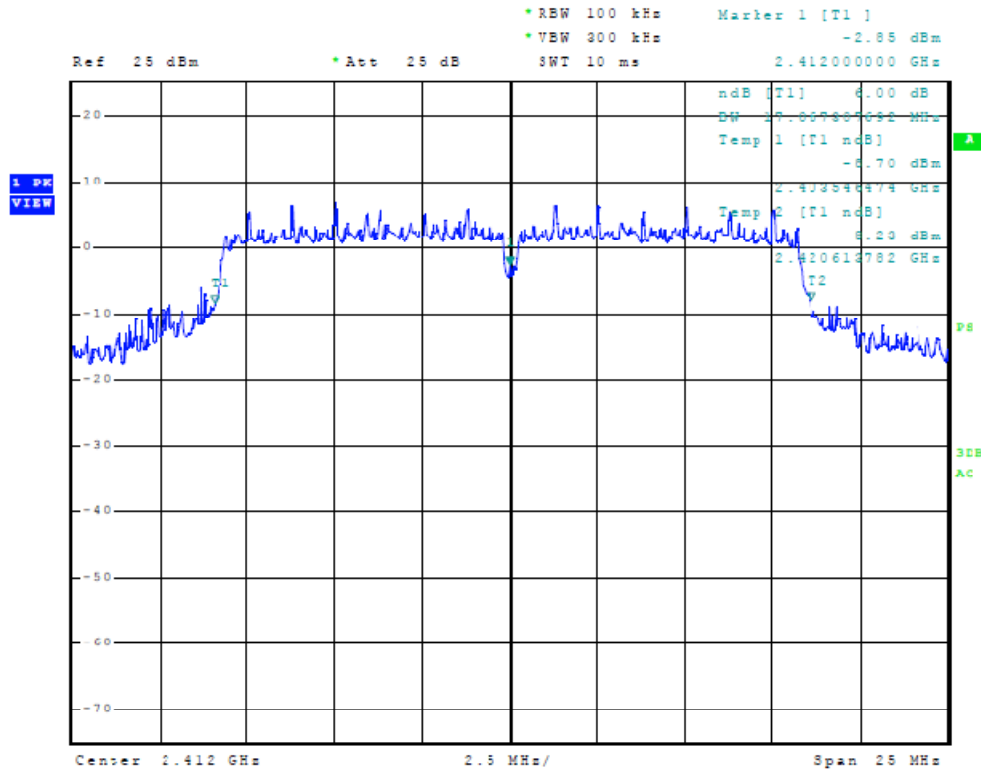
Figure Twenty-three Plot of 6dB Band width (G-Mode, 2412 MHz)
