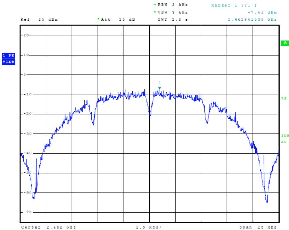
Figure Twenty-eight Plot of Power Spectral Density (B-Mode, 2462 MHz)
