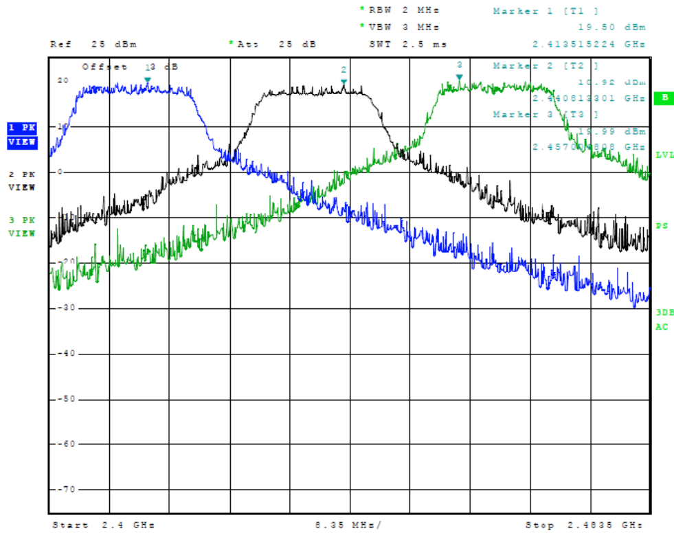
Figure Seventeen Plot of Output Across Operational Band (G-Mode)
