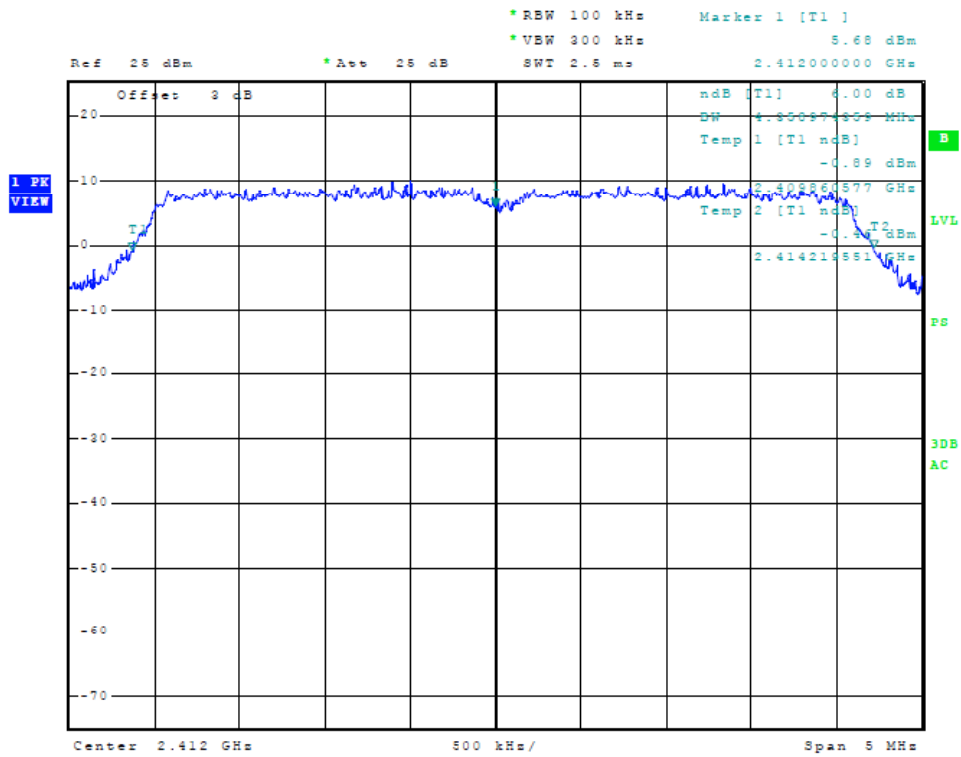
Figure Twenty-six Plot of 6dB Band width (5-MHz Mode, 2412 MHz)
