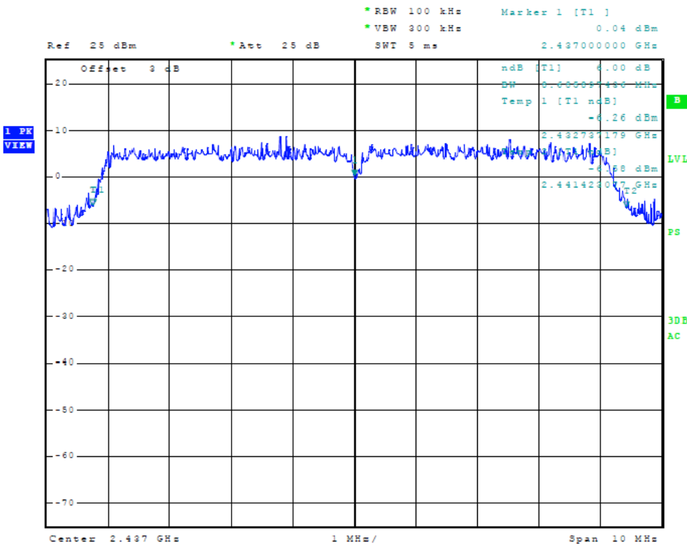
Figure Twenty-seven Plot of 6dB Band width (10-MHz Mode, 2437 MHz)
