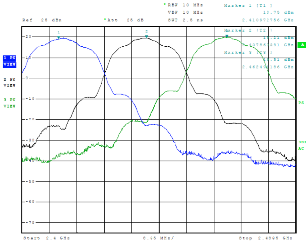
Figure Sixteen Plot of Output Across Operational Band (B-Mode)
