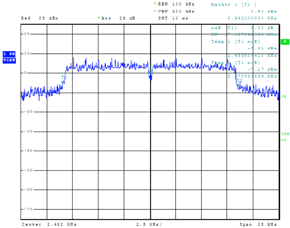
Figure Twenty-five Plot of 6dB Band width (G-Mode, 2462 MHz)
