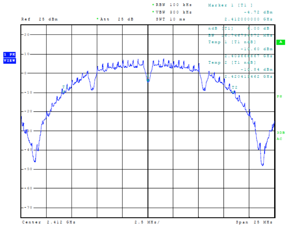
Figure Twenty Plot of 6dB Band width (B-Mode, 2412 MHz)
