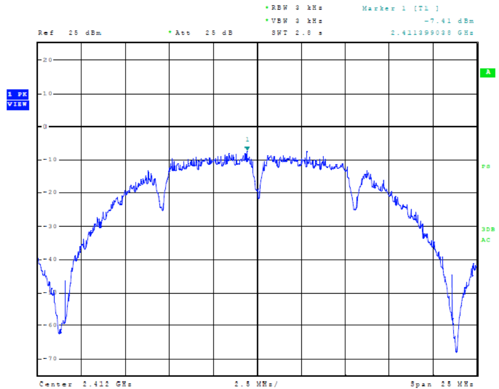
Figure Twenty-six Plot of Power Spectral Density (B-Mode, 2412 MHz)
