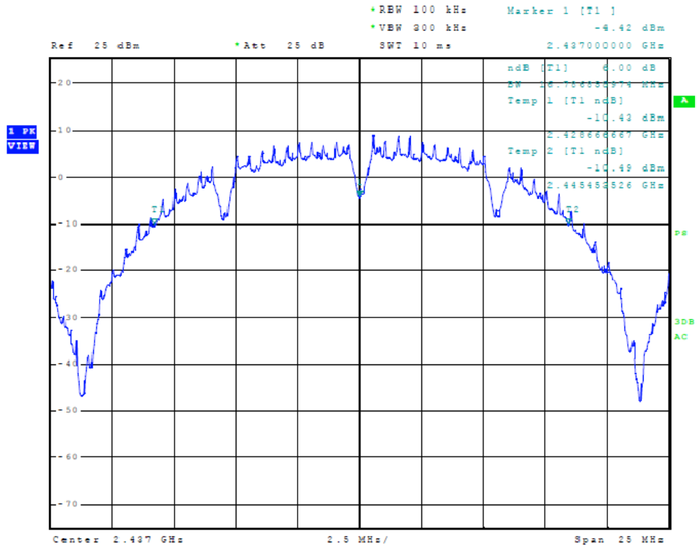
Figure Twenty-one Plot of 6dB Band width (B-Mode, 2437 MHz)
