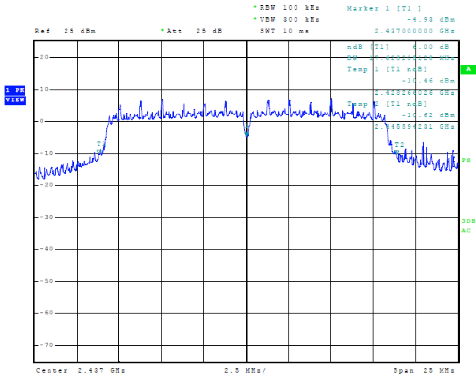
Figure Twenty-four Plot of 6dB Band width (G-Mode, 2437 MHz)
