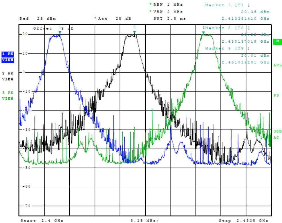
Figure Eighteen Plot of Output Across Operational Band (5-MHz Mode)
