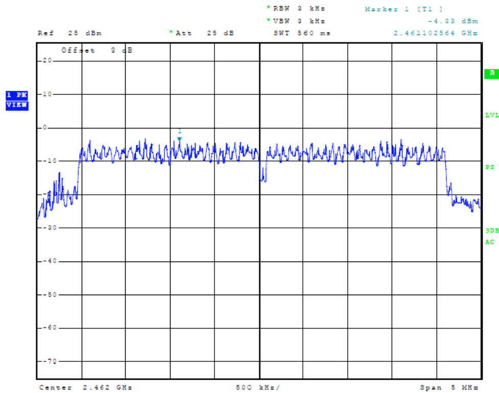
Figure Thirty-four Plot of Power Spectral Density (5-MHz Mode, 2462 MHz)
