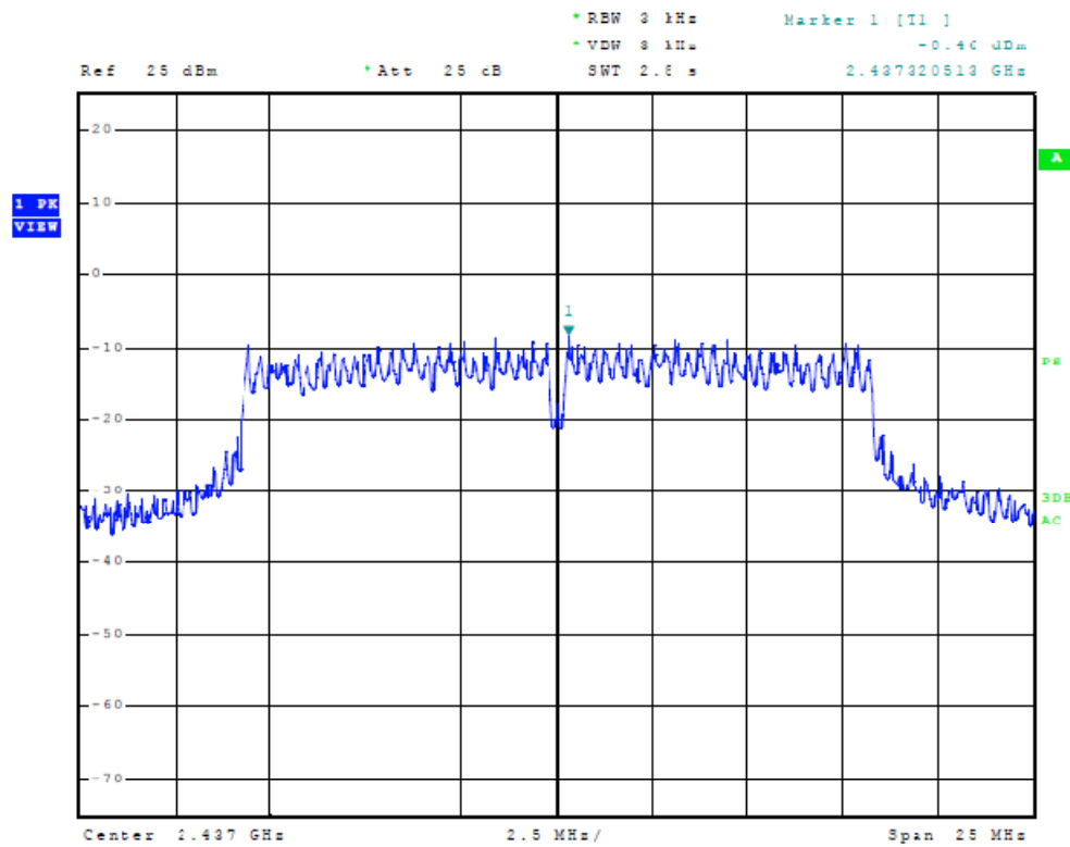
Figure Thirty Plot of Power Spectral Density (G-Mode, 2437 MHz)
