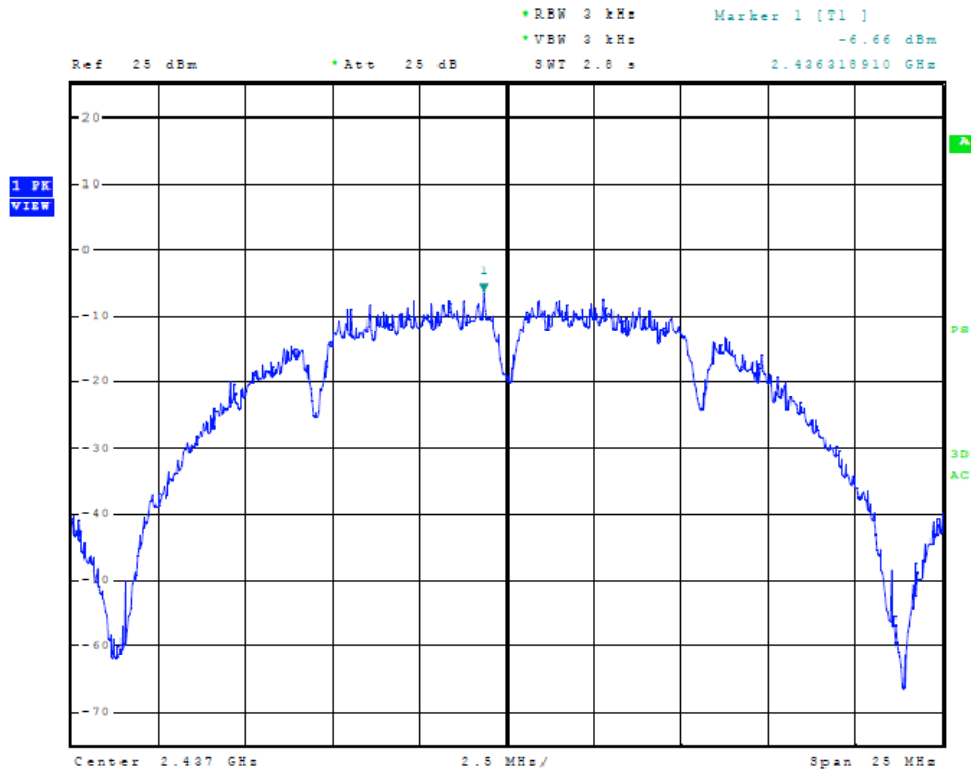
Figure Twenty-seven Plot of Power Spectral Density (B-Mode, 2437 MHz)
