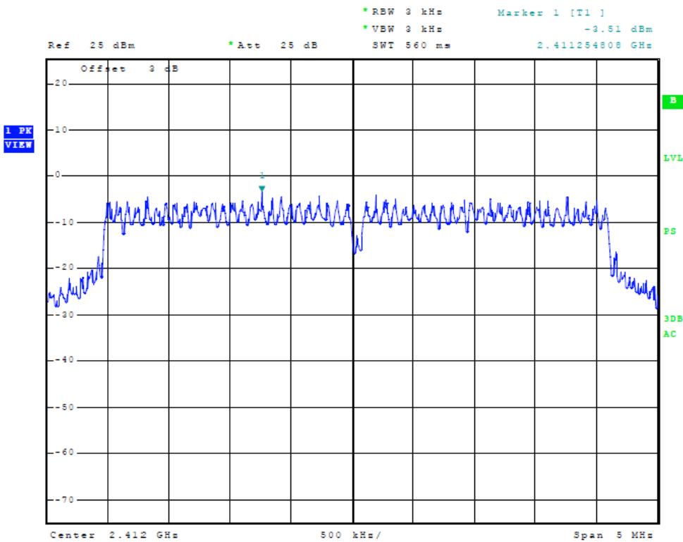
Figure Thirty-two Plot of Power Spectral Density (5-MHz Mode, 2412 MHz)
