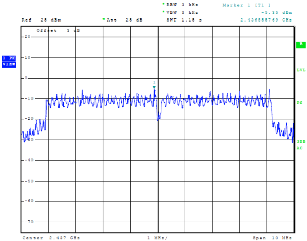
Figure Thirty-six Plot of Power Spectral Density (10-MHz Mode, 2437 MHz)
