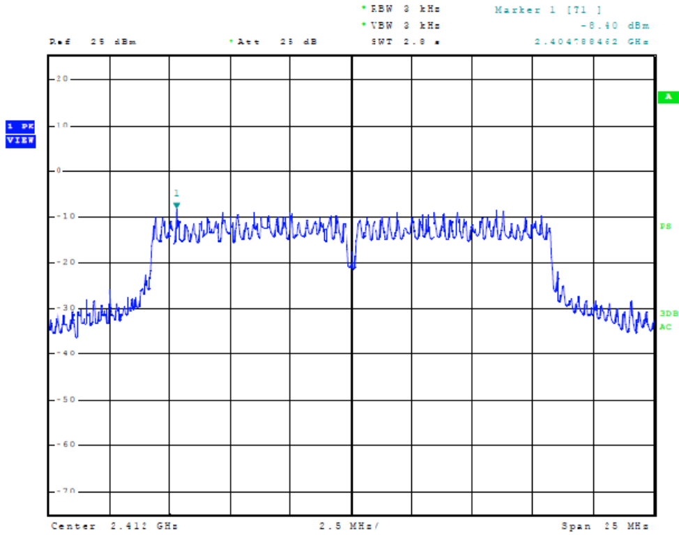
Figure Twenty-nine Plot of Power Spectral Density (G-Mode, 2412 MHz)
