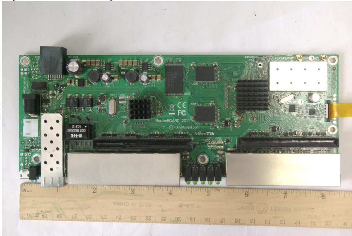
Top side of PCB shields in place
