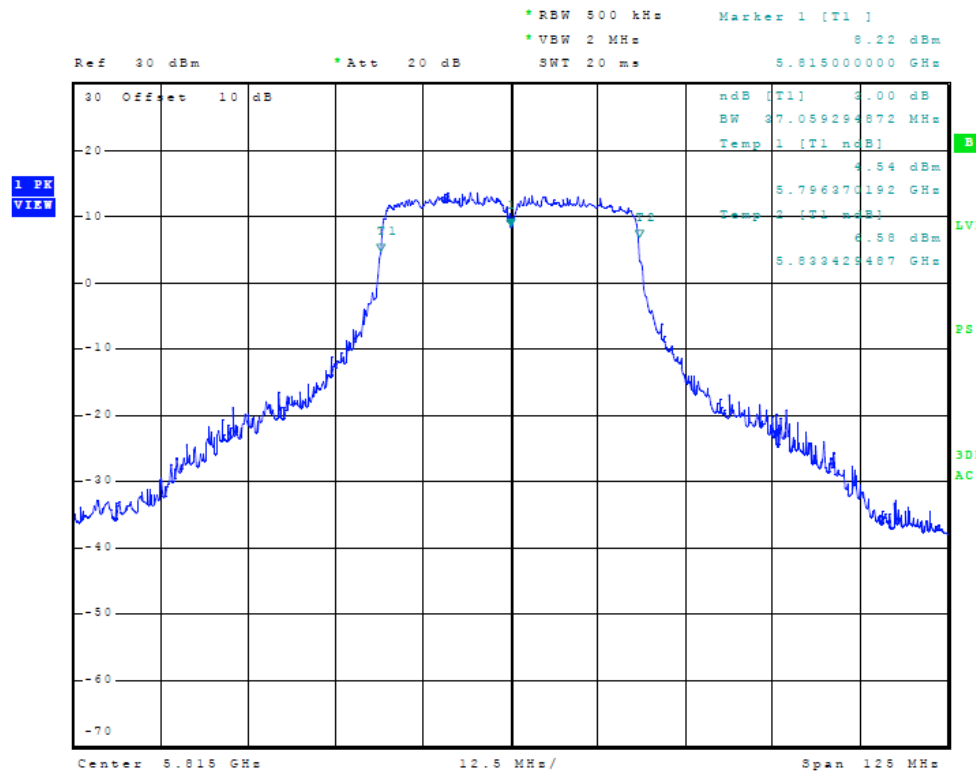
Figure Twenty-seven Plot of 6dB Band width (40 MHz Mode, 5815 MHz)
