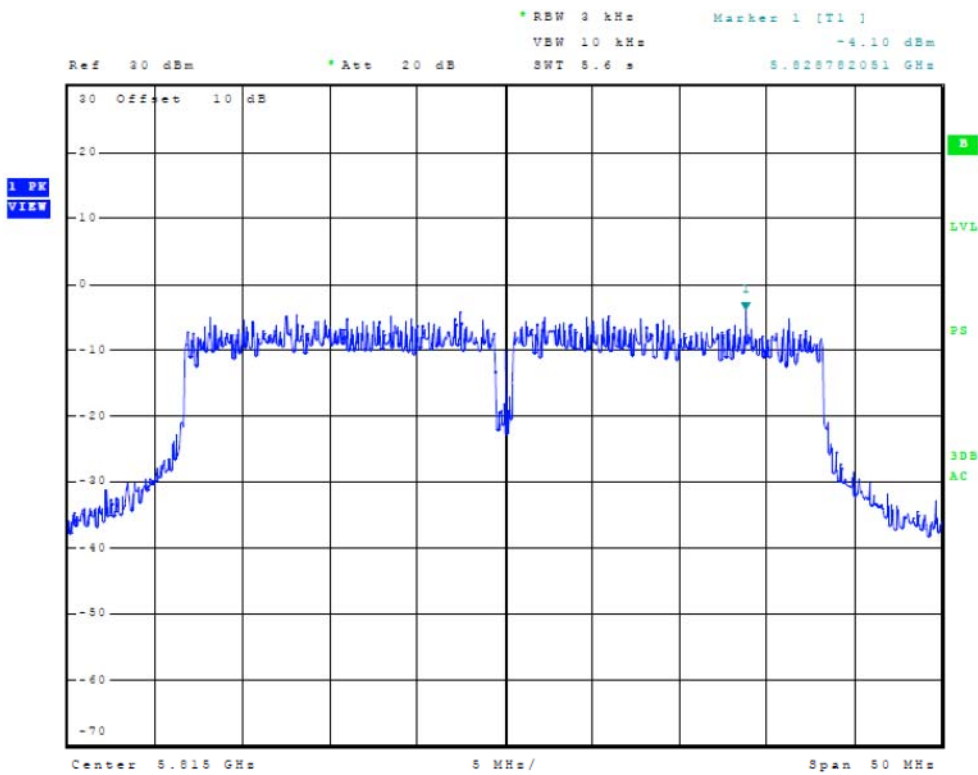
Figure Thirty-nine Plot of Power Spectral Density (40 MHz Mode, 5815 MHz)
