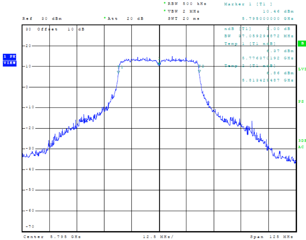
Figure Twenty-six Plot of 6dB Band width (40 MHz Mode, 5795 MHz)
