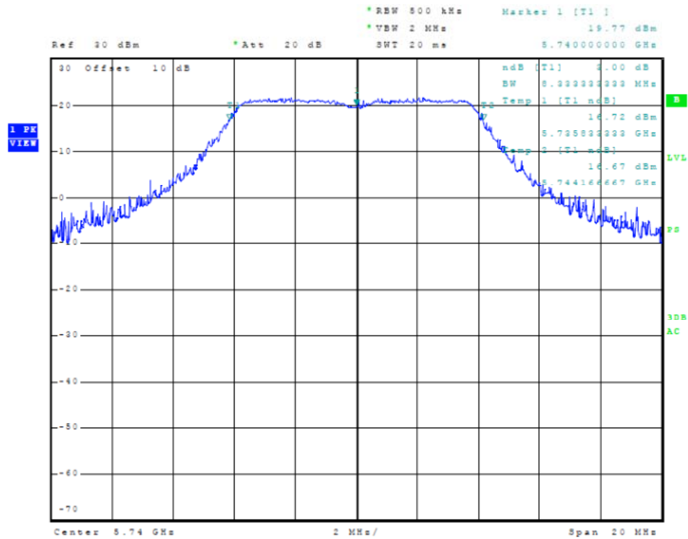
Figure Nineteen Plot of 6dB Band width (10 MHz Mode, 5740 MHz)
