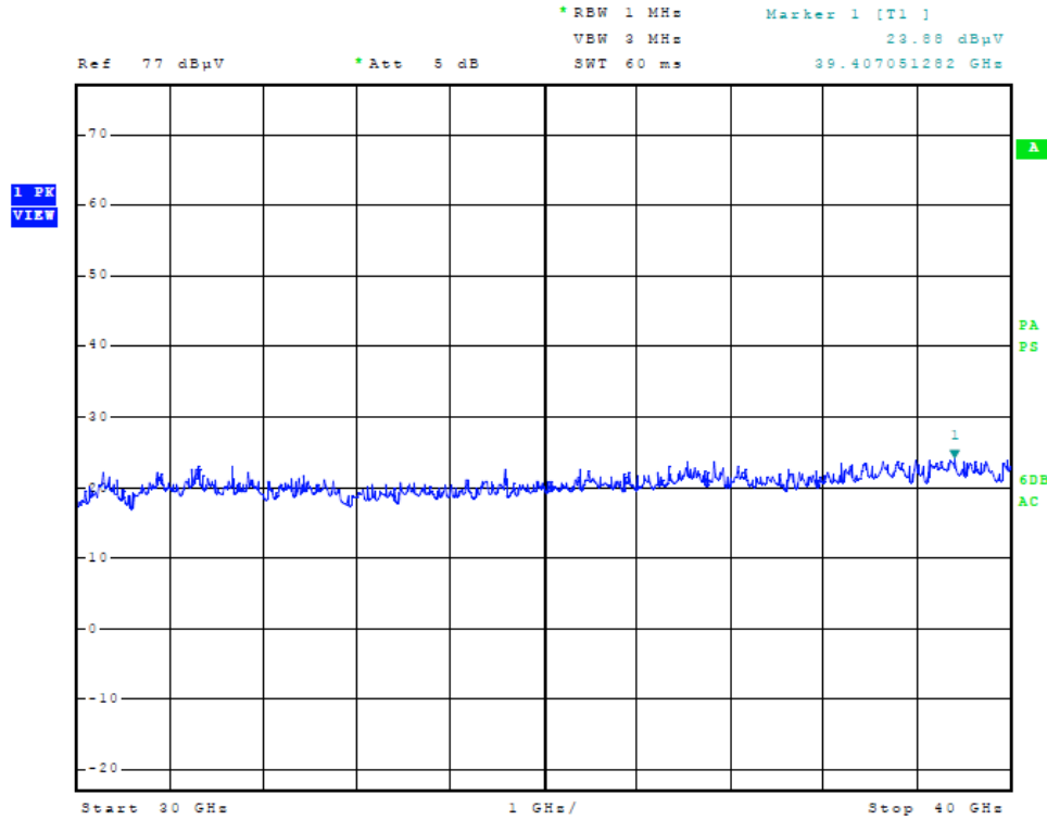
Figure Eleven General Radiated Emissions taken at 1 meter in screen room General Radiated Emissions from EUT Data (Highest Emissions all antenna options)
