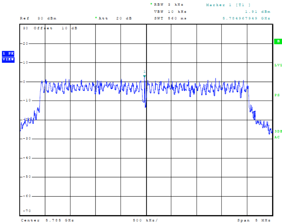
Figure Twenty-nine Plot of Power Spectral Density (5 MHz Mode, 5785 MHz)
