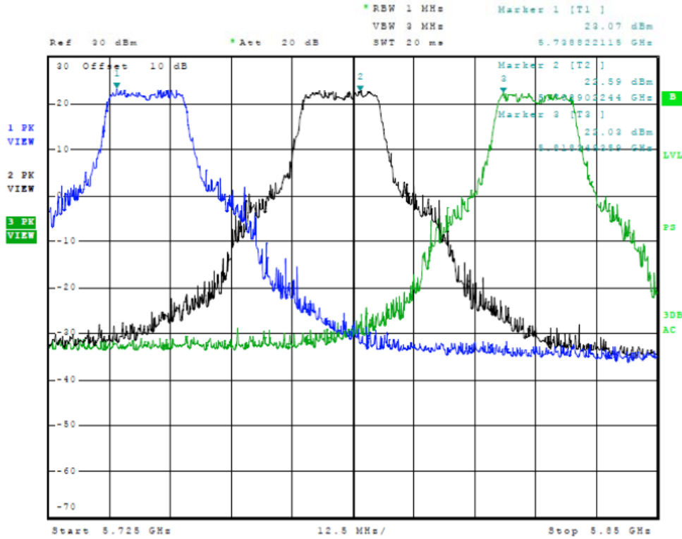
Figure Fourteen Plot of Antenna Port Emissions (Across Operational Band, 20MHz Mode)
