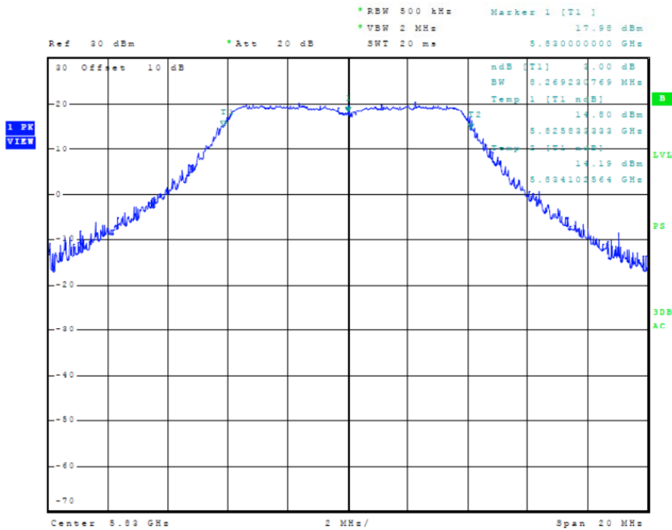
Figure Twenty-one Plot of 6dB Band width (10 MHz Mode, 5830 MHz)
