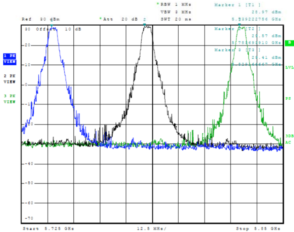
Figure Twelve Plot of Antenna Port Emissions (Across Operational Band, 5MHz Mode)
