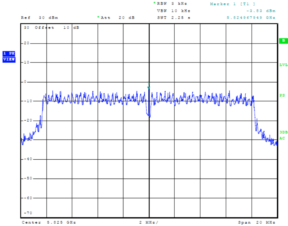
Figure Thirty-six Plot of Power Spectral Density (20 MHz Mode, 5825 MHz)
