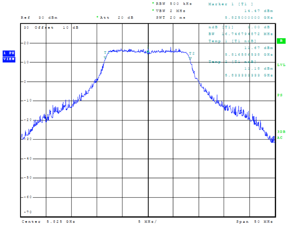
Figure Twenty-four Plot of 6dB Band width (20 MHz Mode, 5825 MHz)
