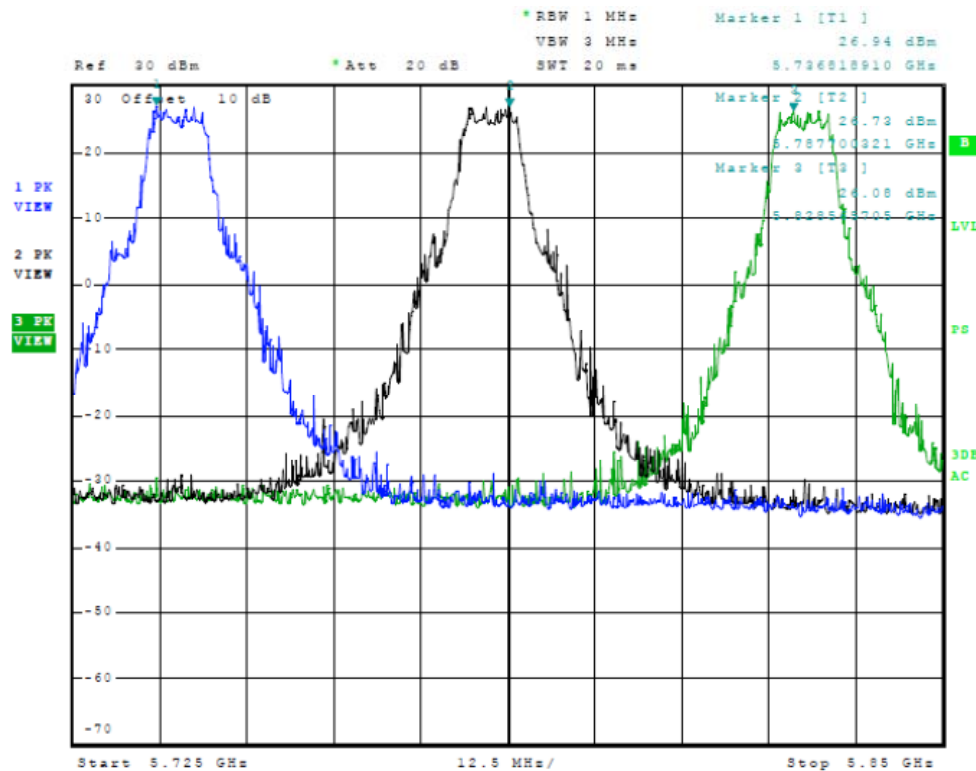
Figure Thirteen Plot of Antenna Port Emissions (Across Operational Band, 10MHz Mode)
