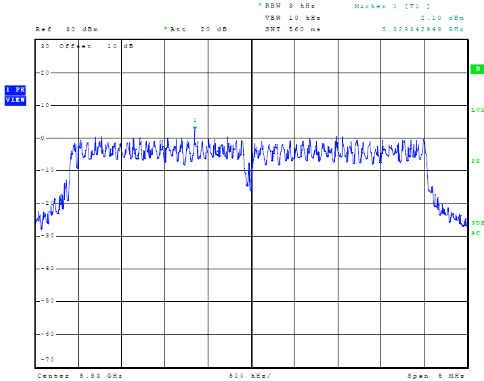
Figure Thirty Plot of Power Spectral Density (5 MHz Mode, 5830 MHz)
