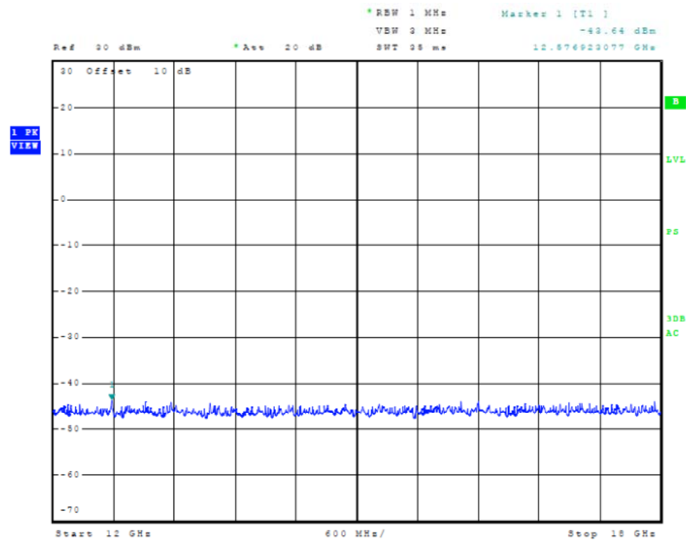
Figure Forty-three Plot of Antenna port conducted emissions
