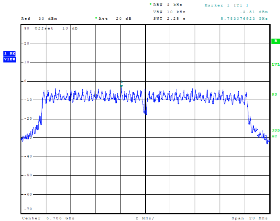
Figure Thirty-five Plot of Power Spectral Density (20 MHz Mode, 5785 MHz)
