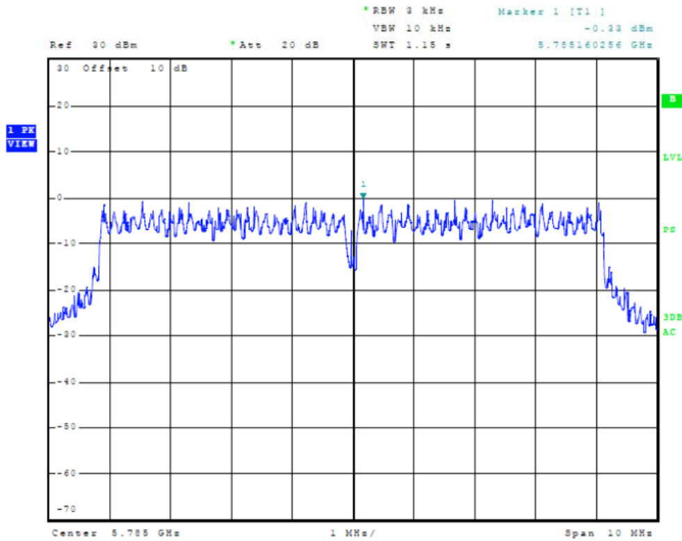
Figure Thirty-two Plot of Power Spectral Density (10 MHz Mode, 5785 MHz)
