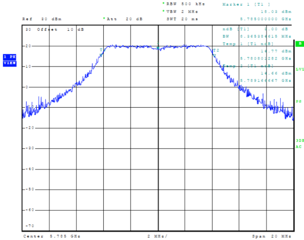
Figure Twenty Plot of 6dB Band width (10 MHz Mode, 5785 MHz)
