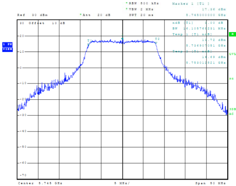
Figure Twenty-two Plot of 6dB Band width (20 MHz Mode, 5745 MHz)
