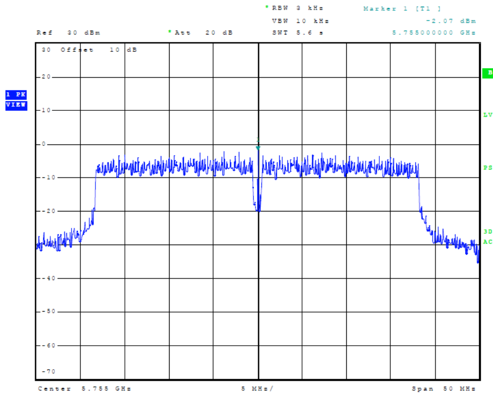
Figure Thirty-seven Plot of Power Spectral Density (40 MHz Mode, 5755 MHz)
