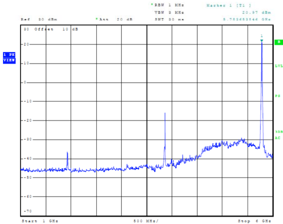
Figure Forty-one Plot of Antenna port conducted emissions
