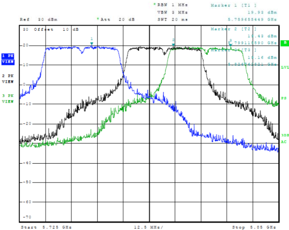
Figure Fifteen Plot of Antenna Port Emissions (Across Operational Band, 40MHz Mode)
