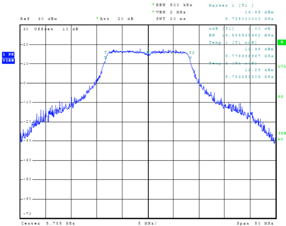
Figure Twenty-three Plot of 6dB Band width (20 MHz Mode, 5785 MHz)
