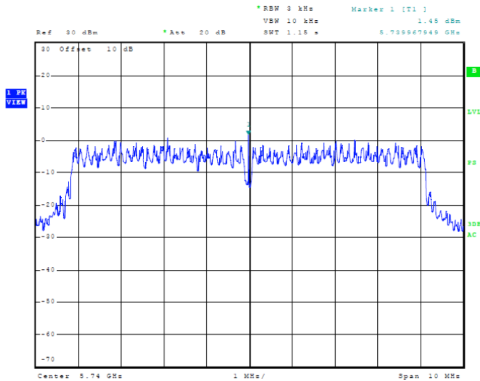
Figure Thirty-one Plot of Power Spectral Density (10 MHz Mode, 5740 MHz)
