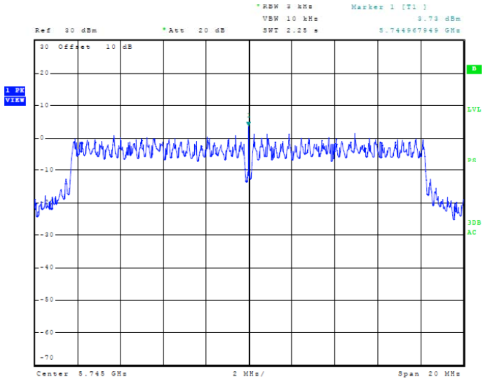
Figure Thirty-four Plot of Power Spectral Density (20 MHz Mode, 5745 MHz)
