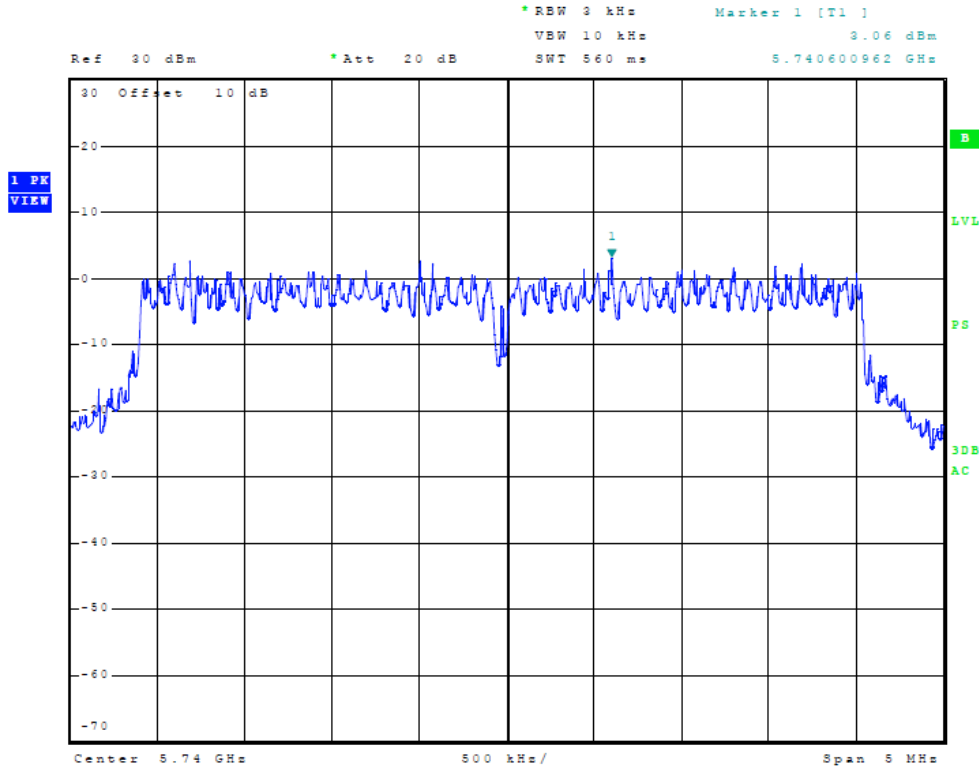
Figure Twenty-eight Plot of Power Spectral Density (5 MHz Mode, 5740 MHz)
