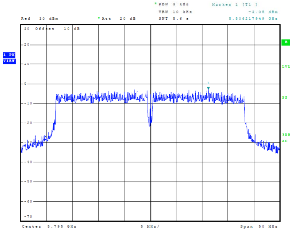
Figure Thirty-eight Plot of Power Spectral Density (40 MHz Mode, 5795 MHz)
