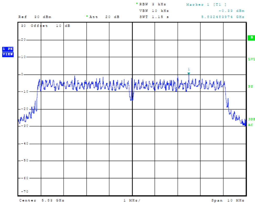
Figure Thirty-three Plot of Power Spectral Density (10 MHz Mode, 5830 MHz)
