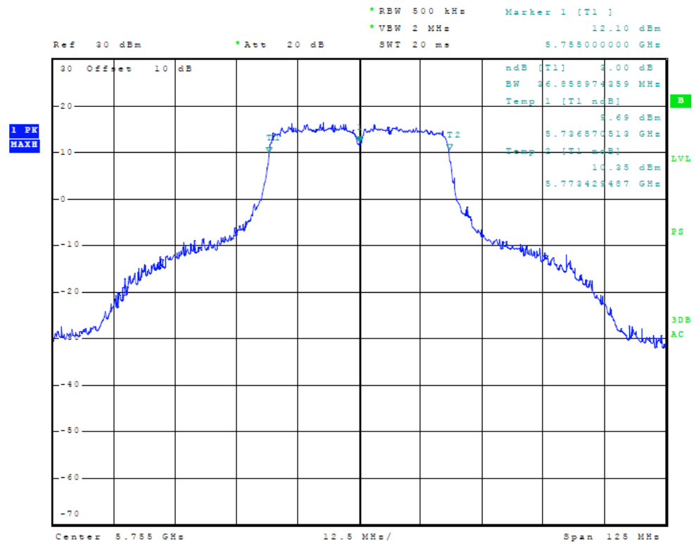
Figure Twenty-five Plot of 6dB Band width (40 MHz Mode, 5755 MHz)
