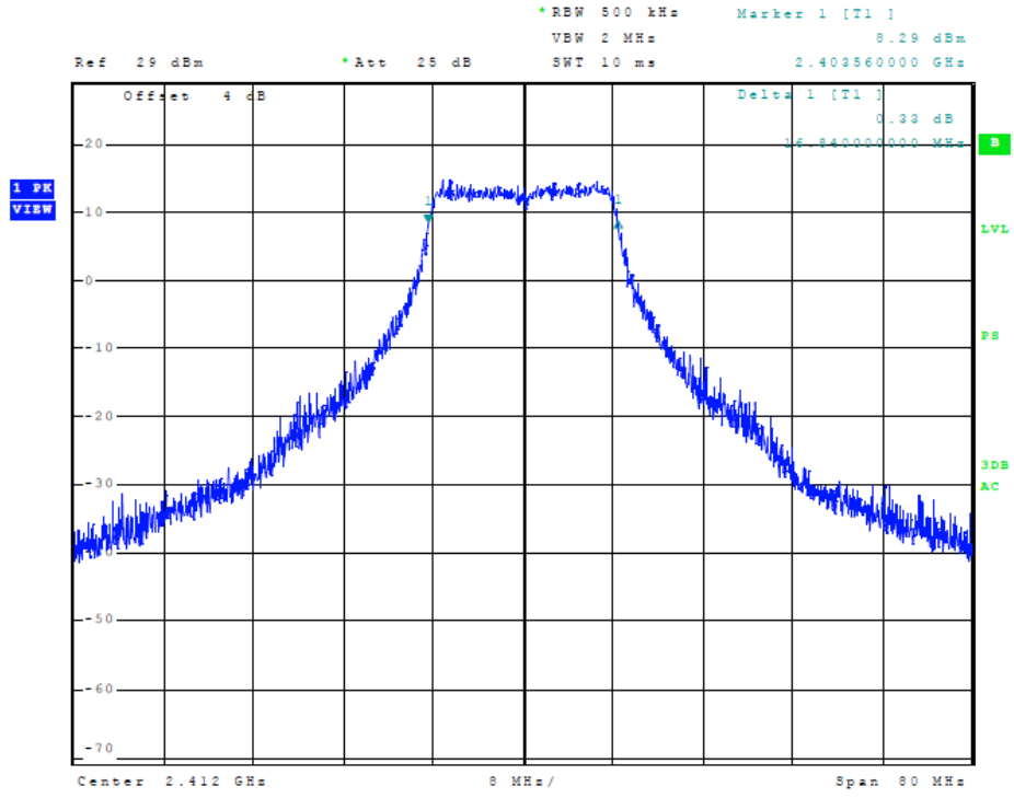
Figure 17 Plot of Transmitter 6-dB Occupied Band Width (802.11n, (HT20) Chain 0)
