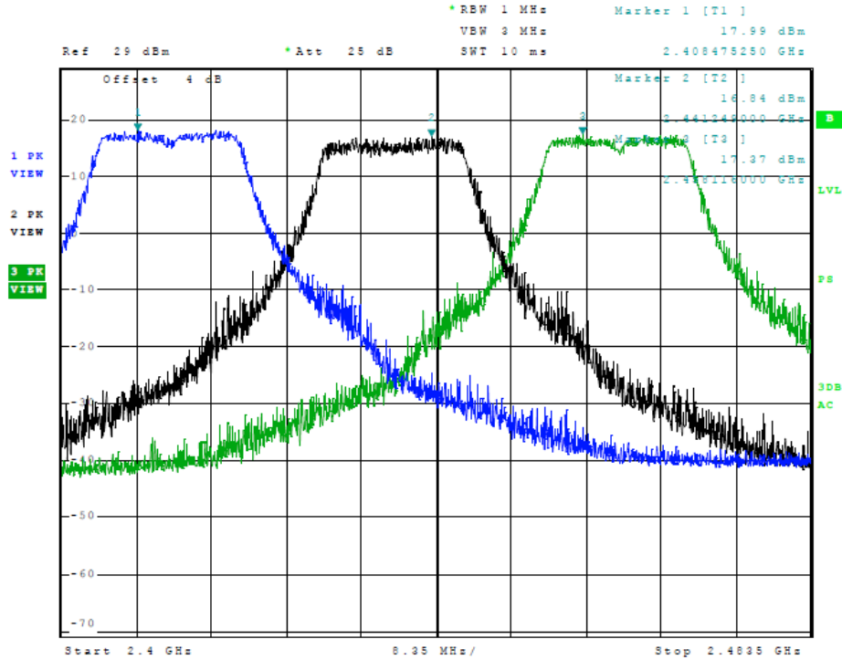
Figure 5 Plot of Transmitter Emissions (Across Operational Band, 802.11n (HT20), Chain 0)
