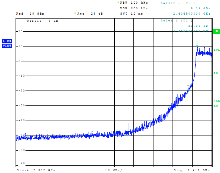
Figure 9 Plot of Transmitter Low Band Edge (802.11n (HT20), Chain 0)
