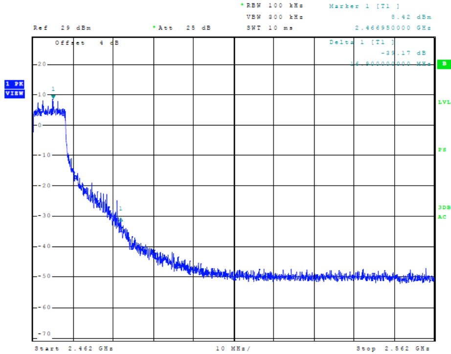
Figure 13 Plot of Transmitter High Band Edge (802.11n (HT20), Chain 0)
