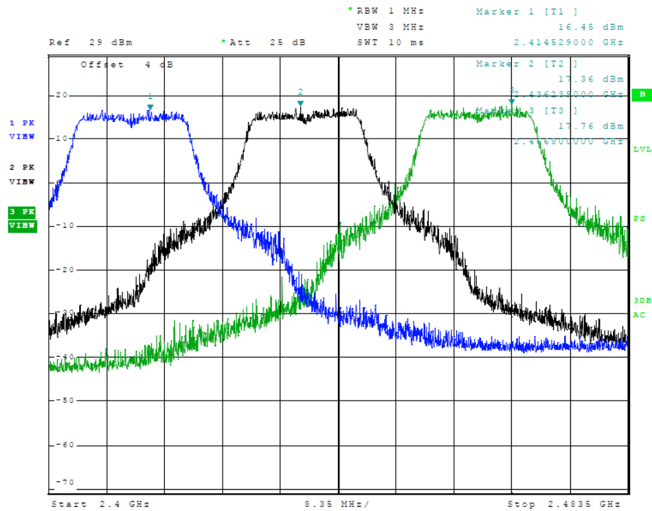
Figure 20 Plot of Transmitter Emissions (Across Operational Band, 802.11g, Chain 1)
