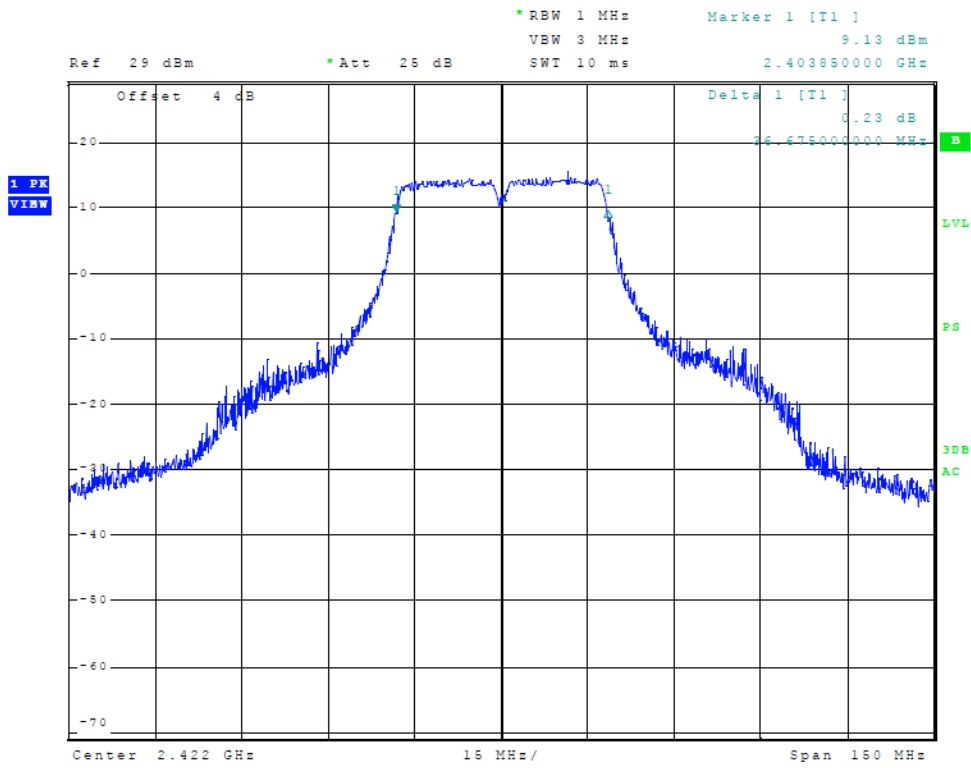
Figure 18 Plot of Transmitter 6-dB Occupied Band Width (802.11n (40), Chain 0)
