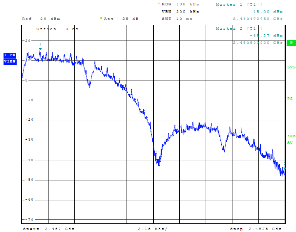
Figure 7 Plot of High Band Edge (b/g/n Mode)
