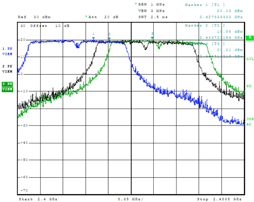
Figure 4 Plot of Transmitter Emissions (Across Operational Band, n Mode)
