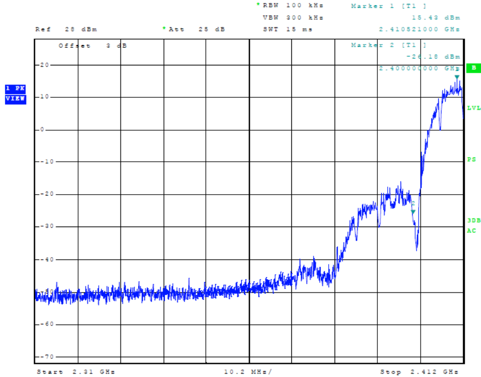
Figure 5 Plot of Low Band Edge (b/g/n Mode)
