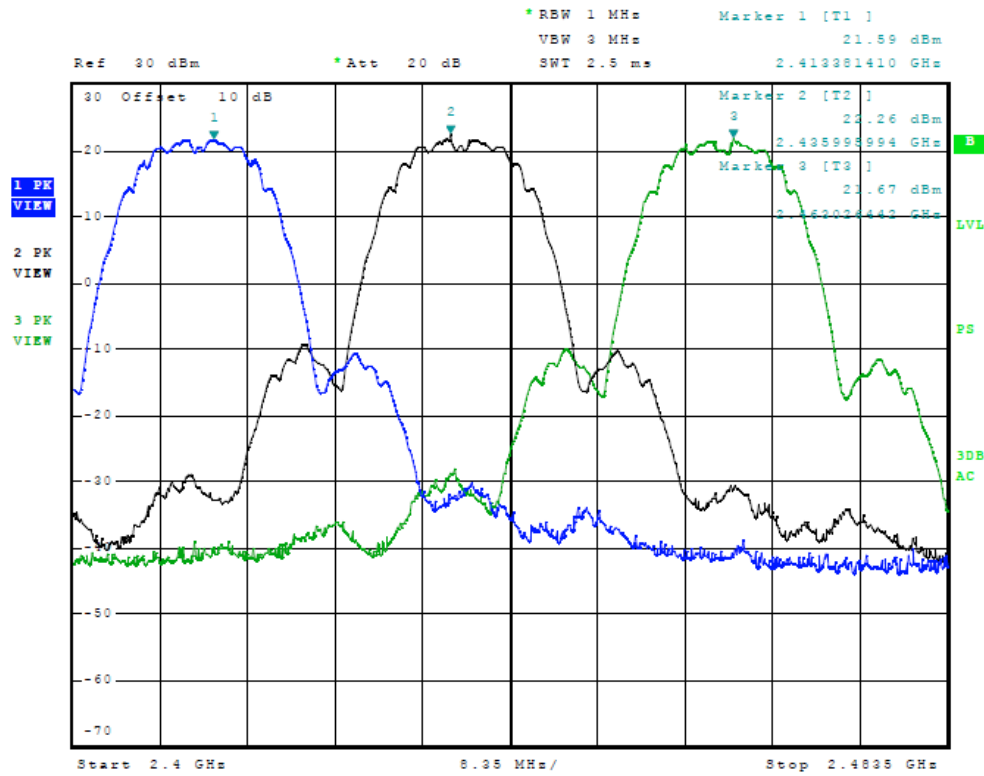
Figure 3 Plot of Transmitter Emissions (Across Operational Band, b/g/n Mode)
