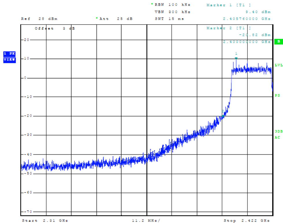
Figure 6 Plot of Low Band Edge (n Mode)
