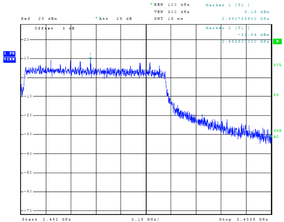
Figure 8 Plot of High Band Edge (n Mode)
