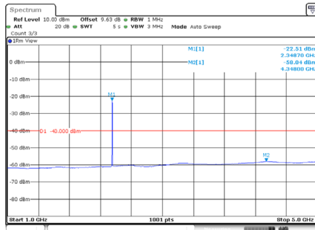
Band40_5MHz_QPSK_38725_25RB#0
