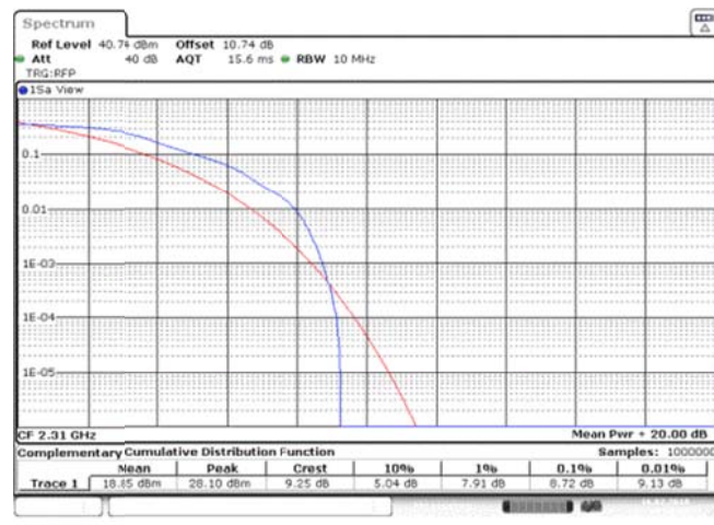
Band40_5MHz_QPSK_38750_1RB#0
