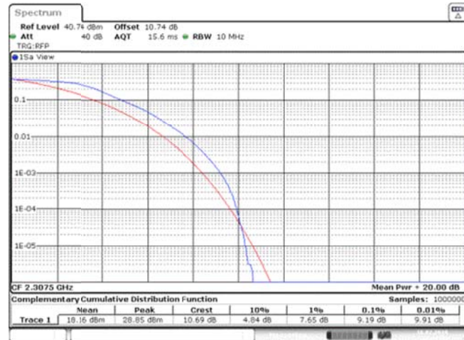
Band40_5MHz_QPSK_38725_25RB#0
