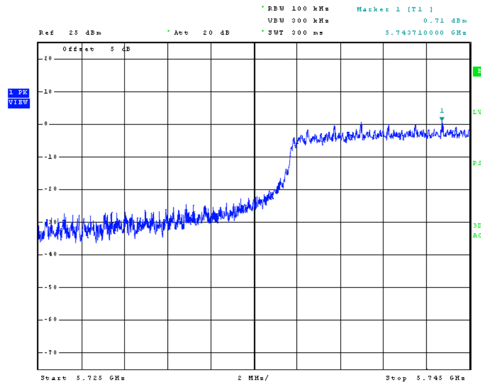
Figure 10 Plot of Transmitter Low Band Edge (Chain 1, 40 MHz Channel)
