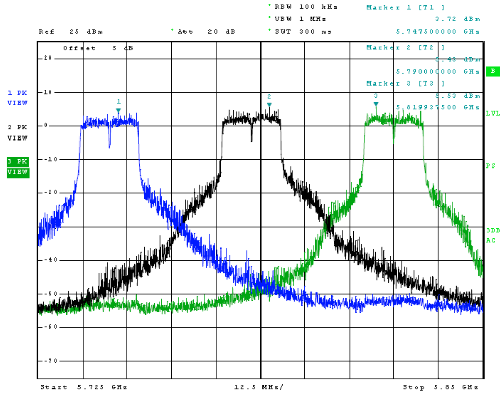
Figure 3 Plot of Transmitter Emissions (Across Operational Band, Chain 0, 20 MHz Channel)
