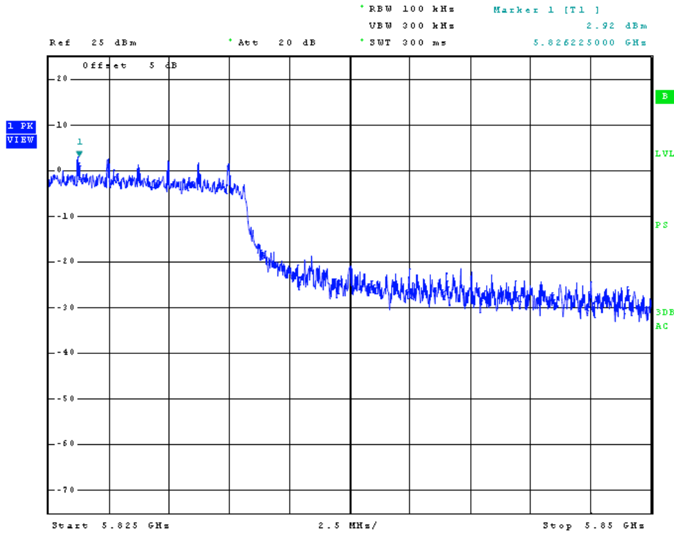
Figure 13 Plot of Transmitter High Band Edge (Chain 0, 40 MHz Channel)
