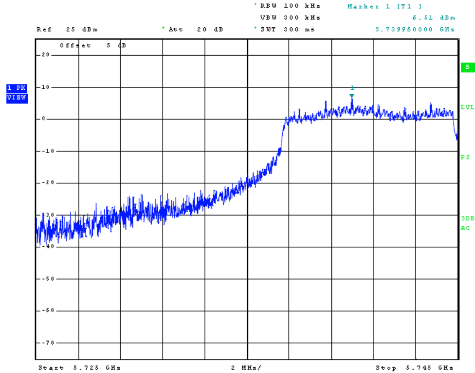
Figure 7 Plot of Transmitter Low Band Edge (Chain 0, 20 MHz Channel)
