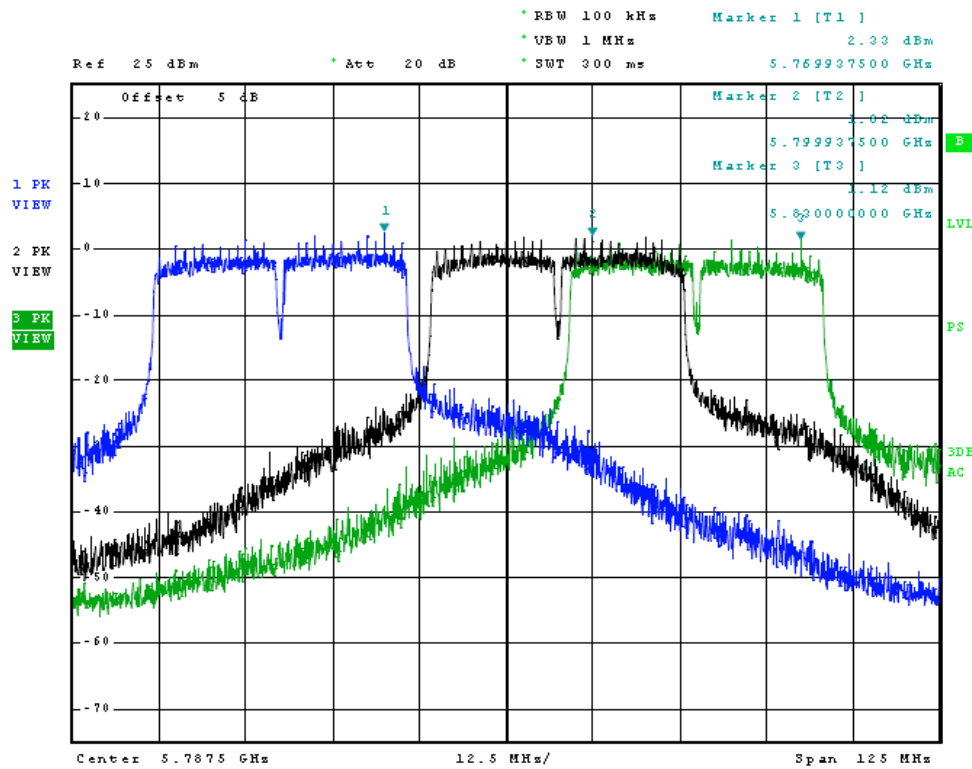
Figure 6 Plot of Transmitter Emissions (Across Operational Band, Chain 1, 40 MHz Channel)
