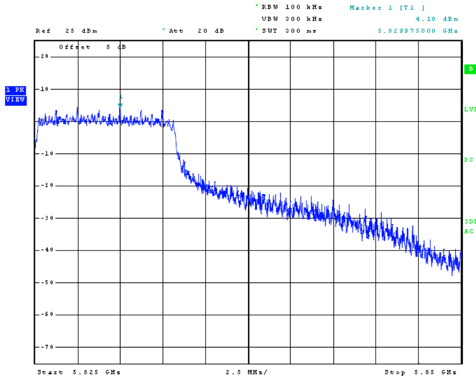
Figure 12 Plot of Transmitter High Band Edge (Chain 1, 20 MHz Channel)
