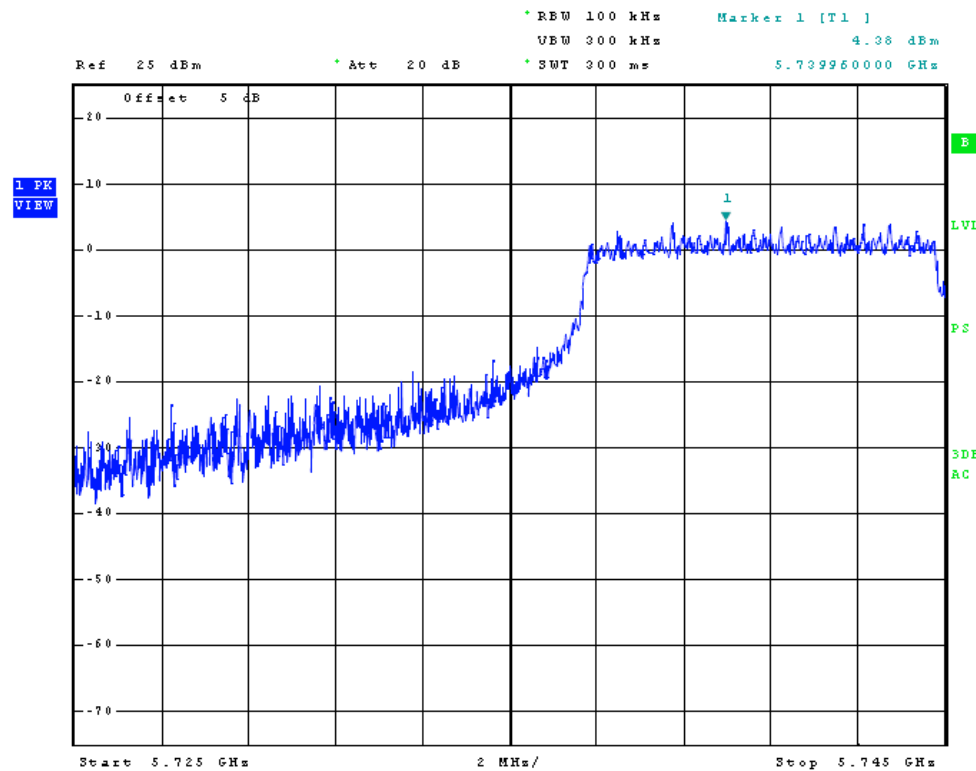
Figure 8 Plot of Transmitter Low Band Edge (Chain 1, 20 MHz Channel)
