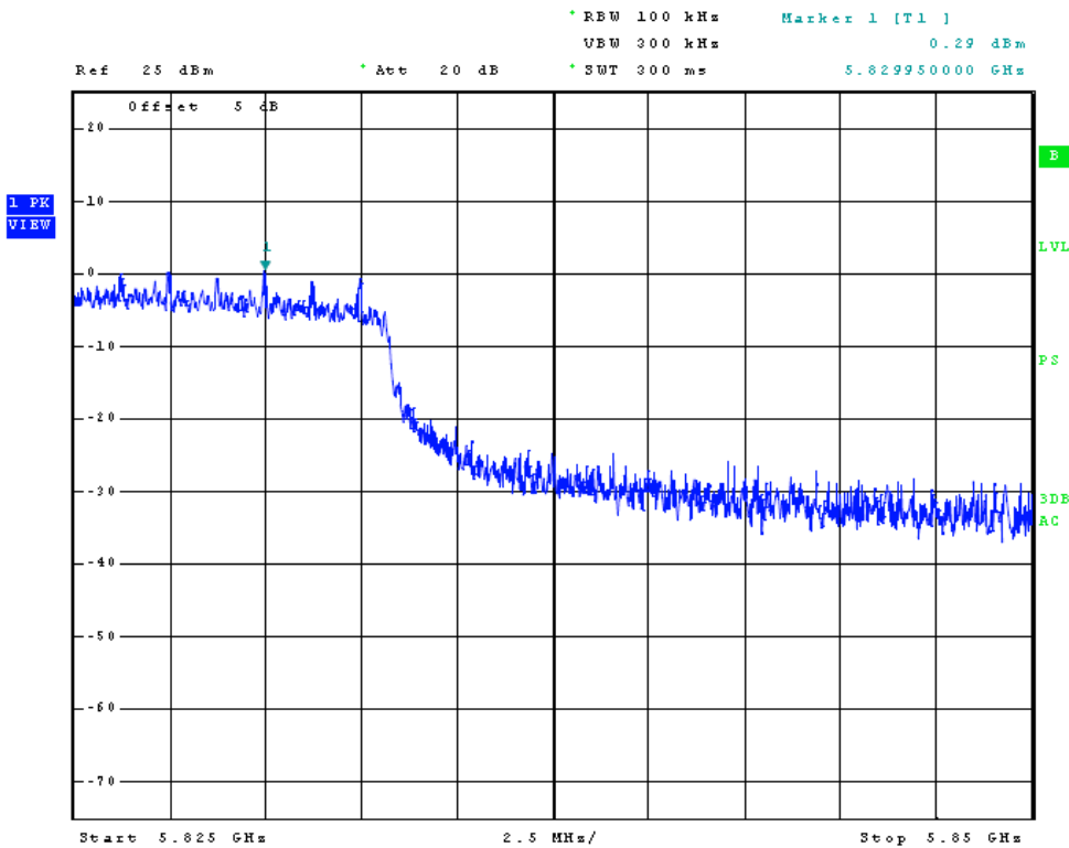
Figure 14 Plot of Transmitter High Band Edge (Chain 1, 40 MHz Channel)
