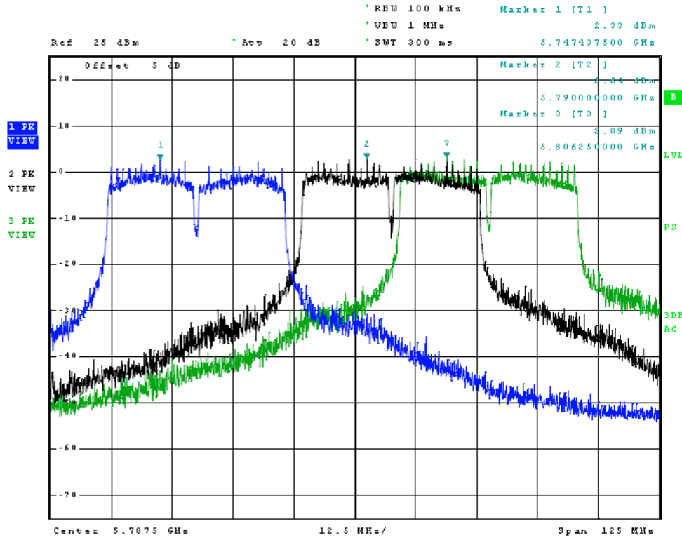
Figure 5 Plot of Transmitter Emissions (Across Operational Band, Chain 0, 40 MHz Channel)
