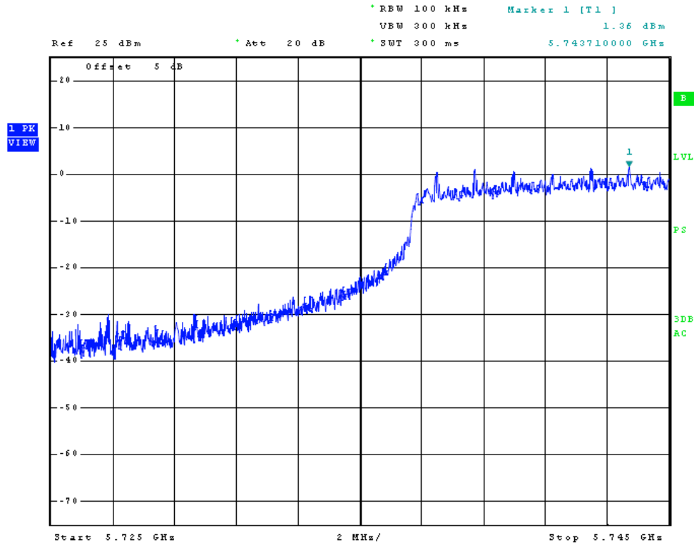
Figure 9 Plot of Transmitter Low Band Edge (Chain 0, 40 MHz Channel)
