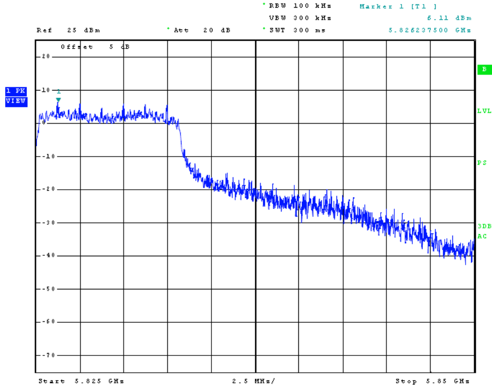
Figure 11 Plot of Transmitter High Band Edge (Chain 0, 20 MHz Channel)
