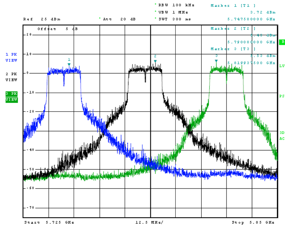
Figure 4 Plot of Transmitter Emissions (Across Operational Band, Chain 1, 20 MHz Channel)
