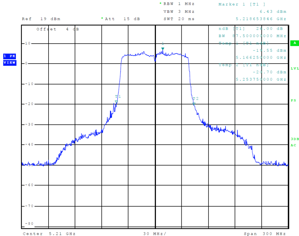
Figure 32 Plot of Transmitter Emissions (5150-5250 MHz Band, 802.11ac, Chain 1, 26 dB OBW)
