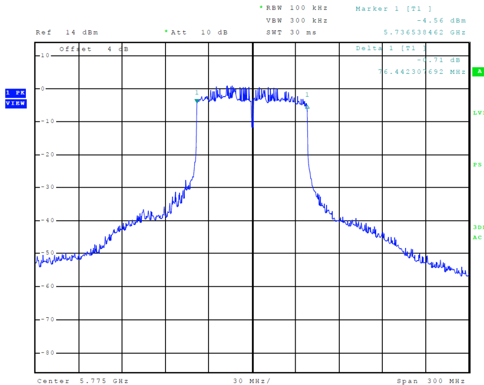
Figure 62 Plot of Transmitter Emissions (5725-5850 MHz Band, 802.11ac, Chain 1, 6-dB OBW)
