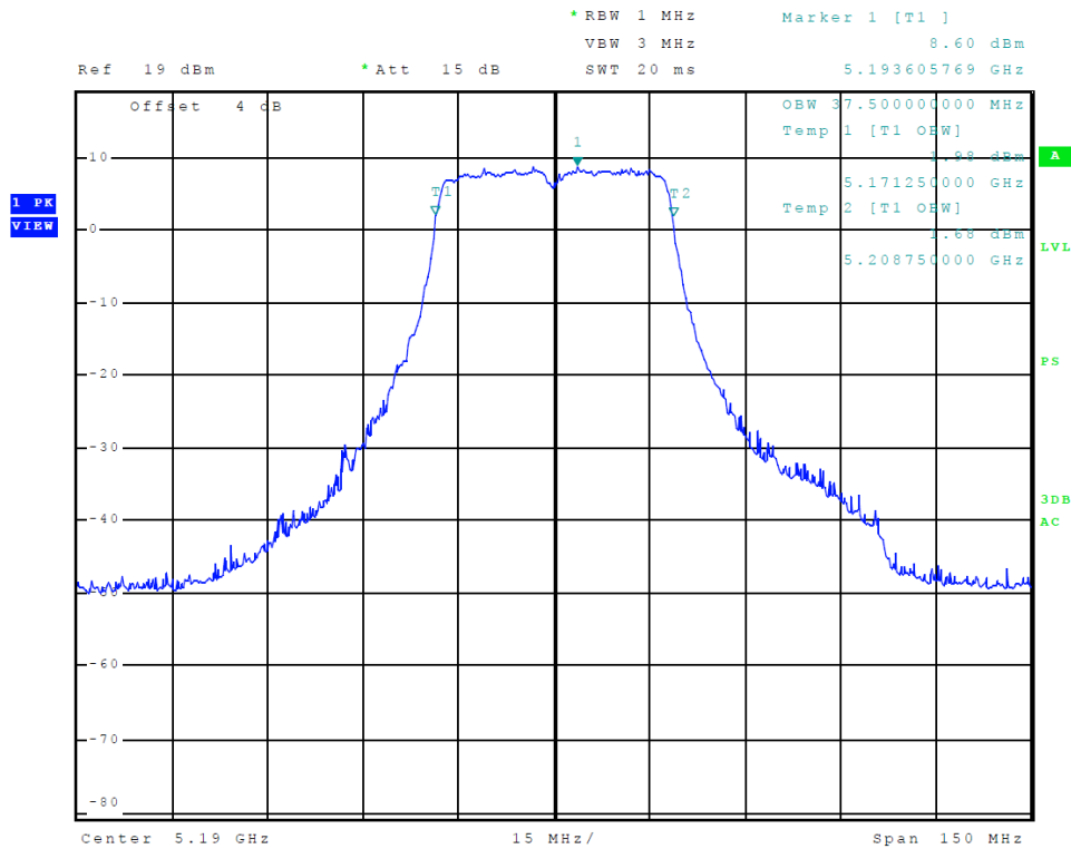
Figure 25 Plot of Transmitter Emissions (5150-5250 MHz Band, 802.11n40, Chain 0, 99% OBW)
