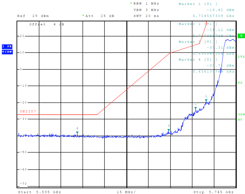
Figure 40 Plot of Transmitter Low Band Edge (5725-5850 MHz Band, Chain 1, 802.11a)
