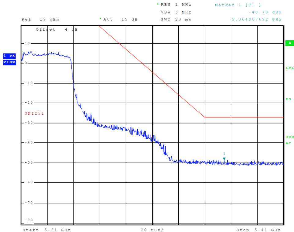
Figure 20 Plot of Transmitter High Band Edge (5150-5250 MHz Band, Chain 1, 802.11ac)
