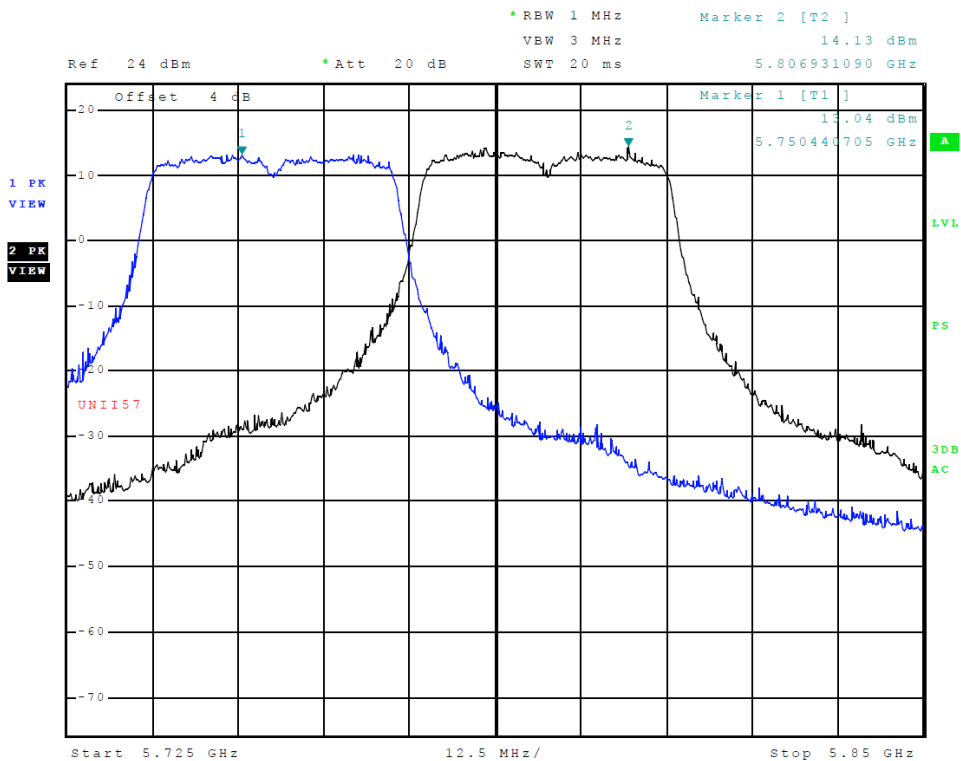
Figure 36 Plot of Transmitter Emissions (Across 5725-5850 MHz Band, Chain 1, 802.11n40)
