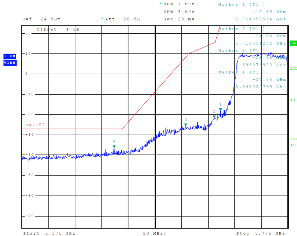
Figure 44 Plot of Transmitter Low Band Edge (5725-5850 MHz Band, Chain 1, 802.11ac)
