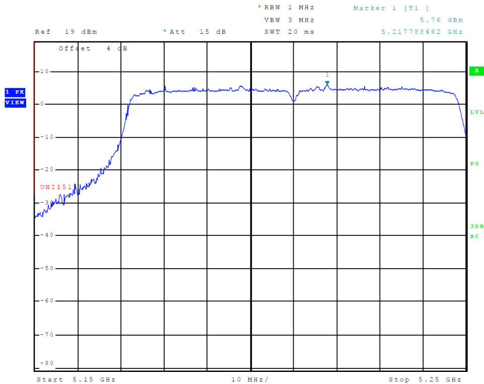
Figure 7 Plot of Transmitter Emissions (Across 5150-5250 MHz Band, Chain 0, 802.11ac)
