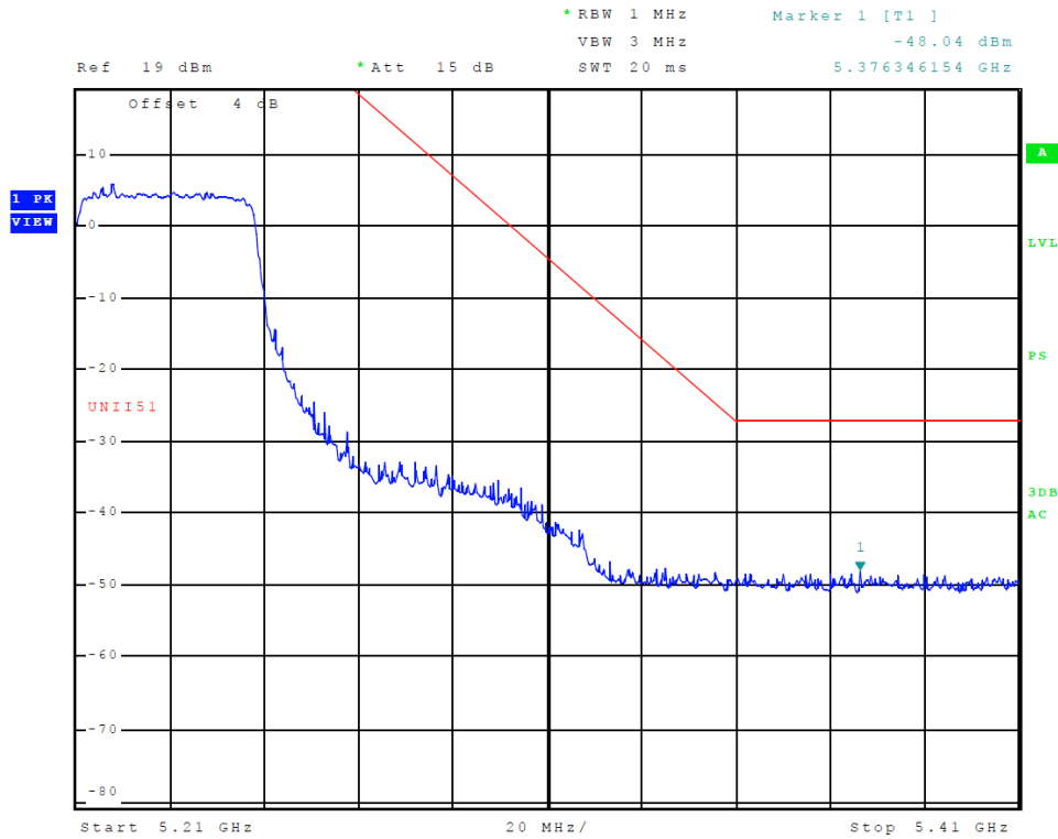
Figure 19 Plot of Transmitter High Band Edge (5150-5250 MHz Band, Chain 0, 802.11ac)
