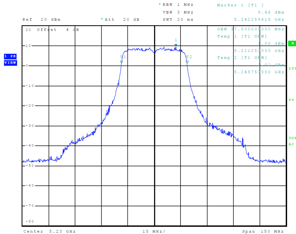
Figure 26 Plot of Transmitter Emissions (5150-5250 MHz Band, 802.11n40, Chain 1, 99% OBW)
