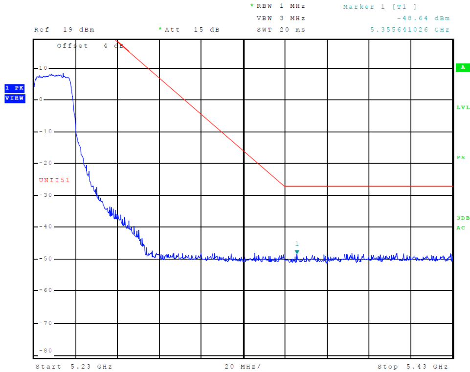
Figure 17 Plot of Transmitter High Band Edge (5150-5250 MHz Band, Chain 0, 802.11n40)
