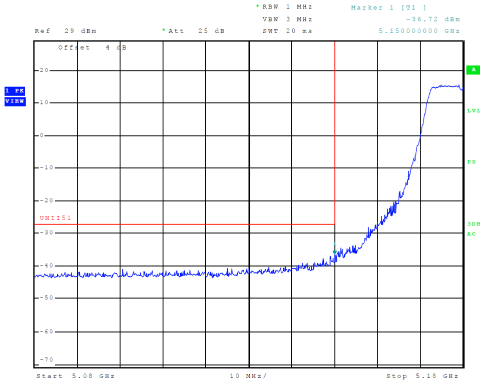
Figure 9 Plot of Transmitter Low Band Edge (5150-5250 MHz Band, Chain 0, 802.11a)
