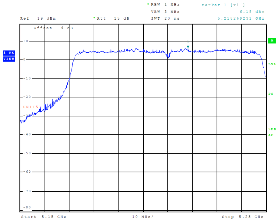
Figure 8 Plot of Transmitter Emissions (Across 5150-5250 MHz Band, Chain 1, 802.11ac)
