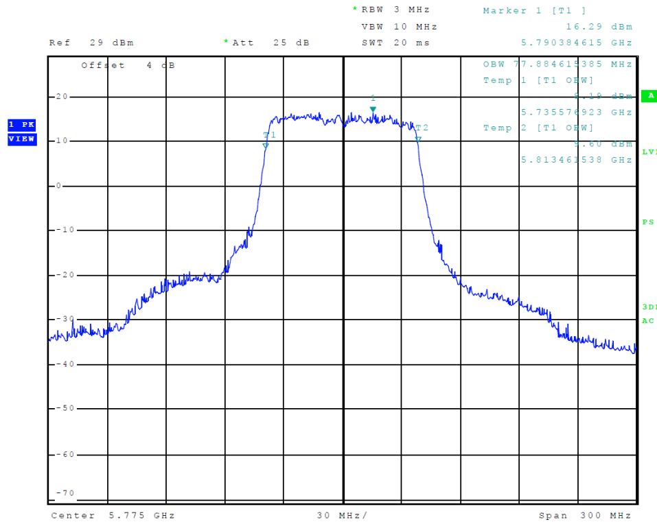
Figure 60 Plot of Transmitter Emissions (5725-5850 MHz Band, 802.11ac, Chain 1, 99% OBW)
