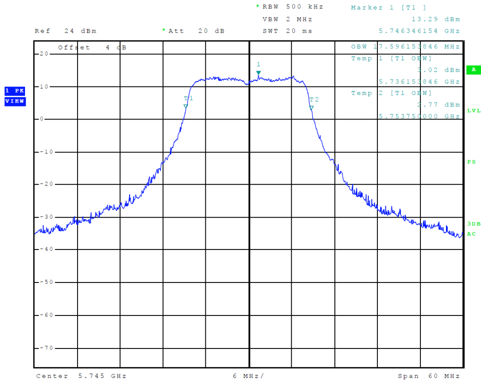
Figure 51 Plot of Transmitter Emissions (5725-5850 MHz Band, 802.11a, Chain 0, 99% OBW)
