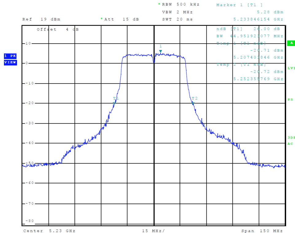
Figure 28 Plot of Transmitter Emissions (5150-5250 MHz Band, 802.11n40, Chain 1, 26 dB OBW)
