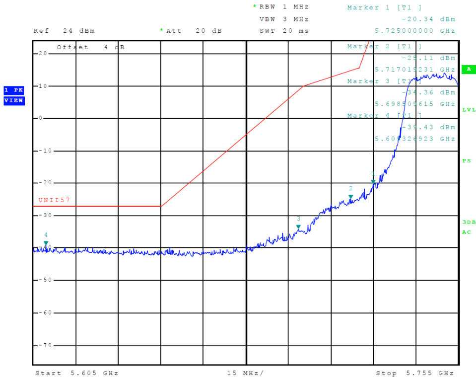
Figure 42 Plot of Transmitter Low Band Edge (5725-5850 MHz Band, Chain 1, 802.11n40)
