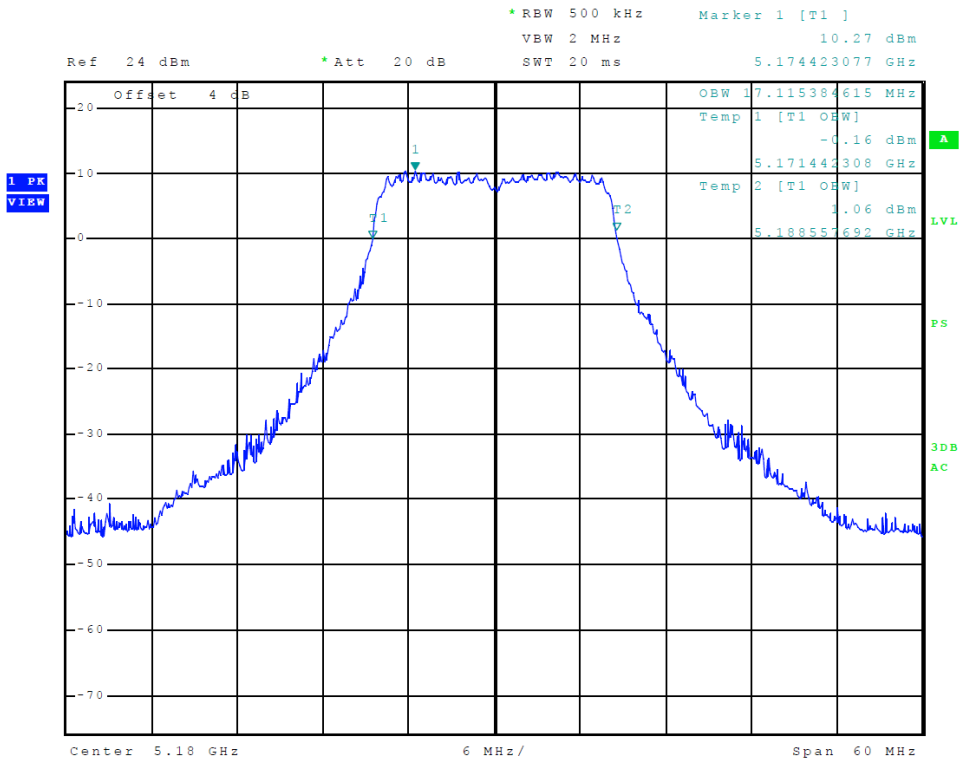
Figure 22 Plot of Transmitter Emissions (5150-5250 MHz Band, 802.11a, Chain 1, 99% OBW)
