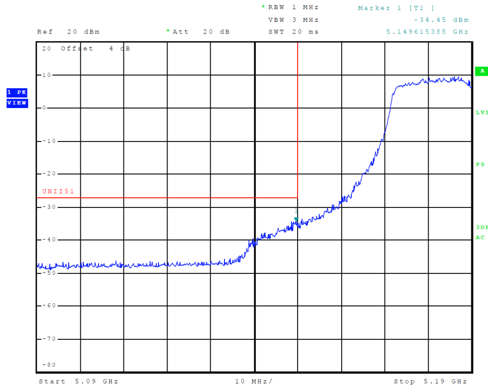
Figure 12 Plot of Transmitter Low Band Edge (5150-5250 MHz Band, Chain 1, 802.11n40)
