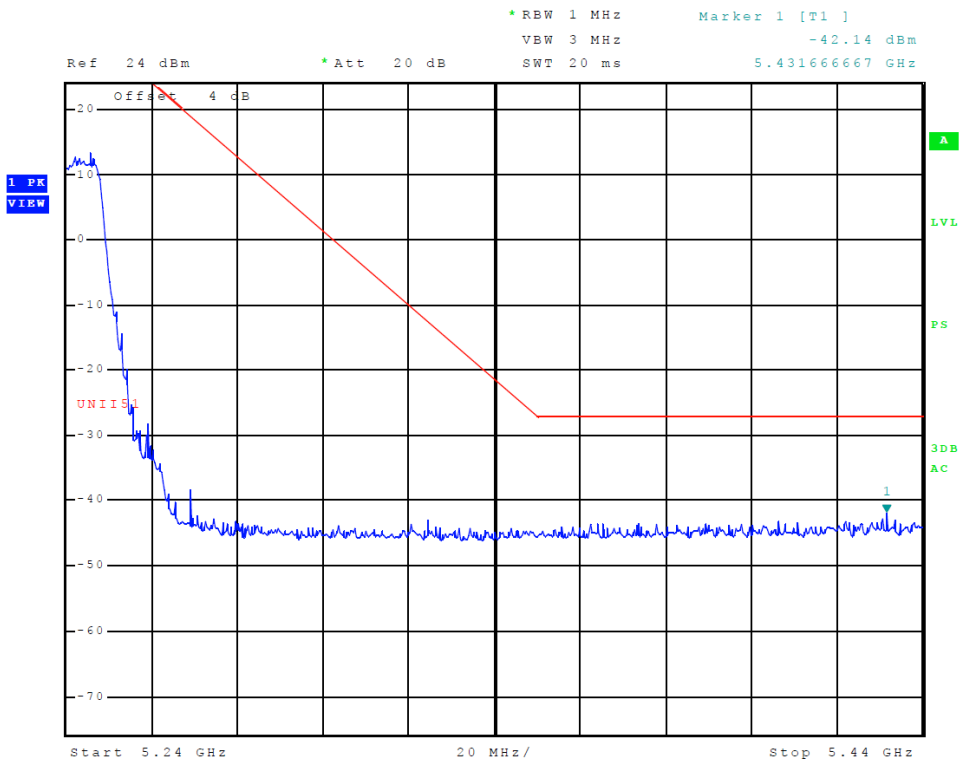
Figure 16 Plot of Transmitter High Band Edge (5150-5250 MHz Band, Chain 1, 802.11a)
