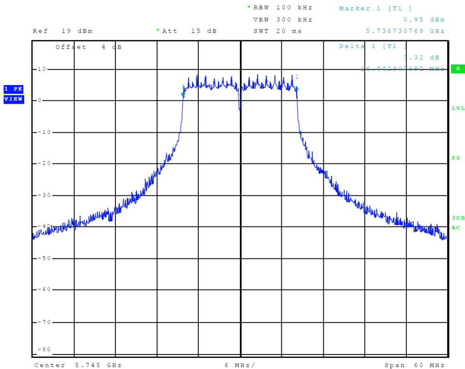
Figure 54 Plot of Transmitter Emissions (5725-5850 MHz Band, 802.11a, Chain 1, 6-dB OBW)
