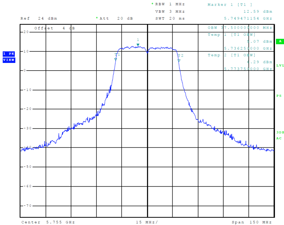
Figure 55 Plot of Transmitter Emissions (5725-5850 MHz Band, 802.11n40, Chain 0, 99% OBW)
