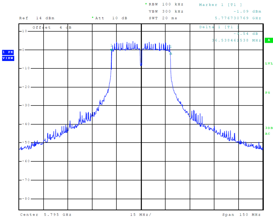
Figure 58 Plot of Transmitter Emissions (5725-5850 MHz Band, 802.11n40, Chain 1, 6-dB OBW)
