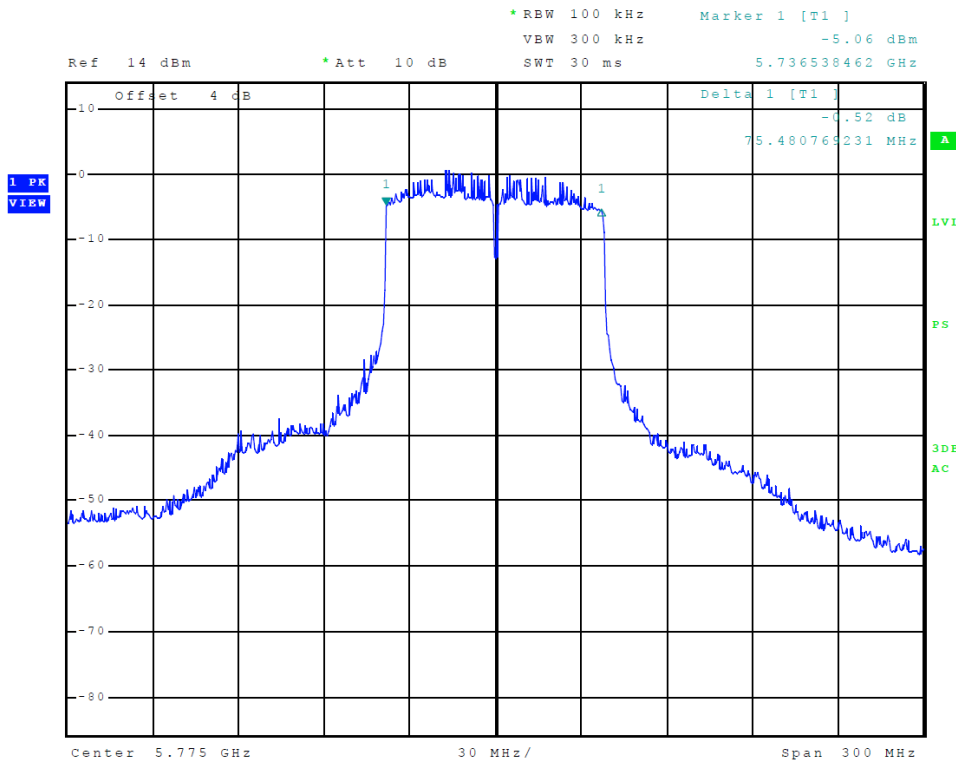
Figure 61 Plot of Transmitter Emissions (5725-5850 MHz Band, 802.11ac, Chain 0, 6-dB OBW)
