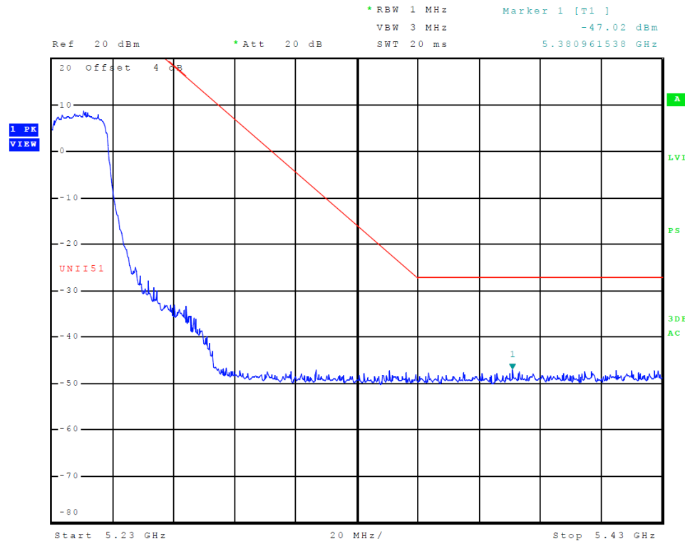
Figure 18 Plot of Transmitter High Band Edge (5150-5250 MHz Band, Chain 1, 802.11n40)
