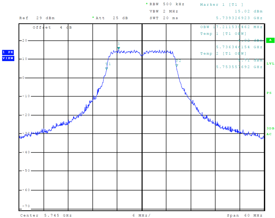
Figure 52 Plot of Transmitter Emissions (5725-5850 MHz Band, 802.11a, Chain 1, 99% OBW)
