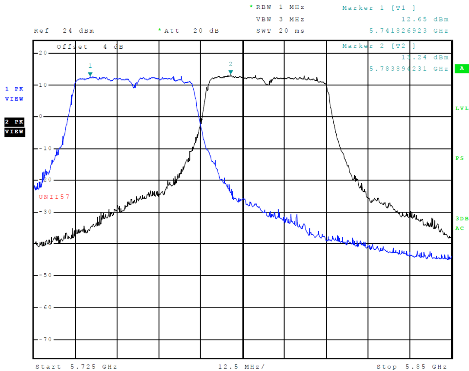
Figure 35 Plot of Transmitter Emissions (Across 5725-5850 MHz Band, Chain 0, 802.11n40)
