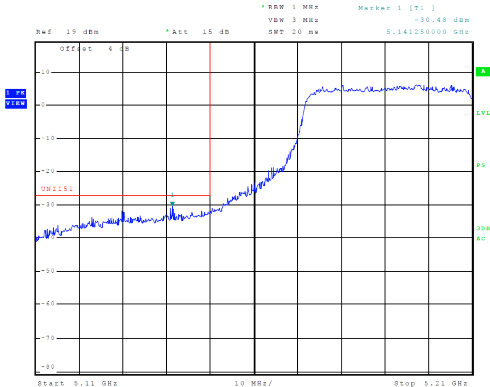
Figure 14 Plot of Transmitter Low Band Edge (5150-5250 MHz Band, Chain 1, 802.11ac)
