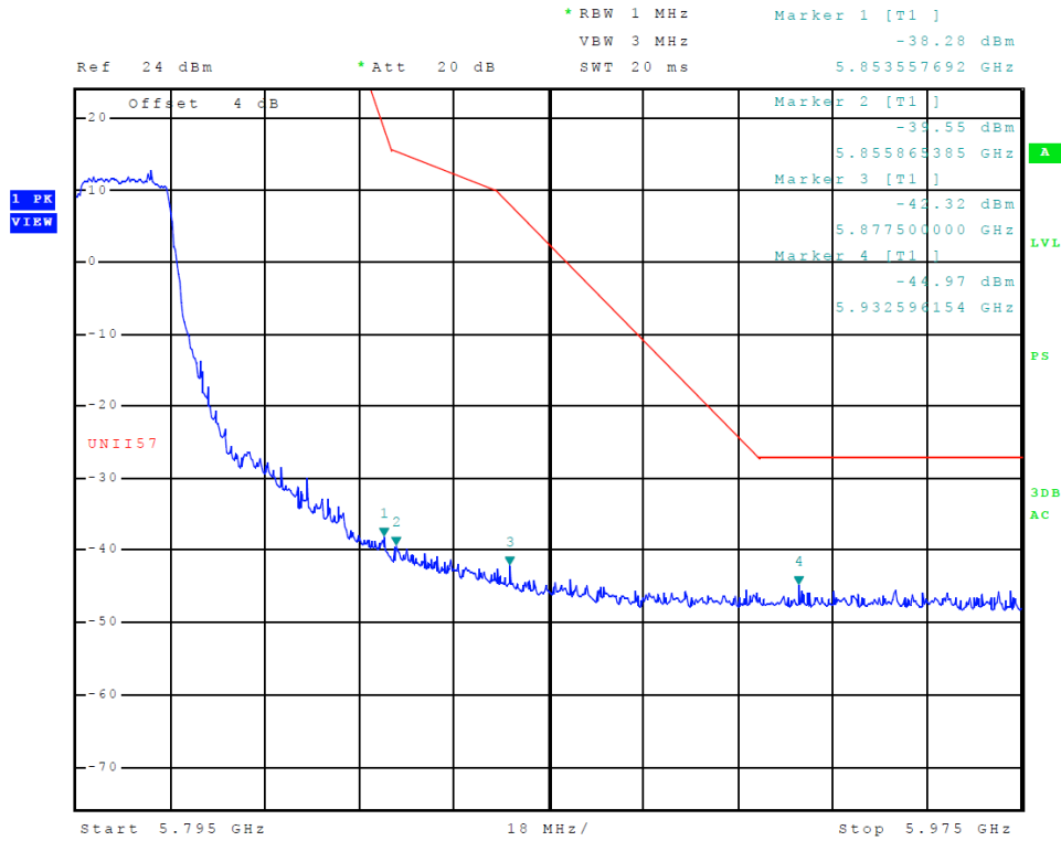
Figure 47 Plot of Transmitter High Band Edge (5725-5850 MHz Band, Chain 0, 802.11n40)
