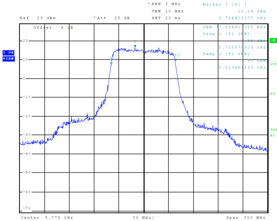
Figure 59 Plot of Transmitter Emissions (5725-5850 MHz Band, 802.11ac, Chain 0, 99% OBW)
