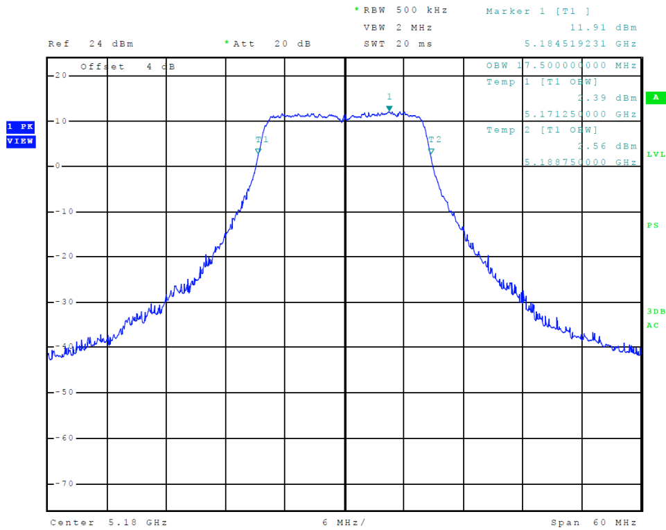
Figure 21 Plot of Transmitter Emissions (5150-5250 MHz Band, 802.11a, Chain 0, 99% OBW)
