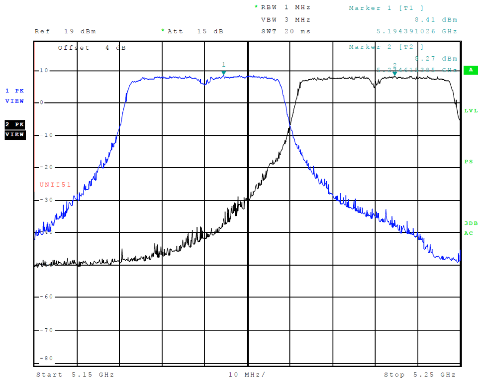
Figure 5 Plot of Transmitter Emissions (Across 5150-5250 MHz Band, Chain 0, 802.11n40)
