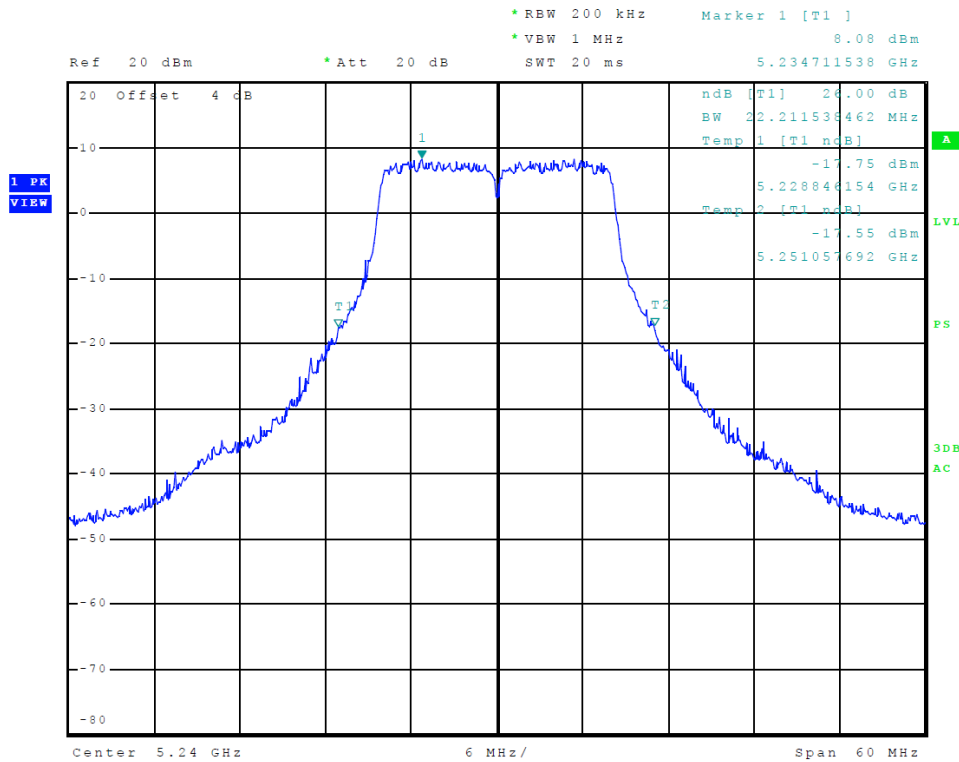
Figure 23 Plot of Transmitter Emissions (5150-5250 MHz Band, 802.11a, Chain 0, 26 dB OBW)
