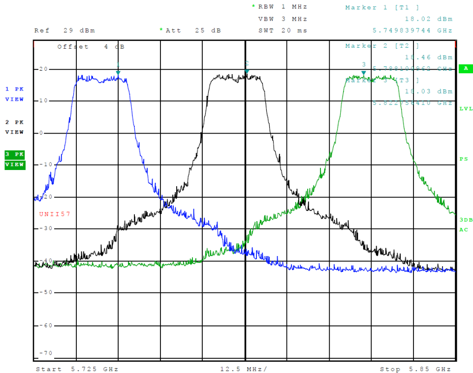
Figure 34 Plot of Transmitter Emissions (Across 5725-5850 MHz Band, Chain 1, 802.11a)
