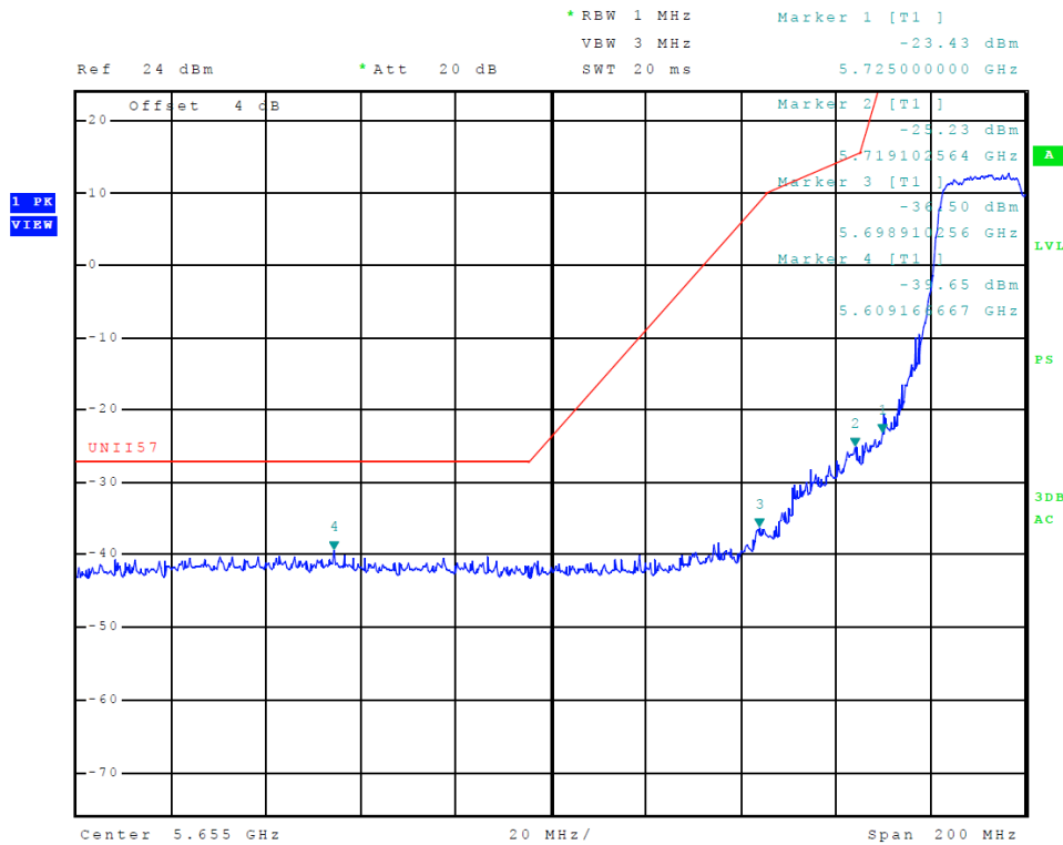
Figure 41 Plot of Transmitter Low Band Edge (5725-5850 MHz Band, Chain 0, 802.11n40)
