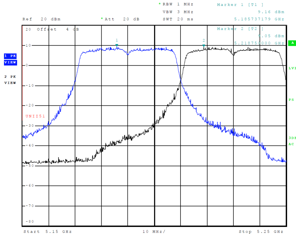
Figure 6 Plot of Transmitter Emissions (Across 5150-5250 MHz Band, Chain 1, 802.11n40)
