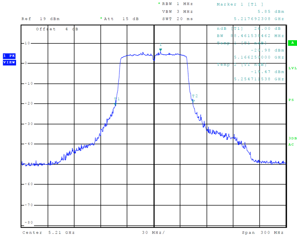
Figure 31 Plot of Transmitter Emissions (5150-5250 MHz Band, 802.11ac, Chain 0, 26 dB OBW)
