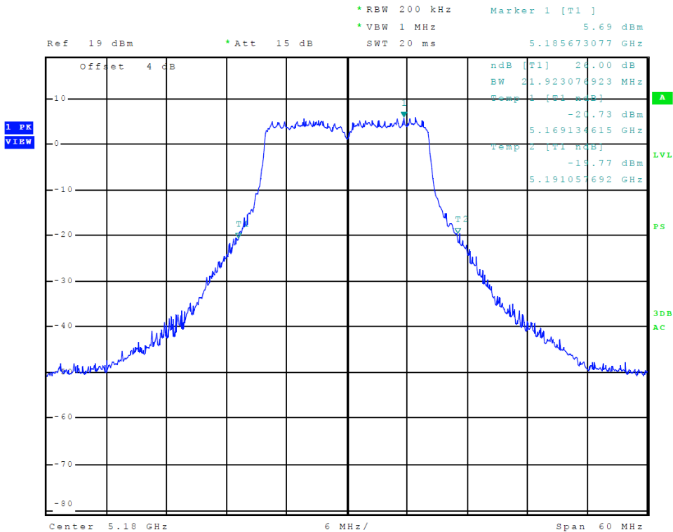
Figure 24 Plot of Transmitter Emissions (5150-5250 MHz Band, 802.11a, Chain 1, 26 dB OBW)
