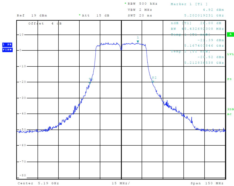
Figure 27 Plot of Transmitter Emissions (5150-5250 MHz Band, 802.11n40, Chain 0, 26 dB OBW)
