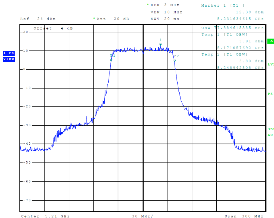
Figure 30 Plot of Transmitter Emissions (5150-5250 MHz Band, 802.11ac, Chain 1, 99% OBW)
