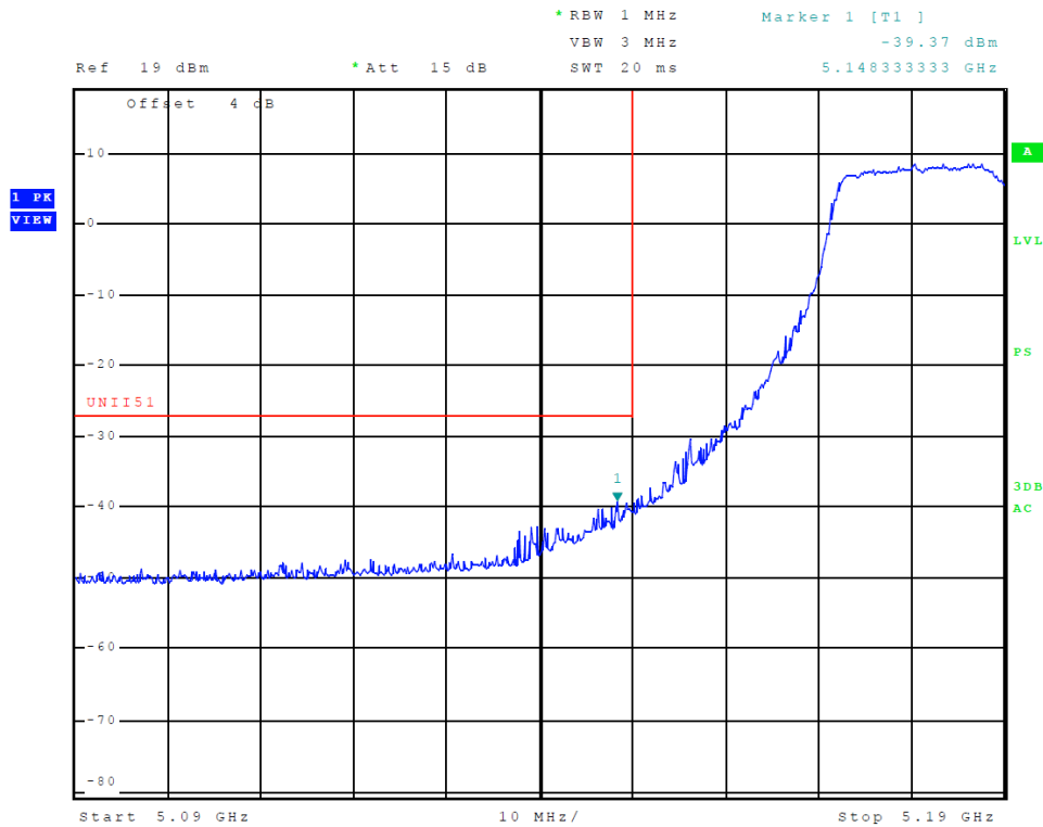
Figure 11 Plot of Transmitter Low Band Edge (5150-5250 MHz Band, Chain 0, 802.11n40)
