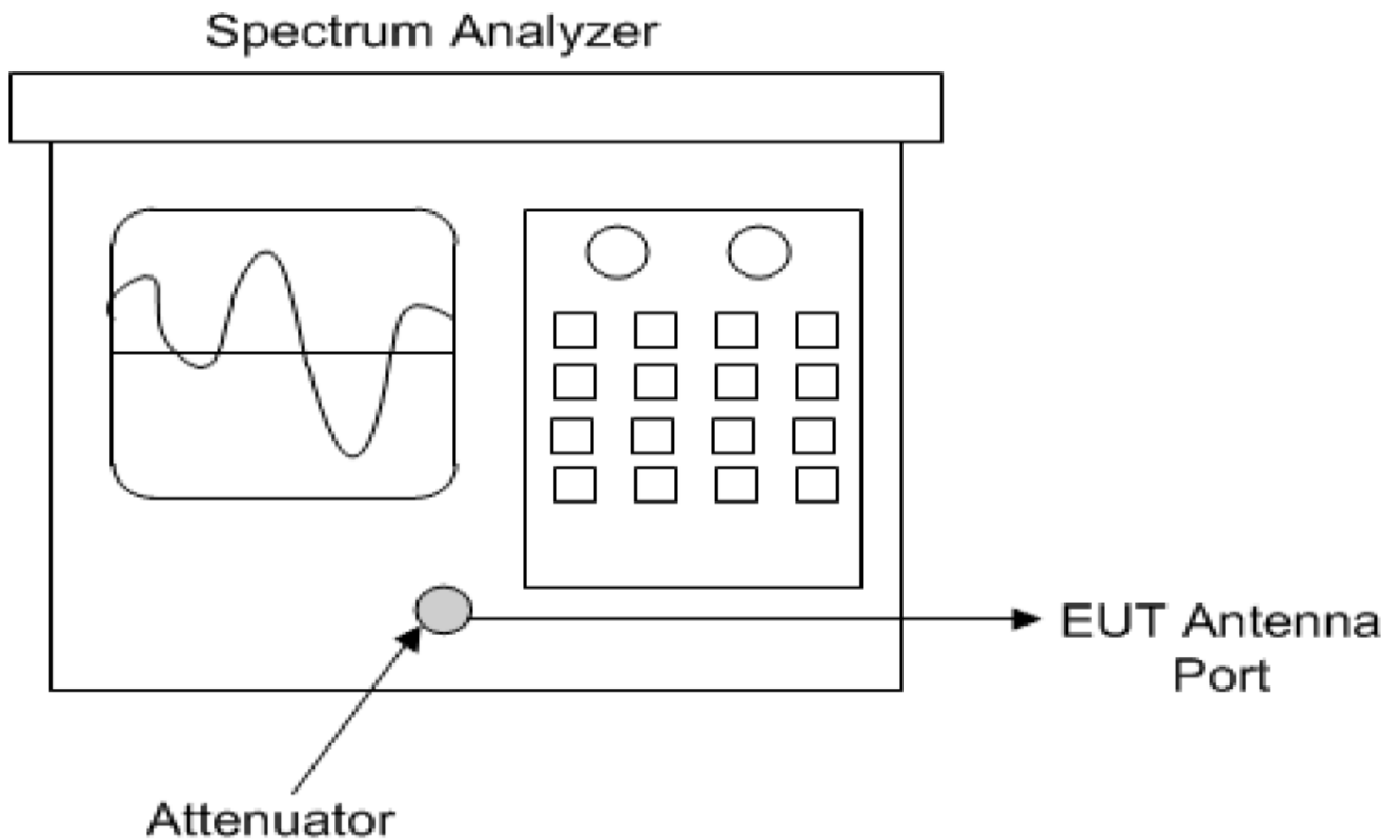
Diagram 4 Test arrangement for Antenna Port Conducted emissions
