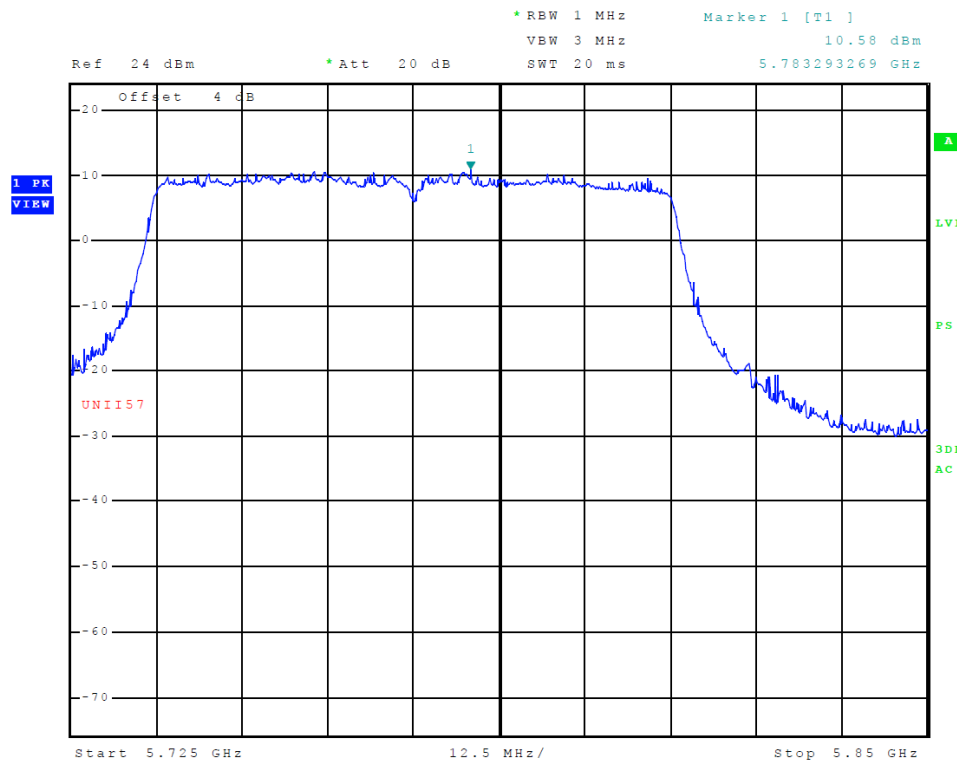
Figure 38 Plot of Transmitter Emissions (Across 5725-5850 MHz Band, Chain 1, 802.11ac)
