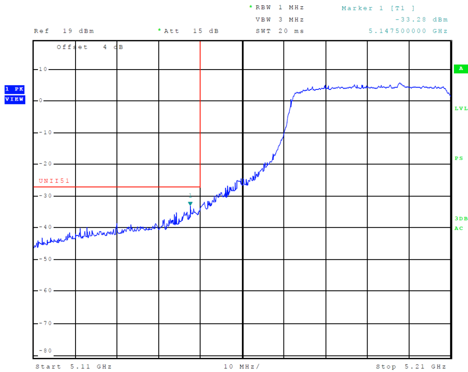
Figure 13 Plot of Transmitter Low Band Edge (5150-5250 MHz Band, Chain 0, 802.11ac)
