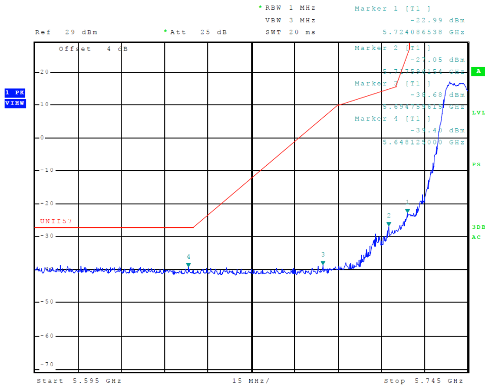
Figure 39 Plot of Transmitter Low Band Edge (5725-5850 MHz Band, Chain 0, 802.11a)
