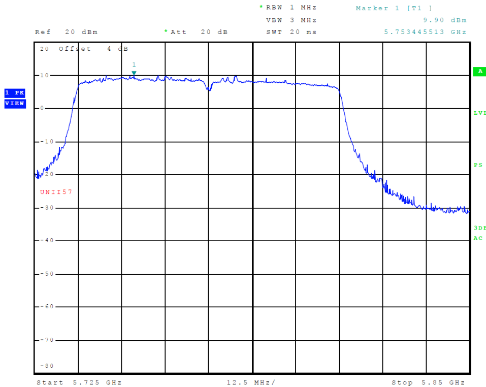
Figure 37 Plot of Transmitter Emissions (Across 5725-5850 MHz Band, Chain 0, 802.11ac)
