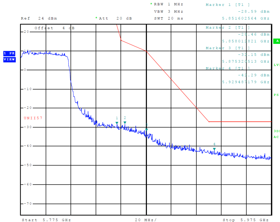
Figure 50 Plot of Transmitter High Band Edge (5725-5850 MHz Band, Chain 1, 802.11ac)
