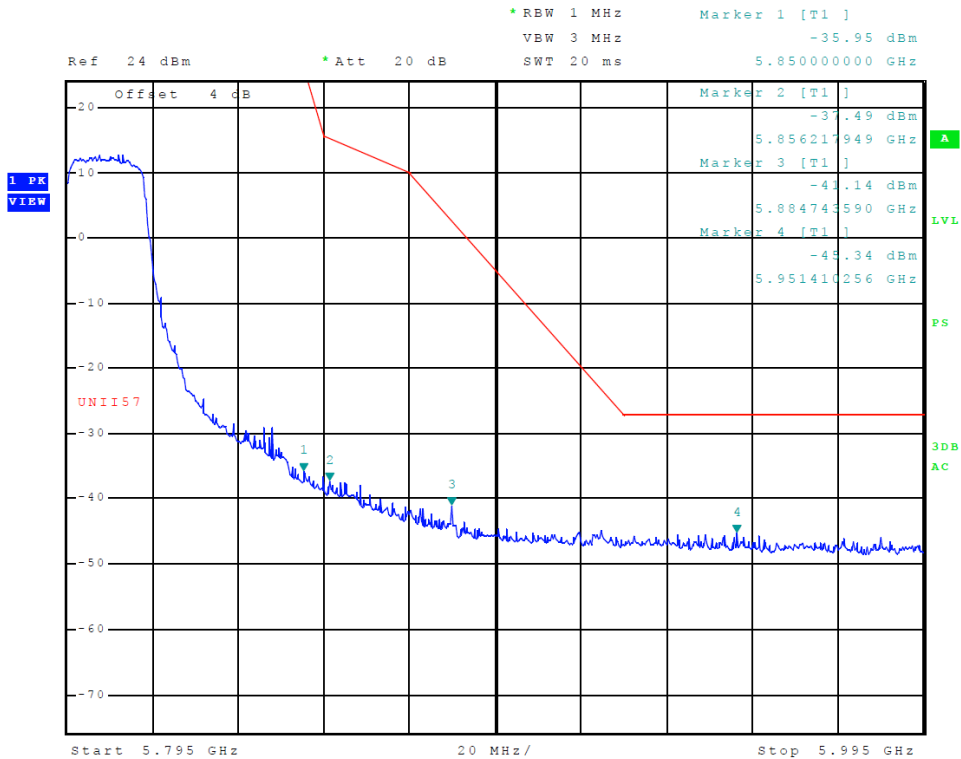
Figure 48 Plot of Transmitter High Band Edge (5725-5850 MHz Band, Chain 1, 802.11n40)
