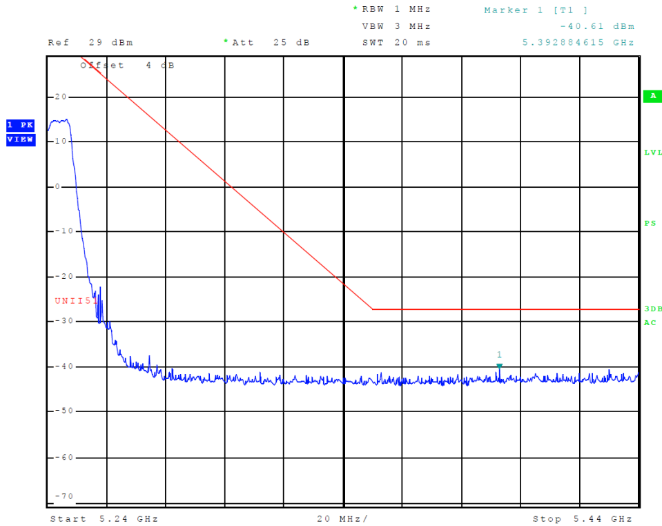
Figure 15 Plot of Transmitter High Band Edge (5150-5250 MHz Band, Chain 0, 802.11a)
