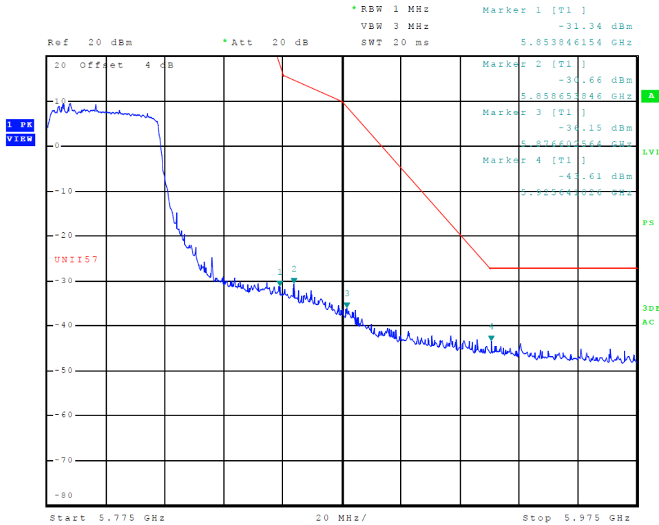
Figure 49 Plot of Transmitter High Band Edge (5725-5850 MHz Band, Chain 0, 802.11ac)
