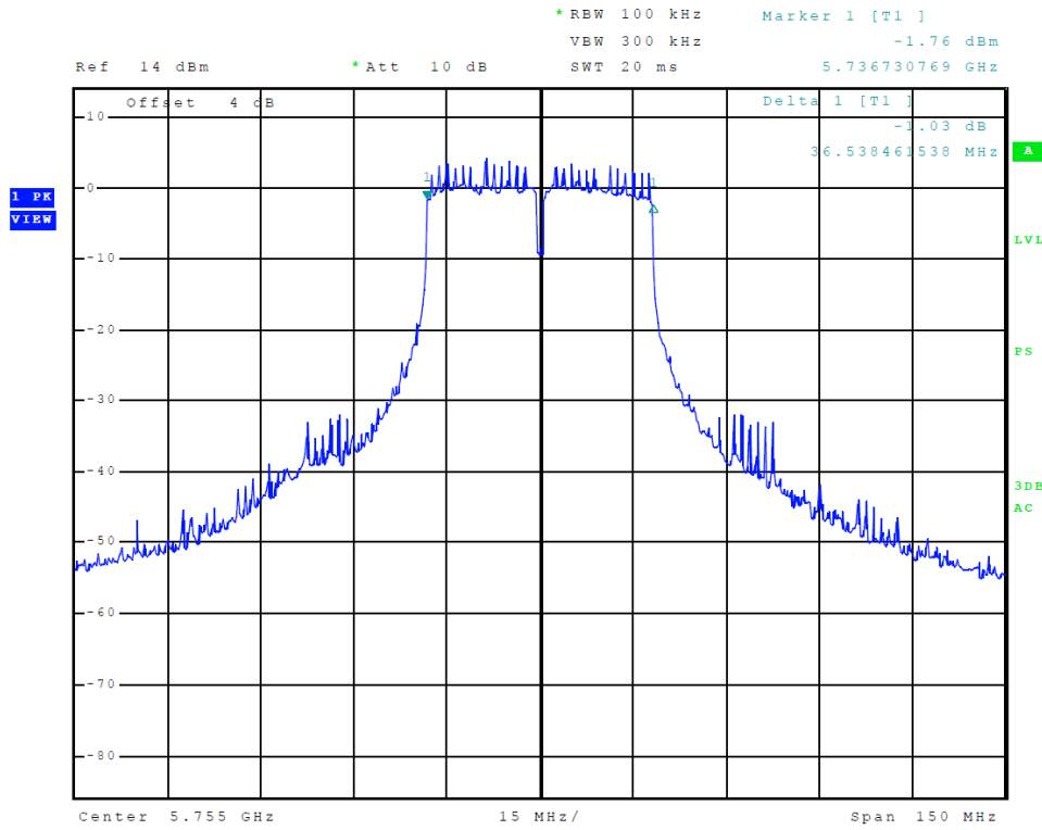
Figure 57 Plot of Transmitter Emissions (5725-5850 MHz Band, 802.11n40, Chain 0, 6-dB OBW)
