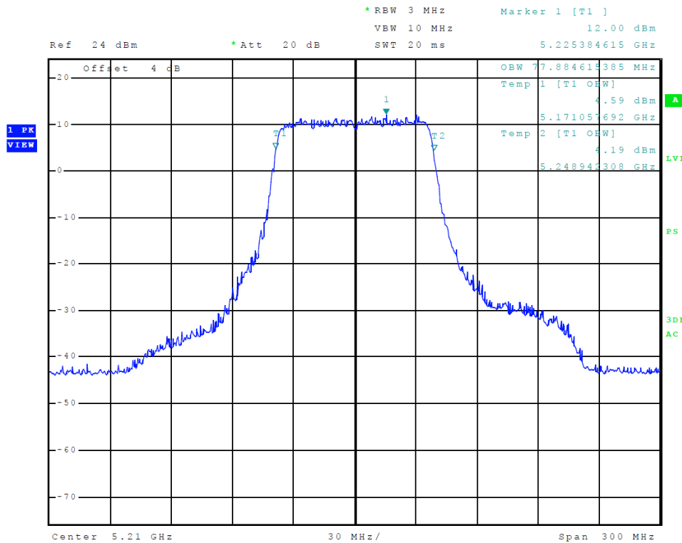
Figure 29 Plot of Transmitter Emissions (5150-5250 MHz Band, 802.11ac, Chain 0, 99% OBW)
