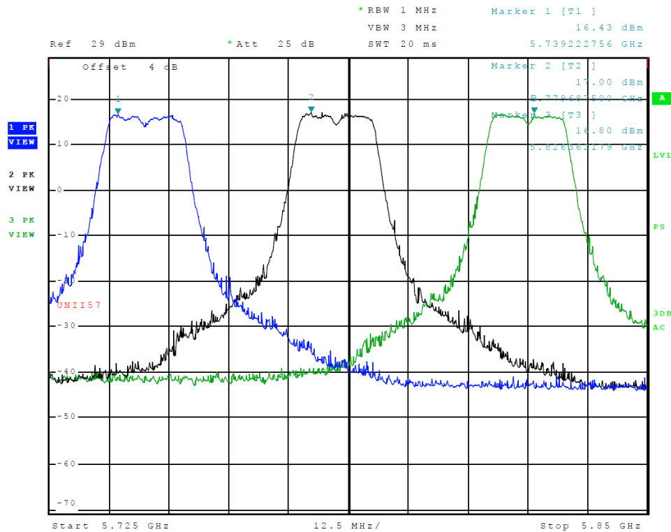
Figure 33 Plot of Transmitter Emissions (Across 5725-5850 MHz Band, Chain 0, 802.11a)
