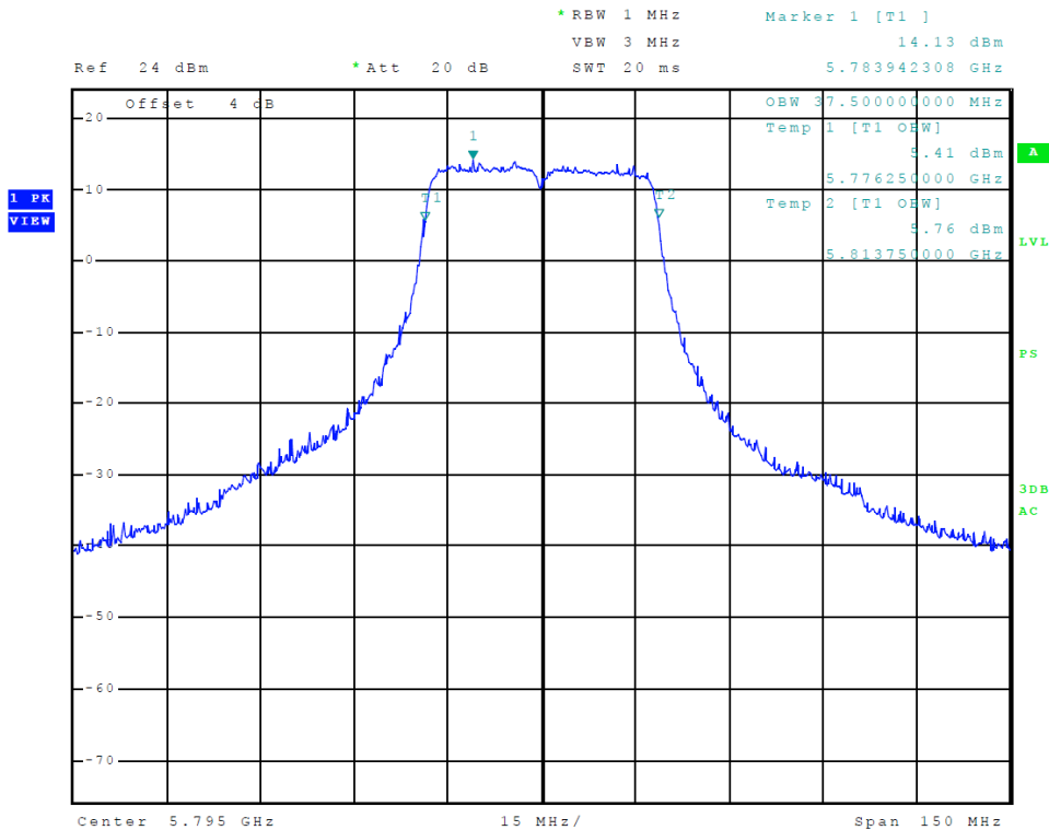
Figure 56 Plot of Transmitter Emissions (5725-5850 MHz Band, 802.11n40, Chain 1, 99% OBW)
