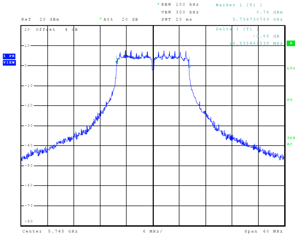
Figure 53 Plot of Transmitter Emissions (5725-5850 MHz Band, 802.11a, Chain 0, 6-dB OBW)
