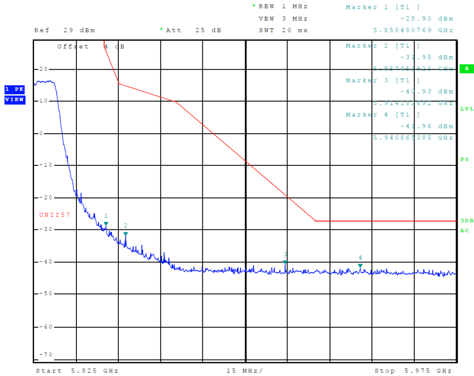
Figure 45 Plot of Transmitter High Band Edge (5725-5850 MHz Band, Chain 0, 802.11a)
