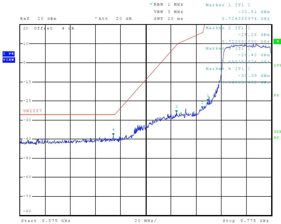
Figure 43 Plot of Transmitter Low Band Edge (5725-5850 MHz Band, Chain 0, 802.11ac)
