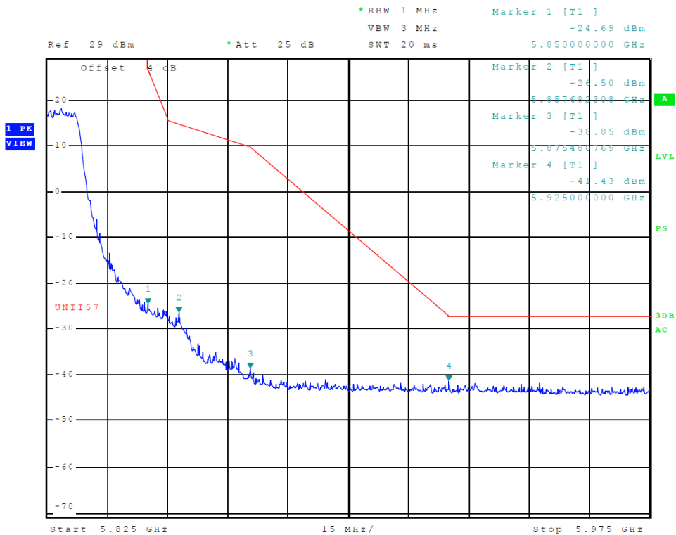
Figure 46 Plot of Transmitter High Band Edge (5725-5850 MHz Band, Chain 1, 802.11a)
