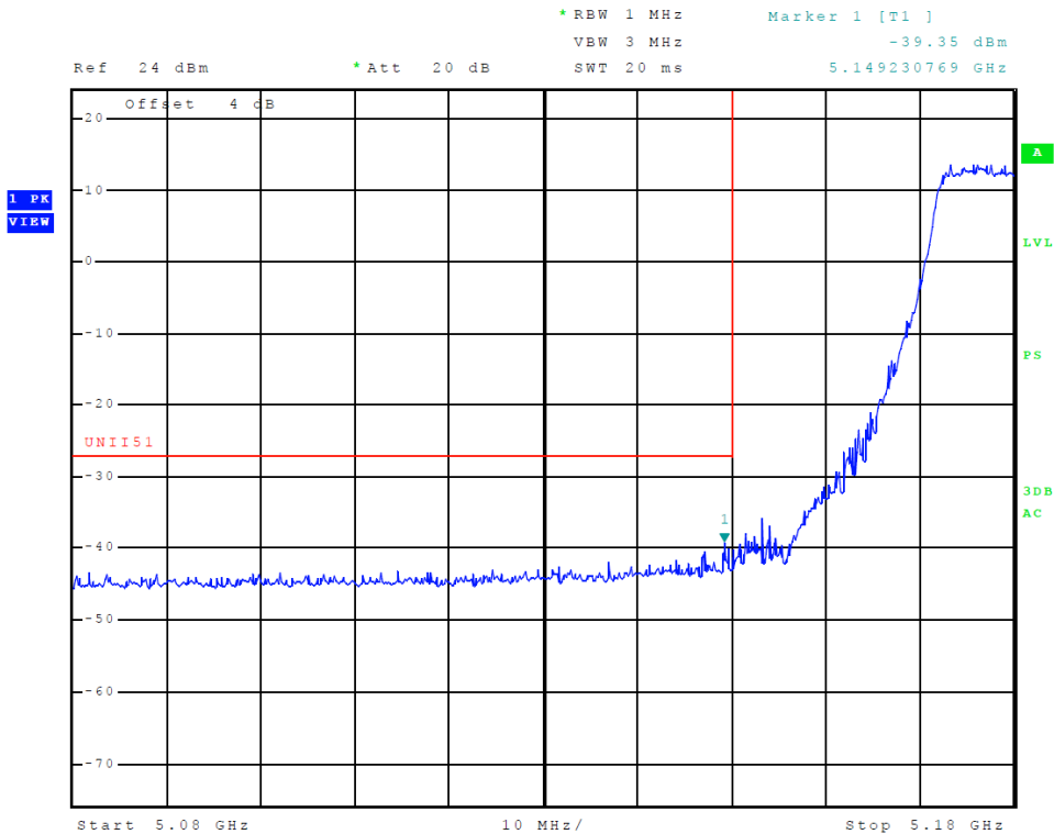
Figure 10 Plot of Transmitter Low Band Edge (5150-5250 MHz Band, Chain 1, 802.11a)
