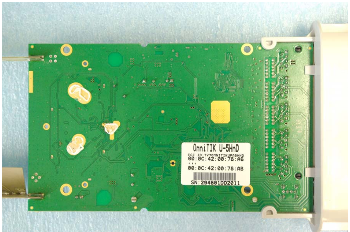
Heat sink removed
