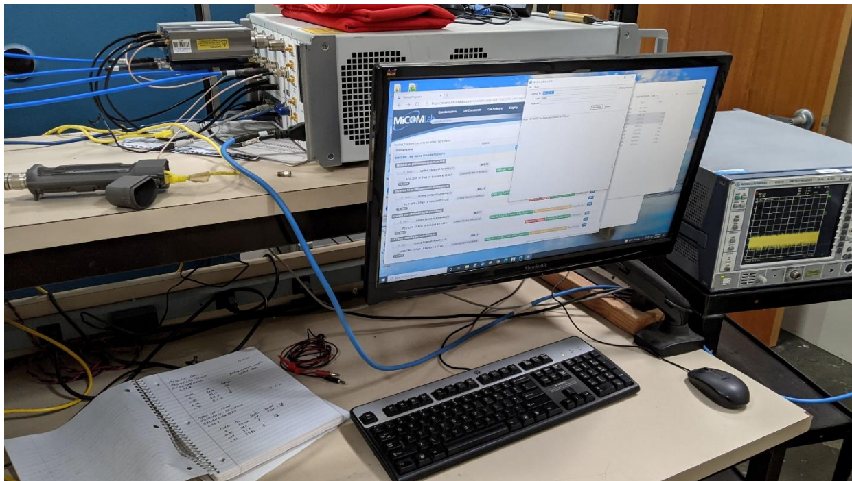
Conducted RF Setup
