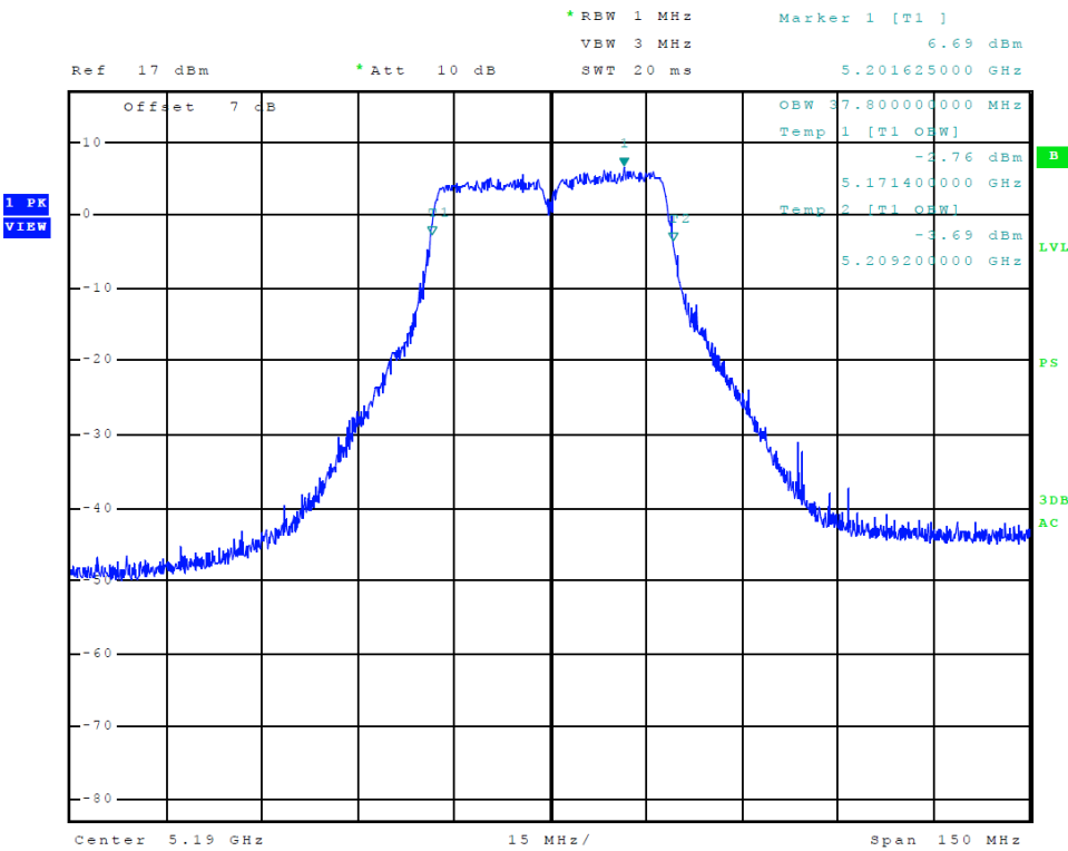
Figure 14 Plot of Transmitter Emissions (5150-5250 MHz Band, 802.11n40, 99% OBW)
