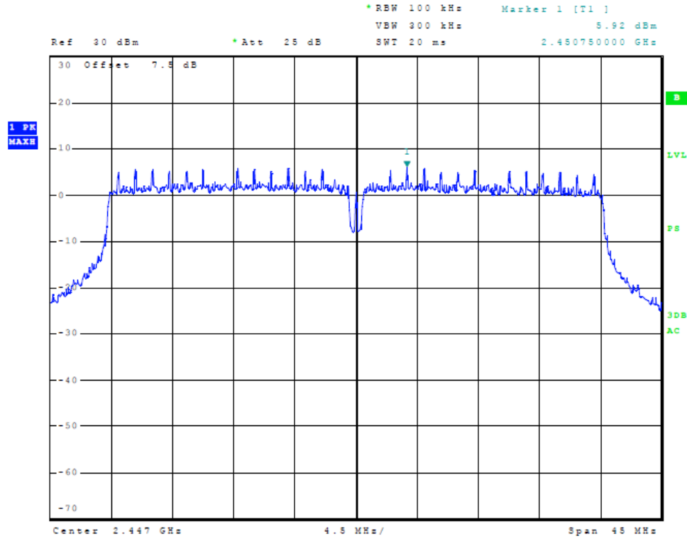
Figure 36 Plot of Power Spectral Density (40 MHz Mode, 2447 MHz)
