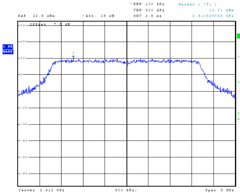
Figure 23 Plot of Power Spectral Density (5 MHz Mode, 2412 MHz)
