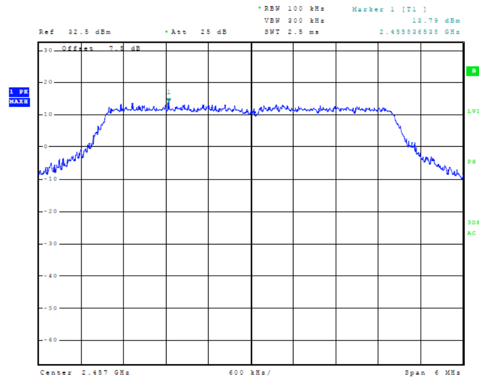
Figure 25 Plot Power Spectral Density (5 MHz Mode, 2457 MHz)
