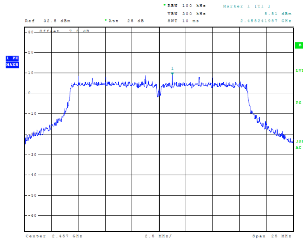
Figure 33 Plot of Power Spectral Density (20 MHz Mode, 2457 MHz)
