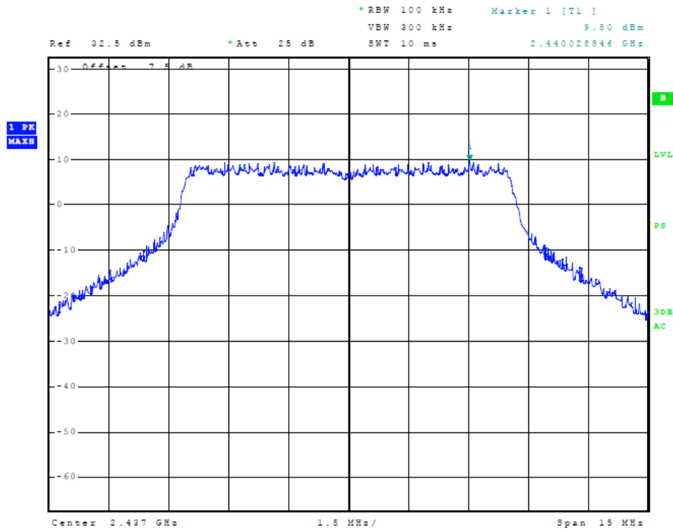
Figure 28 Plot of Power Spectral Density (10 MHz Mode, 2437 MHz)
