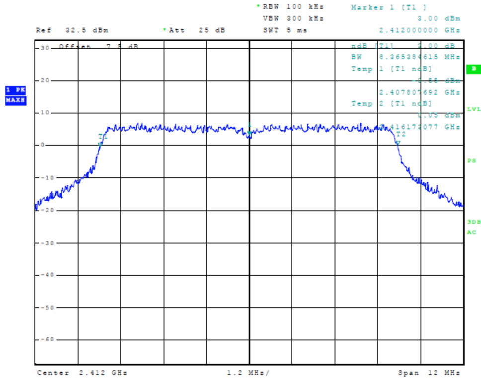
Figure 12 Plot of 6dB Band width (10 MHz Mode, 2412 MHz)
