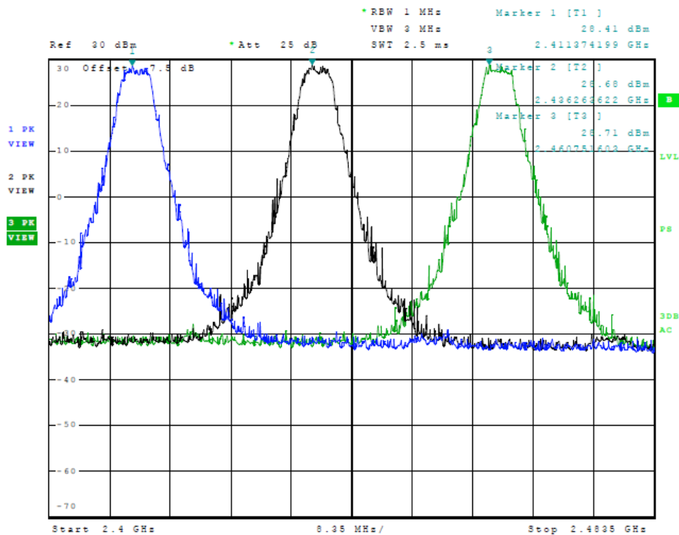
Figure 3 Plot of Output Across Operational Band (5 MHz Mode)
