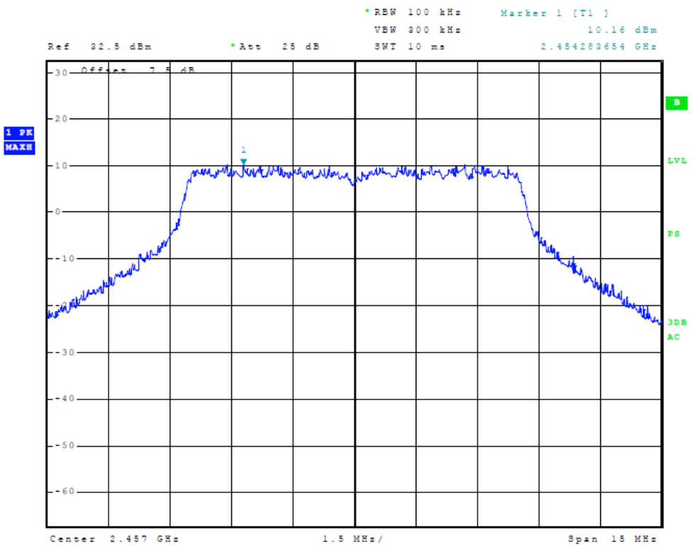
Figure 29 Plot of Power Spectral Density (10 MHz Mode, 2457 MHz)
