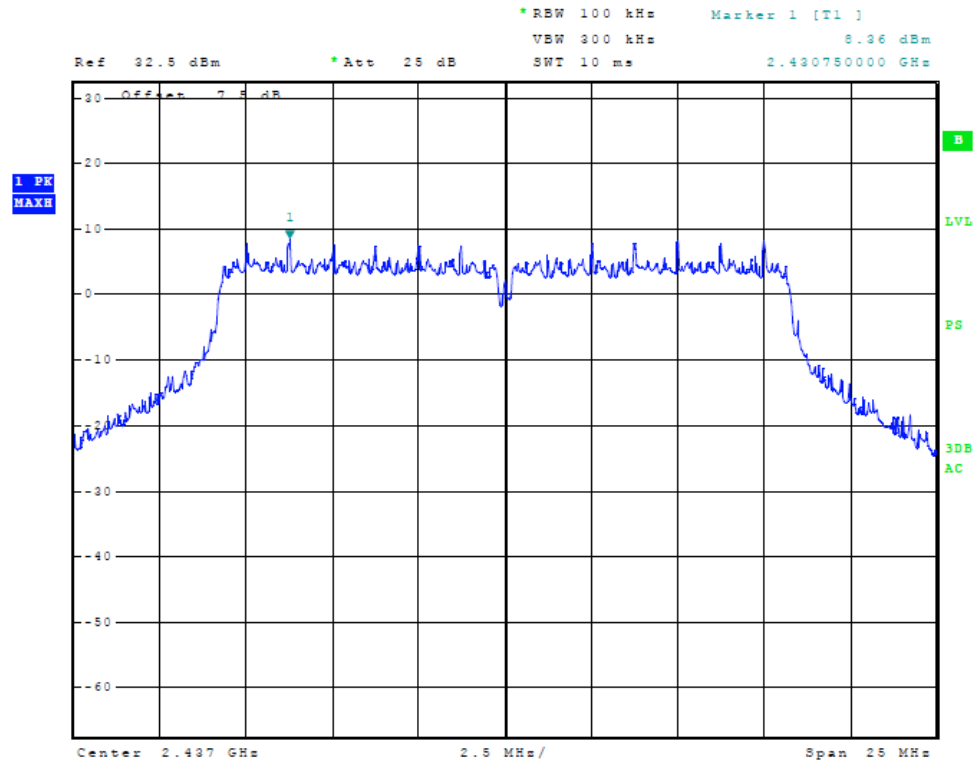
Figure 32 Plot of Power Spectral Density (20 MHz Mode, 2437 MHz)
