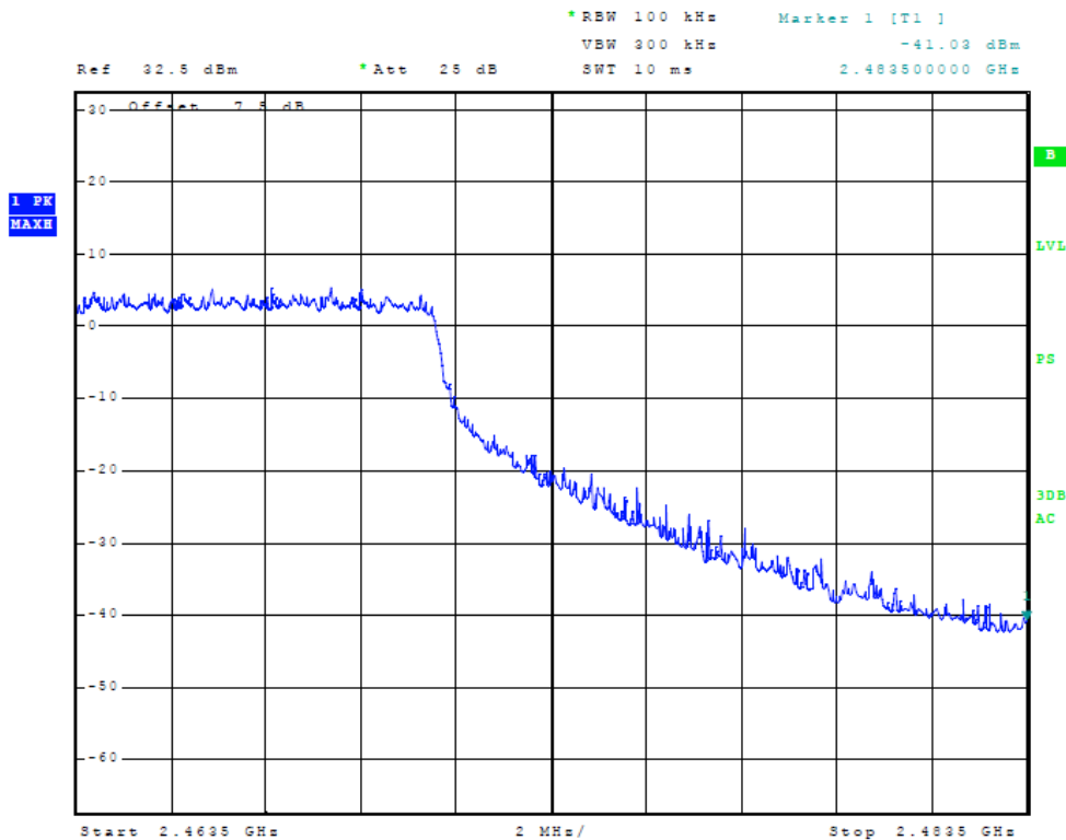
Figure 39 Plot of Upper Band Edge
