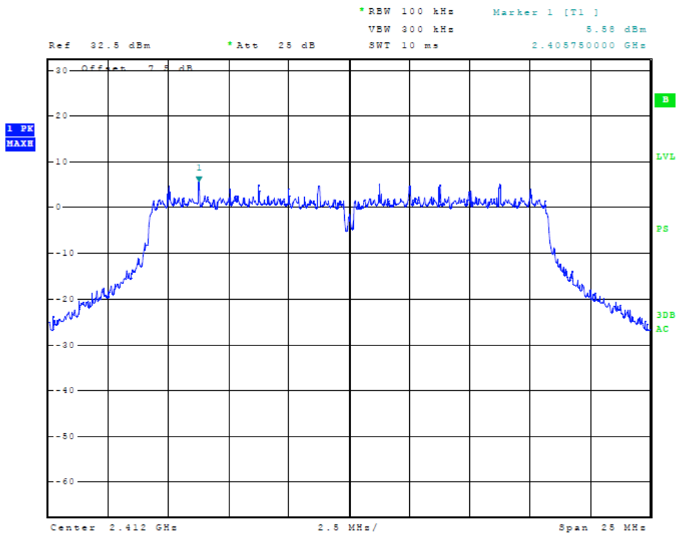
Figure 31 Plot of Power Spectral Density (20 MHz Mode, 2412 MHz)
