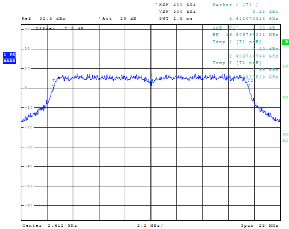
Figure 16 Plot of 6dB Band width (20 MHz Mode, 2412 MHz)
