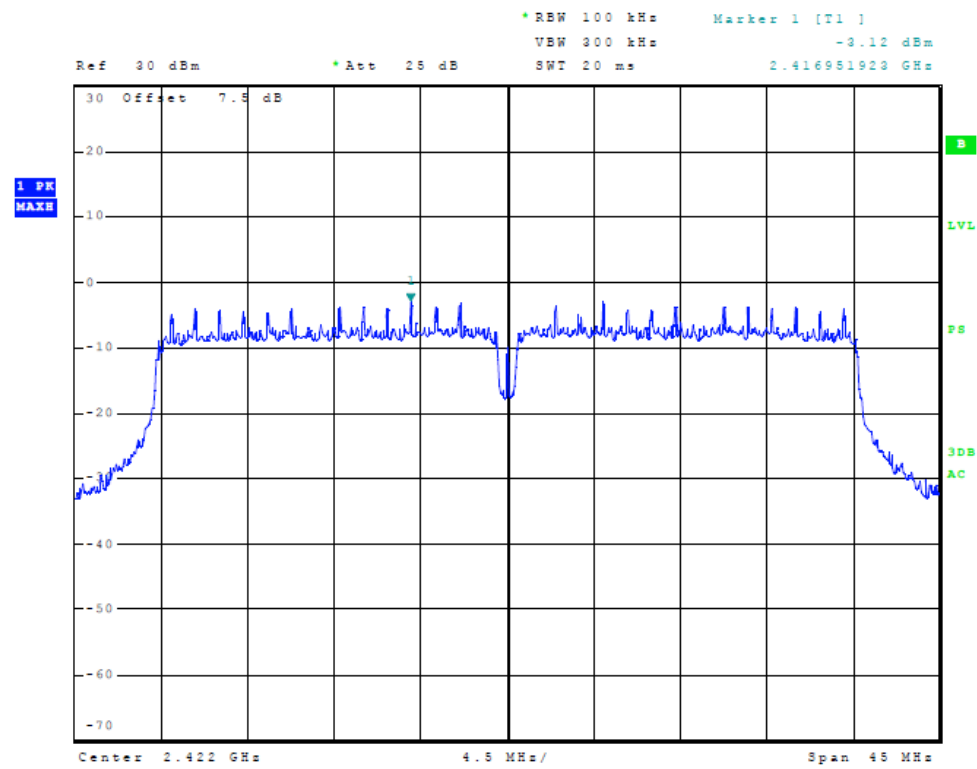
Figure 35 Plot of Power Spectral Density (40 MHz Mode, 2422 MHz)
