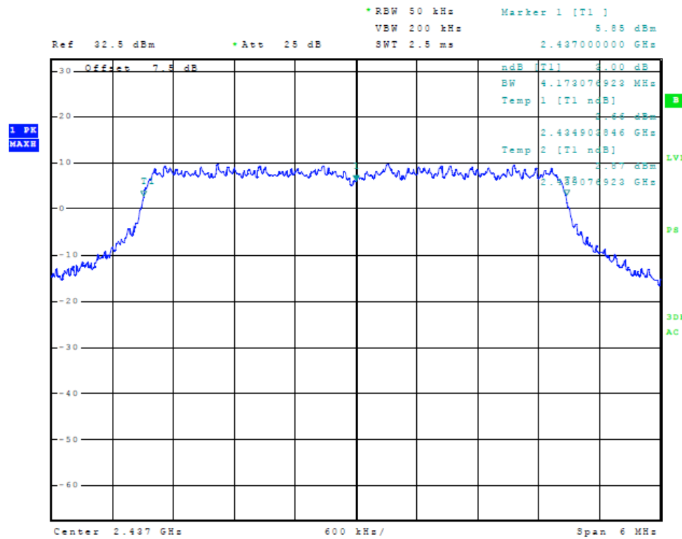
Figure 9 Plot of 6dB Band width (5 MHz Mode, 2437 MHz)
