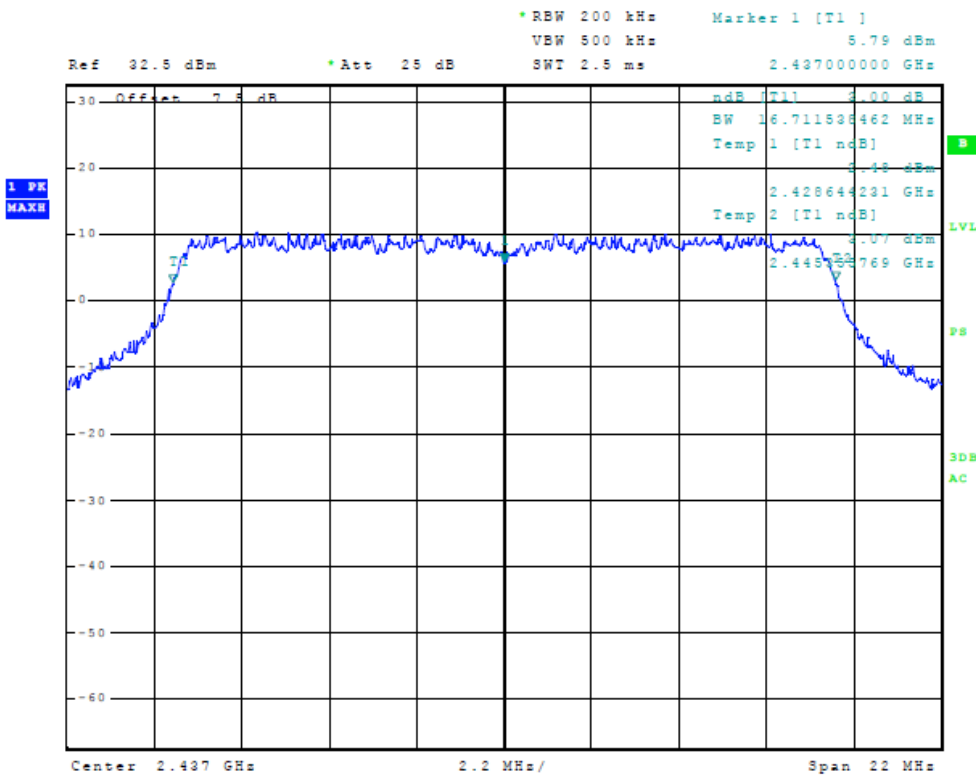
Figure 17 Plot of 6dB Band width (20 MHz Mode, 2437 MHz)
