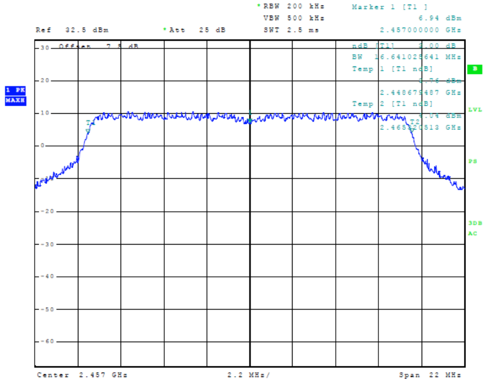
Figure 18 Plot of 6dB Band width (20 MHz Mode, 2457 MHz)
