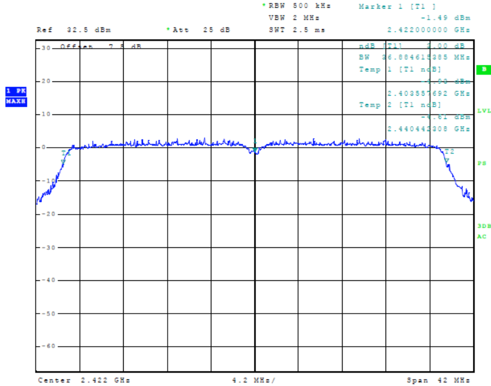
Figure 20 Plot of 6dB Band width (40 MHz Mode, 2422 MHz)
