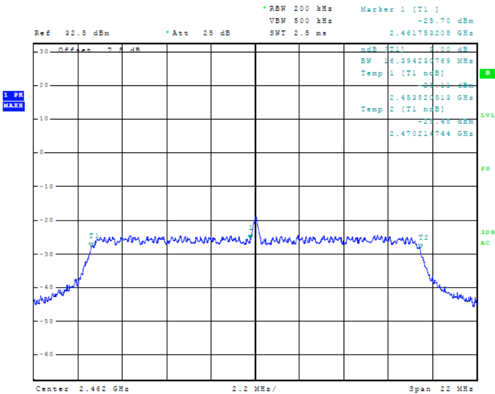
Figure 19 Plot of 6dB Band width (20 MHz Mode, 2462 MHz)
