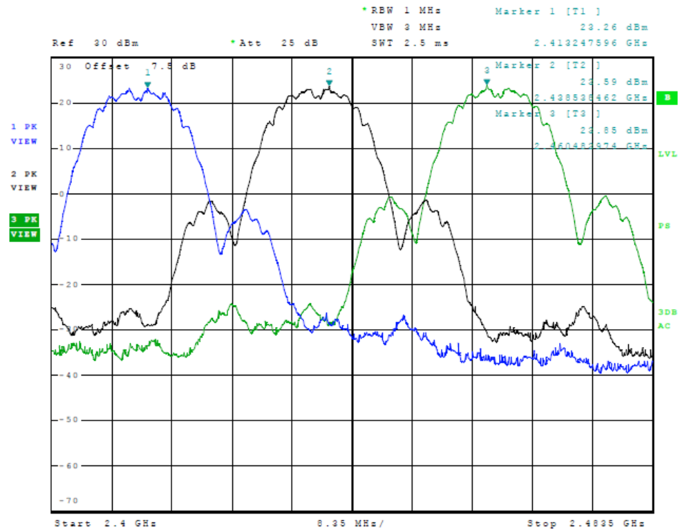
Figure 6 Plot of Output Across Operational Band (20 MHz, B/G/N Mode)
