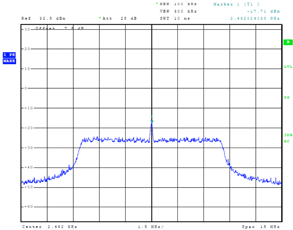
Figure 30 Plot of Power Spectral Density (10 MHz Mode, 2462 MHz)
