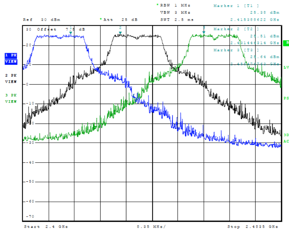
Figure 5 Plot of Output Across Operational Band (20 MHz Mode)
