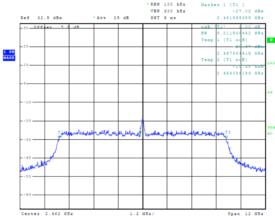
Figure 15 Plot of 6dB Band width (10 MHz Mode, 2462 MHz)
