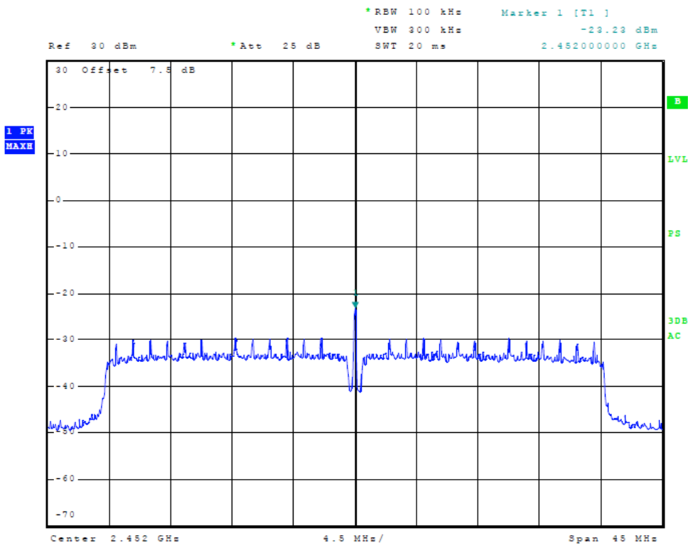
Figure 37 Plot of Power Spectral Density (40 MHz Mode, 2452 MHz)
