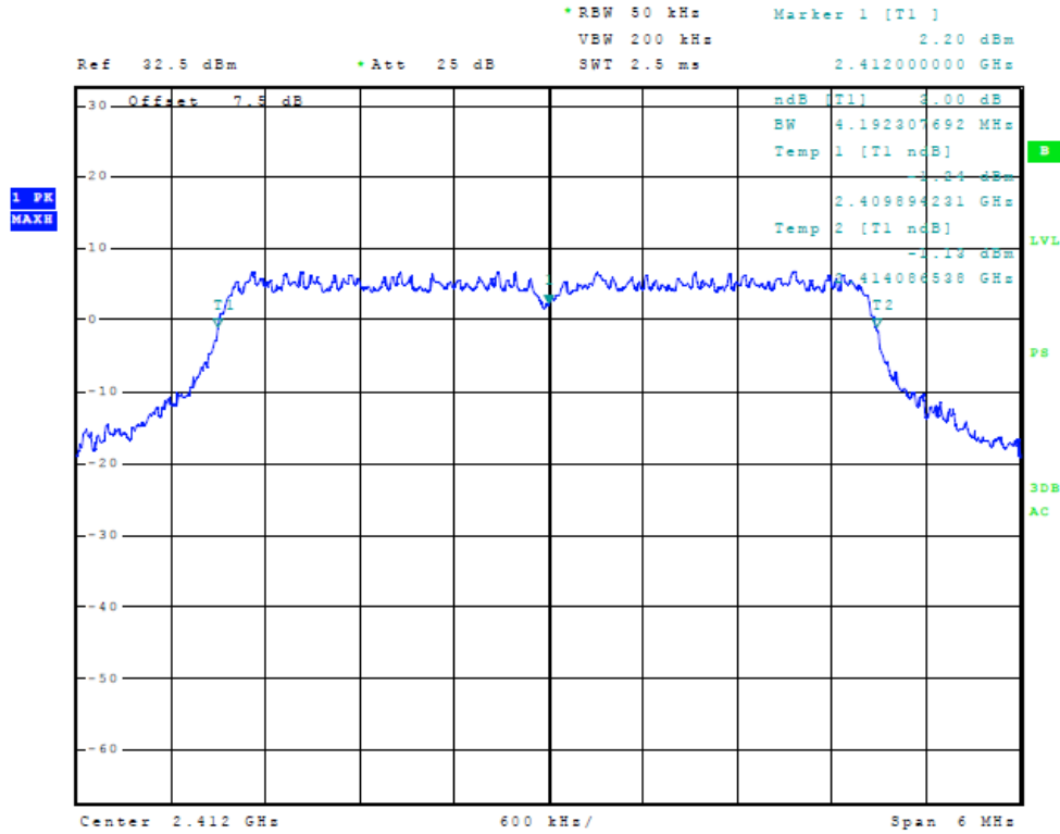
Figure 8 Plot of 6dB Band width (5 MHz Mode, 2412 MHz)
