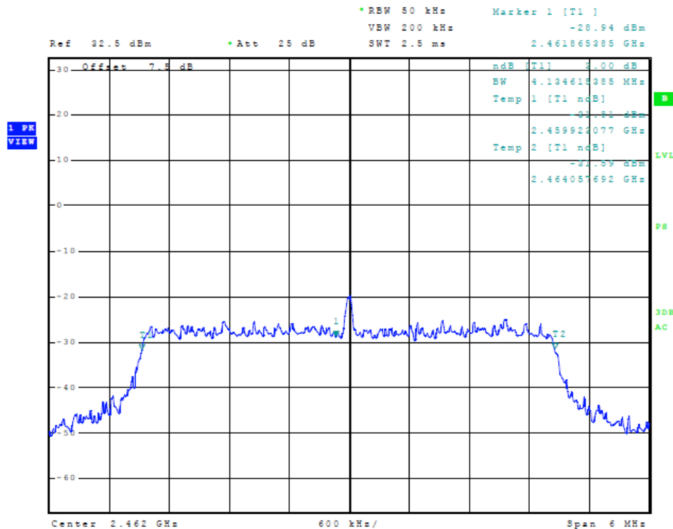
Figure 11 Plot of 6dB Band width (5 MHz Mode, 2462 MHz)
