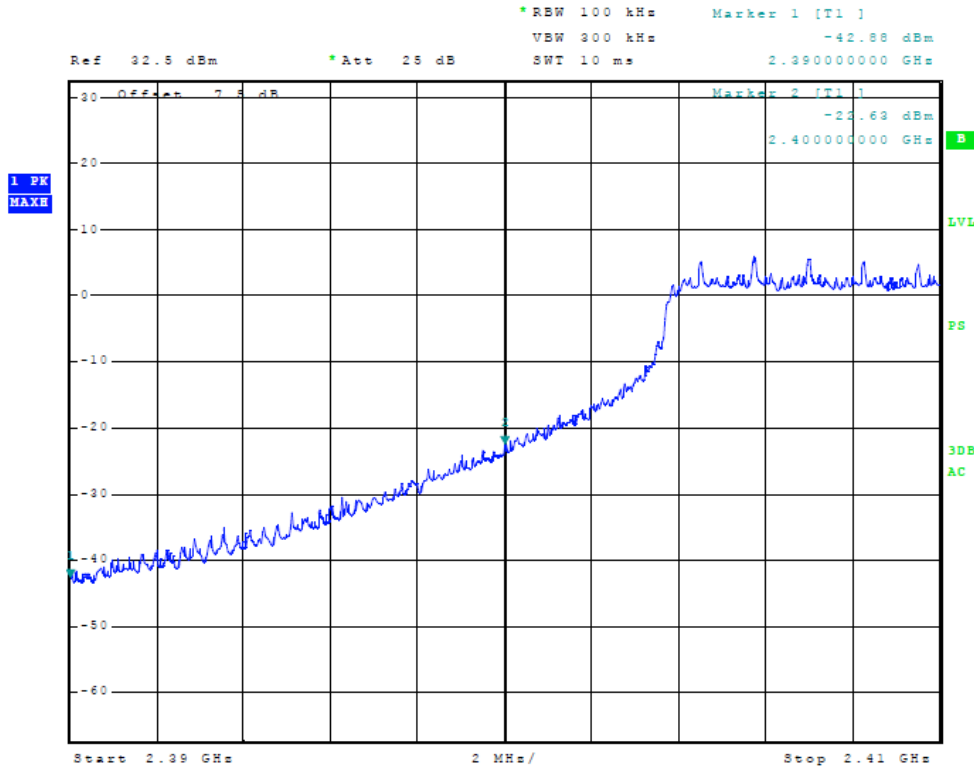
Figure 38 Plot of Lower Band Edge
