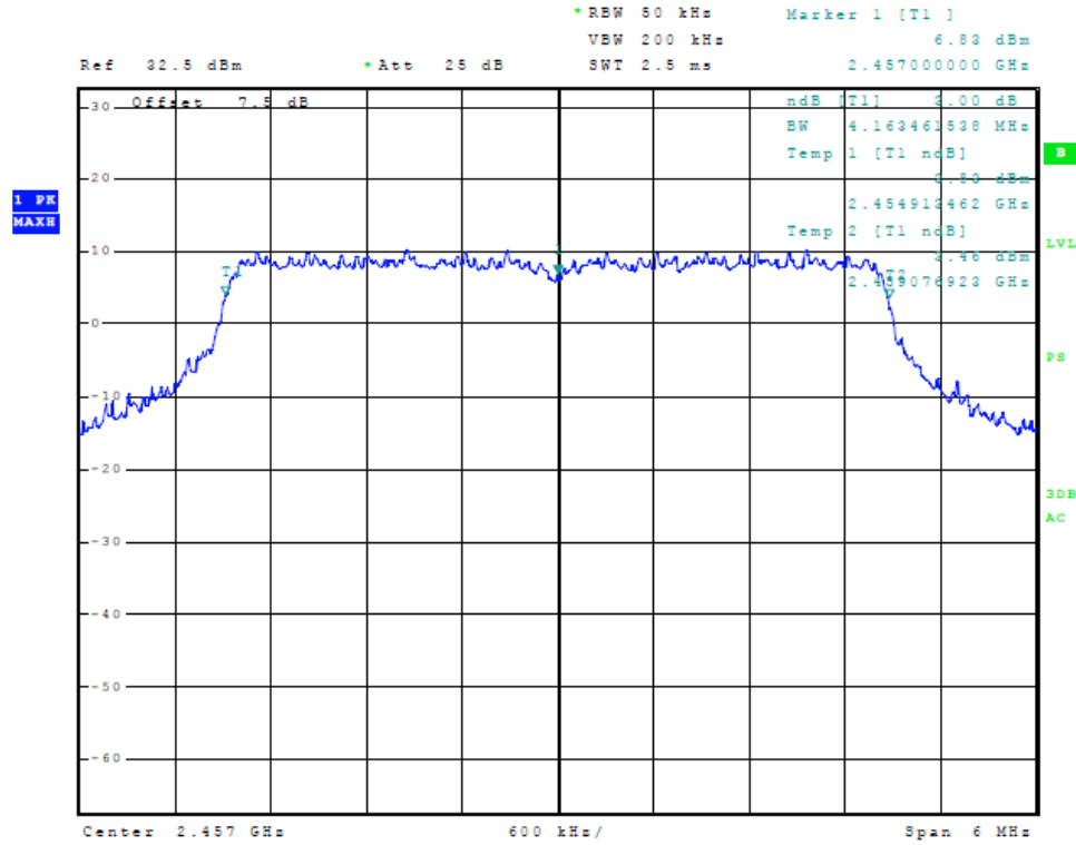
Figure 10 Plot of 6dB Band width (5 MHz Mode, 2457 MHz)
