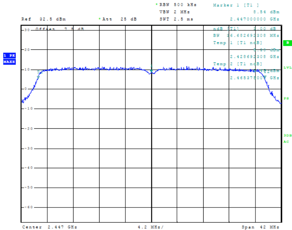
Figure 21 Plot of 6dB Band width (40 MHz Mode, 2447 MHz)
