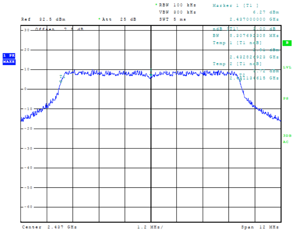
Figure 13 Plot of 6dB Band width (10 MHz Mode, 2437 MHz)
