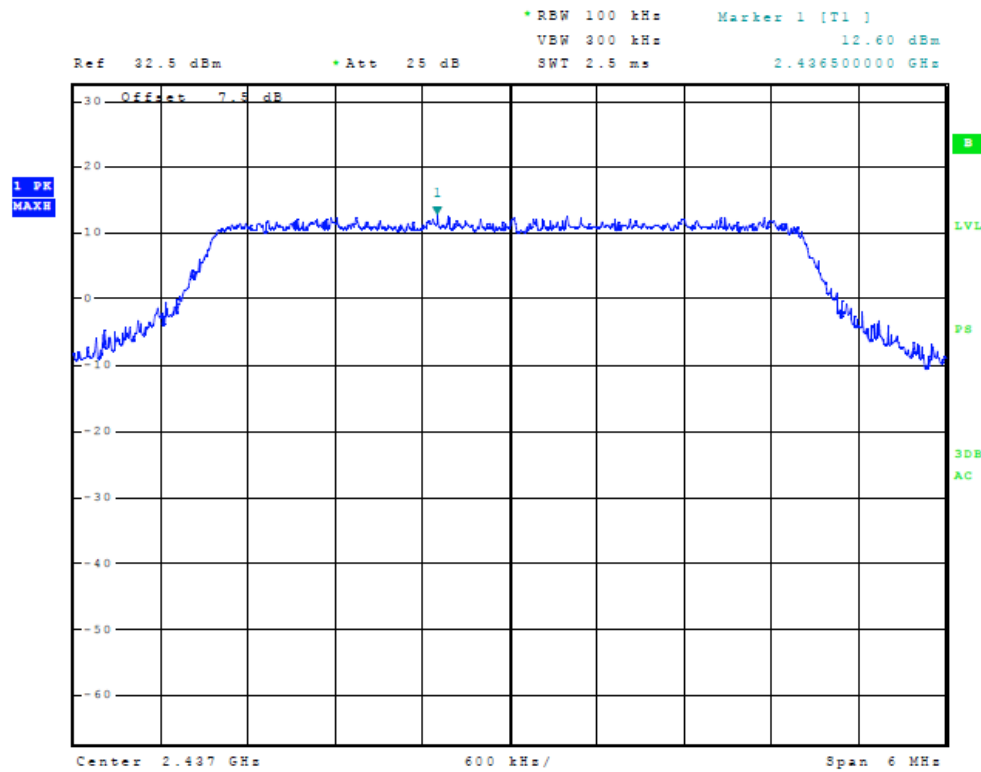
Figure 24 Plot Power Spectral Density (5 MHz Mode, 2437 MHz)
