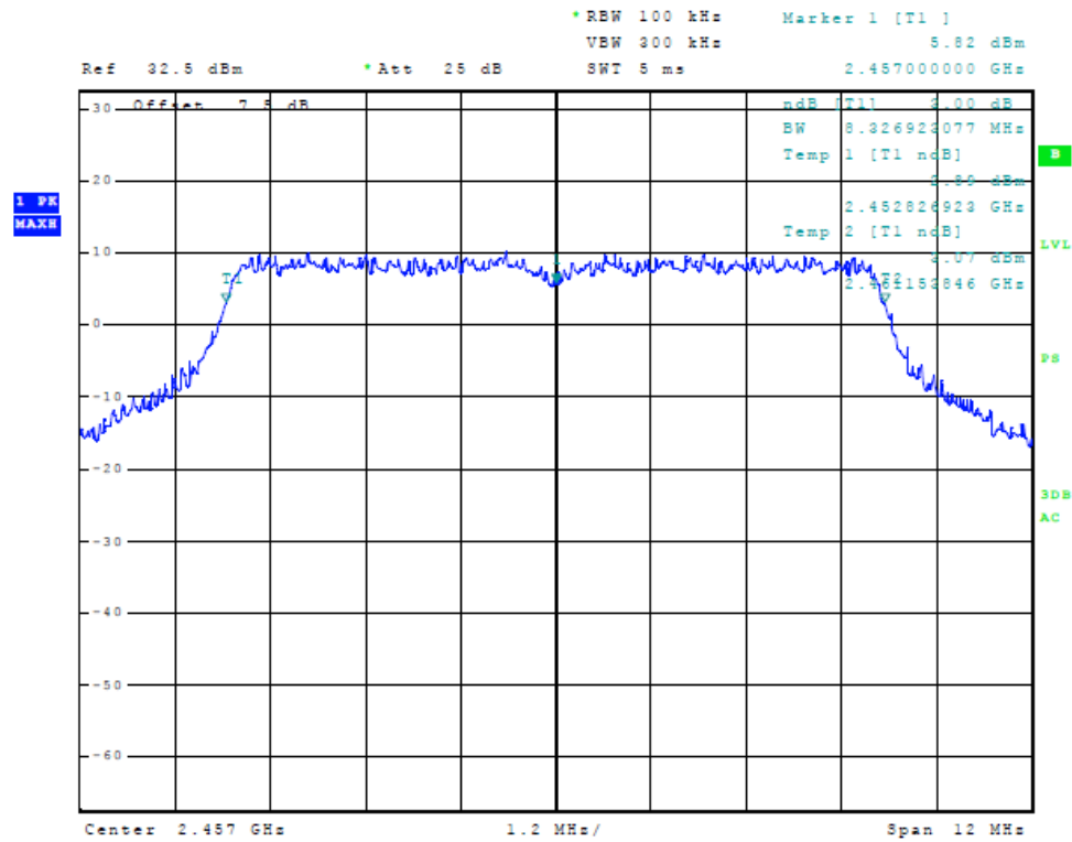
Figure 14 Plot of 6dB Band width (10 MHz Mode, 2457 MHz)
