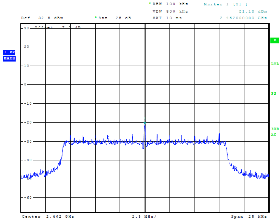
Figure 34 Plot of Power Spectral Density (20 MHz Mode, 2462 MHz)
