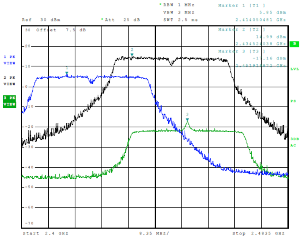
Figure 7 Plot of Output Across Operational Band (40 MHz Mode)
