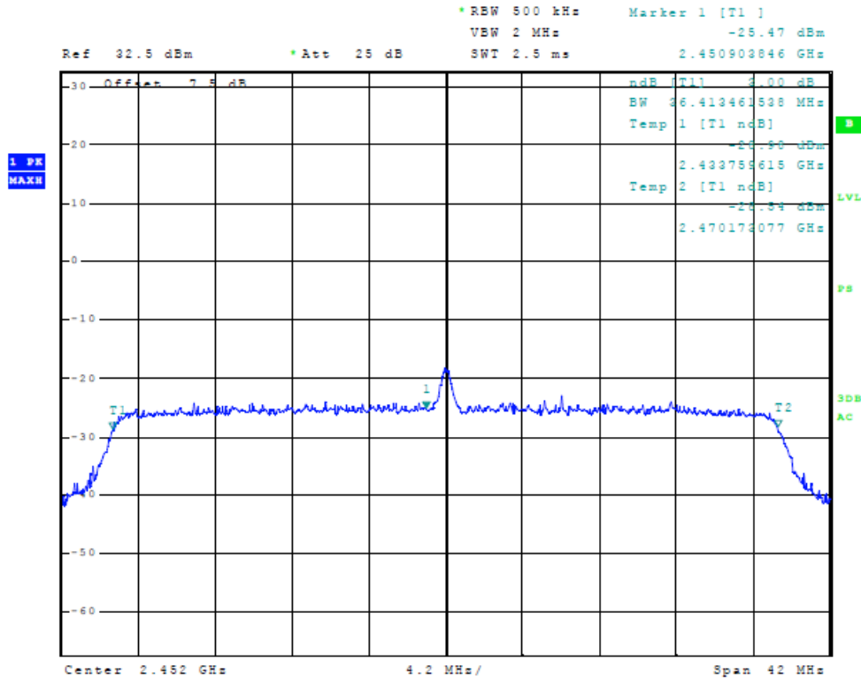
Figure 22 Plot of 6dB Band width (40 MHz Mode, 2452 MHz)
