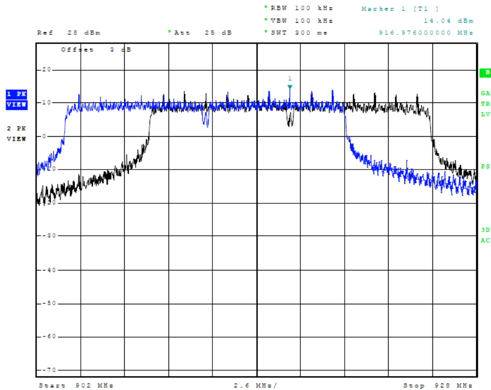
Figure 4 Plot of Transmitter Emissions (Across Operational Band, g Mode)
