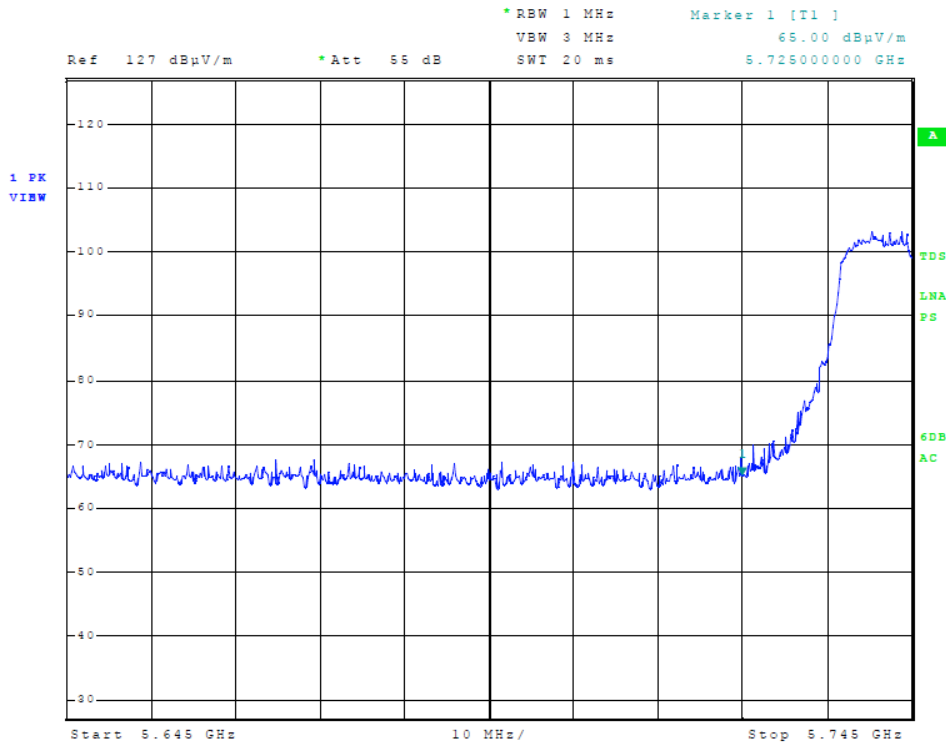
Figure 13 Plot of Transmitter Low Band Edge (5725-5850 MHz Band, 20 MHz Channel)
