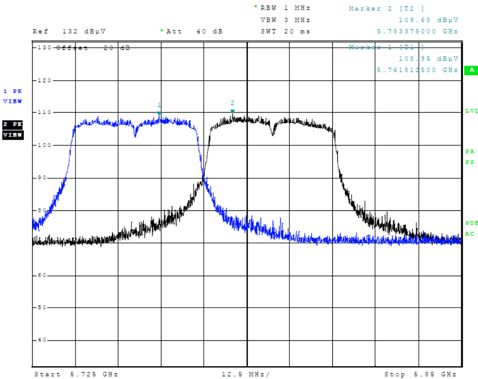
Figure 12 Plot of Transmitter Emissions (Across 5725-5850 MHz Band, 40 MHz Channel)
