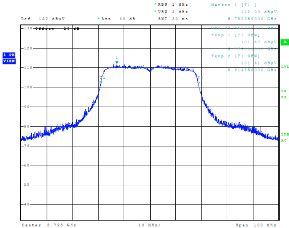
Figure 18 Plot of Transmitter Emissions (5725-5850 MHz Band, 40 MHz Channel, 99% OBW)
