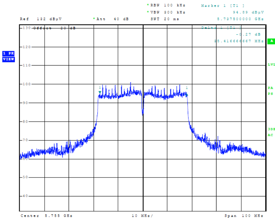
Figure 20 Plot of Transmitter Emissions (5725-5850 MHz Band, 40 MHz Channel, 6-dB OBW)
