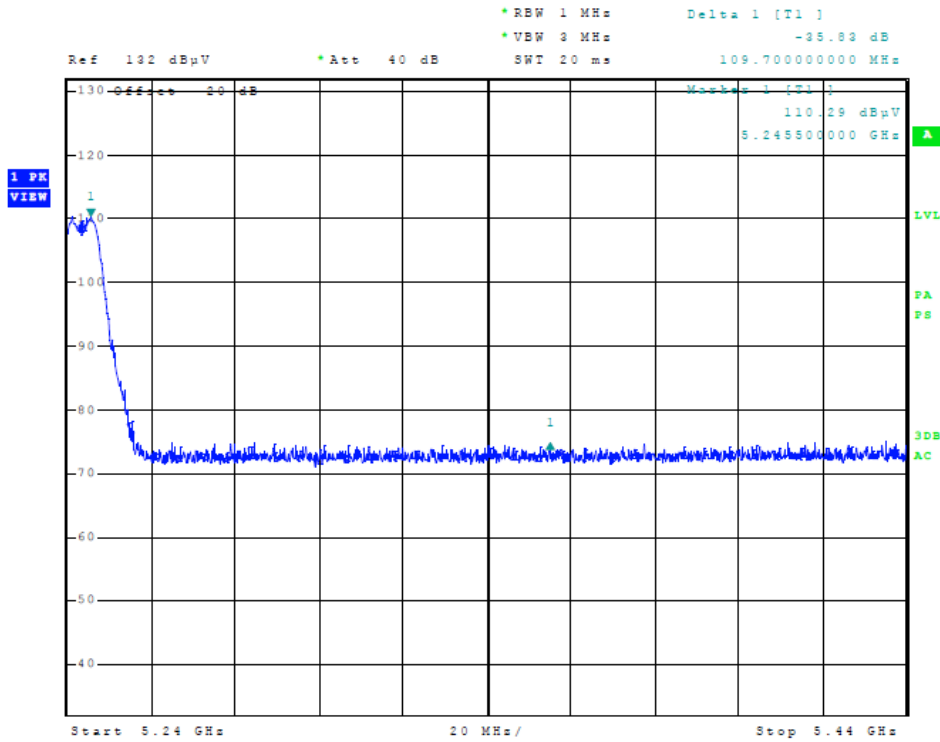
Figure 7 Plot of Transmitter High Band Edge (5150-5250 MHz Band, 20 MHz Channel)
