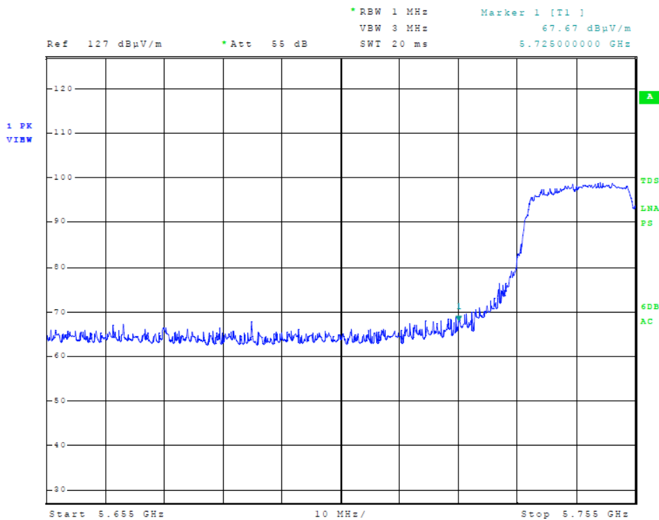
Figure 14 Plot of Transmitter Low Band Edge (5725-5850 MHz Band, 40 MHz Channel)
