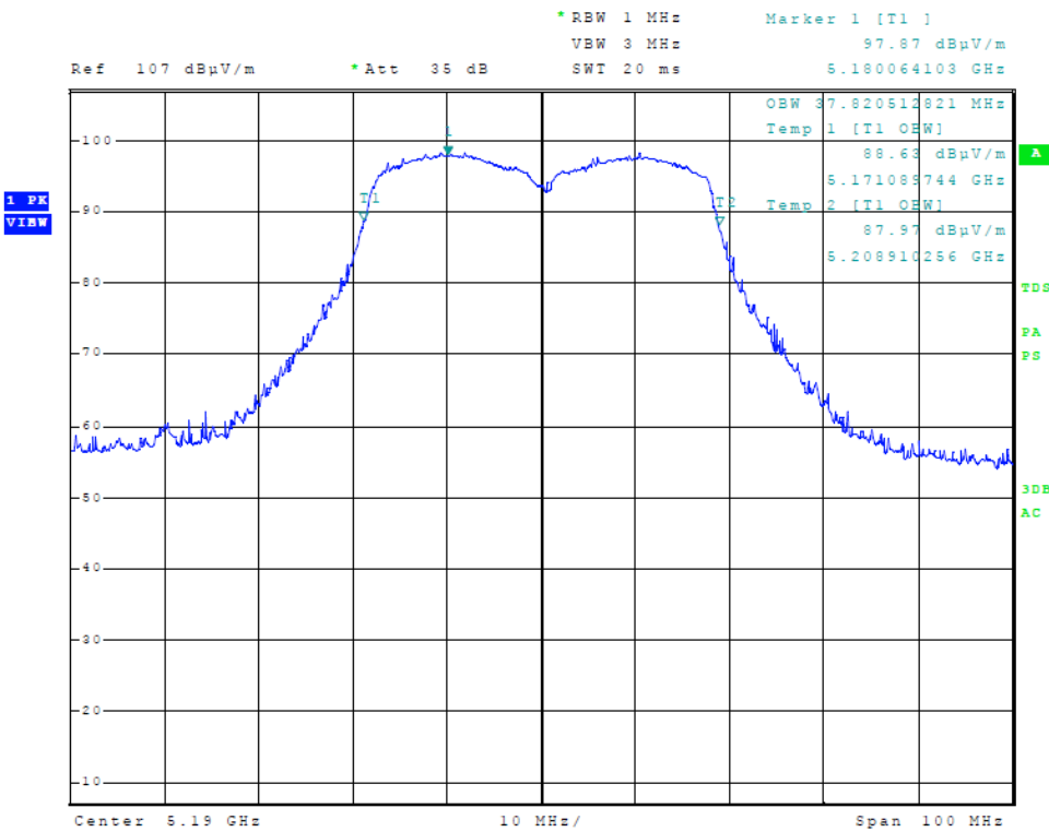
Figure 10 Plot of Transmitter Emissions (5150-5250 MHz Band, 40 MHz Channel, 99% OBW)
