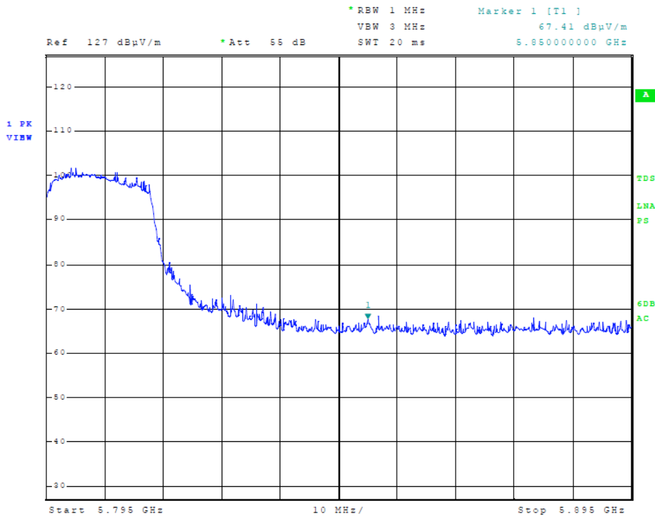
Figure 16 Plot of Transmitter High Band Edge (5725-5850 MHz Band, 40 MHz Channel)
