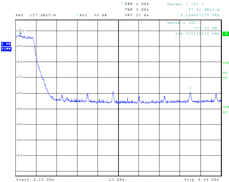
Figure 8 Plot of Transmitter High Band Edge (5150-5250 MHz Band, 40 MHz Channel)
