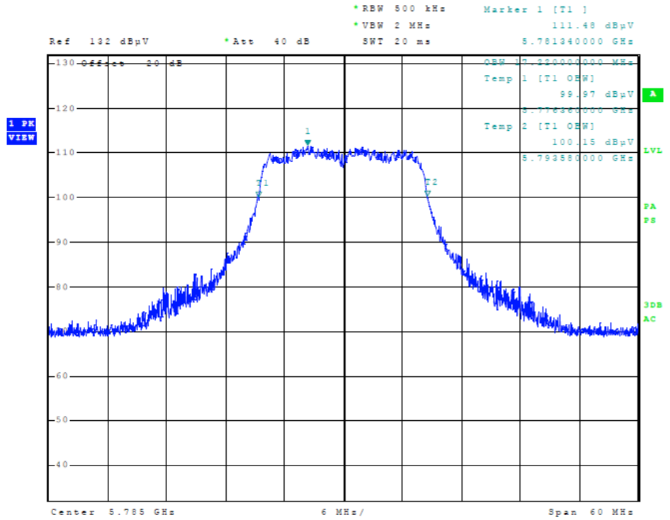
Figure 17 Plot of Transmitter Emissions (5725-5850 MHz Band, 20 MHz Channel, 99% OBW)
