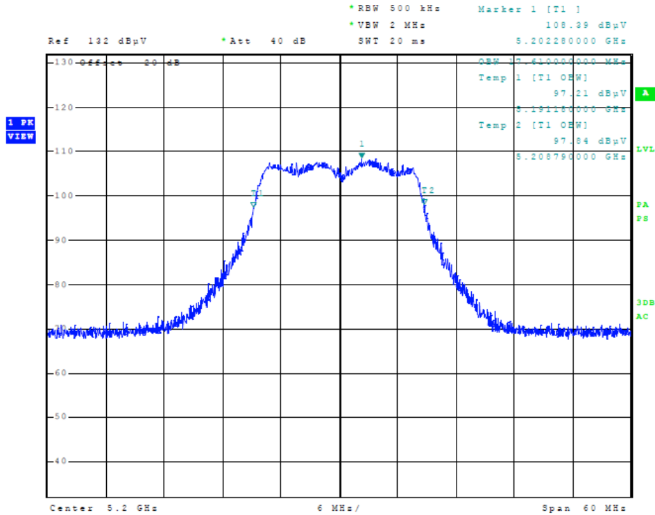
Figure 9 Plot of Transmitter Emissions (5150-5250 MHz Band, 20 MHz Channel, 99% OBW)
