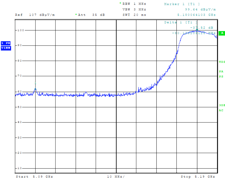
Figure 6 Plot of Transmitter Low Band Edge (5150-5250 MHz Band, 40 MHz Channel)
