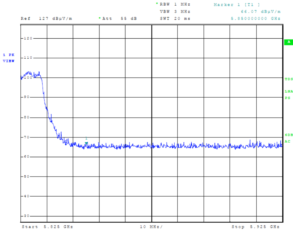
Figure 15 Plot of Transmitter High Band Edge (5725-5850 MHz Band, 20 MHz Channel)
