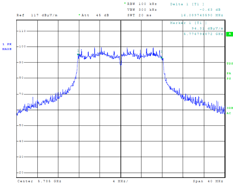
Figure 19 Plot of Transmitter Emissions (5725-5850 MHz Band, 20 MHz Channel, 6-dB OBW)
