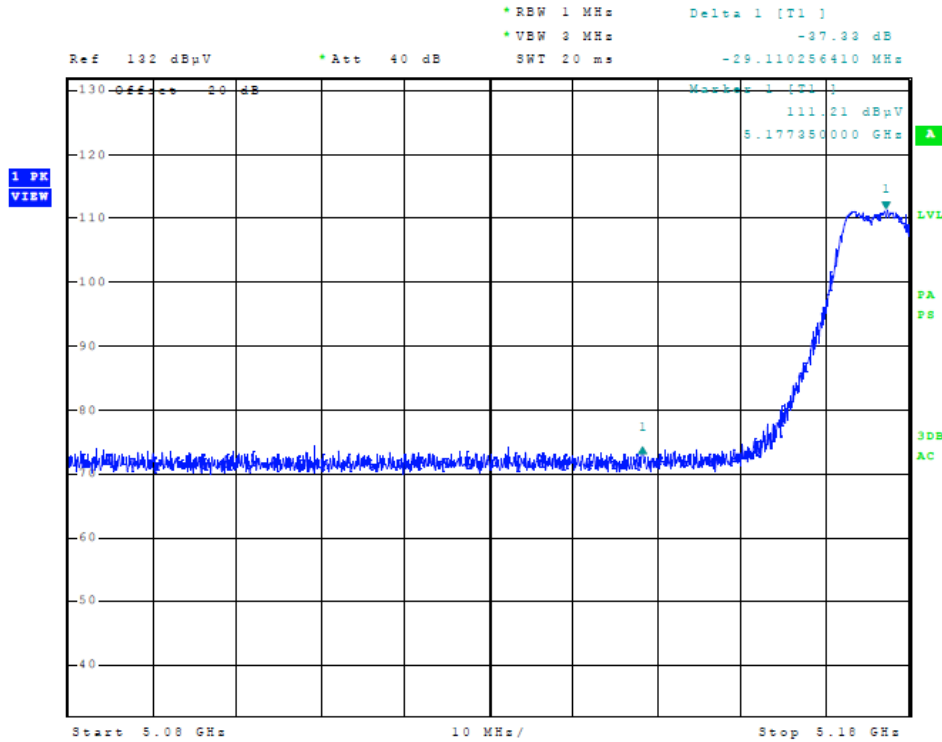
Figure 5 Plot of Transmitter Low Band Edge (5150-5250 MHz Band, 20 MHz Channel)
