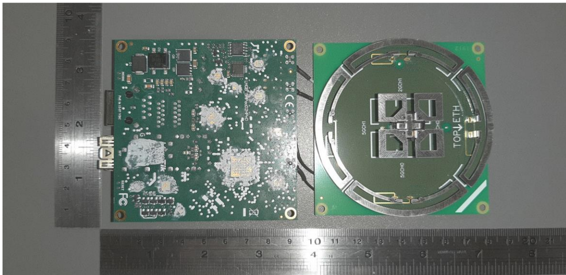
Figure 4 (Bottom view with shielding On and Antenna module attached)
