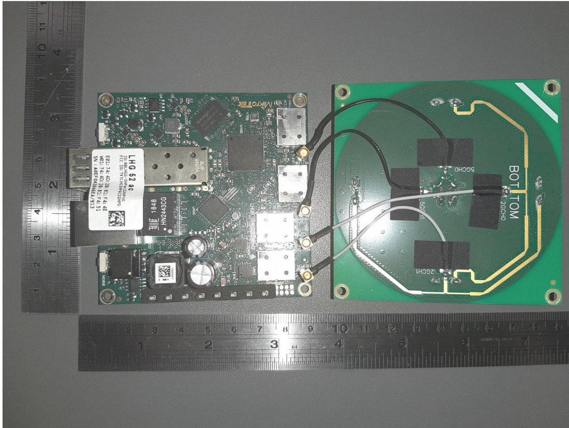
Figure 3 (Top view with shielding On and Antenna module attached)
