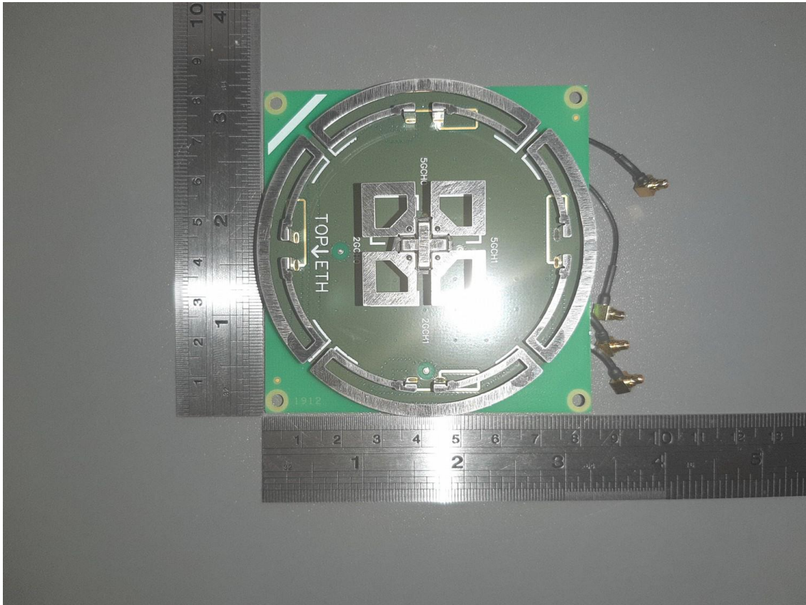
Figure 8 (Antenna module top view)
