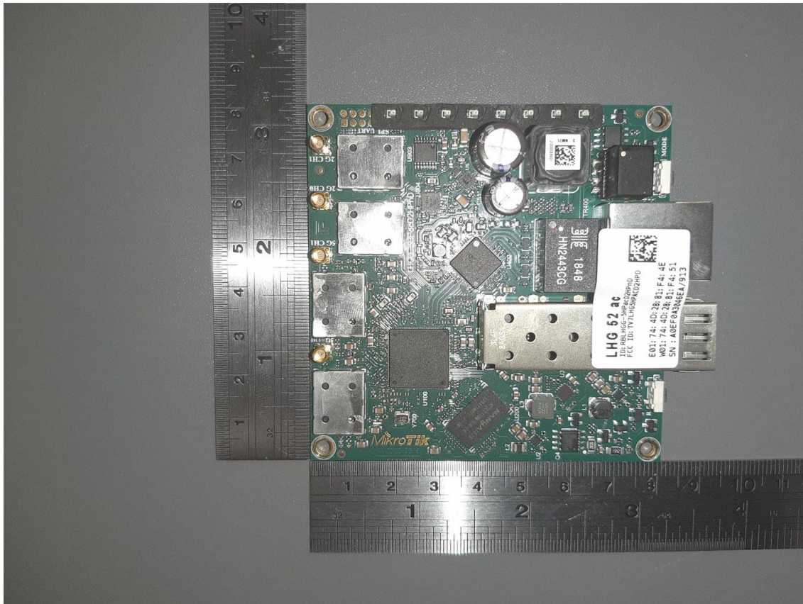
Figure 5 (Top view with shielding On)
