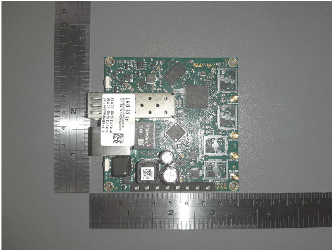
Figure 6 (Top view with shielding Off)
