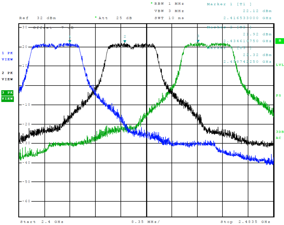
Figure 5 Plot of Transmitter Emissions (Across Operational Band, 802.11n (20))
