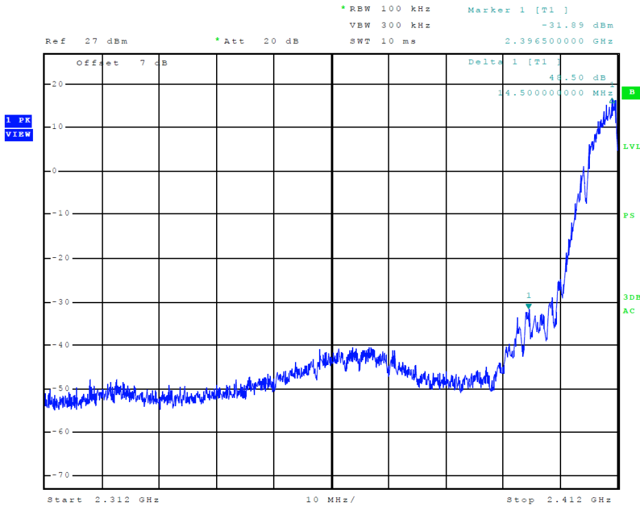
Figure 7 Plot of Transmitter Low Band Edge (802.11b)
