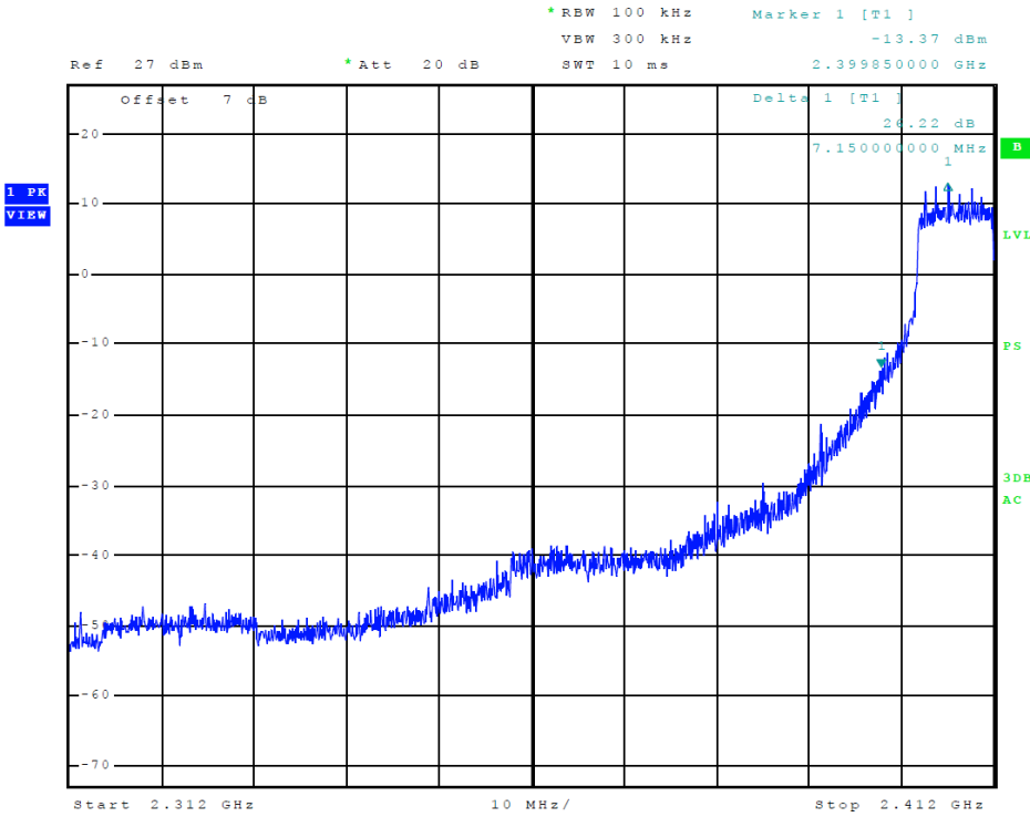
Figure 9 Plot of Transmitter Low Band Edge (802.11n (20))
