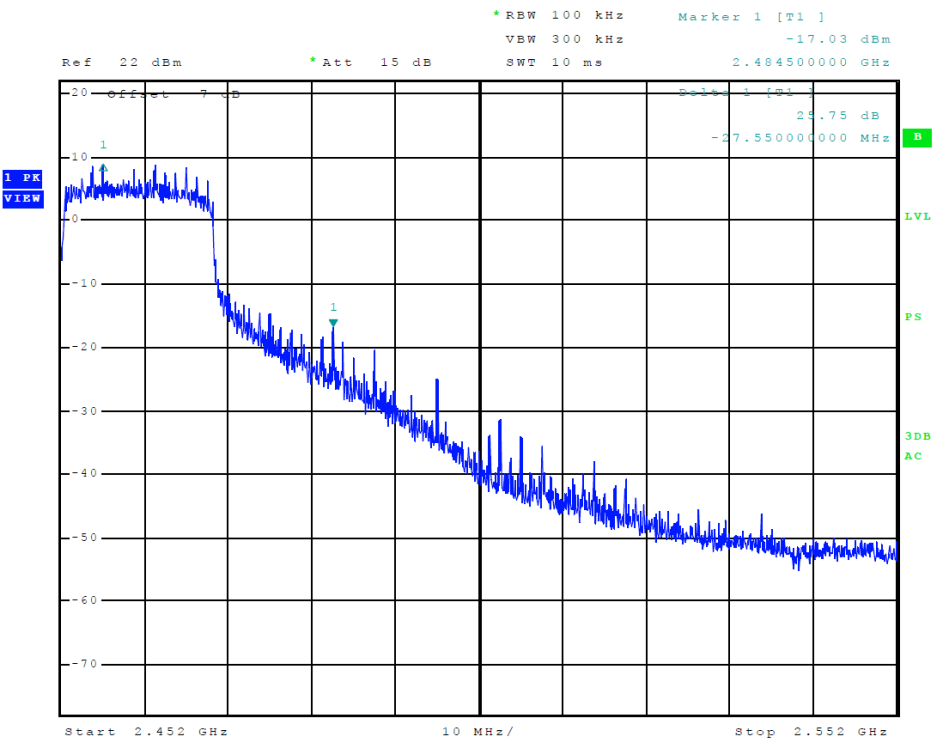
Figure 14 Plot of Transmitter High Band Edge (802.11n (40))
