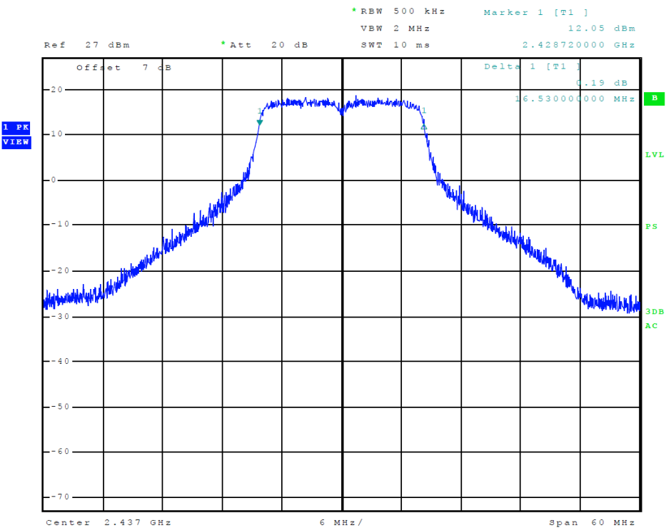
Figure 16 Plot of Transmitter 6-dB Occupied Band Width (802.11g)
