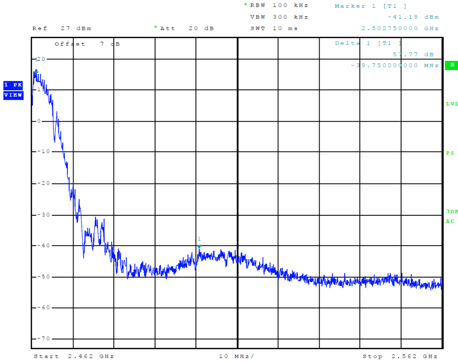
Figure 11 Plot of Transmitter High Band Edge (802.11b)
