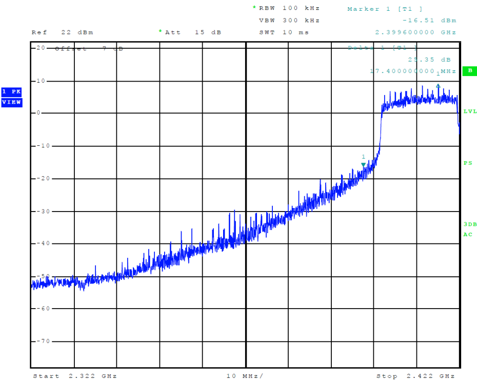
Figure 10 Plot of Transmitter Low Band Edge (802.11n (40))
