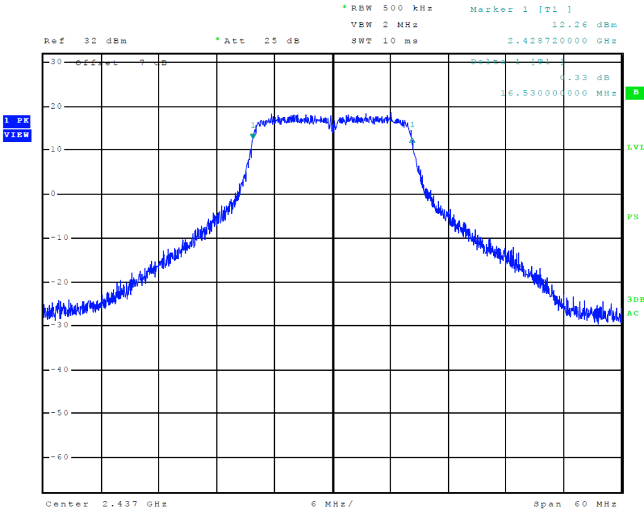
Figure 17 Plot of Transmitter 6-dB Occupied Band Width (802.11n (20))
