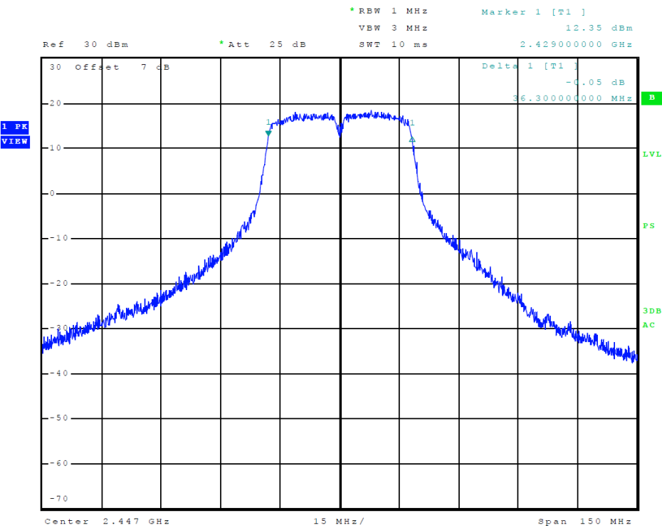
Figure 18 Plot of Transmitter 6-dB Occupied Band Width (802.11n (40))
