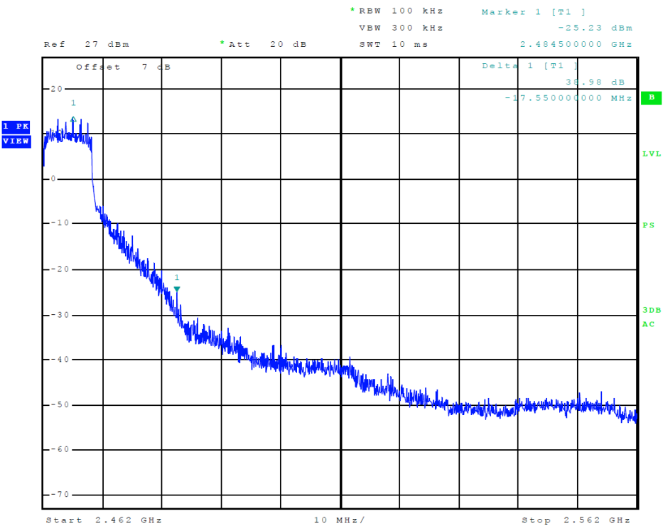
Figure 12 Plot of Transmitter High Band Edge (802.11g)
