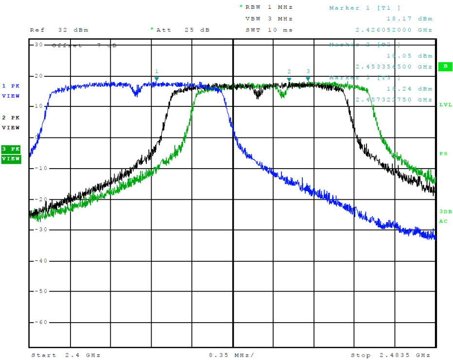
Figure 6 Plot of Transmitter Emissions (Across Operational Band, 802.11n (40))
