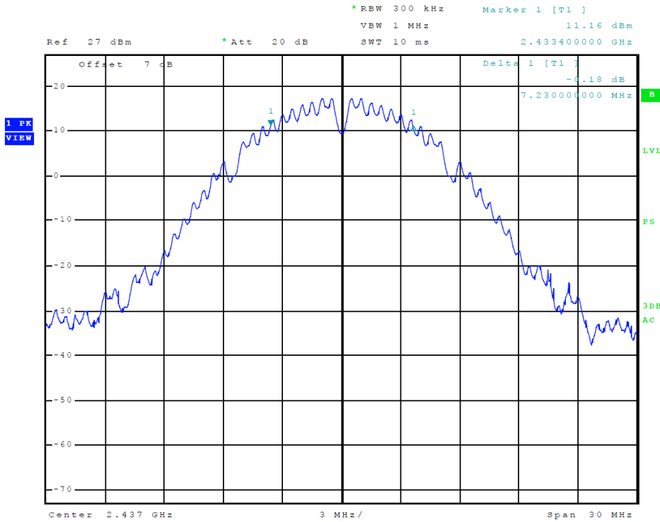
Figure 15 Plot of Transmitter 6-dB Occupied Band Width (802.11b)
