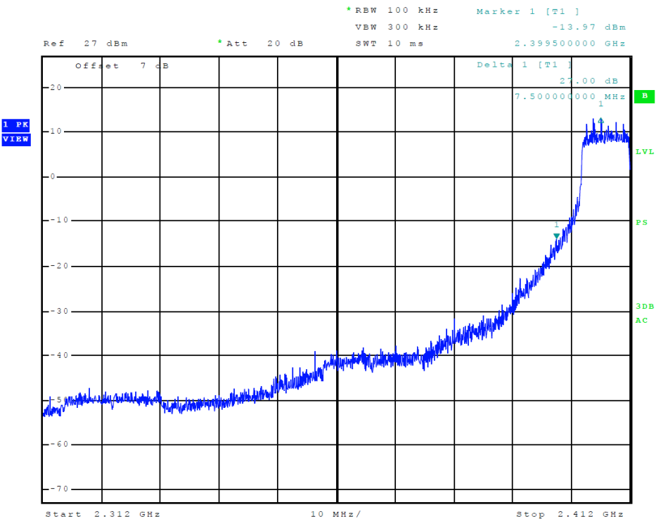
Figure 8 Plot of Transmitter Low Band Edge (802.11g)
