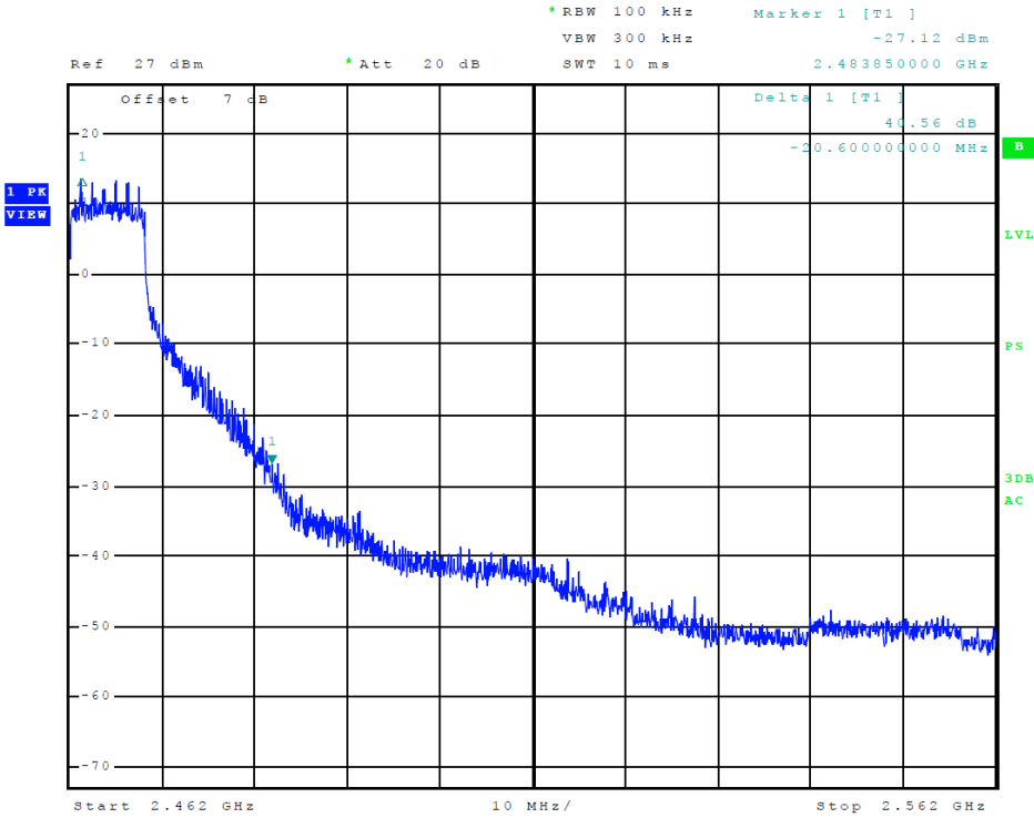
Figure 13 Plot of Transmitter High Band Edge (802.11n (20))
