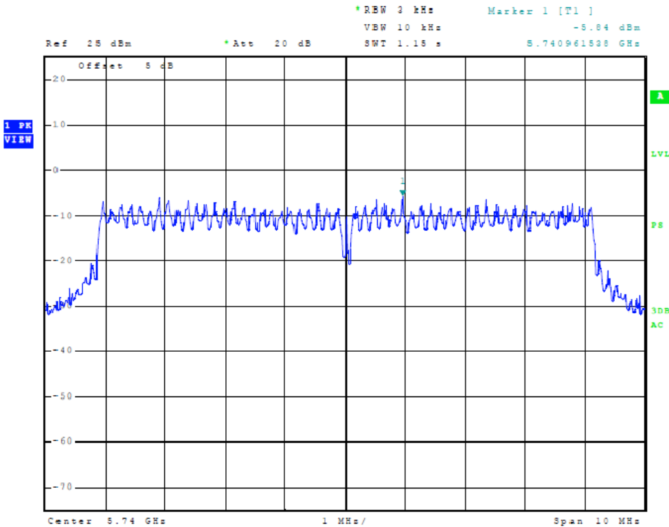
Figure Thirty-three Plot of Power Spectral Density (10 MHz Mode, 5740 MHz)
