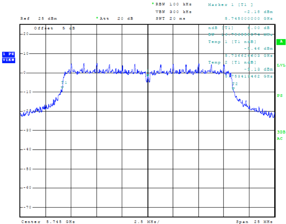
Figure Twenty-seven Plot of 6dB Band width (20 MHz Mode, 5745 MHz)
