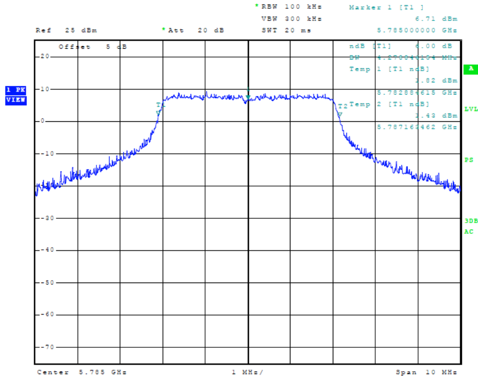
Figure Twenty-two Plot of 6dB Band width (5 MHz Mode, 5785 MHz)
