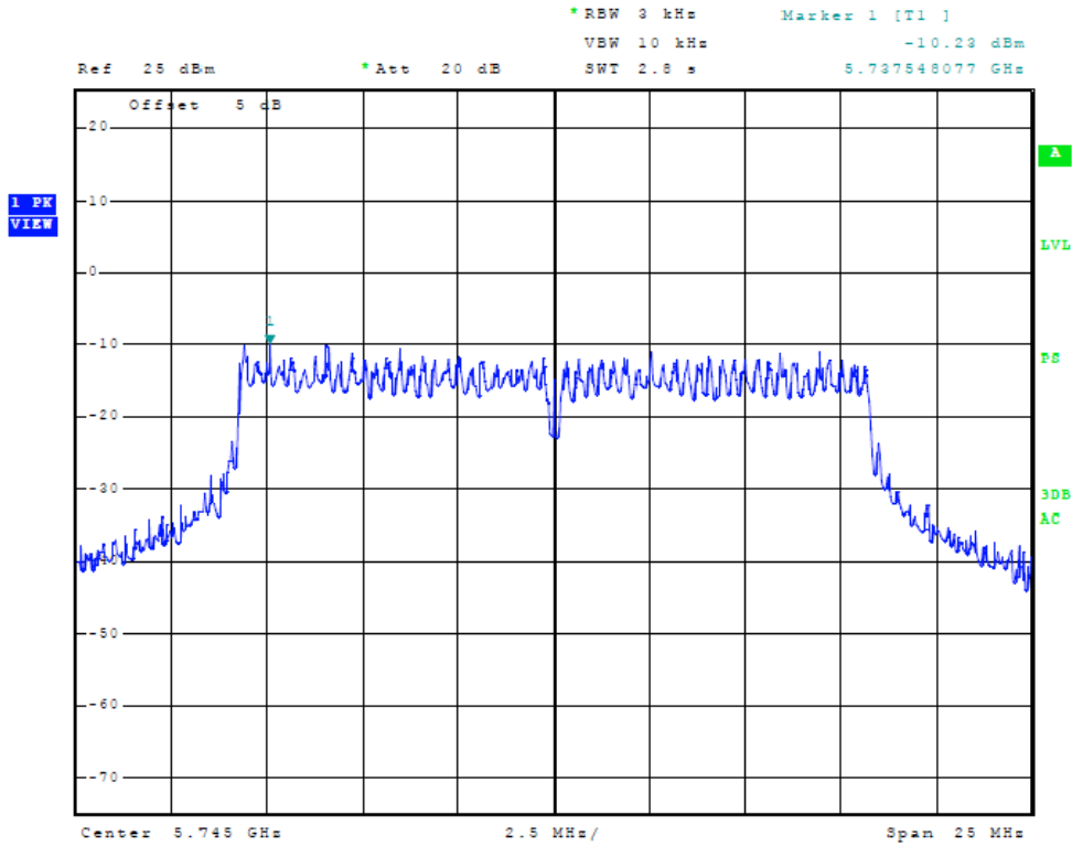
Figure Thirty-six Plot of Power Spectral Density (20 MHz Mode, 5745 MHz)
