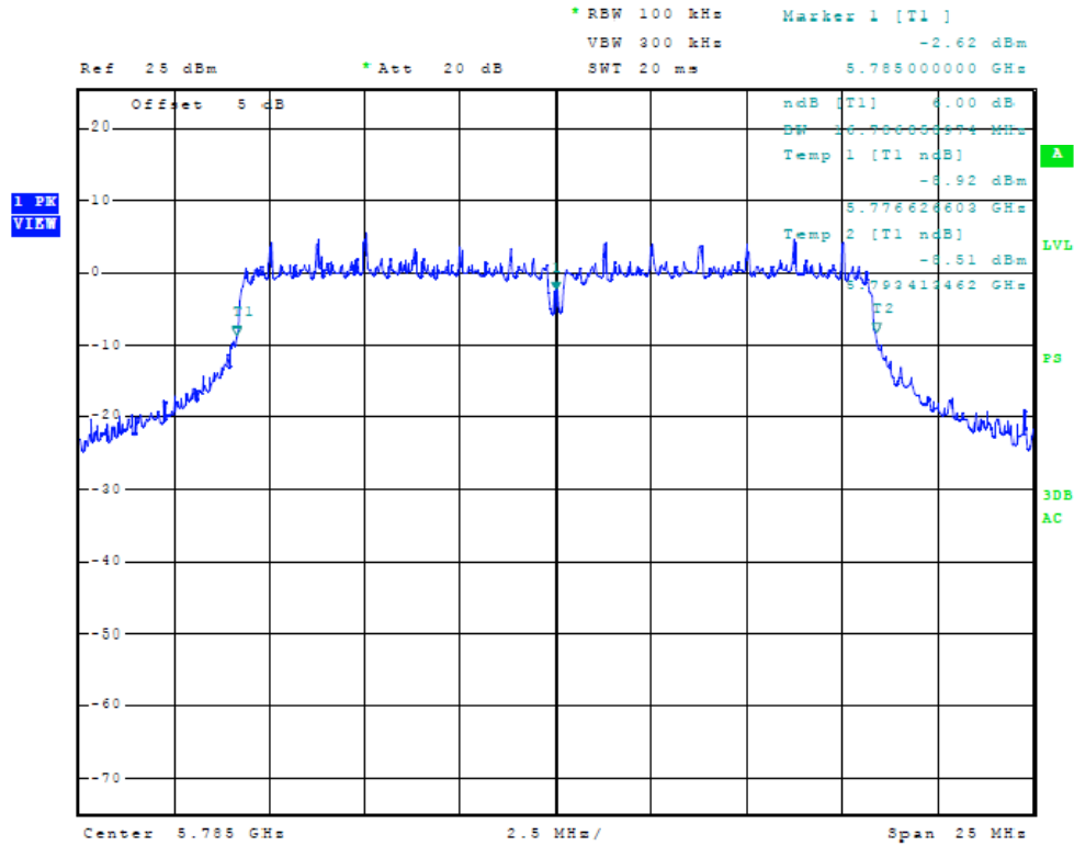
Figure Twenty-eight Plot of 6dB Band width (20 MHz Mode, 5785 MHz)
