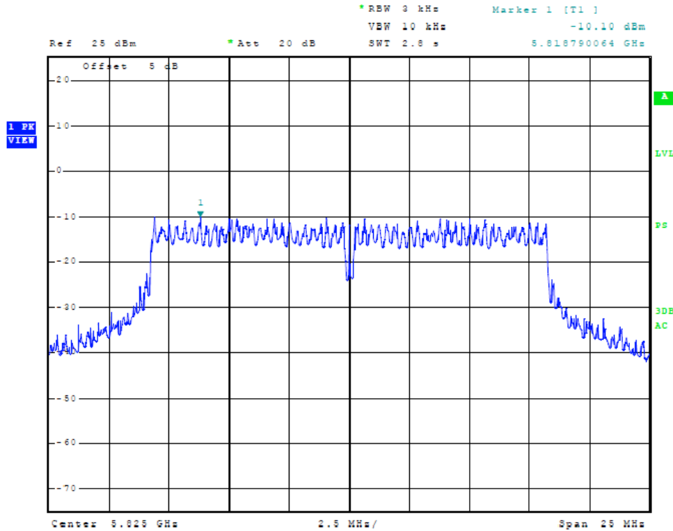
Figure Thirty-eight Plot of Power Spectral Density (20 MHz Mode, 5825 MHz) Transmitter Antenna Conducted Emissions Data
