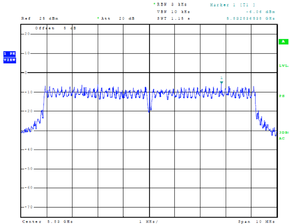
Figure Thirty-five Plot of Power Spectral Density (10 MHz Mode, 5830 MHz)
