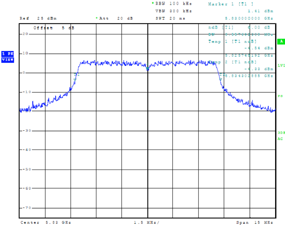
Figure Twenty-six Plot of 6dB Band width (10 MHz Mode, 5830 MHz)
