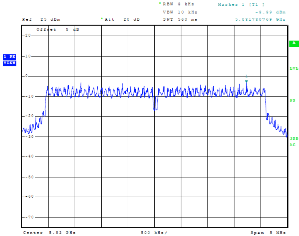
Figure Thirty-two Plot of Power Spectral Density (5 MHz Mode, 5830 MHz)
