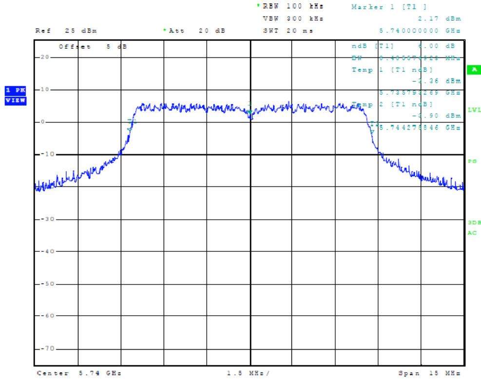
Figure Twenty-four Plot of 6dB Band width (10 MHz Mode, 5740 MHz)
