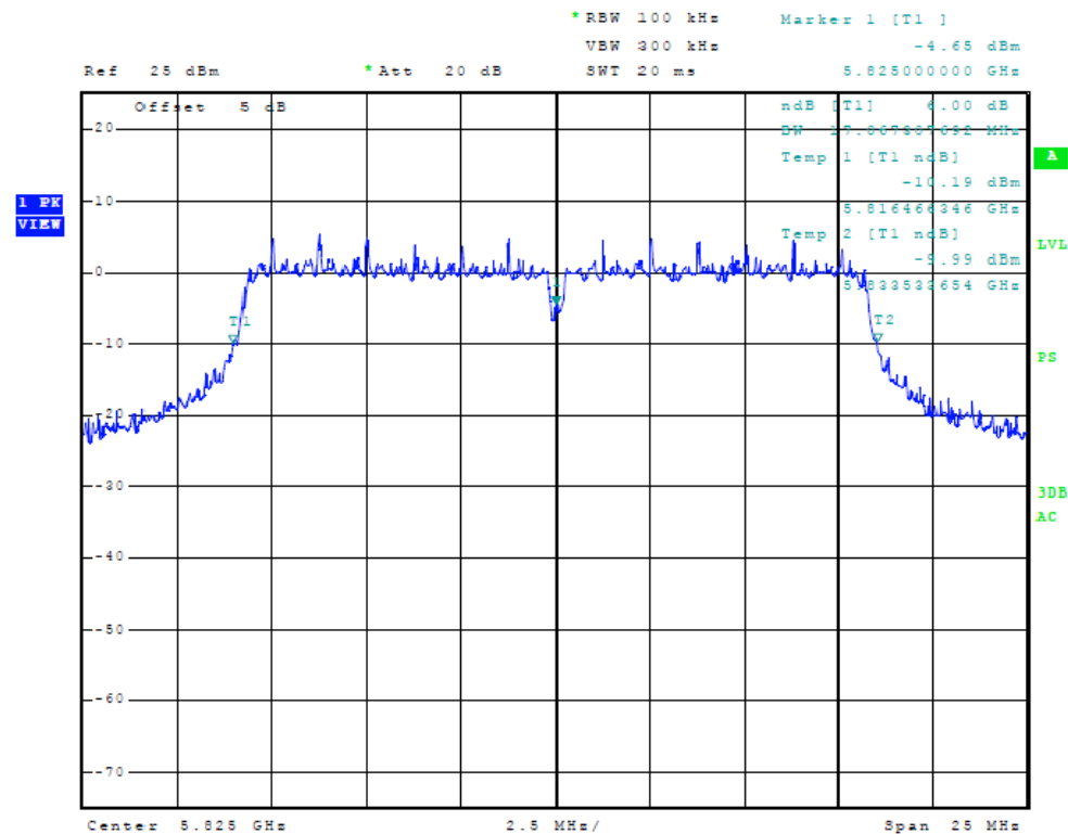
Figure Twenty-nine Plot of 6dB Band width (20 MHz Mode, 5825 MHz)
