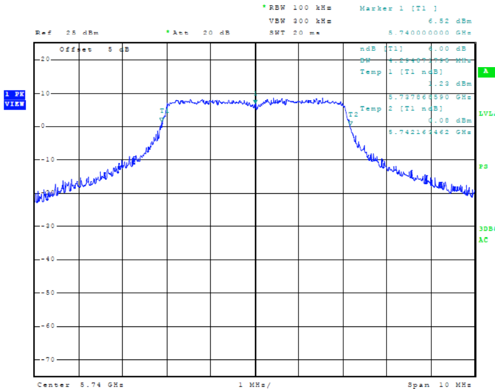
Figure Twenty-one Plot of 6dB Band width (5 MHz Mode, 5740 MHz)
