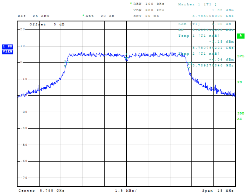
Figure Twenty-five Plot of 6dB Band width (10 MHz Mode, 5785 MHz)
