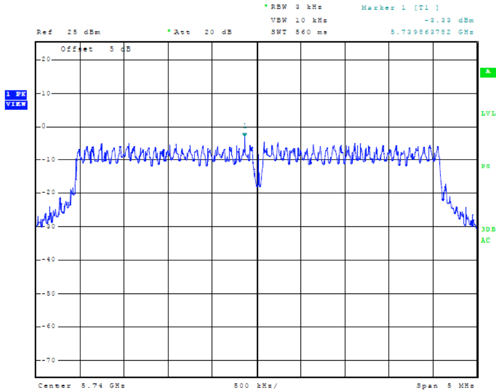
Figure Thirty Plot of Power Spectral Density (5 MHz Mode, 5740 MHz)
