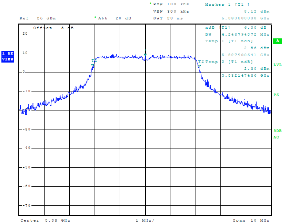
Figure Twenty-three Plot of 6dB Band width (5 MHz Mode, 5830 MHz)
