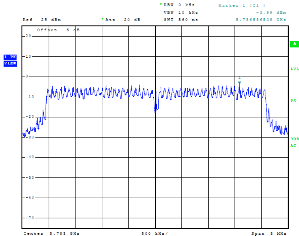
Figure Thirty-one Plot Power Spectral Density (5 MHz Mode, 5785 MHz)
