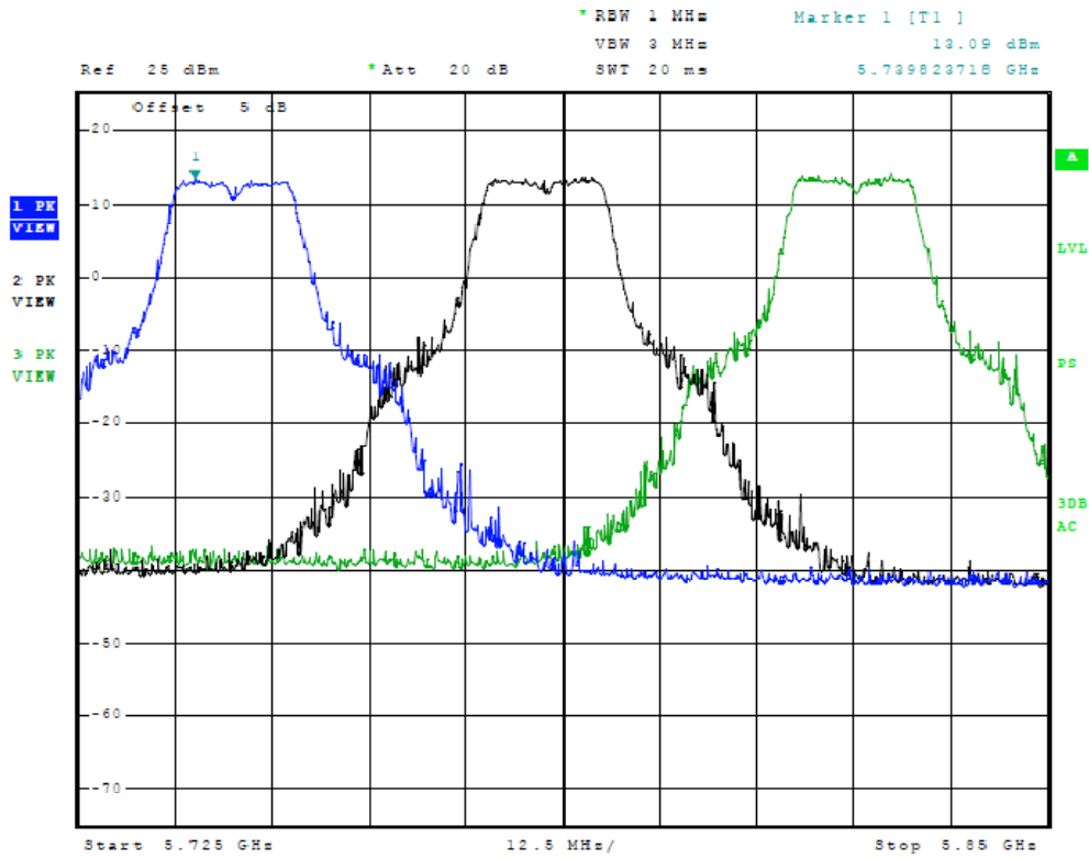
Figure Twenty Plot of Output Across Operational Band (20 MHz Mode)
