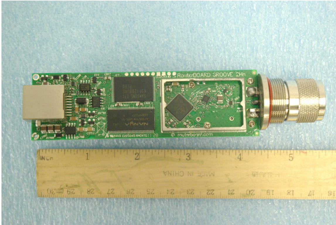
Backside of Heat Sink removed
