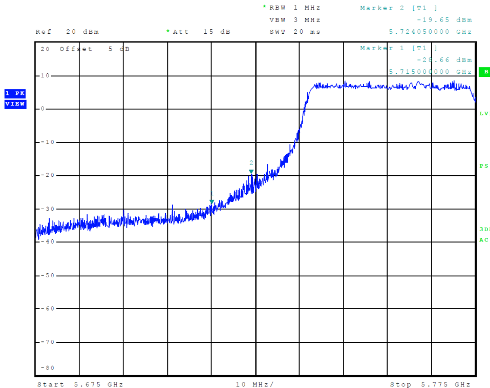
Figure 44 Plot of Transmitter Low Band Edge (Chain 1, 5725-5850 MHz Band, 802.11ac80)
