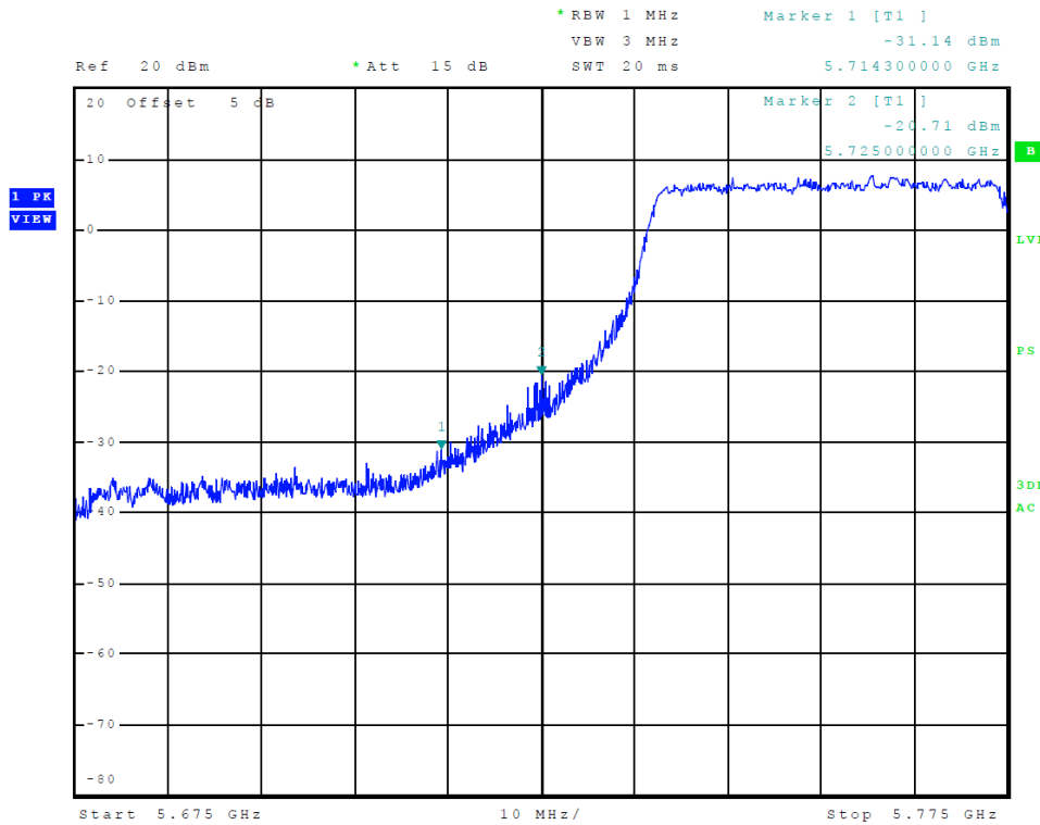
Figure 43 Plot of Transmitter Low Band Edge (Chain 0, 5725-5850 MHz Band, 802.11ac80)
