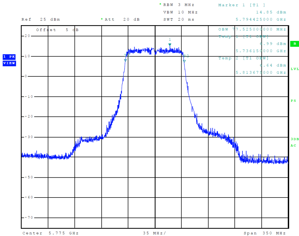
Figure 59 Plot of Transmitter Emissions (Chain 0, 5725-5850 MHz Band, 802.11ac80, 99% OBW)
