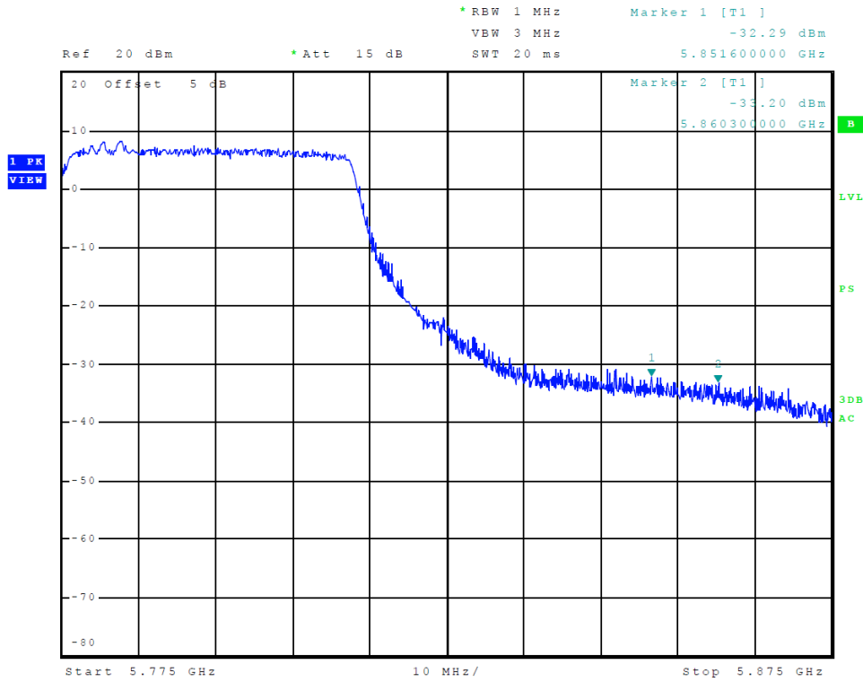
Figure 49 Plot of Transmitter High Band Edge (Chain 0, 5725-5850 MHz Band, 802.11ac80)
