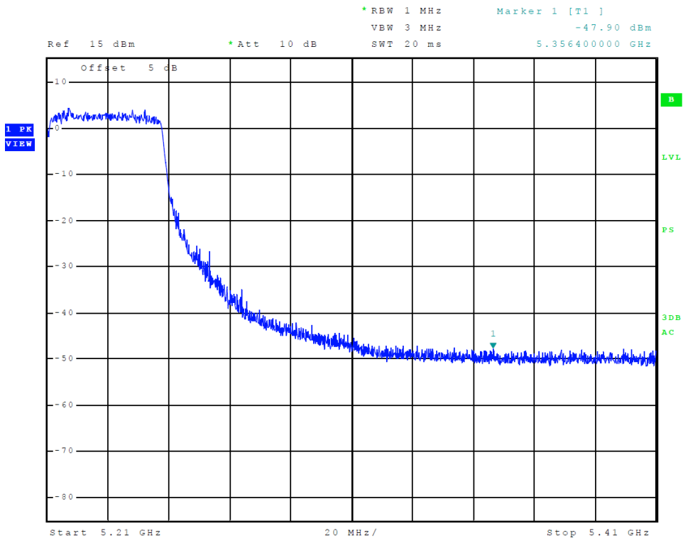
Figure 20 Plot of Transmitter High Band Edge (Chain 1, 5150-5250 MHz Band, 802.11ac80)
