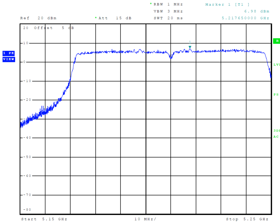
Figure 7 Plot of Transmitter Emissions (Chain 0, Across 5150-5250 MHz Band, 802.11ac80)
