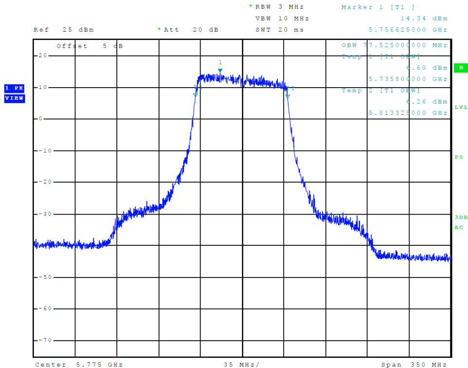
Figure 60 Plot of Transmitter Emissions (Chain 1, 5725-5850 MHz Band, 802.11ac80, 99% OBW)
