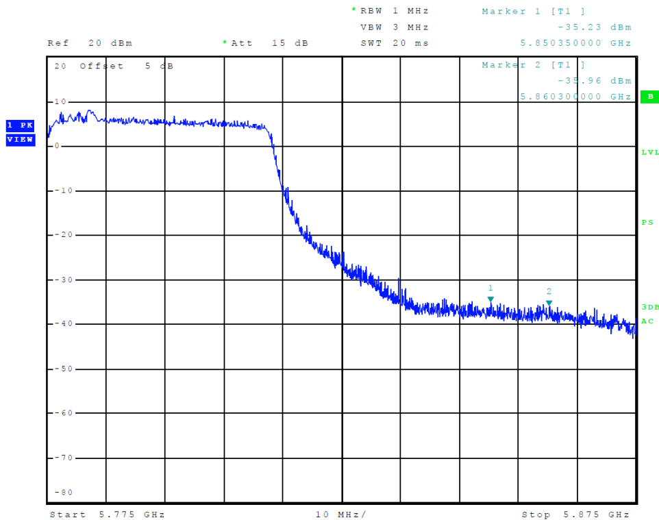
Figure 50 Plot of Transmitter High Band Edge (Chain 1, 5725-5850 MHz Band, 802.11ac80)
