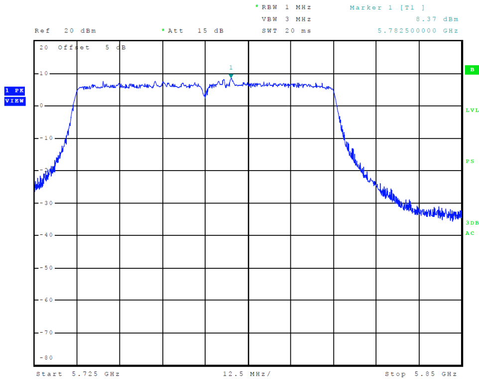
Figure 37 Plot of Transmitter Emissions (Chain 0, Across 5725-5850 MHz Band, 802.11ac80)
