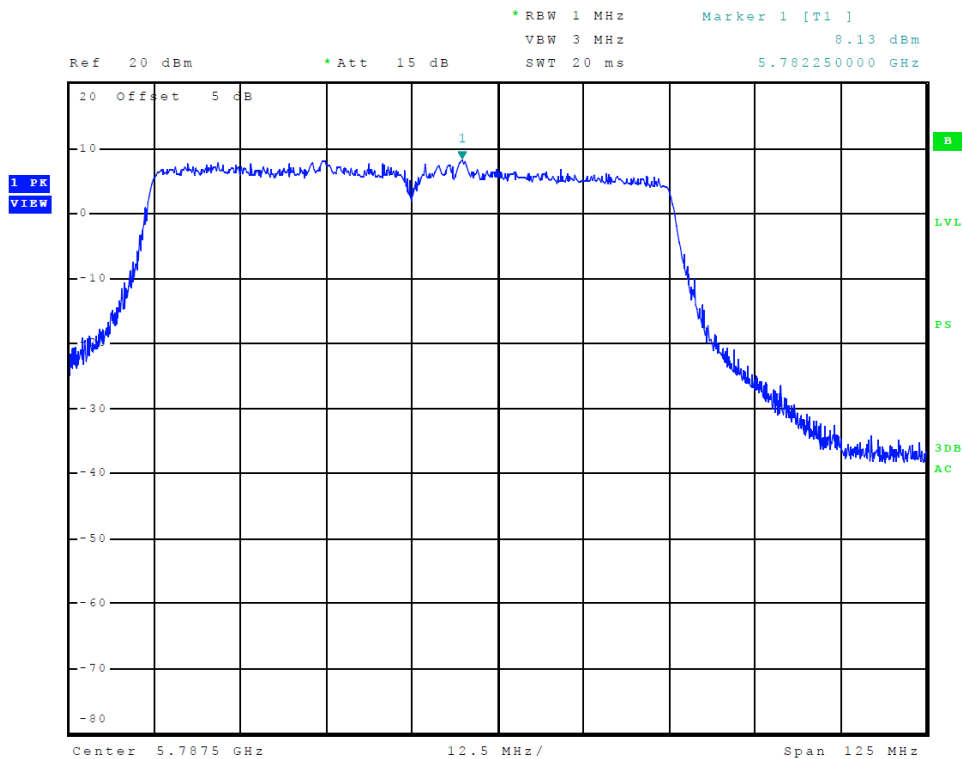
Figure 38 Plot of Transmitter Emissions (Chain 1, Across 5725-5850 MHz Band, 802.11ac80)
