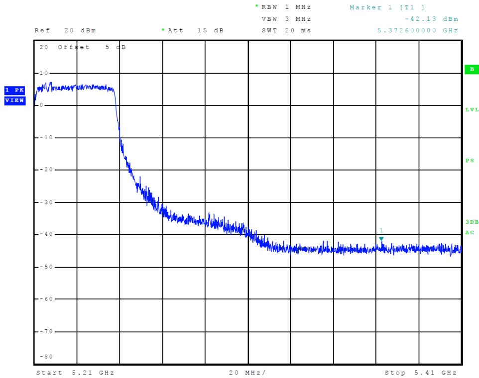
Figure 19 Plot of Transmitter High Band Edge (Chain 0, 5150-5250 MHz Band, 802.11ac80)
