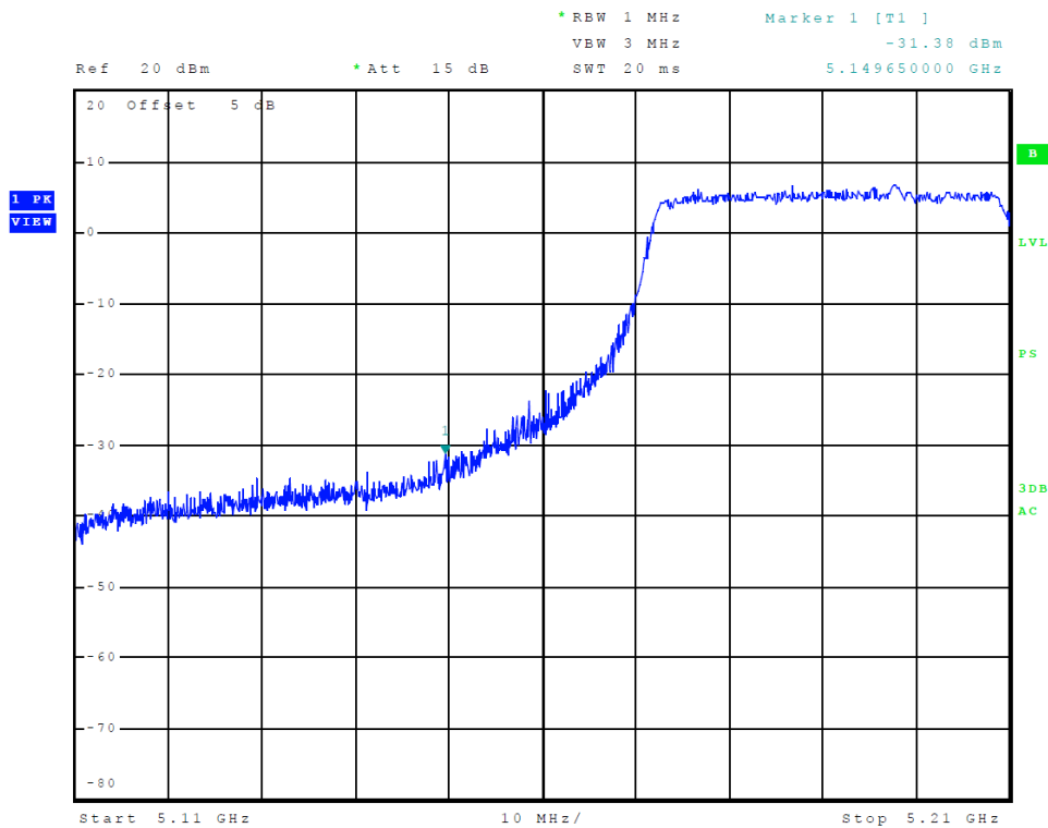
Figure 13 Plot of Transmitter Low Band Edge (Chain 0, 5150-5250 MHz Band, 802.11ac80)
