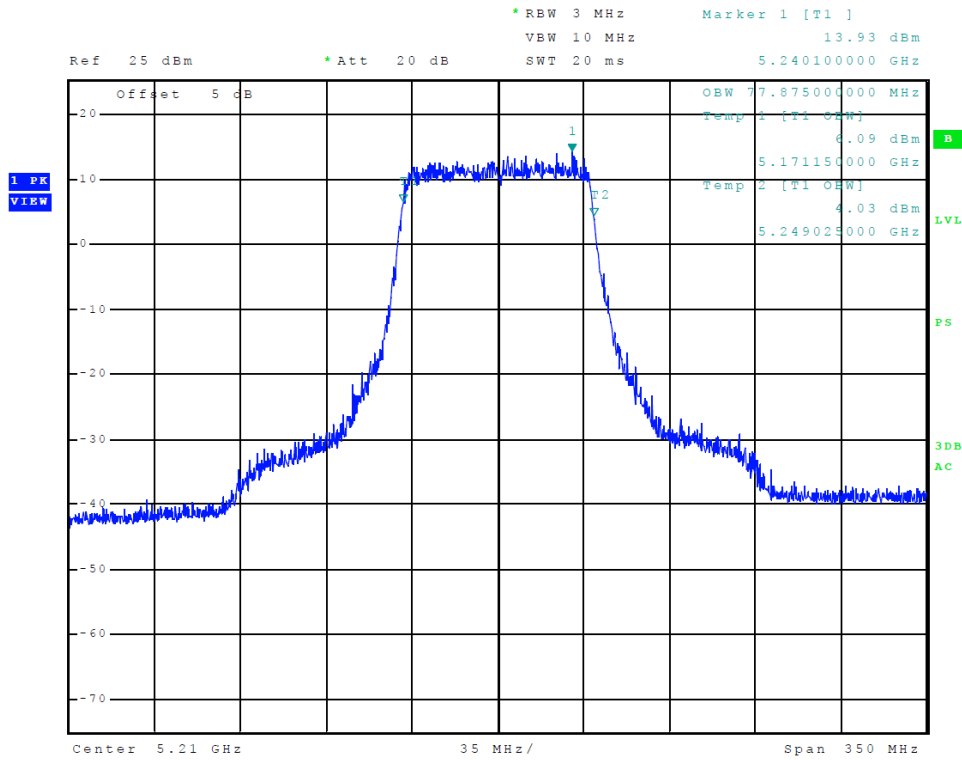
Figure 23 Plot of Transmitter Emissions (Chain 0, 5150-5250 MHz Band, 802.11ac, 99% OBW)
