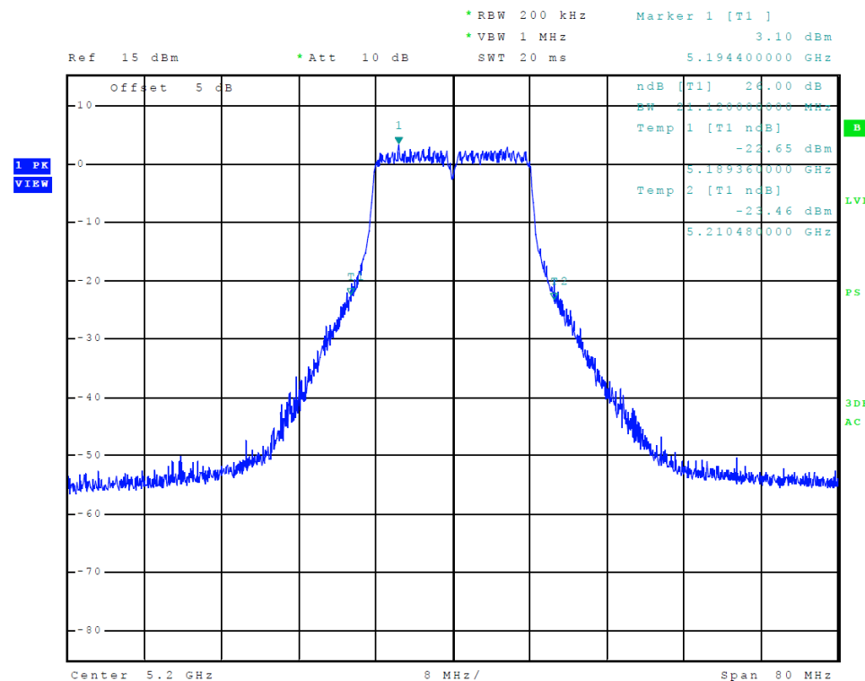
Figure 26 Plot of Transmitter Emissions (Chain 1, 5150-5250 MHz Band, 802.11a, 26 dB OBW)
