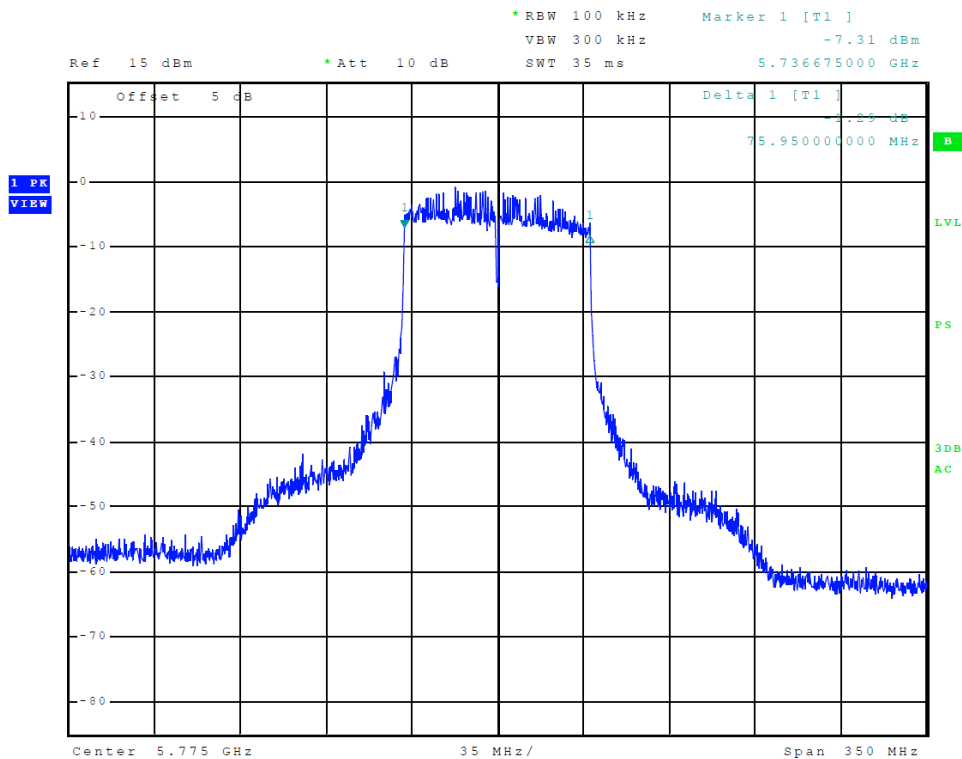
Figure 62 Plot of Transmitter Emissions (Chain 1, 5725-5850 MHz Band, 802.11ac80, 6-dB OBW)
