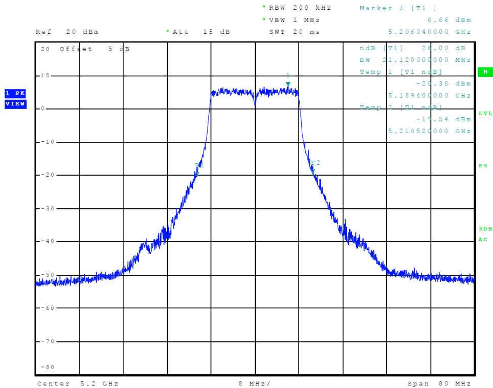
Figure 25 Plot of Transmitter Emissions (Chain 0, 5150-5250 MHz Band, 802.11a, 26 dB OBW)
