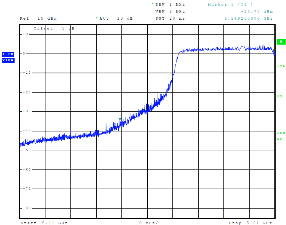
Figure 14 Plot of Transmitter Low Band Edge (Chain 1, 5150-5250 MHz Band, 802.11ac80)
