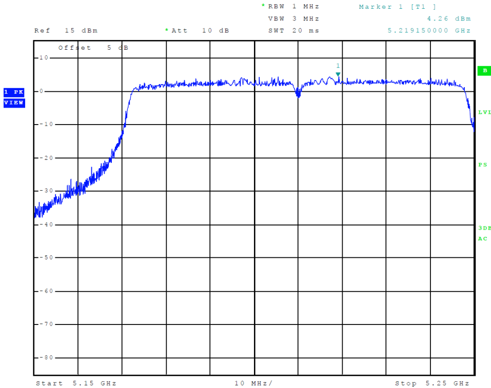
Figure 8 Plot of Transmitter Emissions (Chain 1, Across 5150-5250 MHz Band, 802.11ac80)
