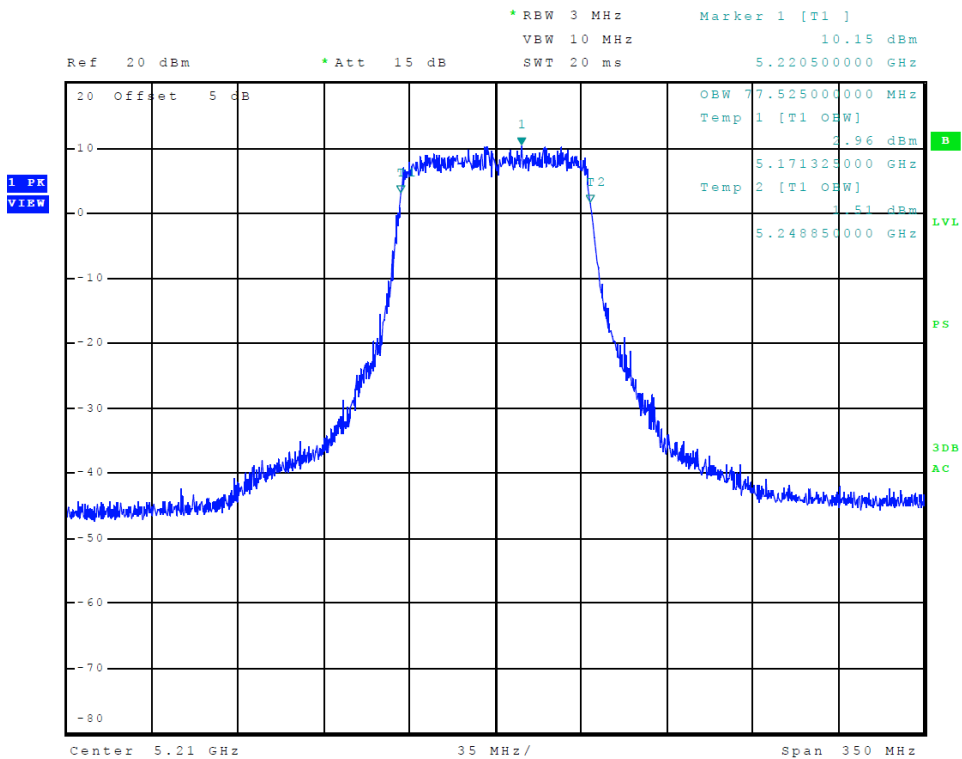
Figure 24 Plot of Transmitter Emissions (Chain 1, 5150-5250 MHz Band, 802.11ac, 99% OBW)
