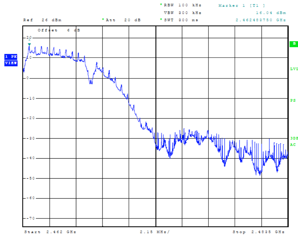
Figure 10 Plot of Transmitter High Band Edge (20 MHz Channel Chain 2)
