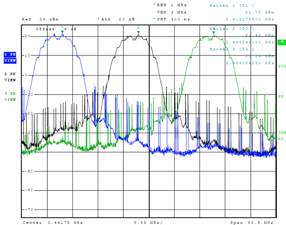
Figure 4 Plot of Transmitter Emissions (Across Operational Band, 20 MHz Channel, Chain 2)
