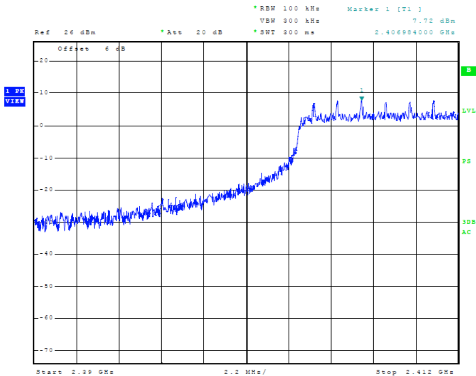
Figure 12 Plot of Transmitter Low Band Edge (40 MHz Channel Chain 2)
