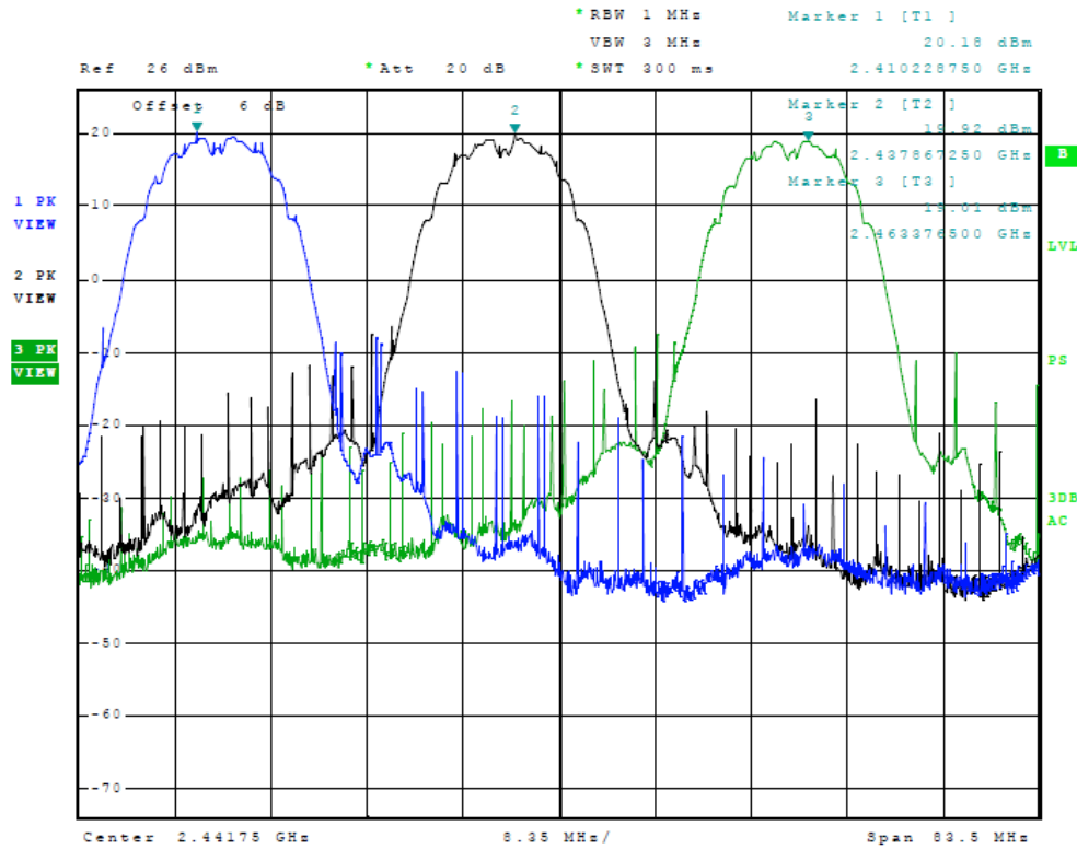
Figure 3 Plot of Transmitter Emissions (Across Operational Band, 20 MHz Channel, Chain 1)
