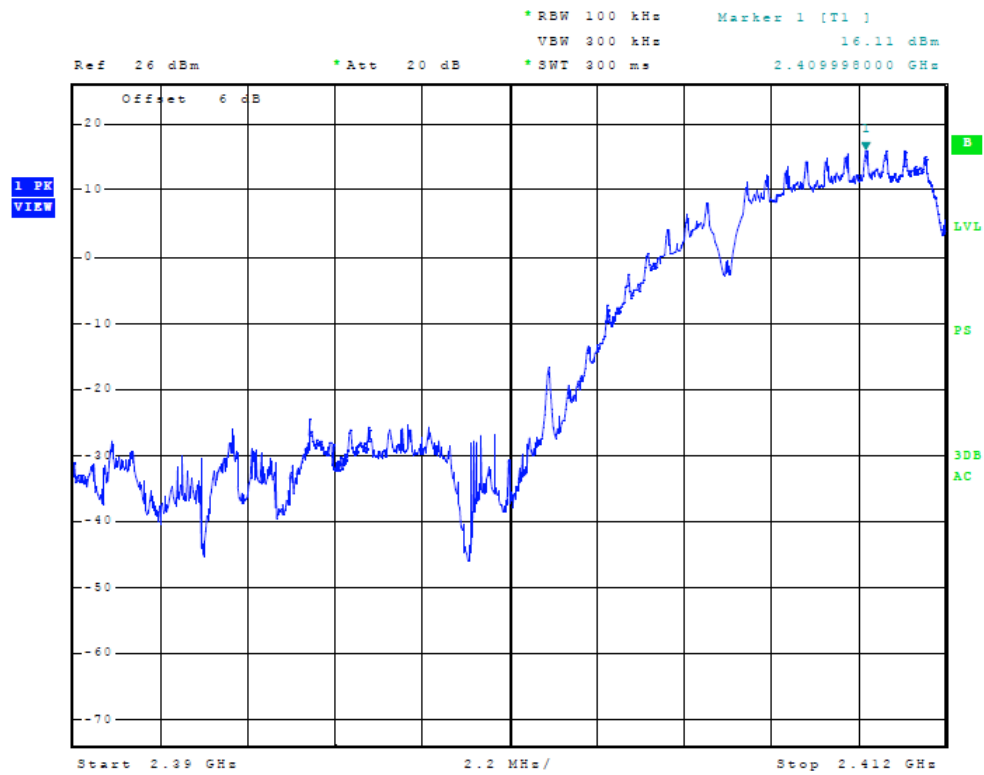
Figure 8 Plot of Transmitter Low Band Edge (20 MHz Channel Chain 2)
