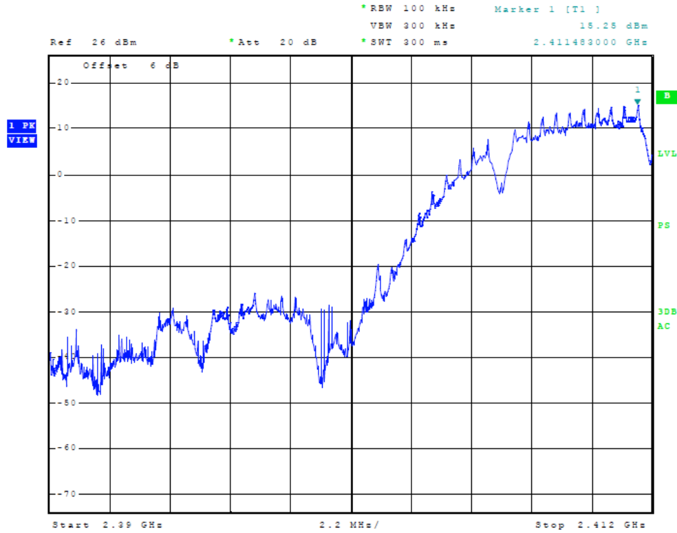
Figure 7 Plot of Transmitter Low Band Edge (20 MHz Channel Chain 1)
