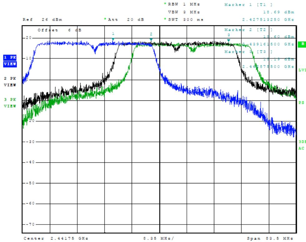
Figure 5 Plot of Transmitter Emissions (Across Operational Band, 40 MHz Channel Chain 1)
