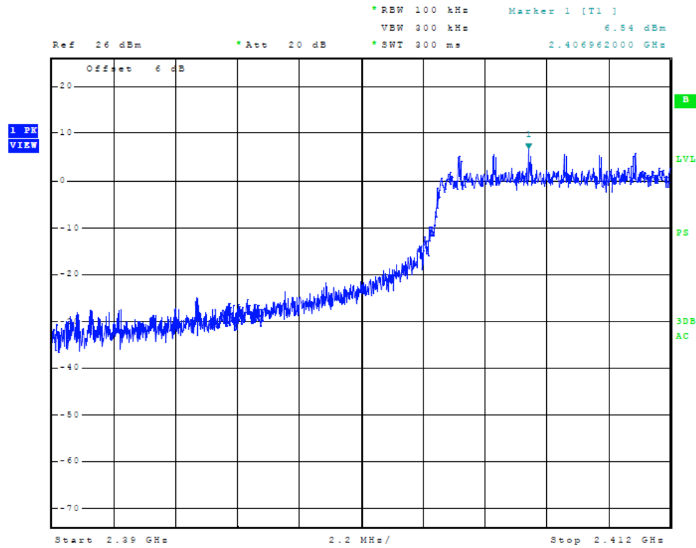
Figure 11 Plot of Transmitter Low Band Edge (40 MHz Channel Chain 1)
