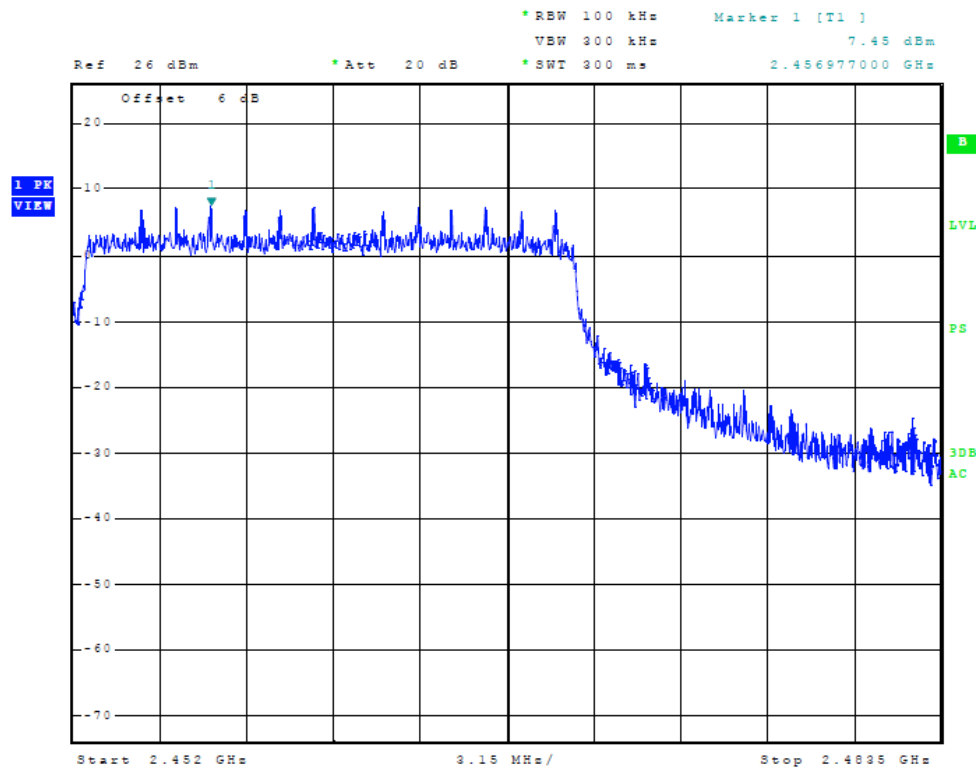
Figure 14 Plot of Transmitter High Band Edge (40 MHz Channel Chain 2)
