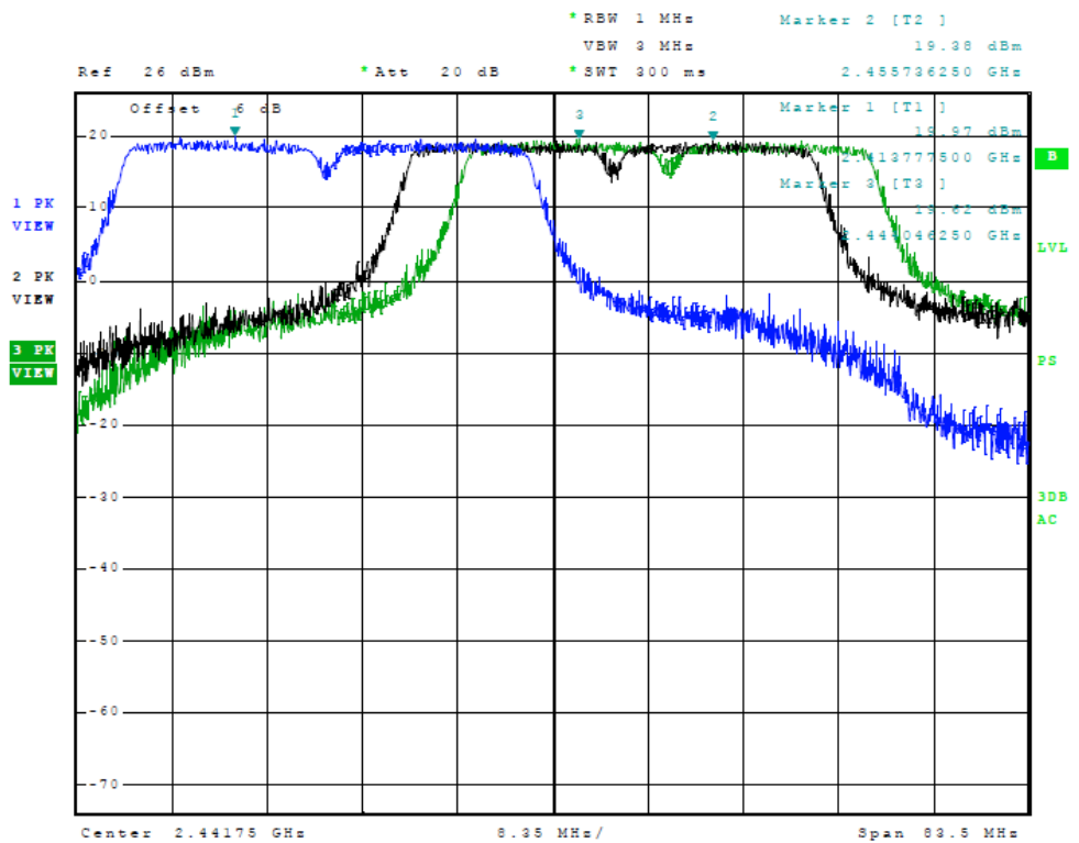
Figure 6 Plot of Transmitter Emissions (Across Operational Band, 40 MHz Channel Chain 2)
