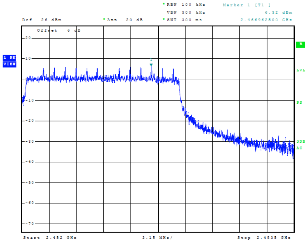
Figure 13 Plot of Transmitter High Band Edge (40 MHz Channel Chain 1)
