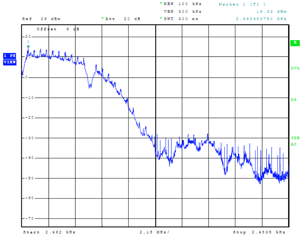
Figure 9 Plot of Transmitter High Band Edge (20 MHz Channel Chain 1)
