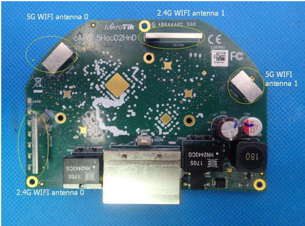
WIFI ANTENNA
