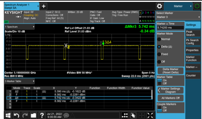
802.11ax-HE40 (T = 5.390ms)
