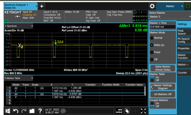
802.11ax-HE80 (T = 5.412ms)
