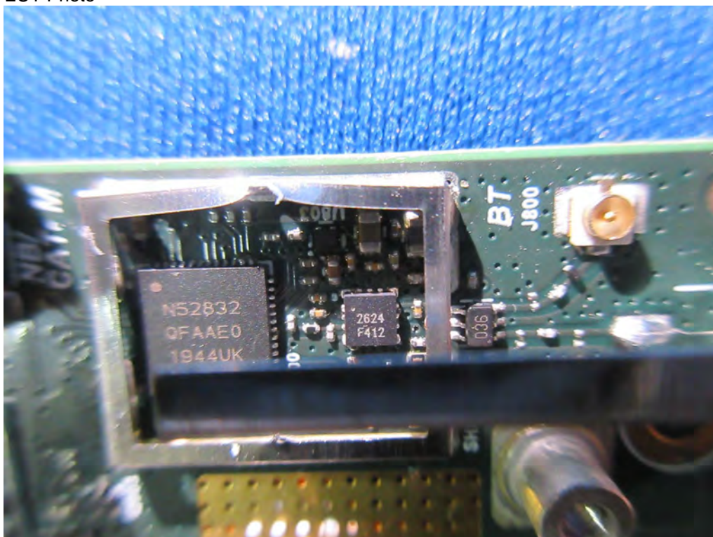
(32) EUT Photo
