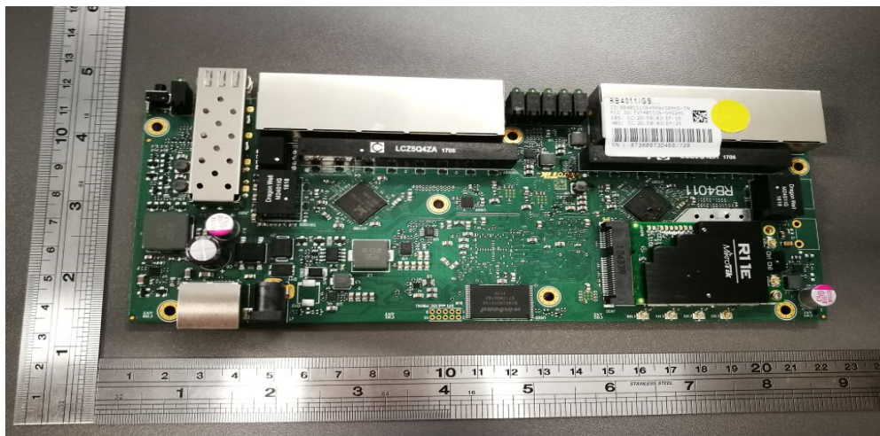
PCB TOP with shields and R11E card
