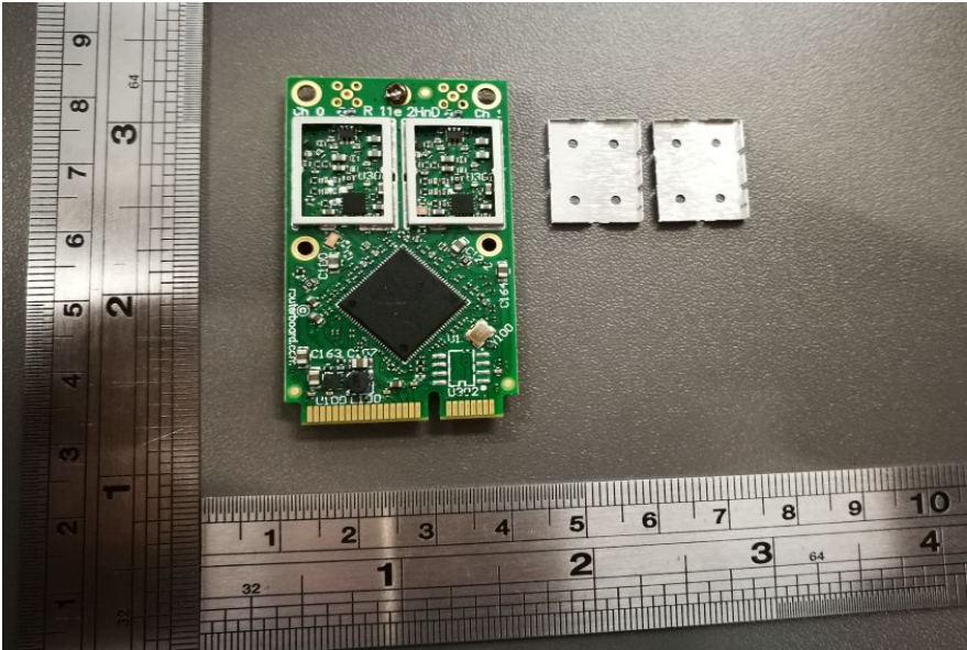
R11E card BACK without shields
