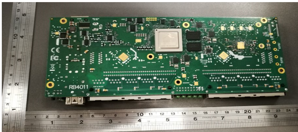
PCB TOP without shields and R11E card
