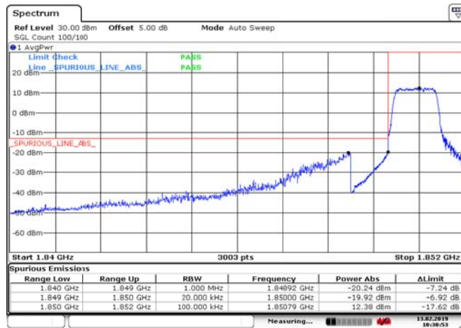
Band2_1.4MHz_QPSK_18607_6RB#0
