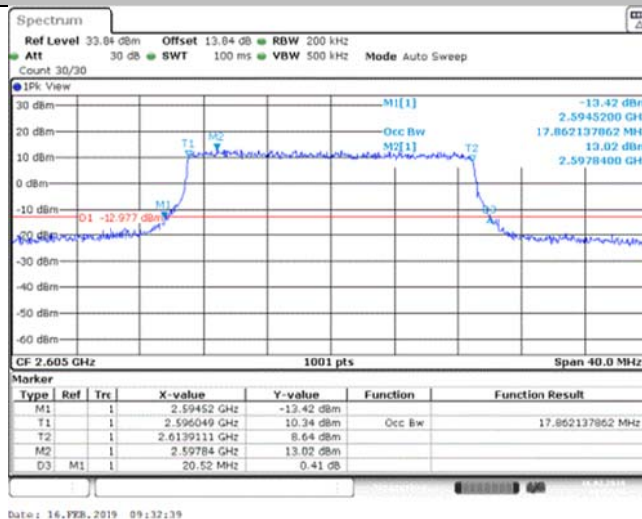
Band41_20MHz_16QAM_40740_100RB#0
