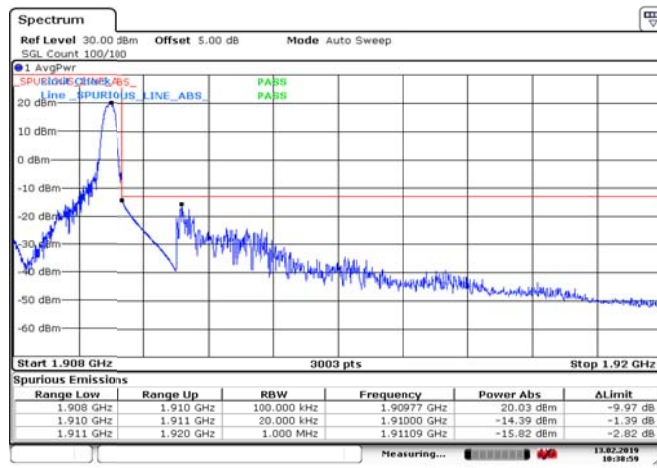
Band2_1.4MHz_QPSK_19193_1RB#5
