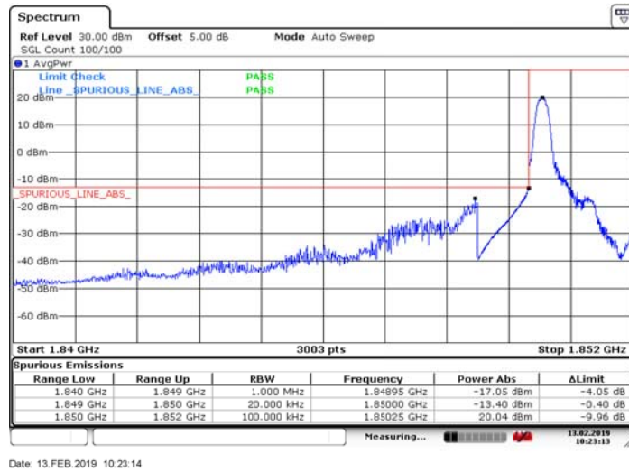
Band2_1.4MHz_QPSK_18607_6RB#0
