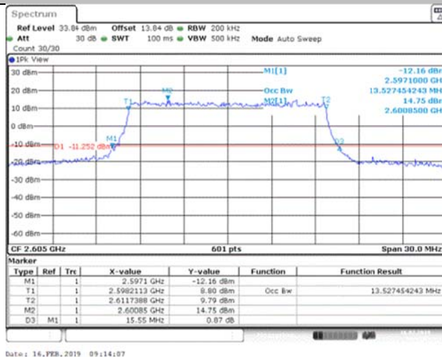
Band41_15MHz_16QAM_40740_75RB#0
