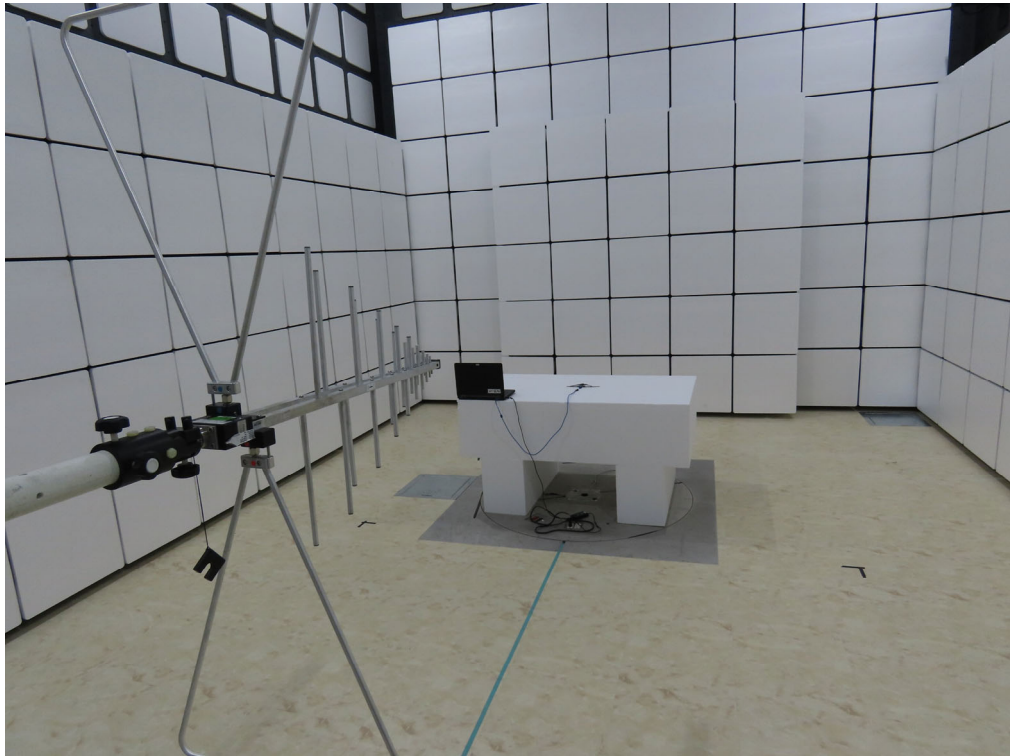
Radiated Test
