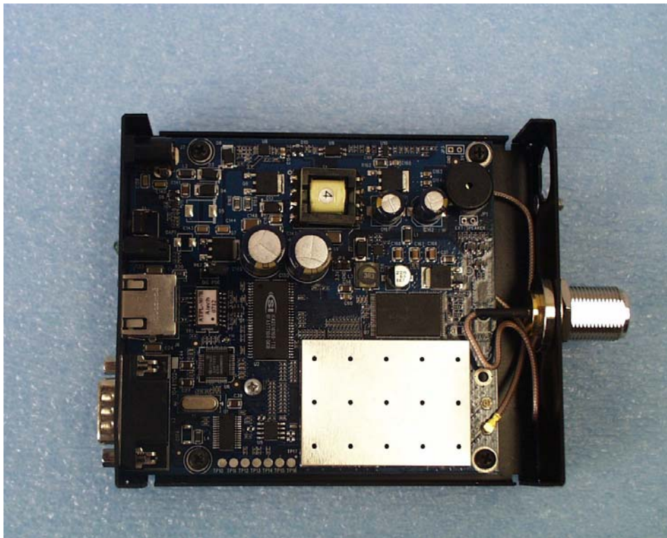
Mounted Printer Circuit Board
