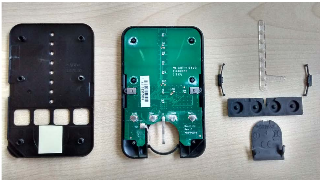
Case Open – PCB component side
