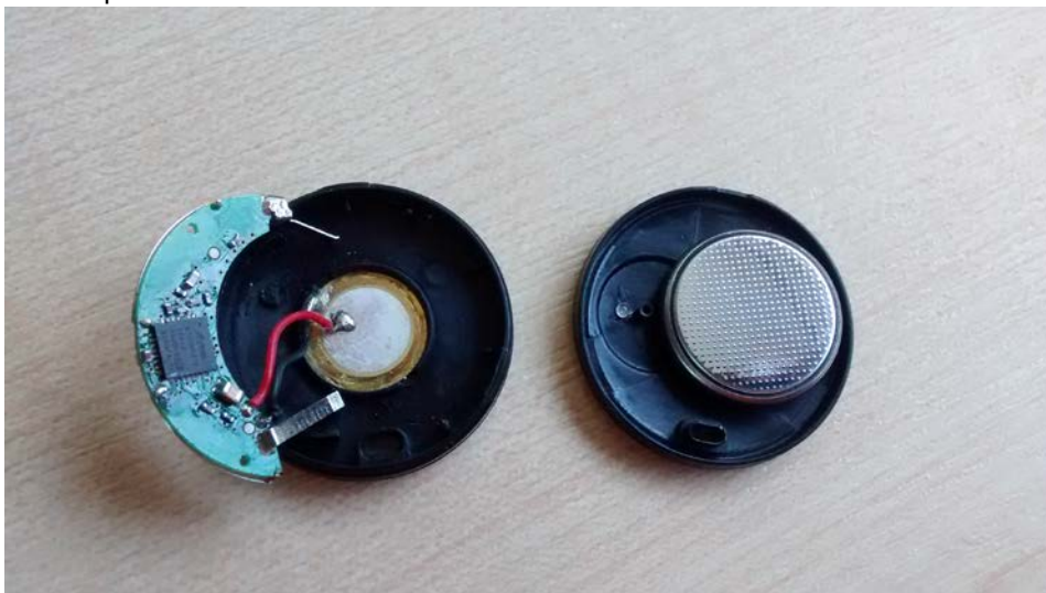
Case Open – PCB Underside
